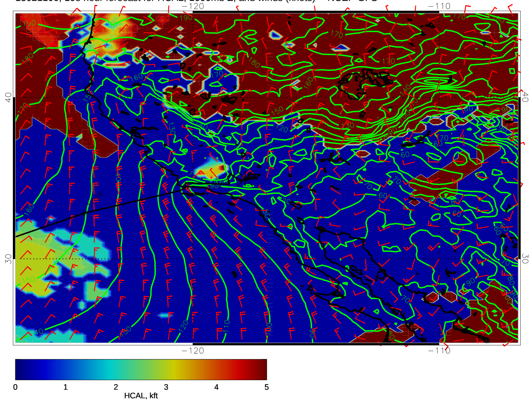
15021100, 108 hour forecast for HCAL, 1000mb Z, and winds (knots) -- NCEP GFS
