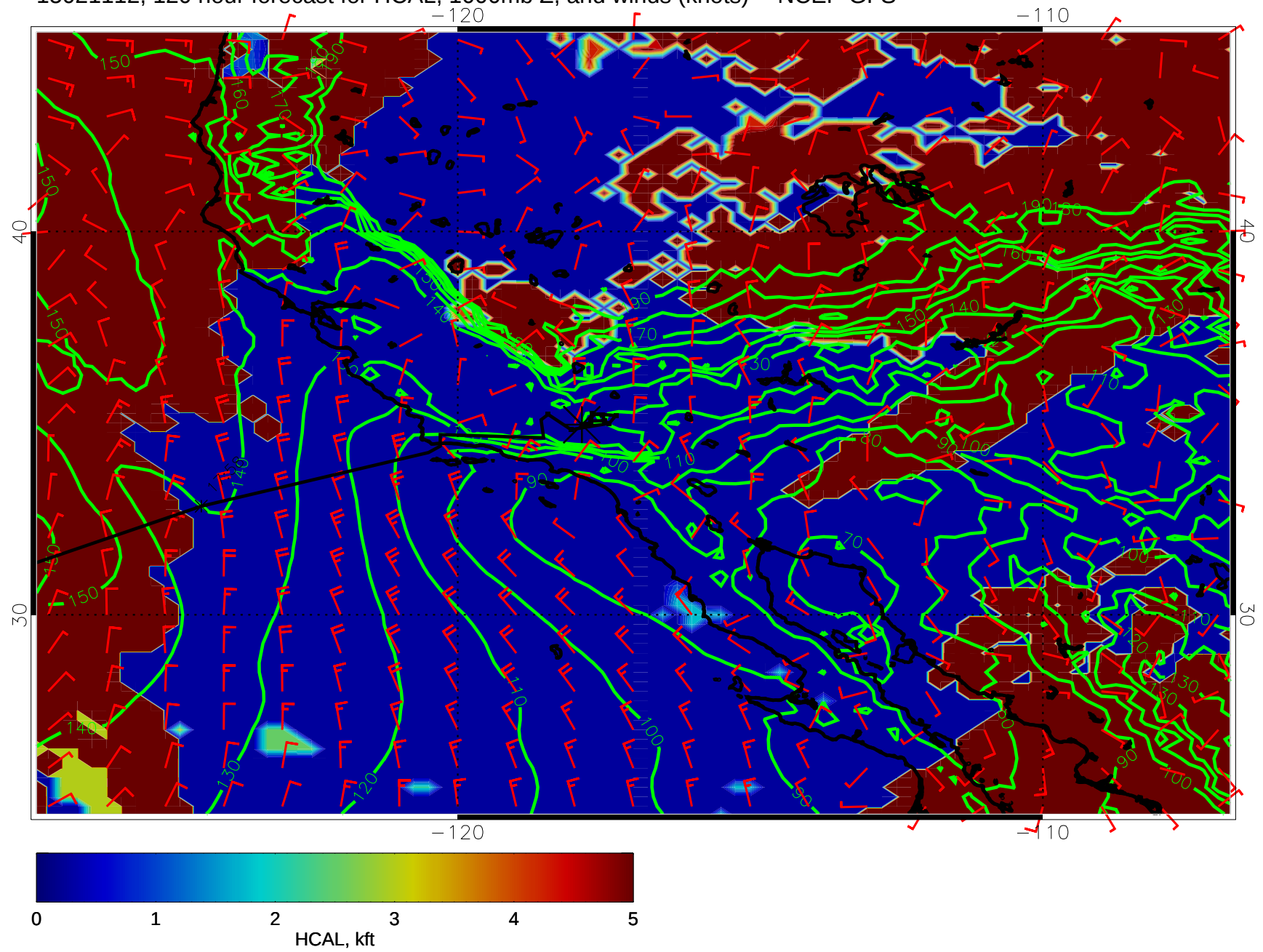
15021112, 120 hour forecast for HCAL, 1000mb Z, and winds (knots) -- NCEP GFS
