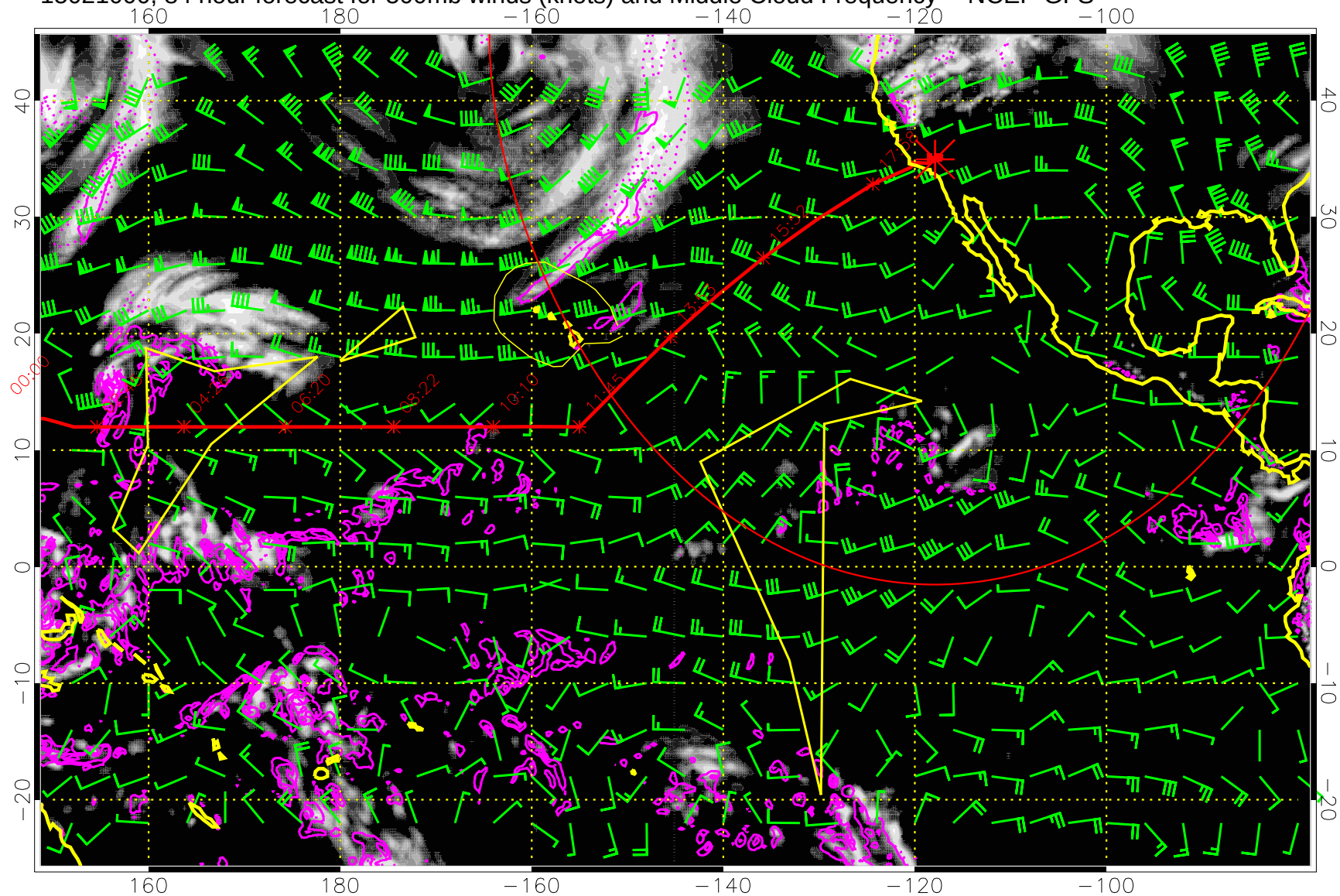
15021000, 84 hour forecast for 500mb winds (knots) and Middle Cloud Frequency -- NCEP GFS
