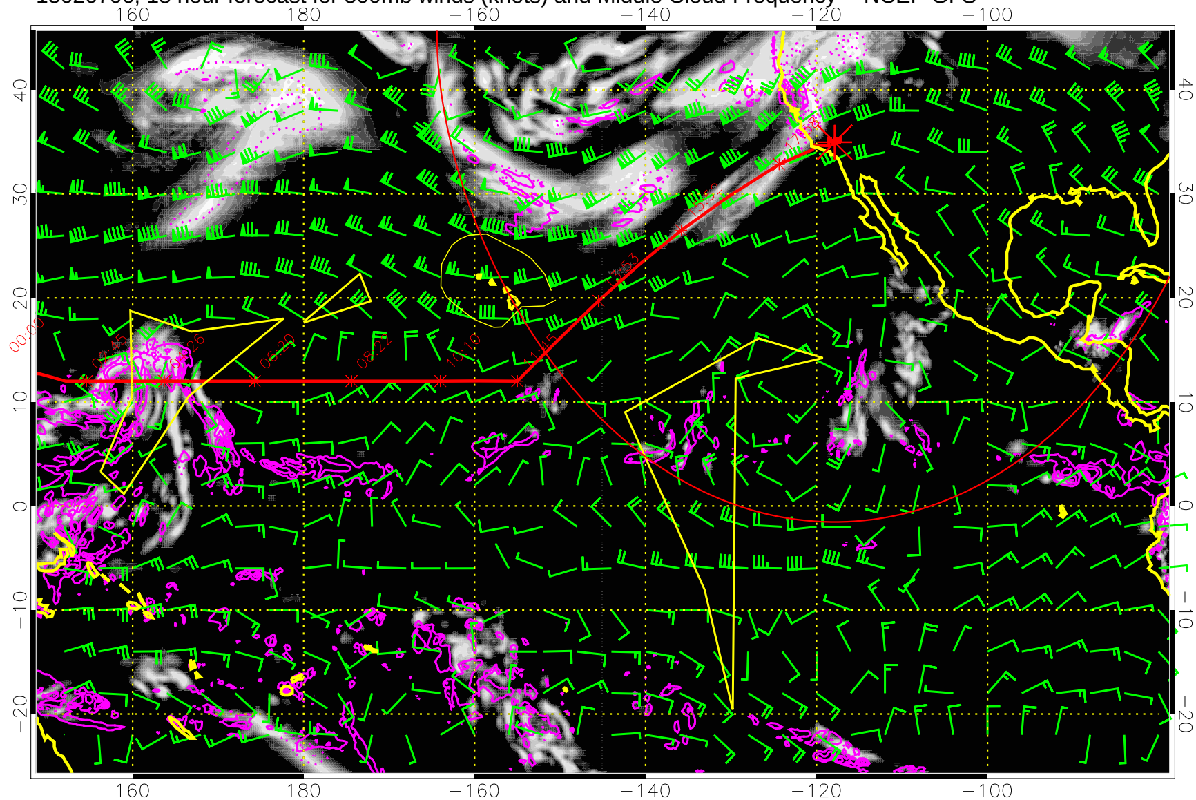
15020706, 18 hour forecast for 500mb winds (knots) and Middle Cloud Frequency -- NCEP GFS
