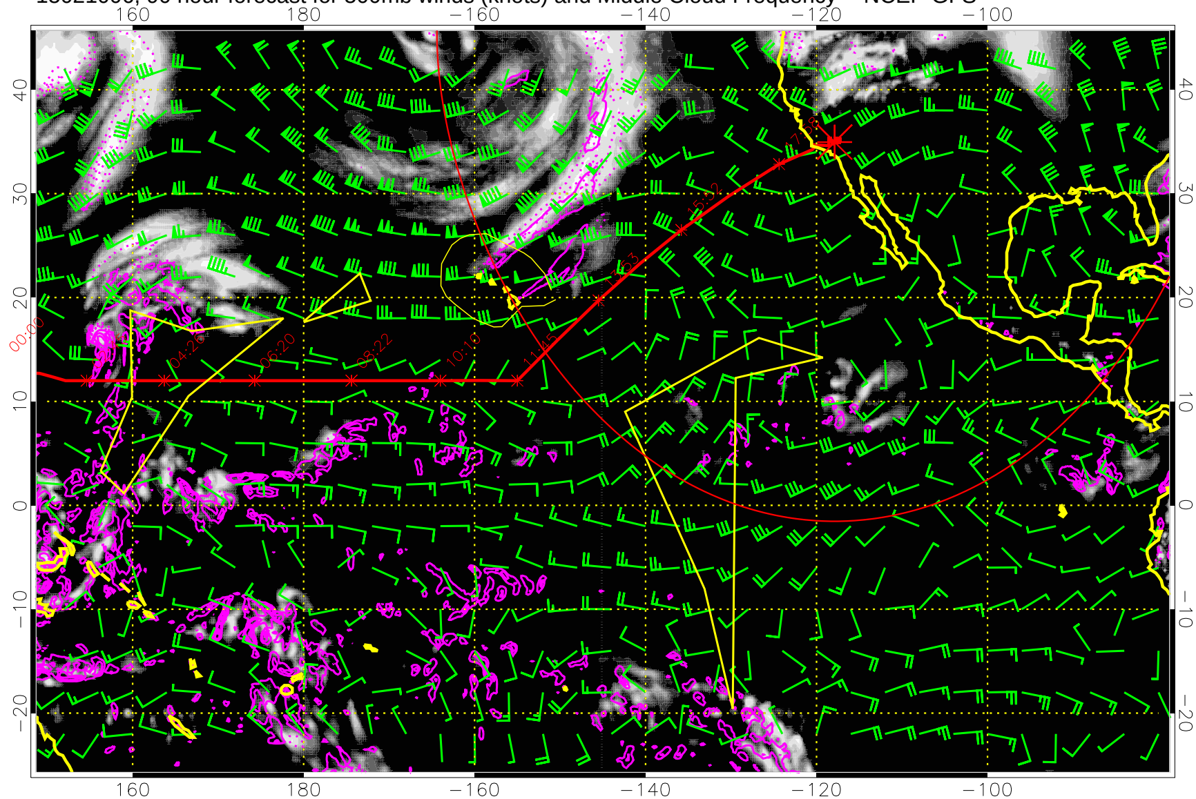
15021006, 90 hour forecast for 500mb winds (knots) and Middle Cloud Frequency -- NCEP GFS
