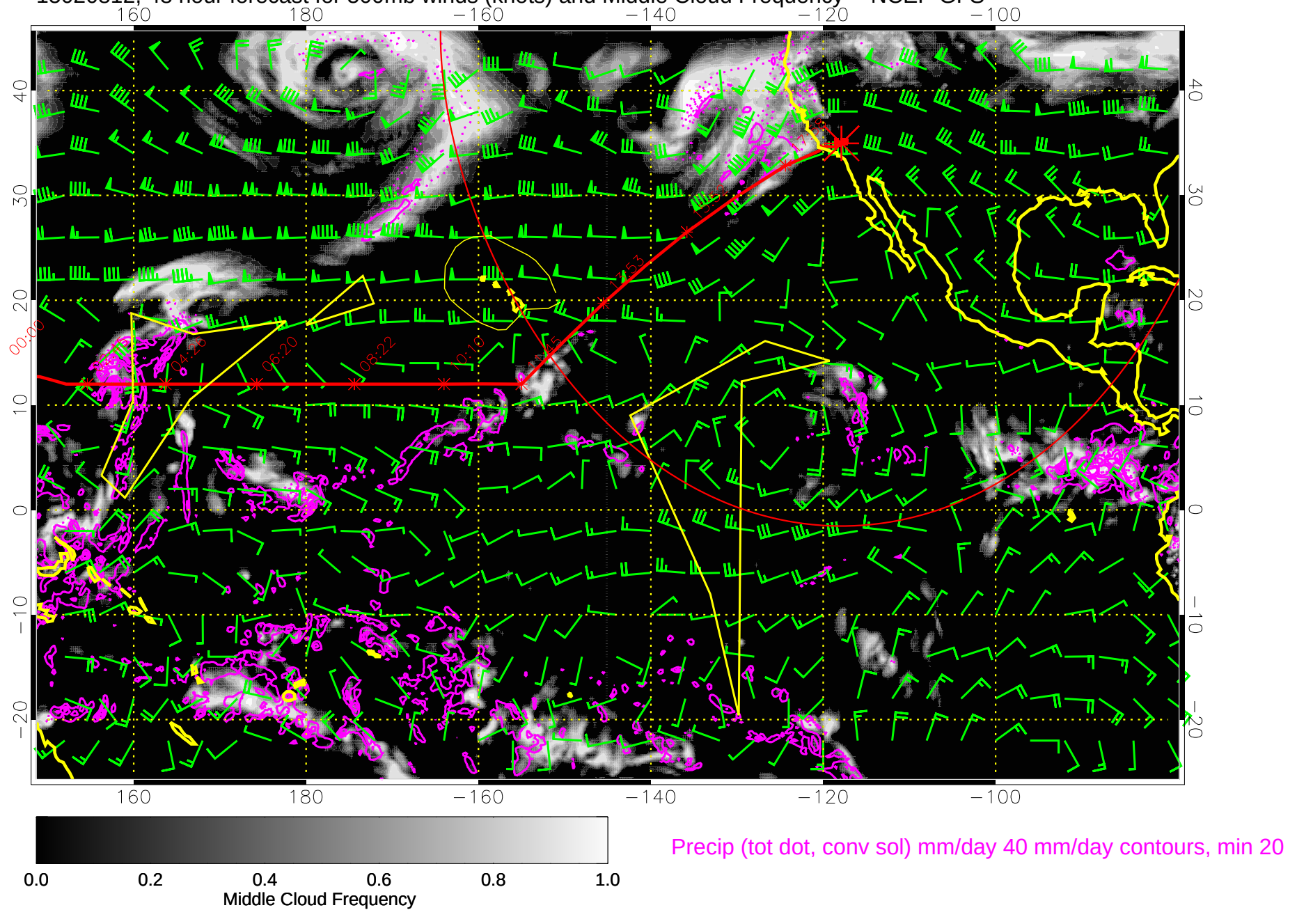
15020812, 48 hour forecast for 500mb winds (knots) and Middle Cloud Frequency -- NCEP GFS
