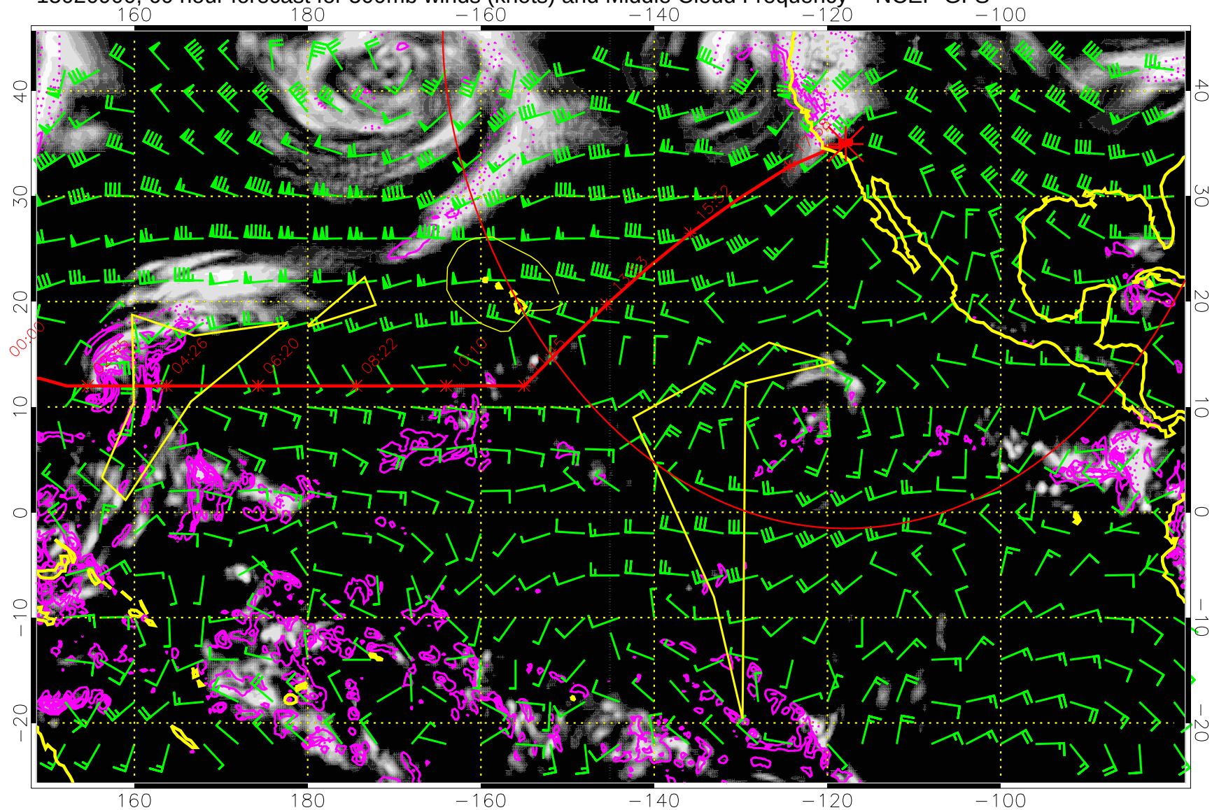
15020900, 60 hour forecast for 500mb winds (knots) and Middle Cloud Frequency -- NCEP GFS
