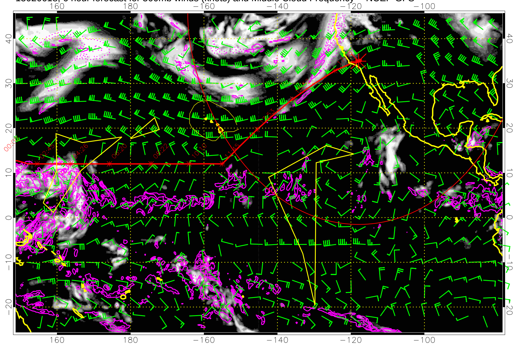
15020618, 6 hour forecast for 500mb winds (knots) and Middle Cloud Frequency -- NCEP GFS
