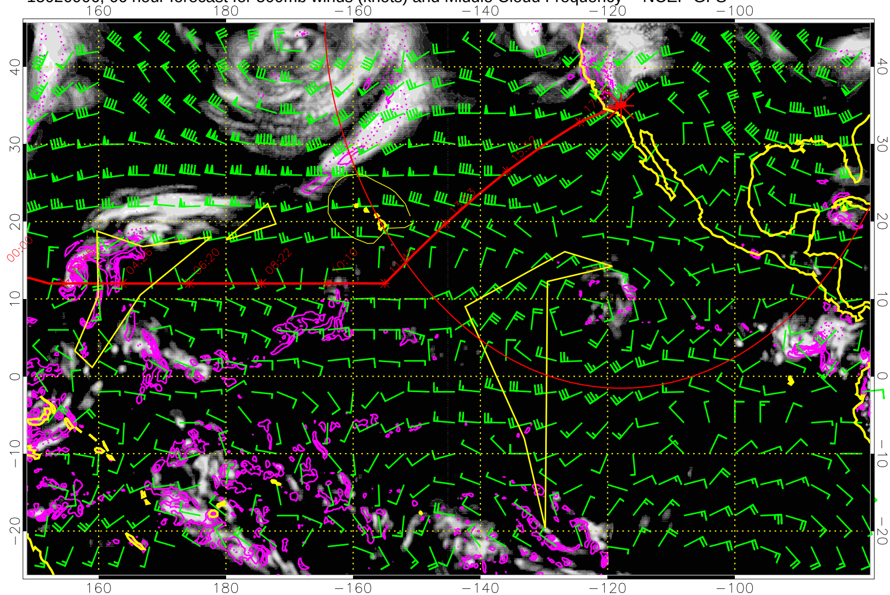
15020906, 66 hour forecast for 500mb winds (knots) and Middle Cloud Frequency -- NCEP GFS
