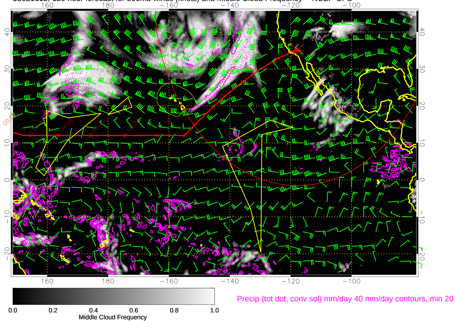
15021112, 120 hour forecast for 500mb winds (knots) and Middle Cloud Frequency -- NCEP GFS
