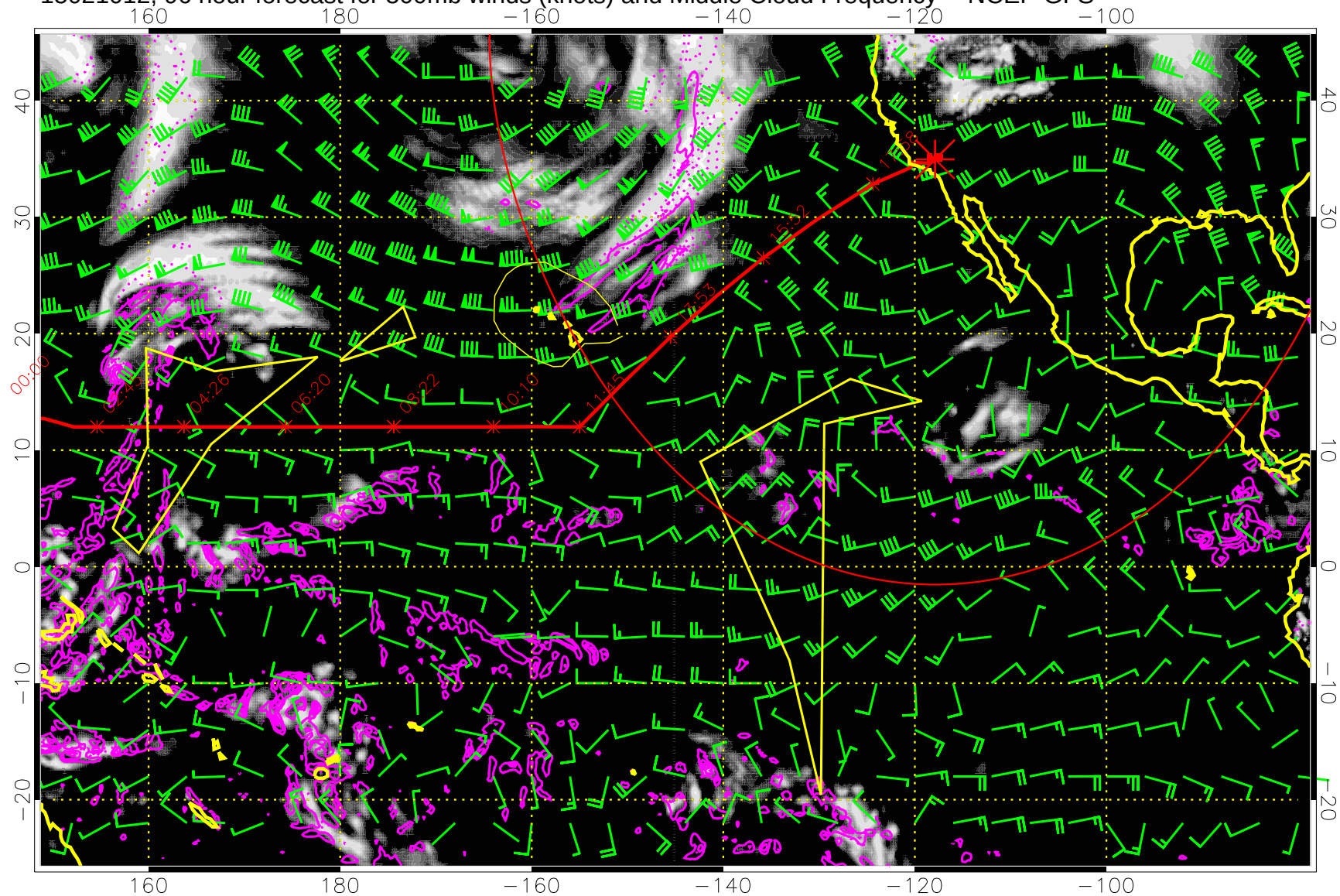
15021012, 96 hour forecast for 500mb winds (knots) and Middle Cloud Frequency -- NCEP GFS
