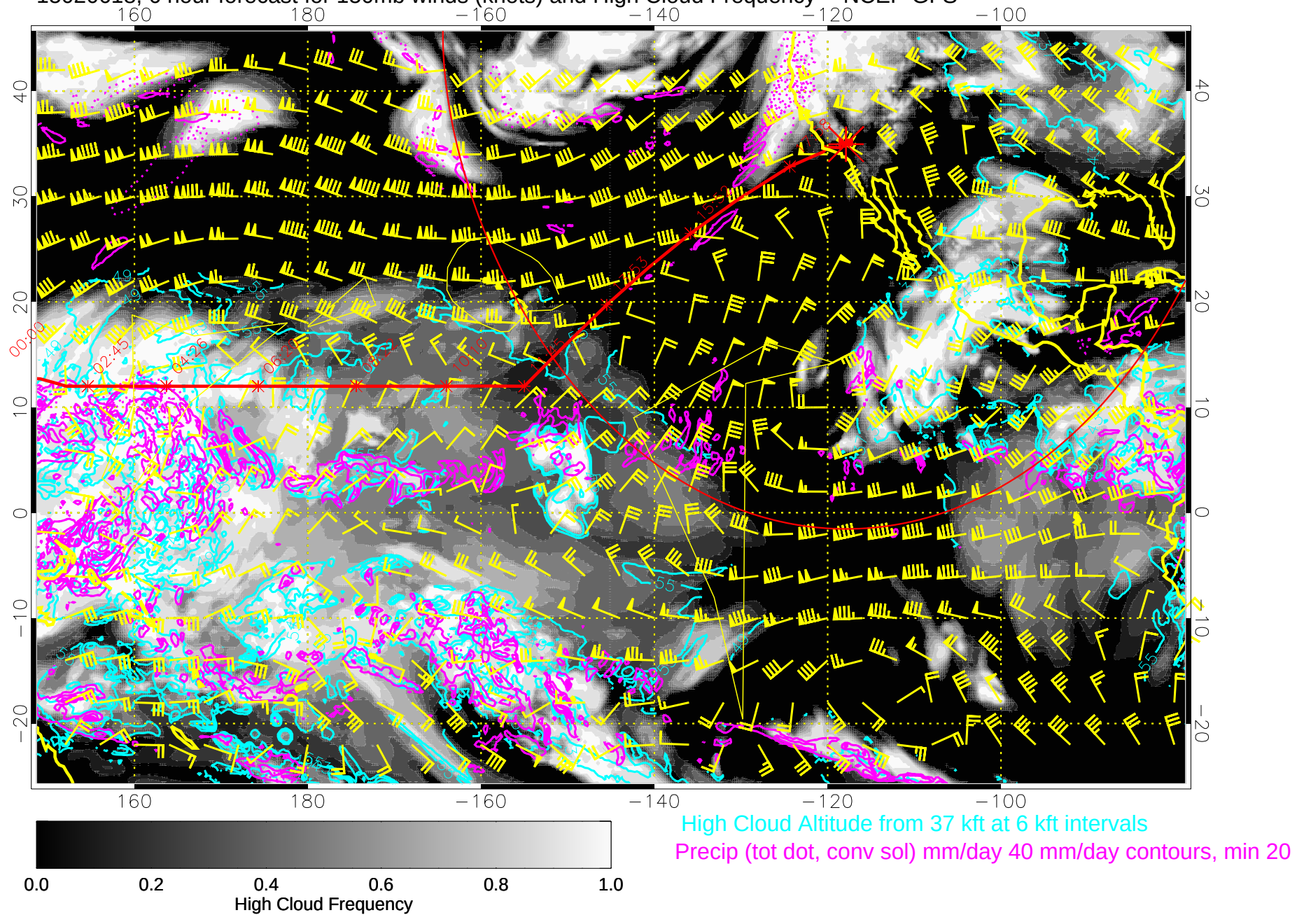
15020618, 6 hour forecast for 150mb winds (knots) and High Cloud Frequency -- NCEP GFS
