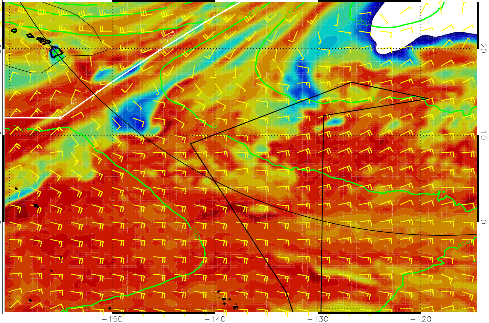
20020100, 00 Near Forecast for Storms (km, h, and winds (knots)) 20020100 20020100 20020100 20020100 -150 -140 -130 -120
