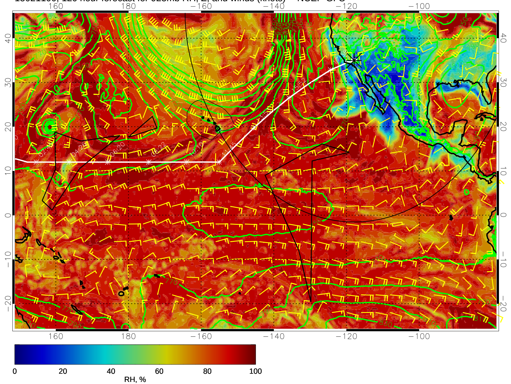
15021100, 120 hour forecast for 925mb RH, Z, and winds (knots) -- NCEP GFS
