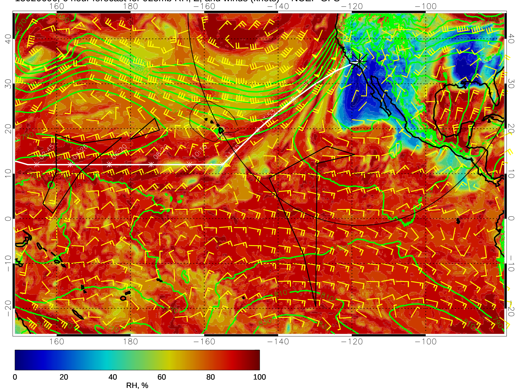
15020606, 6 hour forecast for 925mb RH, Z, and winds (knots) -- NCEP GFS
