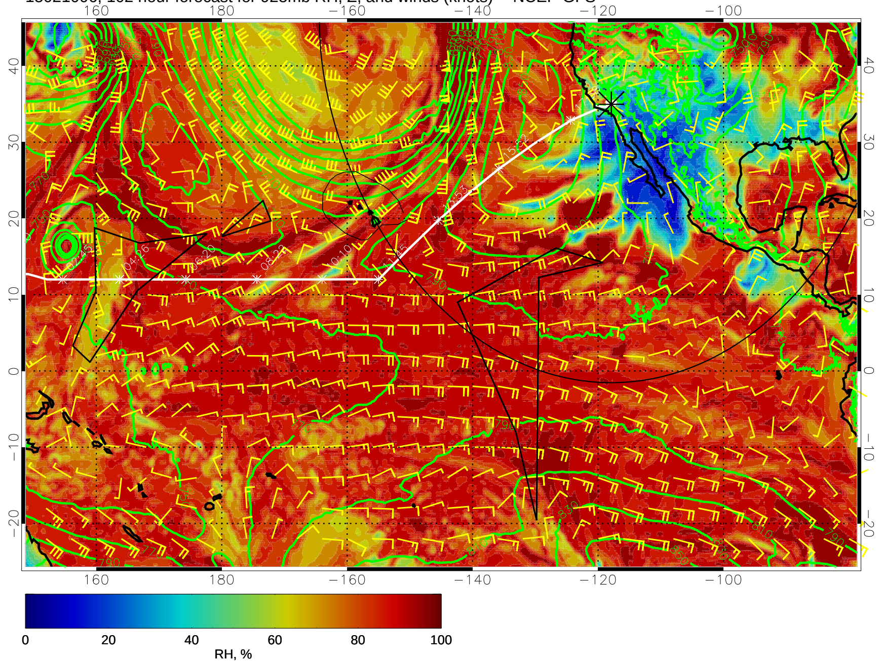
15021006, 102 hour forecast for 925mb RH, Z, and winds (knots) -- NCEP GFS
