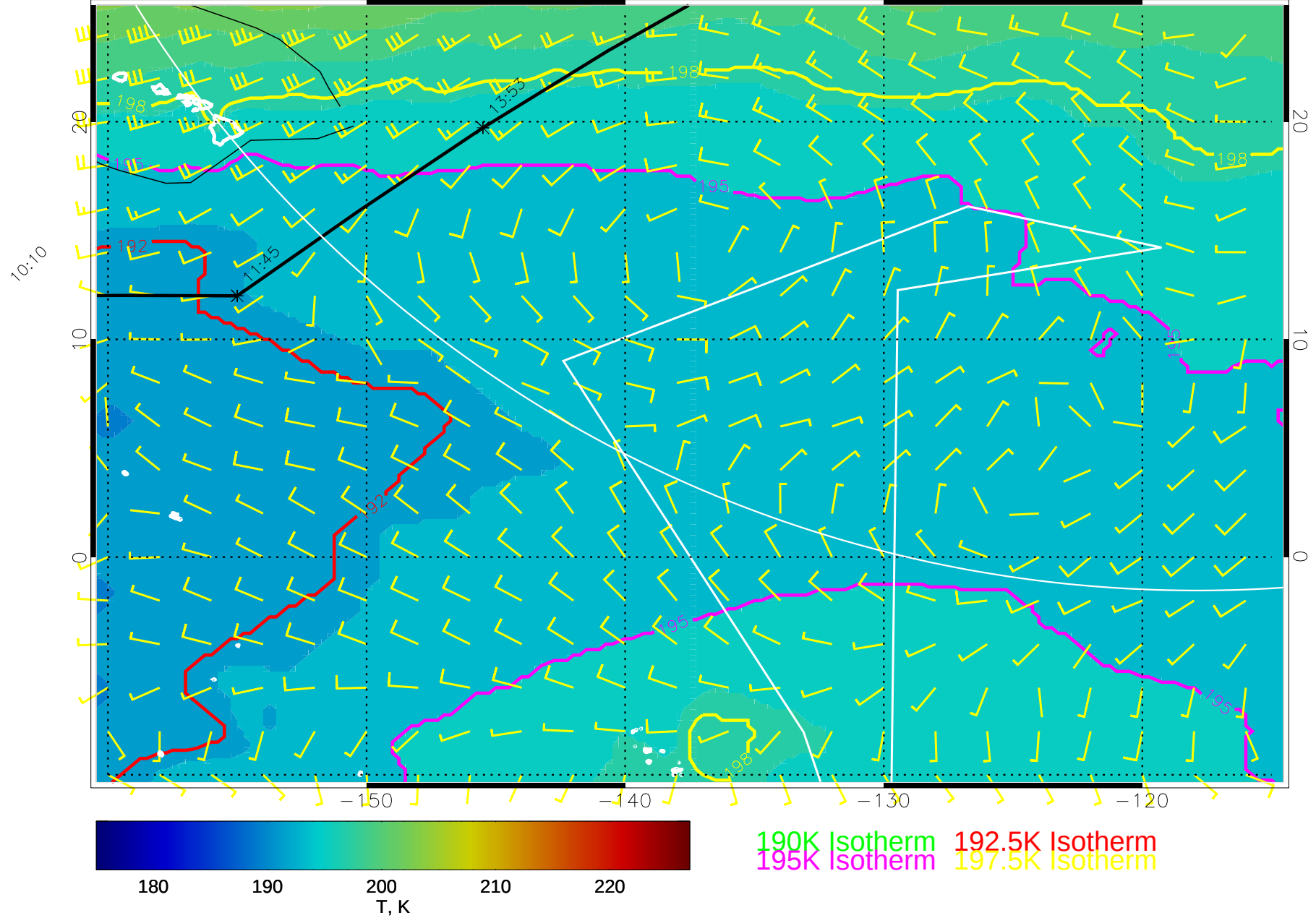
15021012, 108 hour forecast for 70mb T and winds (knots) -- NCEP GFS
