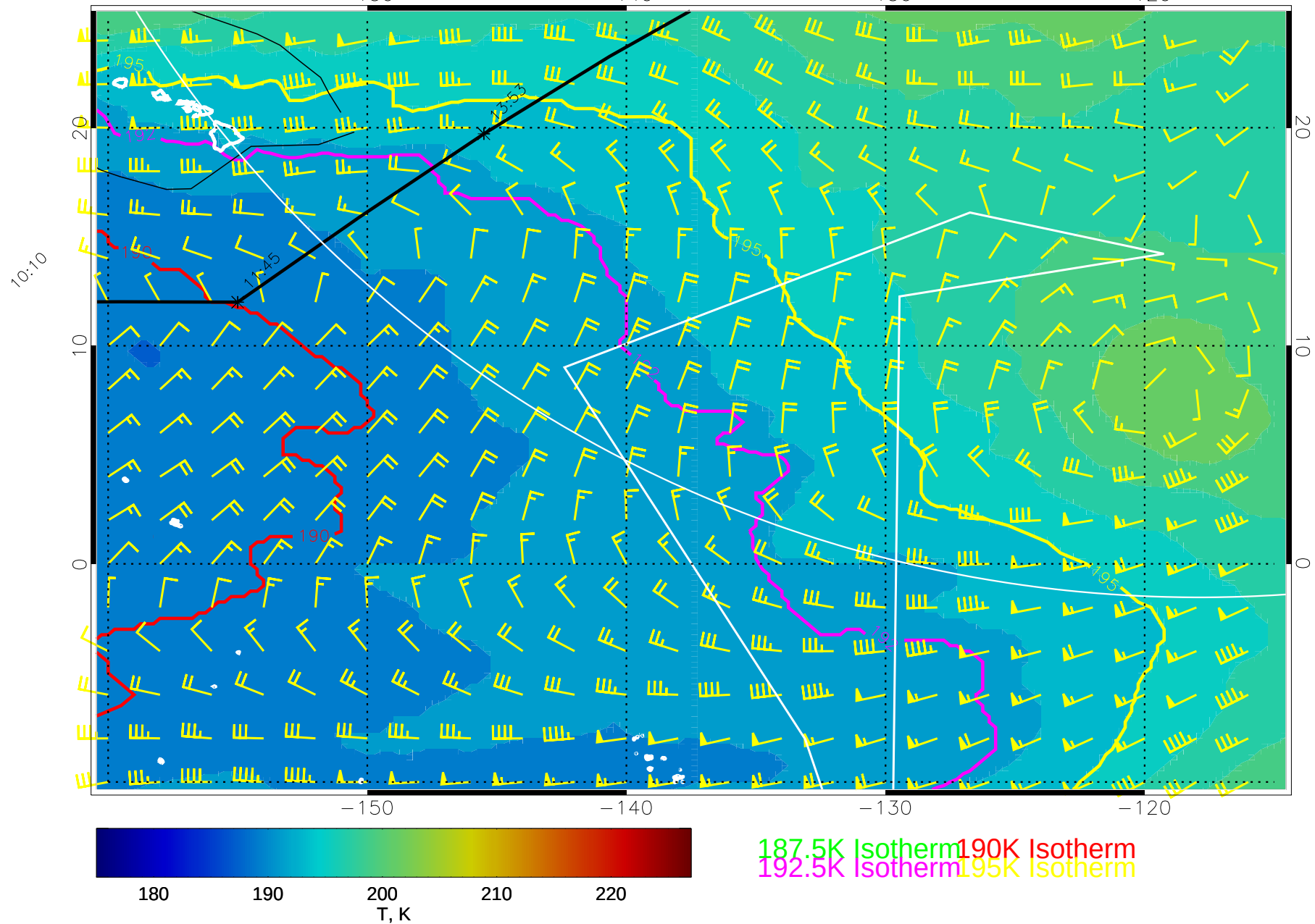
15021000, 96 hour forecast for 100mb T and winds (knots) -- NCEP GFS
