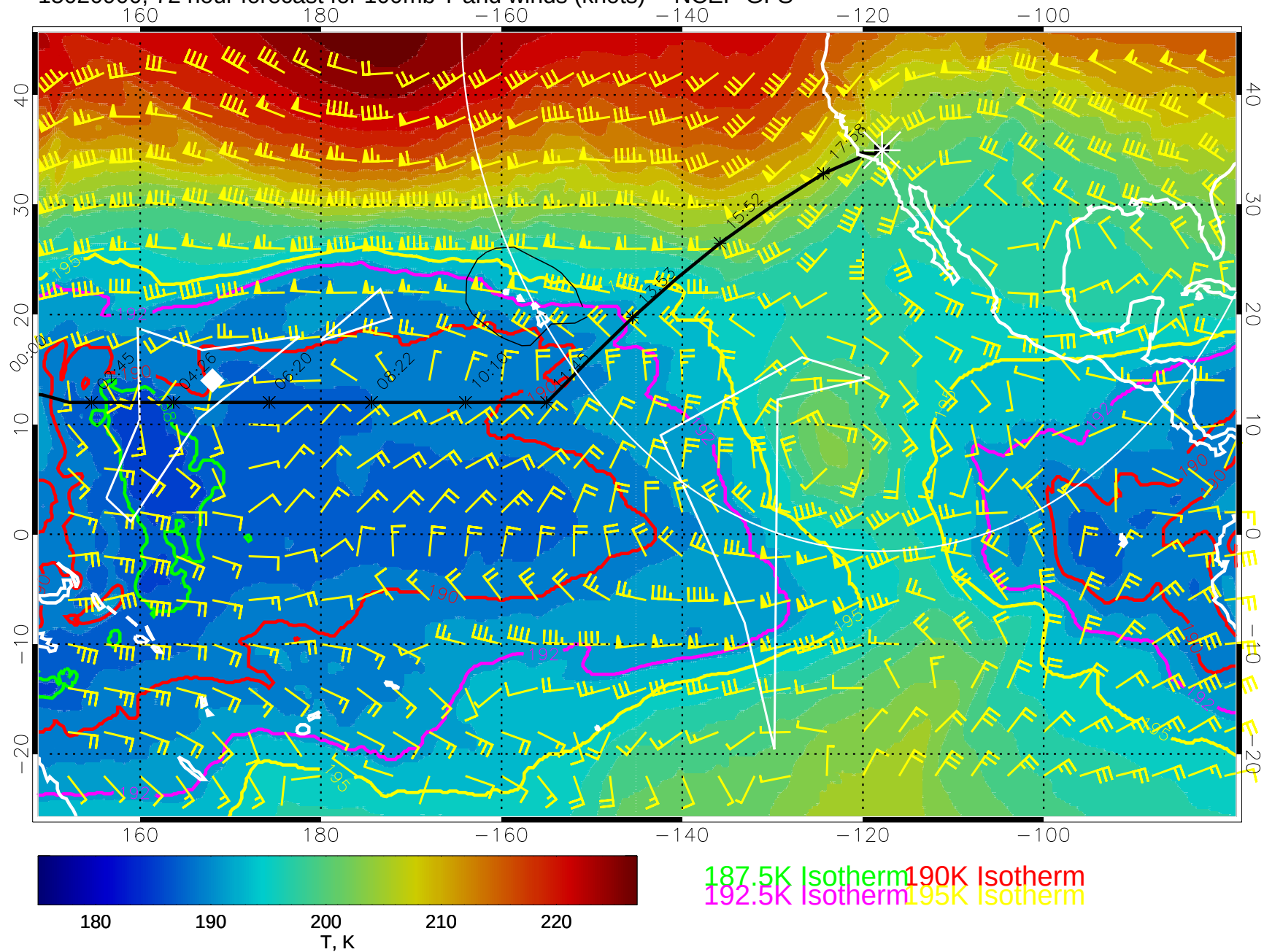
15020900, 72 hour forecast for 100mb T and winds (knots) -- NCEP GFS
