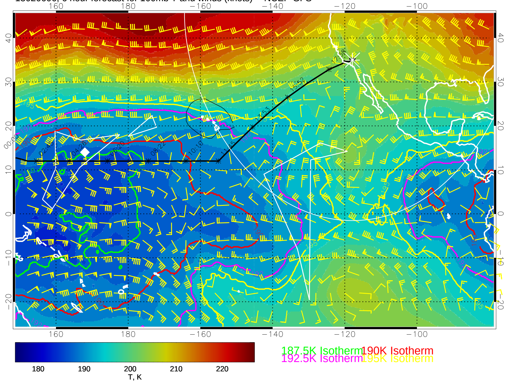
15020606, 6 hour forecast for 100mb T and winds (knots) -- NCEP GFS
