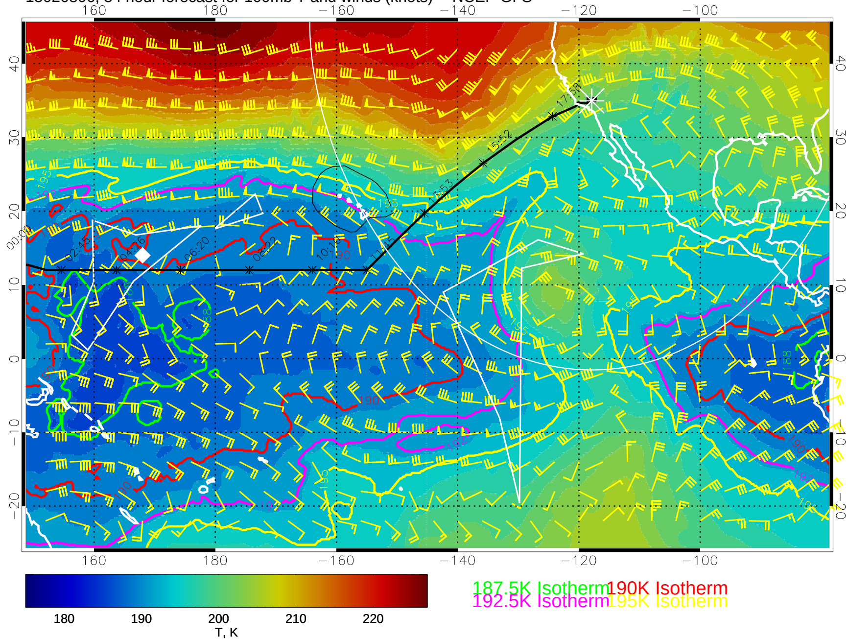
15020806, 54 hour forecast for 100mb T and winds (knots) -- NCEP GFS
