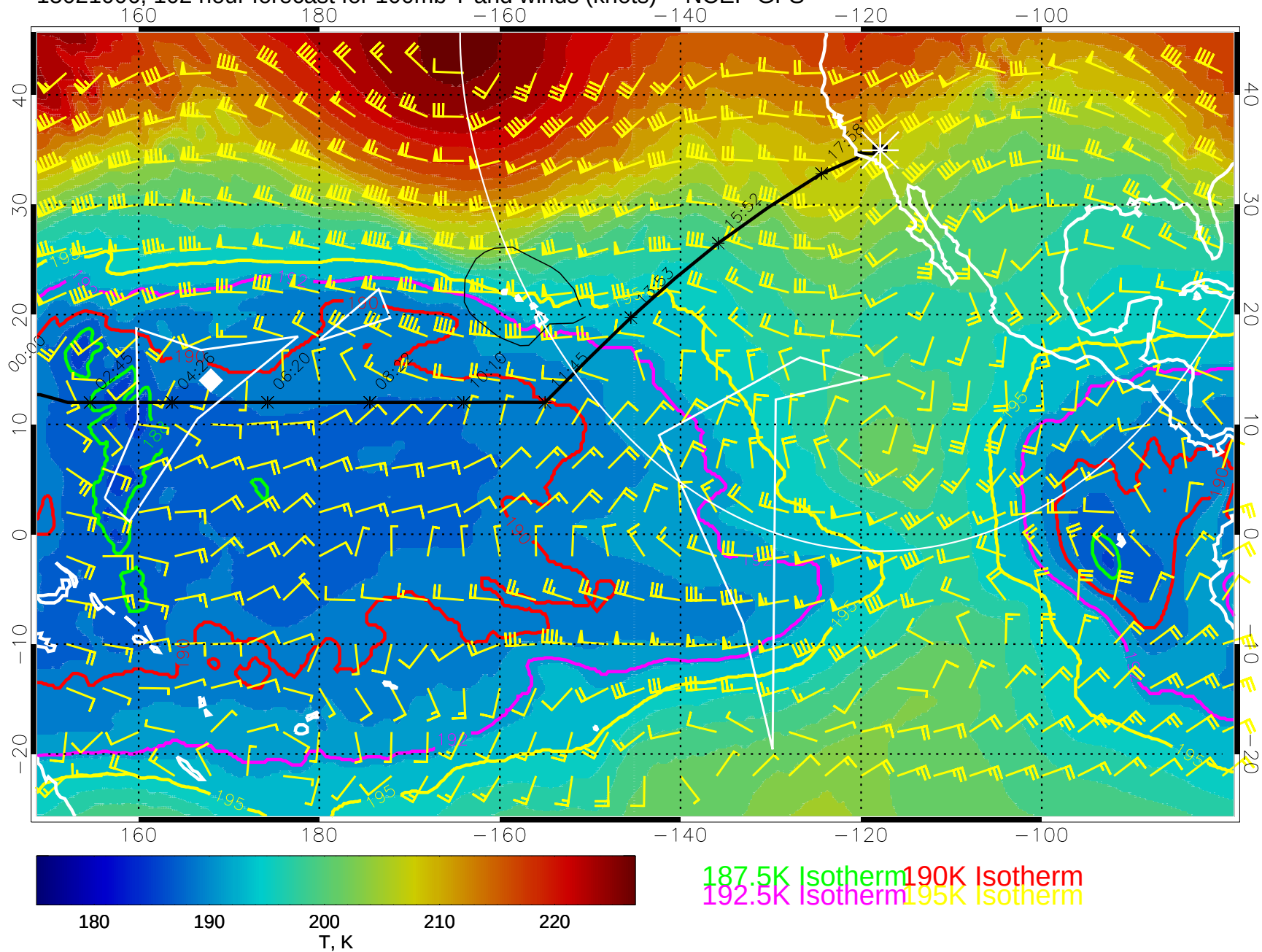
15021006, 102 hour forecast for 100mb T and winds (knots) -- NCEP GFS
