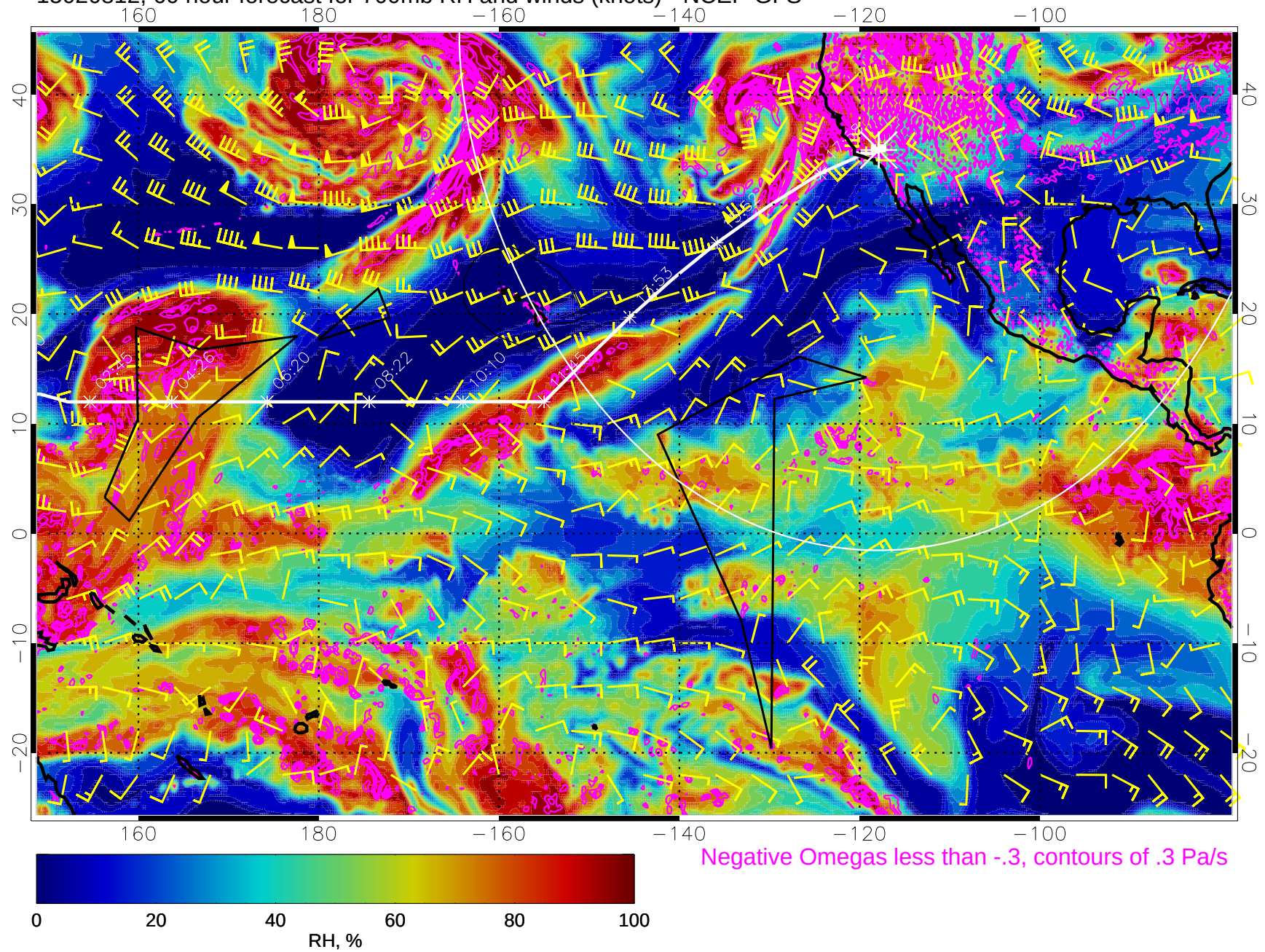
15020812, 60 hour forecast for 700mb RH and winds (knots) - NCEP GFS
