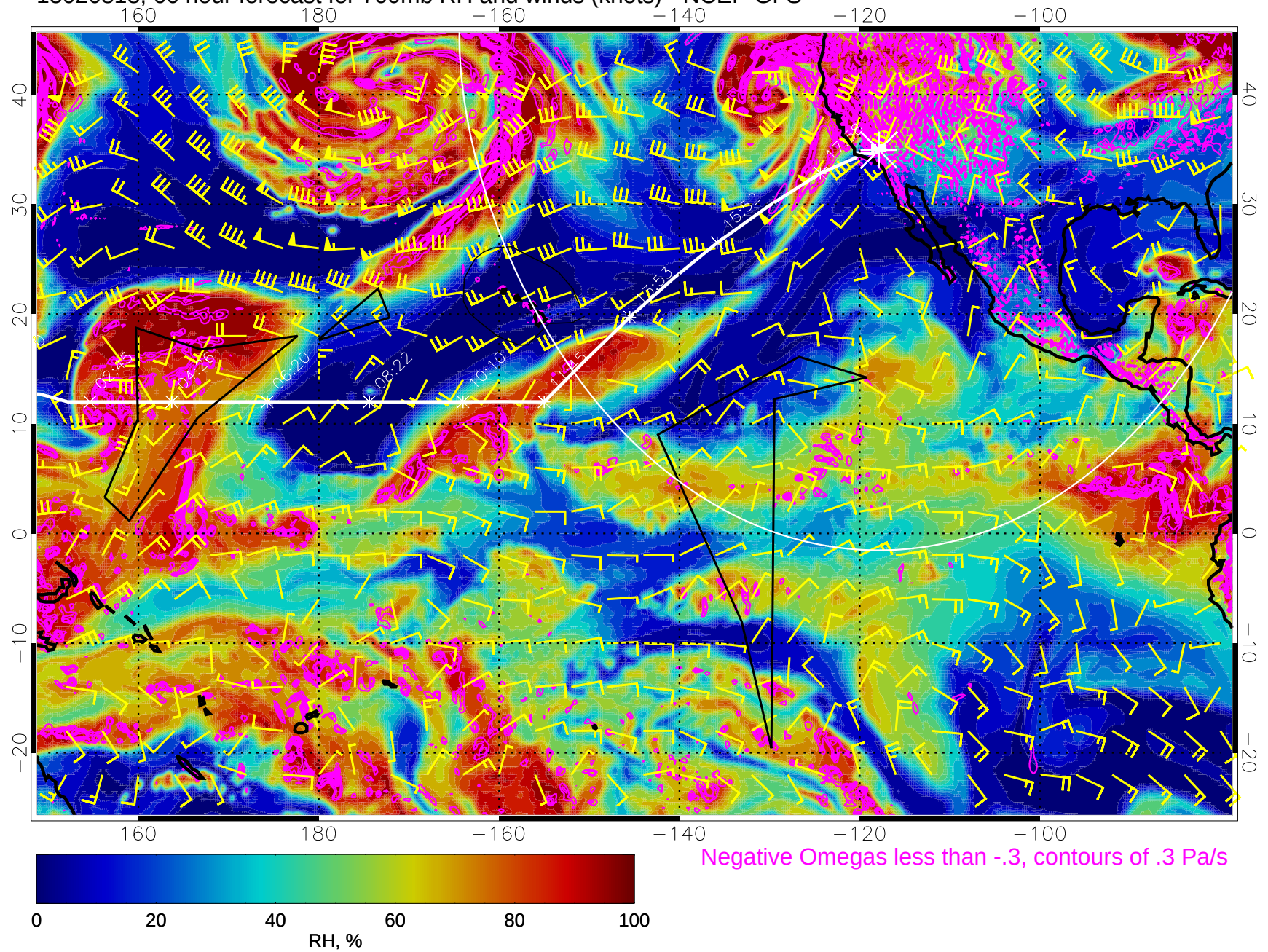
15020818, 66 hour forecast for 700mb RH and winds (knots) - NCEP GFS
