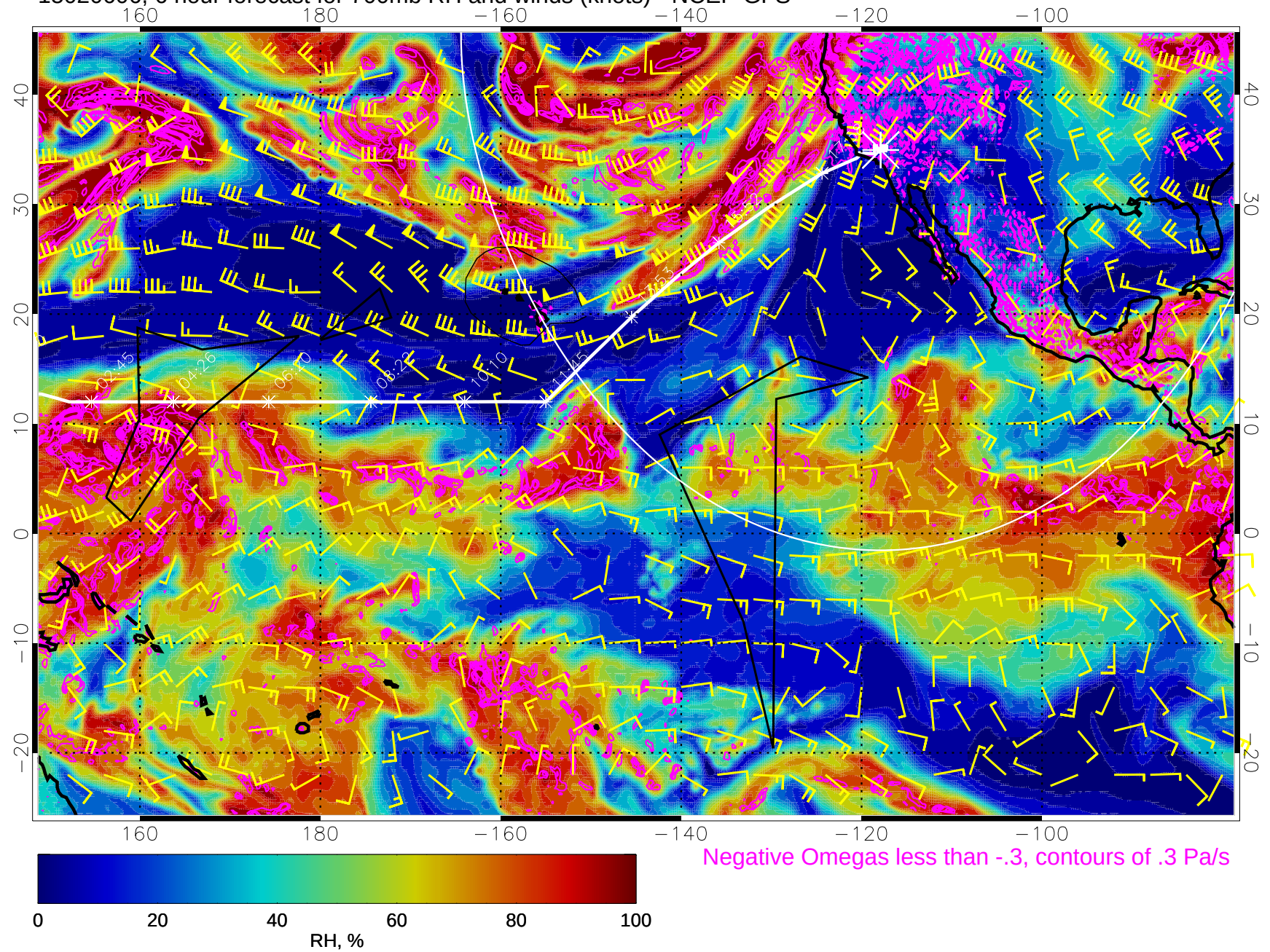
15020606, 6 hour forecast for 700mb RH and winds (knots) - NCEP GFS
