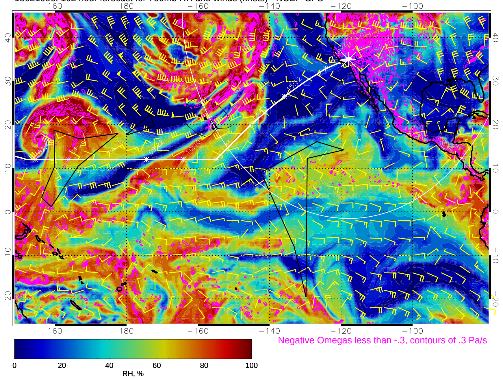
15021006, 102 hour forecast for 700mb RH and winds (knots) - NCEP GFS
