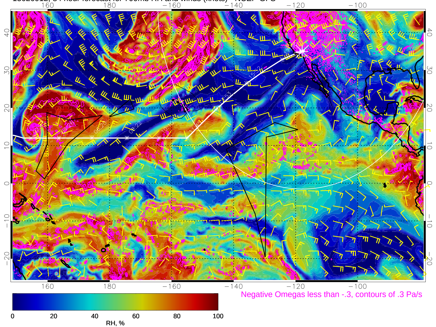
15020912, 84 hour forecast for 700mb RH and winds (knots) - NCEP GFS
