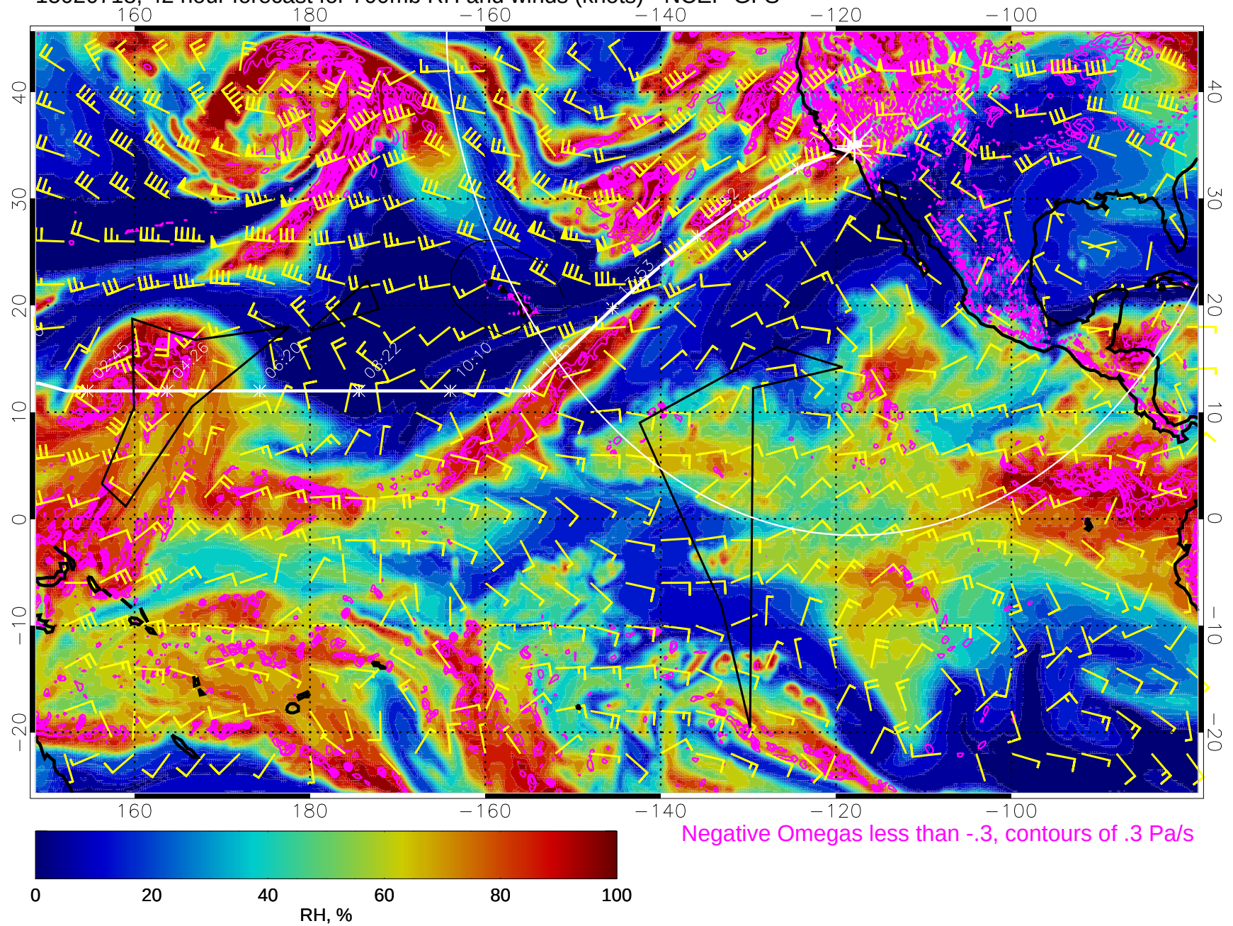
15020718, 42 hour forecast for 700mb RH and winds (knots) - NCEP GFS
