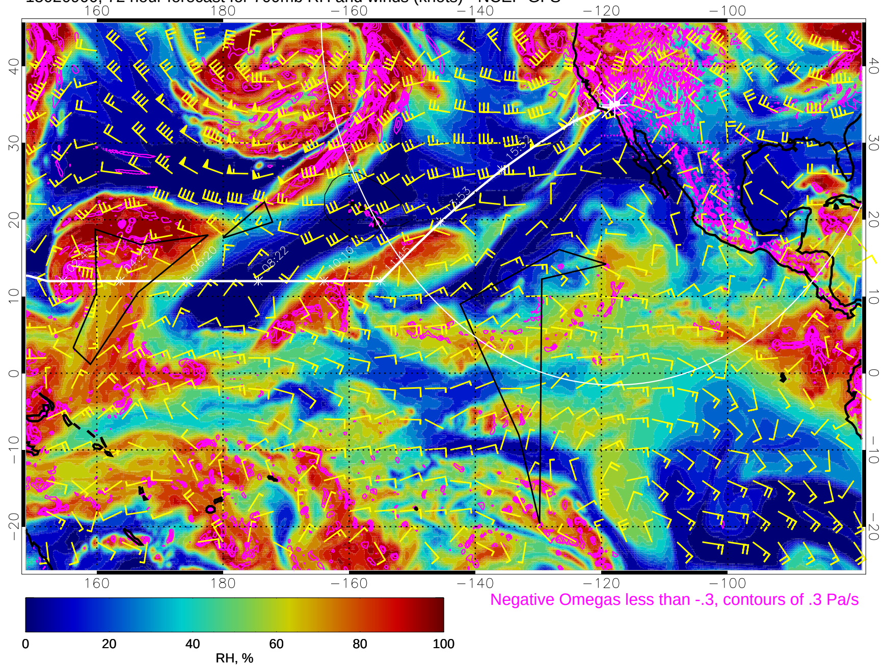
15020900, 72 hour forecast for 700mb RH and winds (knots) - NCEP GFS
