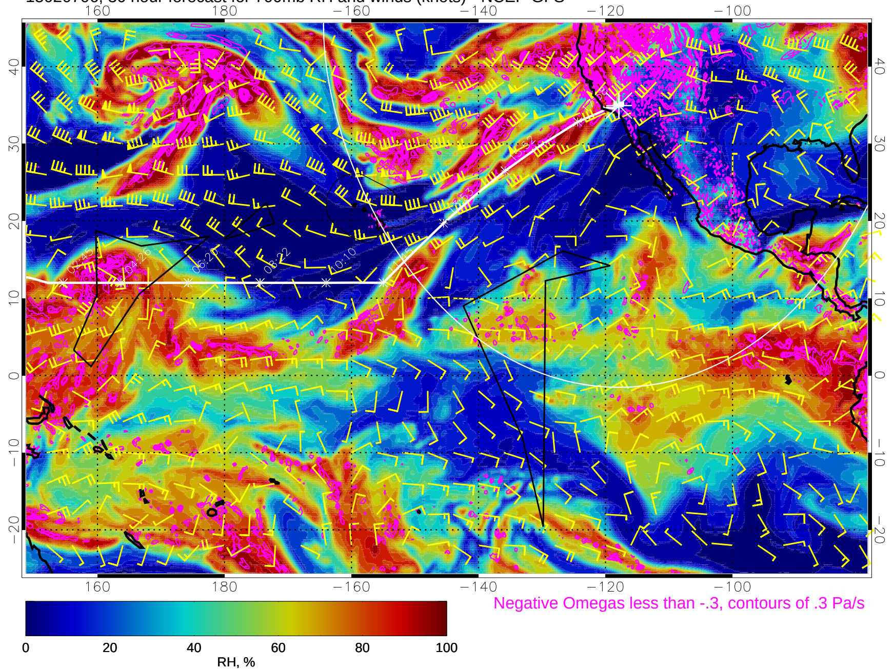
15020706, 30 hour forecast for 700mb RH and winds (knots) - NCEP GFS
