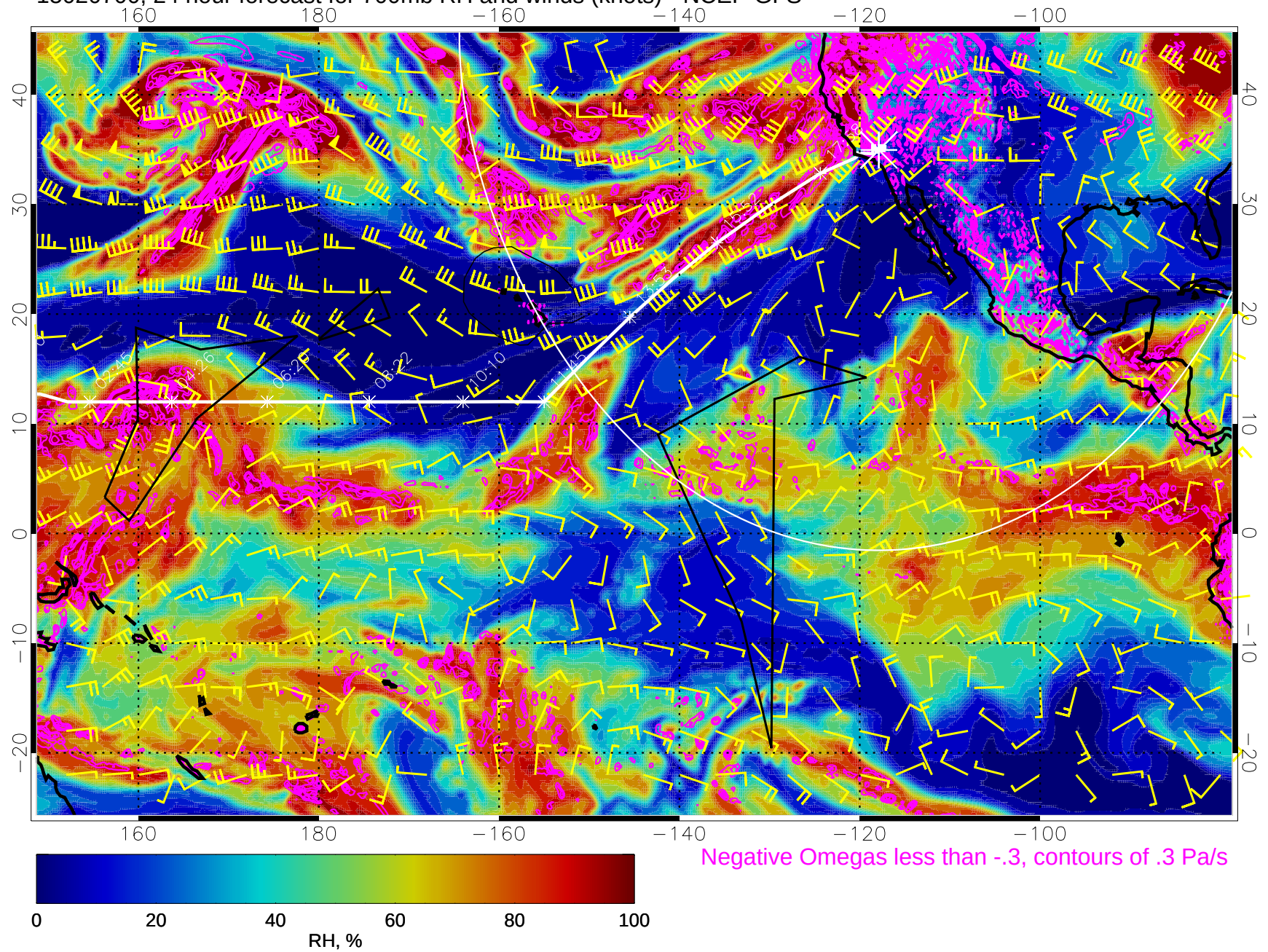
15020700, 24 hour forecast for 700mb RH and winds (knots) - NCEP GFS
