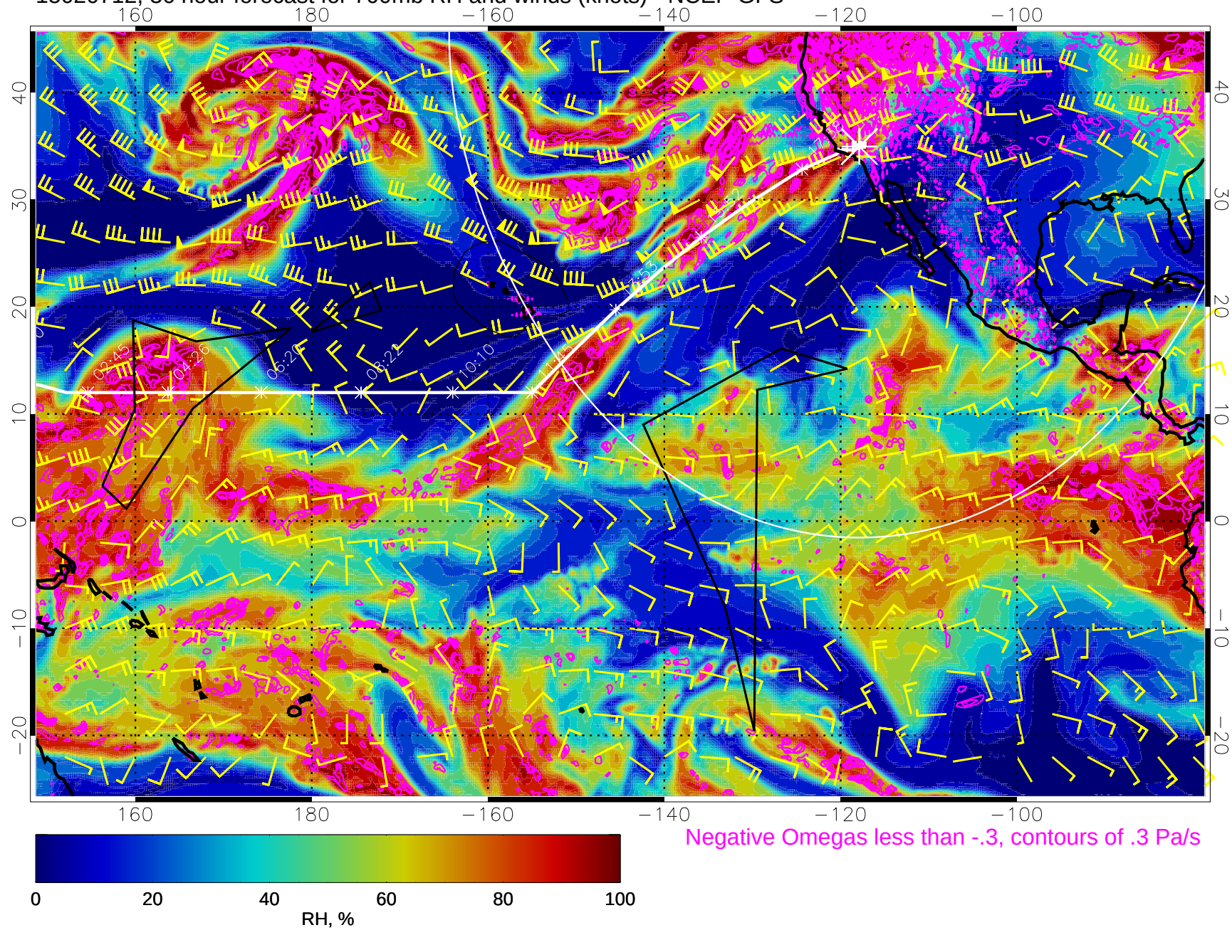
15020712, 36 hour forecast for 700mb RH and winds (knots) - NCEP GFS
