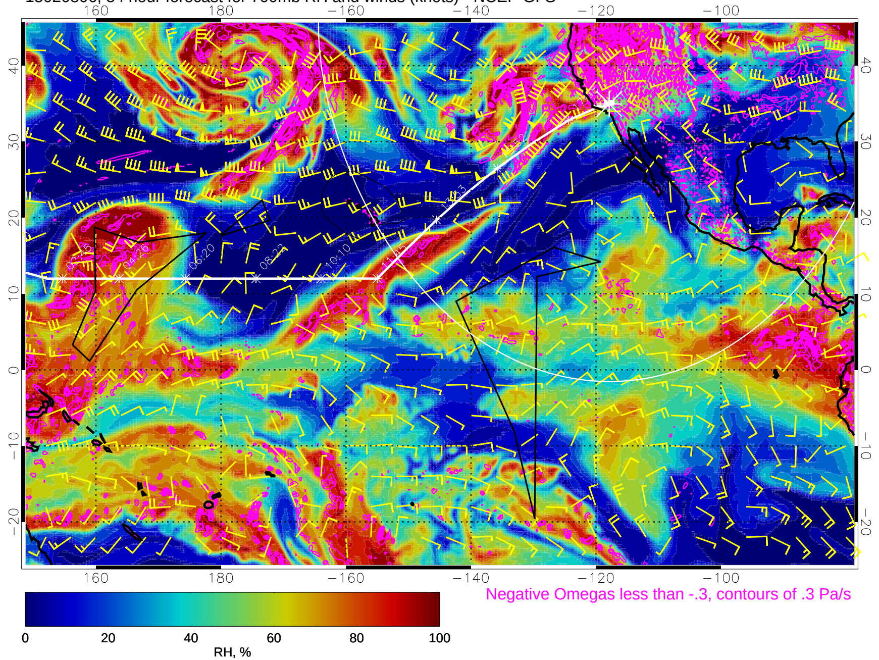
15020806, 54 hour forecast for 700mb RH and winds (knots) - NCEP GFS
