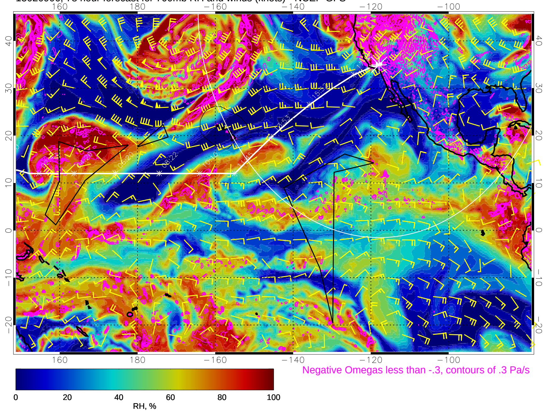
15020906, 78 hour forecast for 700mb RH and winds (knots) - NCEP GFS
