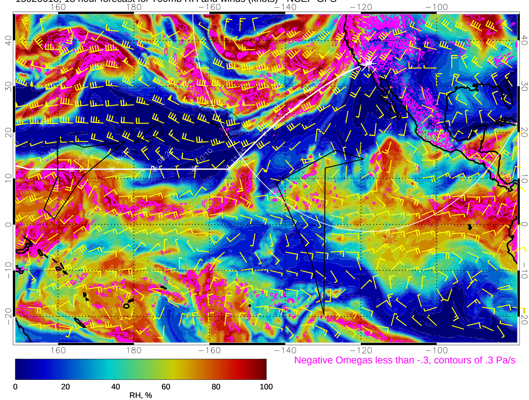
15020618, 18 hour forecast for 700mb RH and winds (knots) - NCEP GFS
