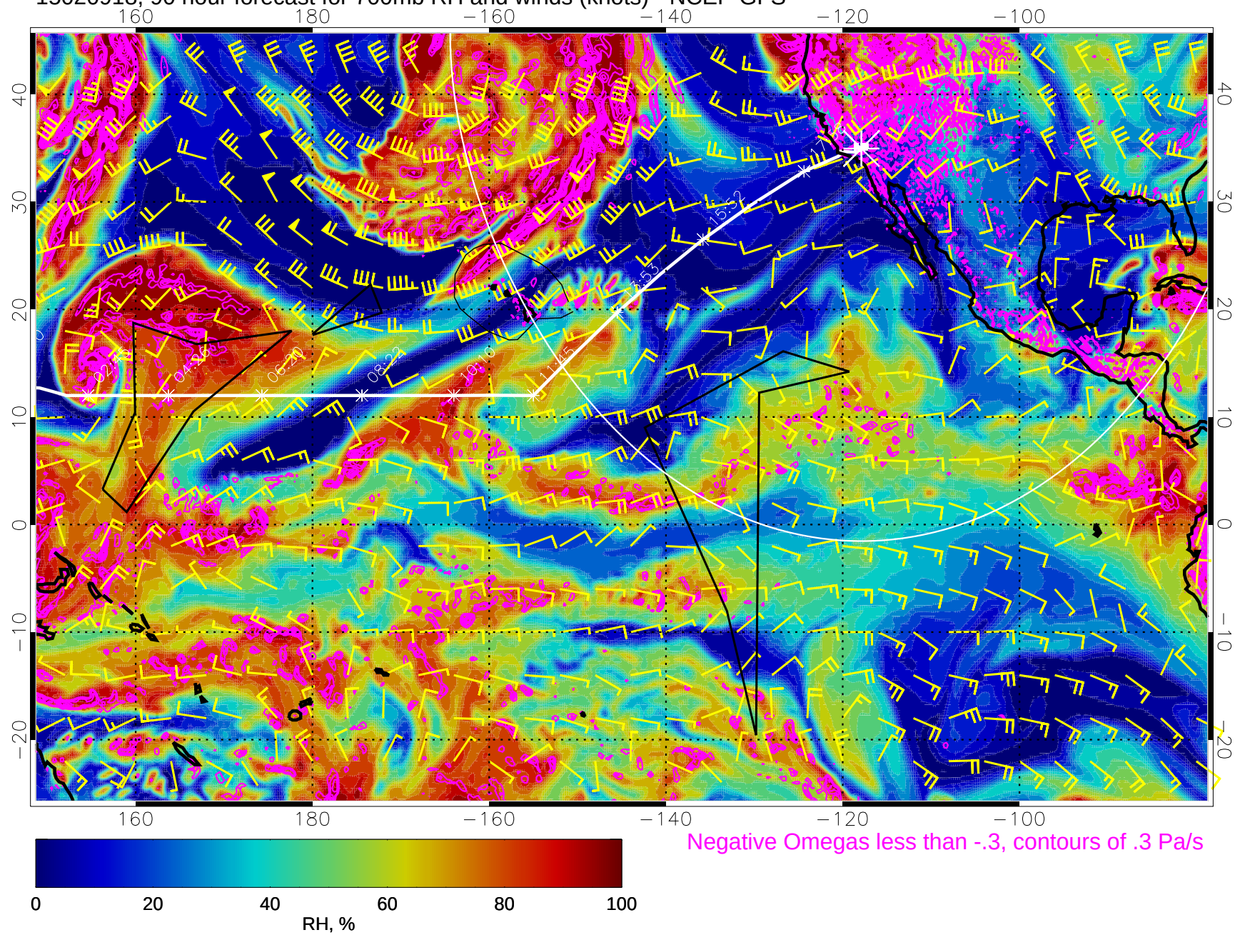
15020918, 90 hour forecast for 700mb RH and winds (knots) - NCEP GFS
