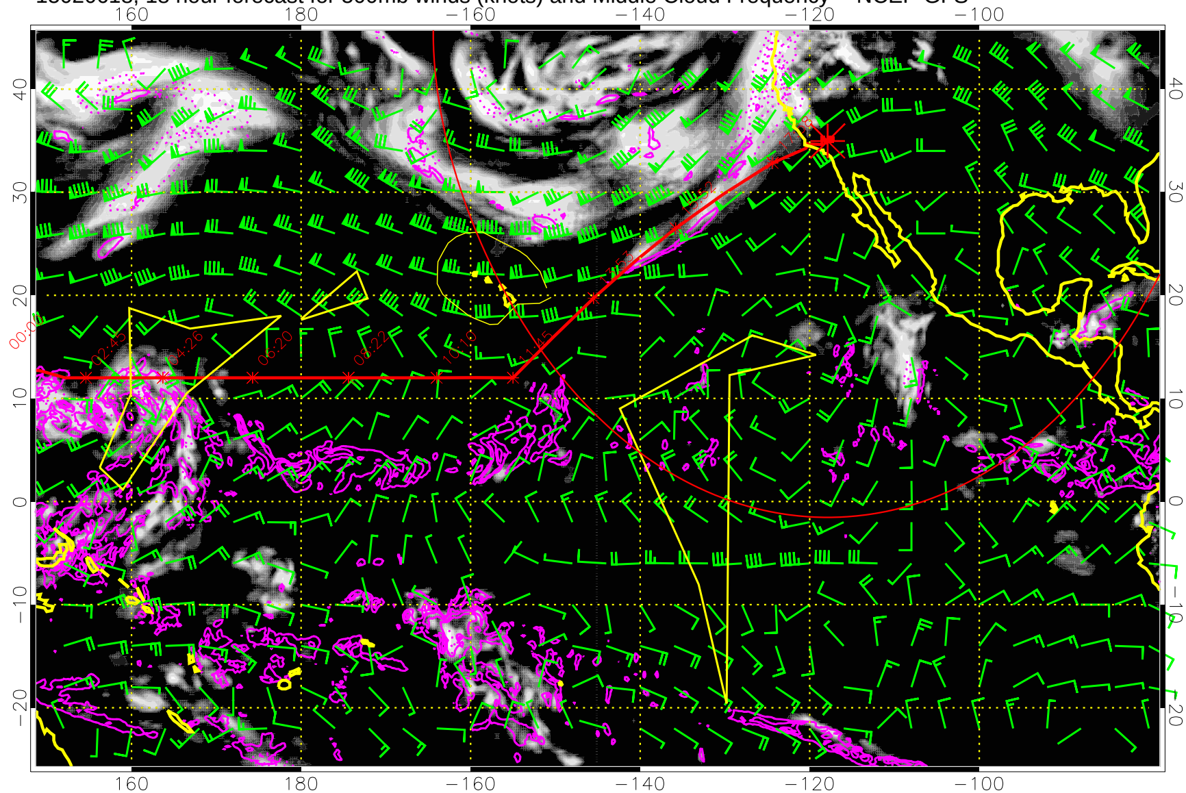
15020618, 18 hour forecast for 500mb winds (knots) and Middle Cloud Frequency -- NCEP GFS
