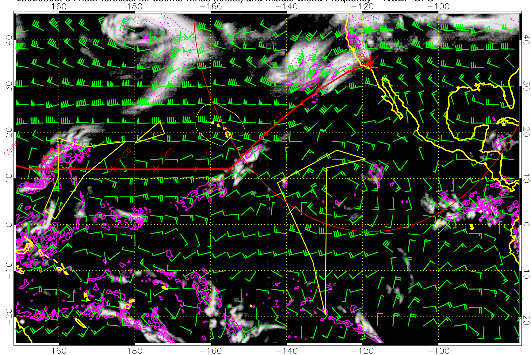
15020806, 54 hour forecast for 500mb winds (knots) and Middle Cloud Frequency -- NCEP GFS
