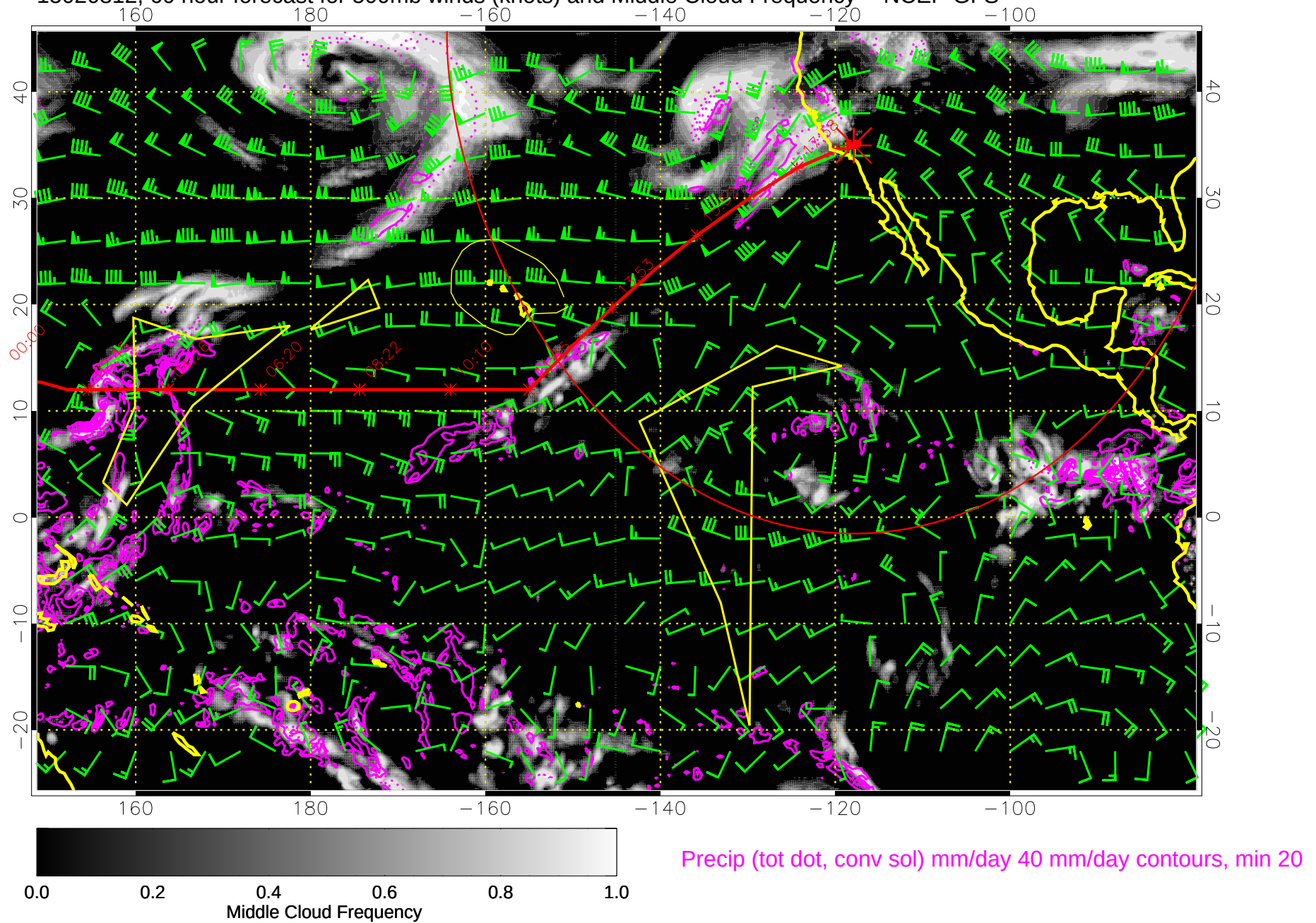
15020812, 60 hour forecast for 500mb winds (knots) and Middle Cloud Frequency -- NCEP GFS
