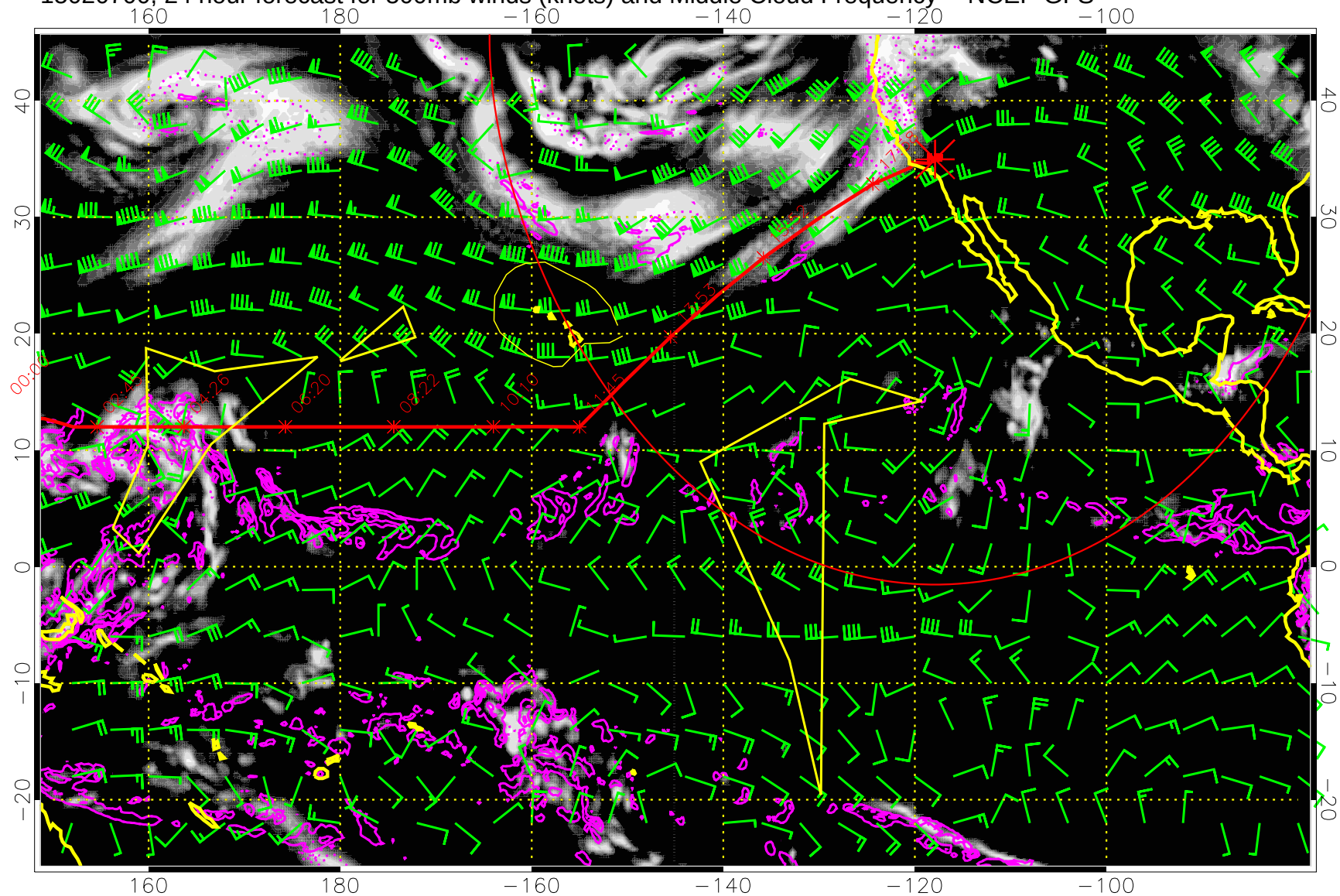
15020700, 24 hour forecast for 500mb winds (knots) and Middle Cloud Frequency -- NCEP GFS
