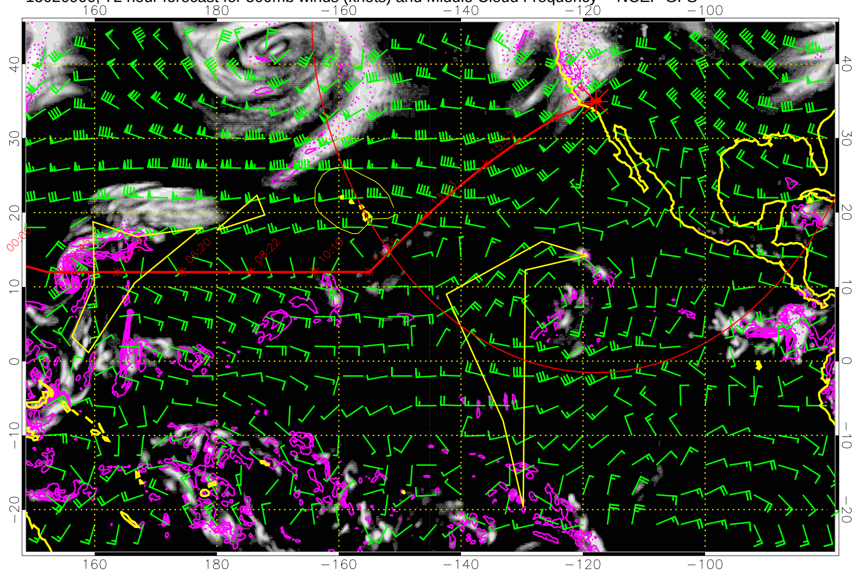
15020900, 72 hour forecast for 500mb winds (knots) and Middle Cloud Frequency -- NCEP GFS
