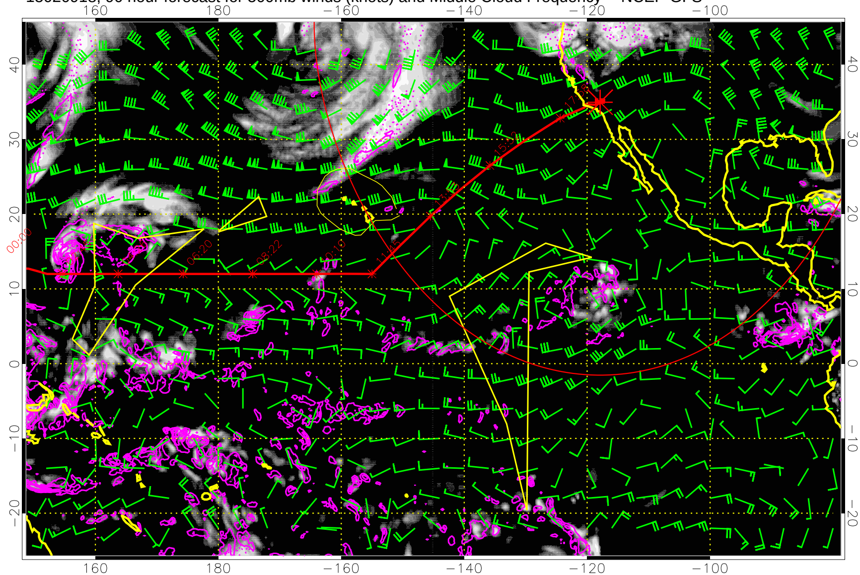
15020918, 90 hour forecast for 500mb winds (knots) and Middle Cloud Frequency -- NCEP GFS
