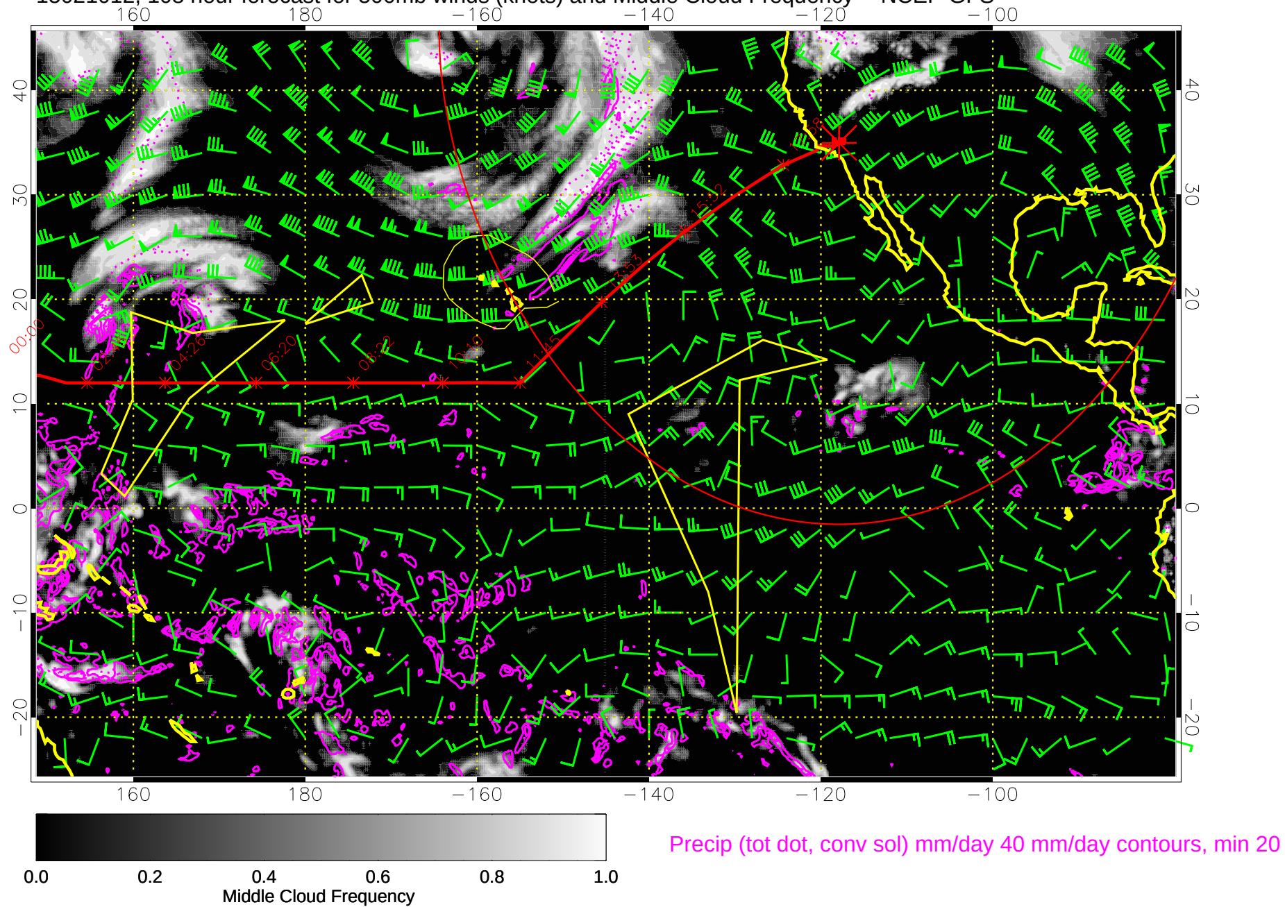
15021012, 108 hour forecast for 500mb winds (knots) and Middle Cloud Frequency -- NCEP GFS
