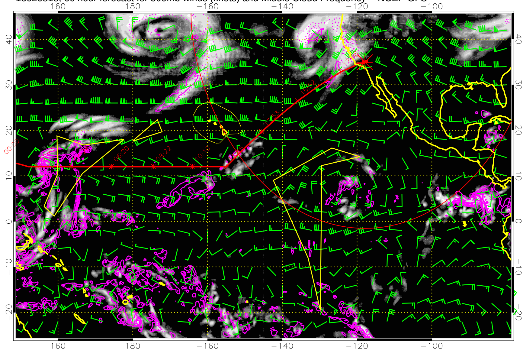
15020818, 66 hour forecast for 500mb winds (knots) and Middle Cloud Frequency -- NCEP GFS
