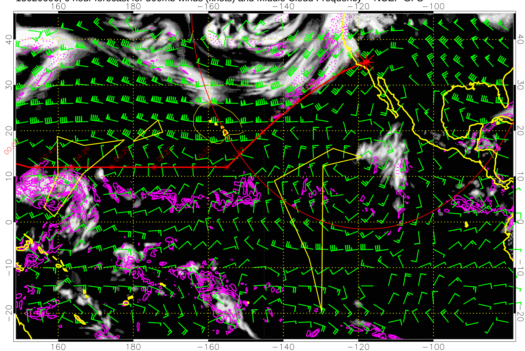
15020606, 6 hour forecast for 500mb winds (knots) and Middle Cloud Frequency -- NCEP GFS
