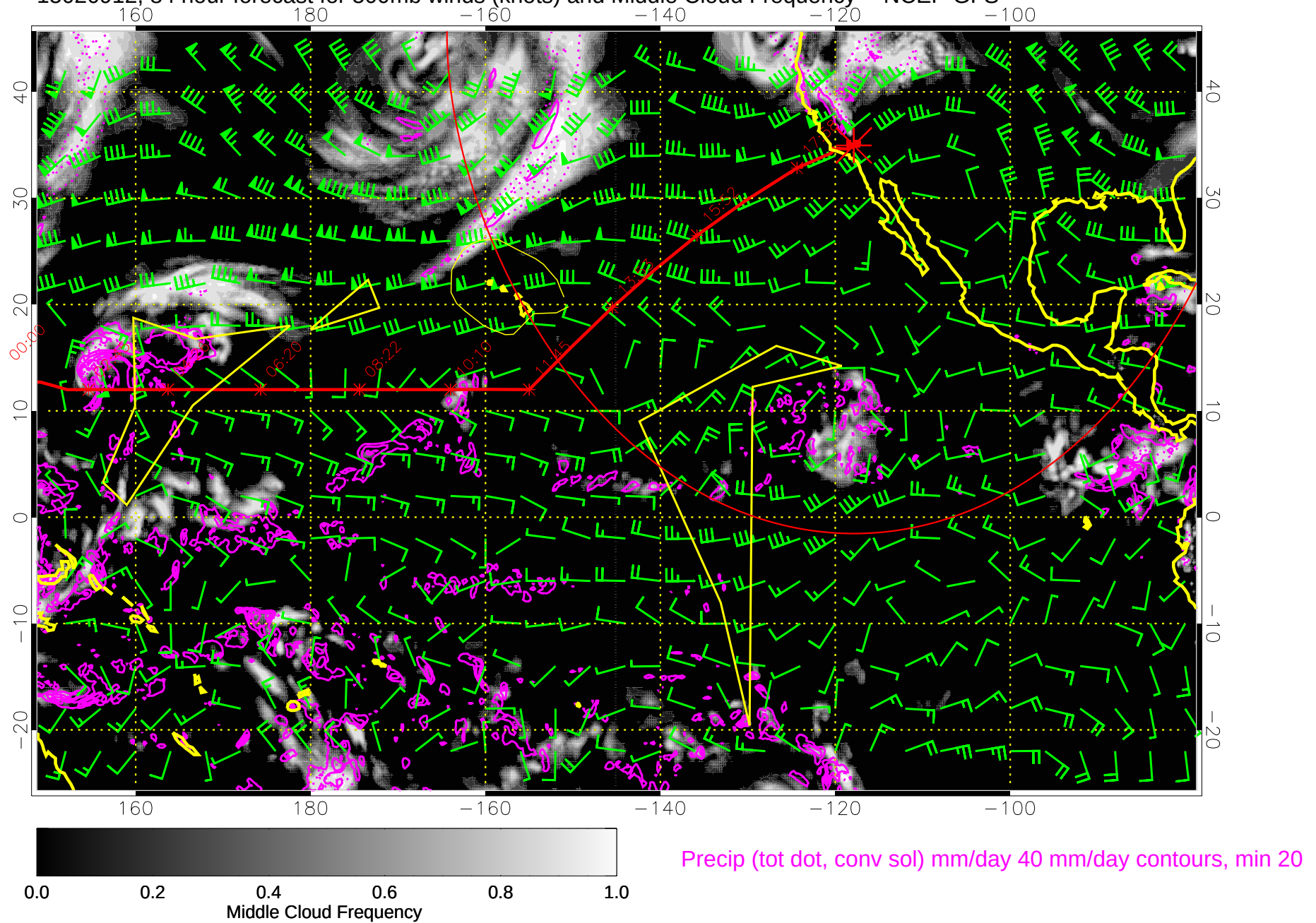
15020912, 84 hour forecast for 500mb winds (knots) and Middle Cloud Frequency -- NCEP GFS
