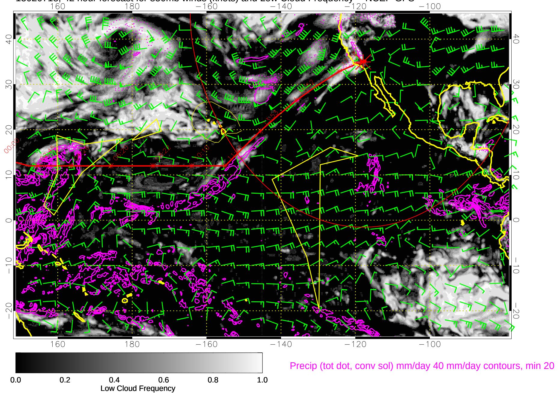
15020718, 42 hour forecast for 850mb winds (knots) and Low Cloud Frequency -- NCEP GFS
