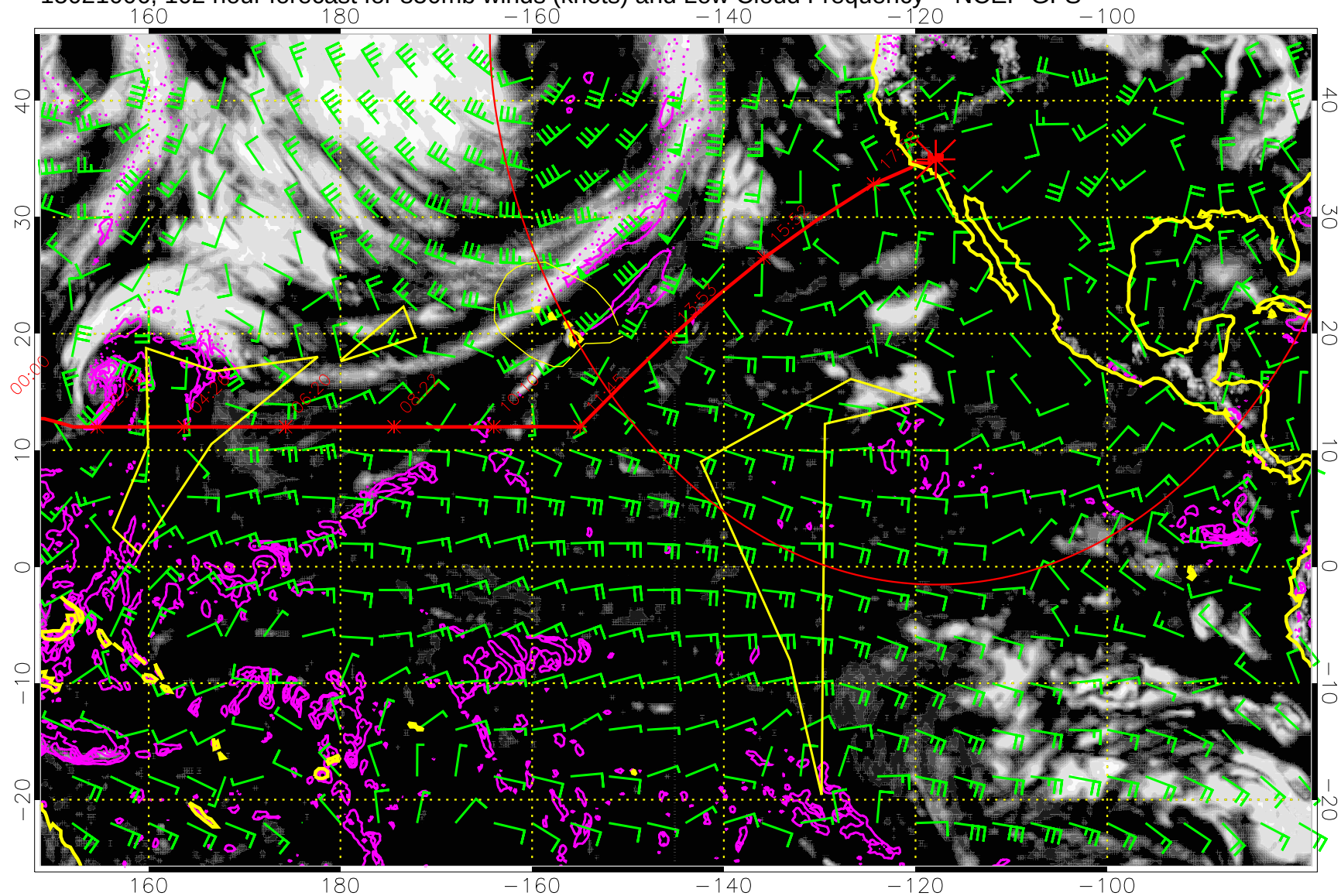
15021006, 102 hour forecast for 850mb winds (knots) and Low Cloud Frequency -- NCEP GFS
