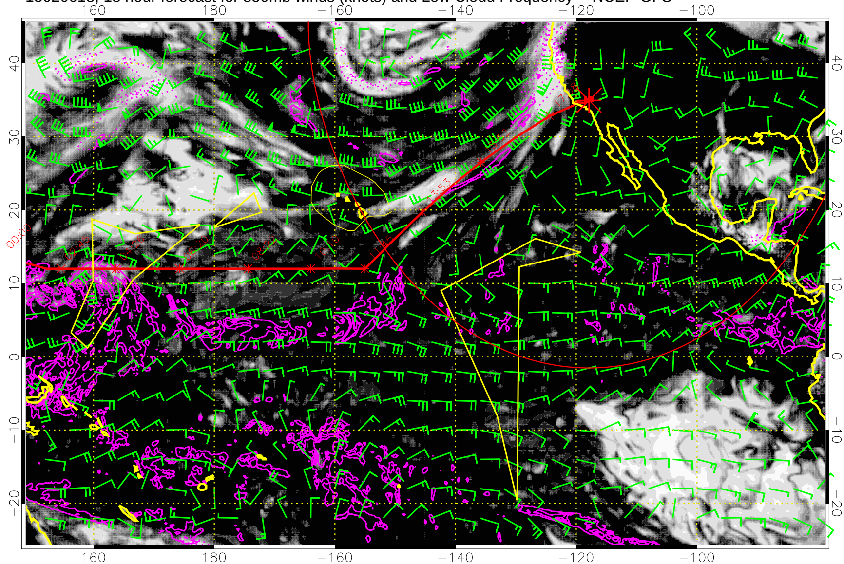
15020618, 18 hour forecast for 850mb winds (knots) and Low Cloud Frequency -- NCEP GFS
