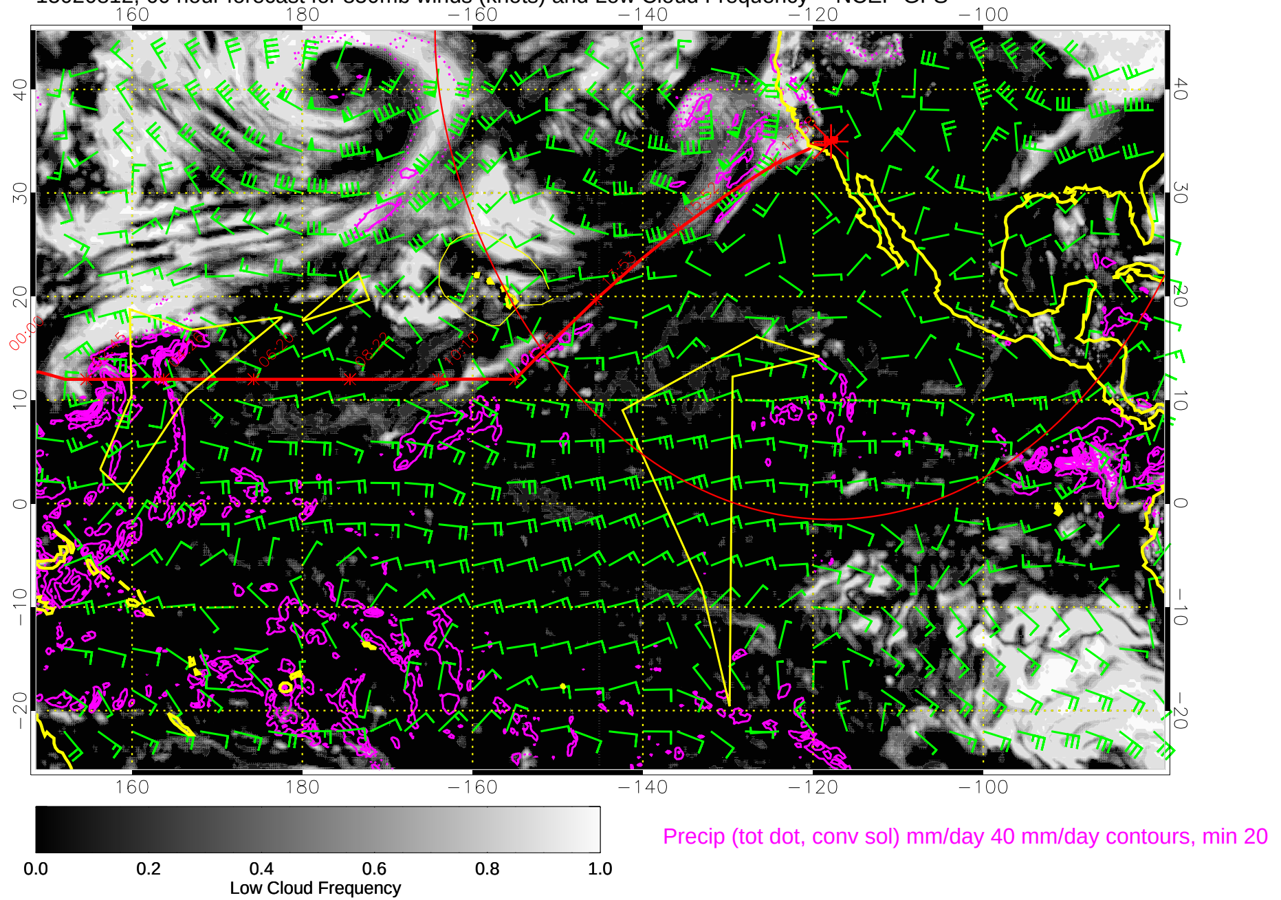
15020812, 60 hour forecast for 850mb winds (knots) and Low Cloud Frequency -- NCEP GFS
