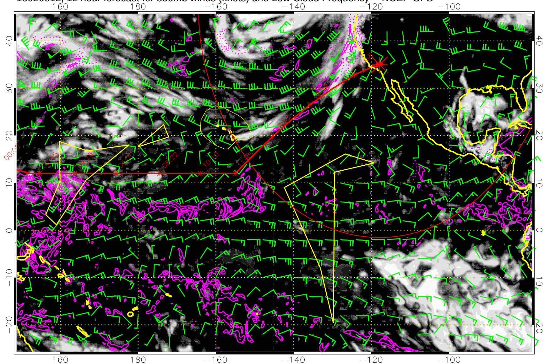
15020612, 12 hour forecast for 850mb winds (knots) and Low Cloud Frequency -- NCEP GFS
