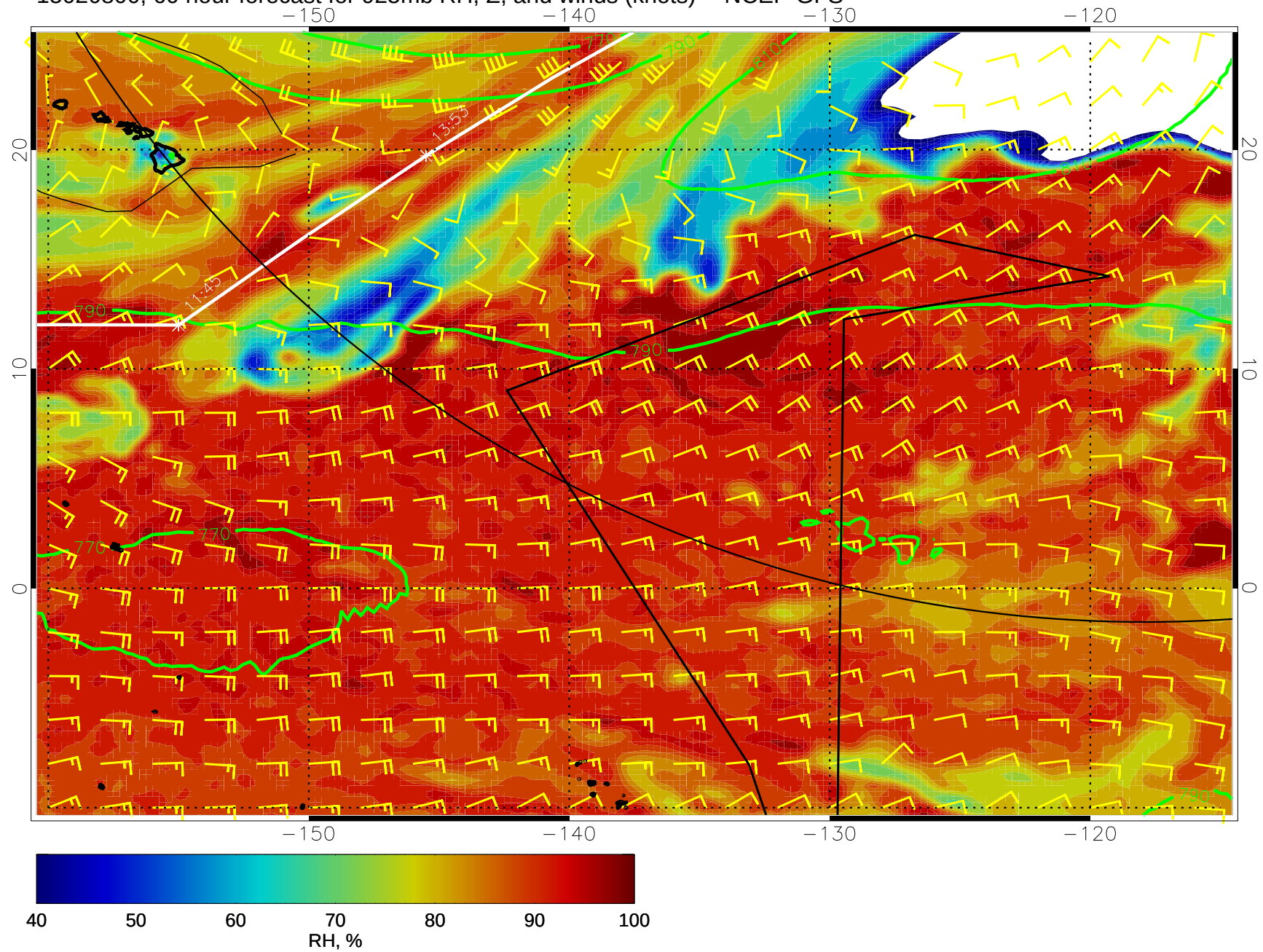
15020800, 60 hour forecast for 925mb RH, Z, and winds (knots) -- NCEP GFS
