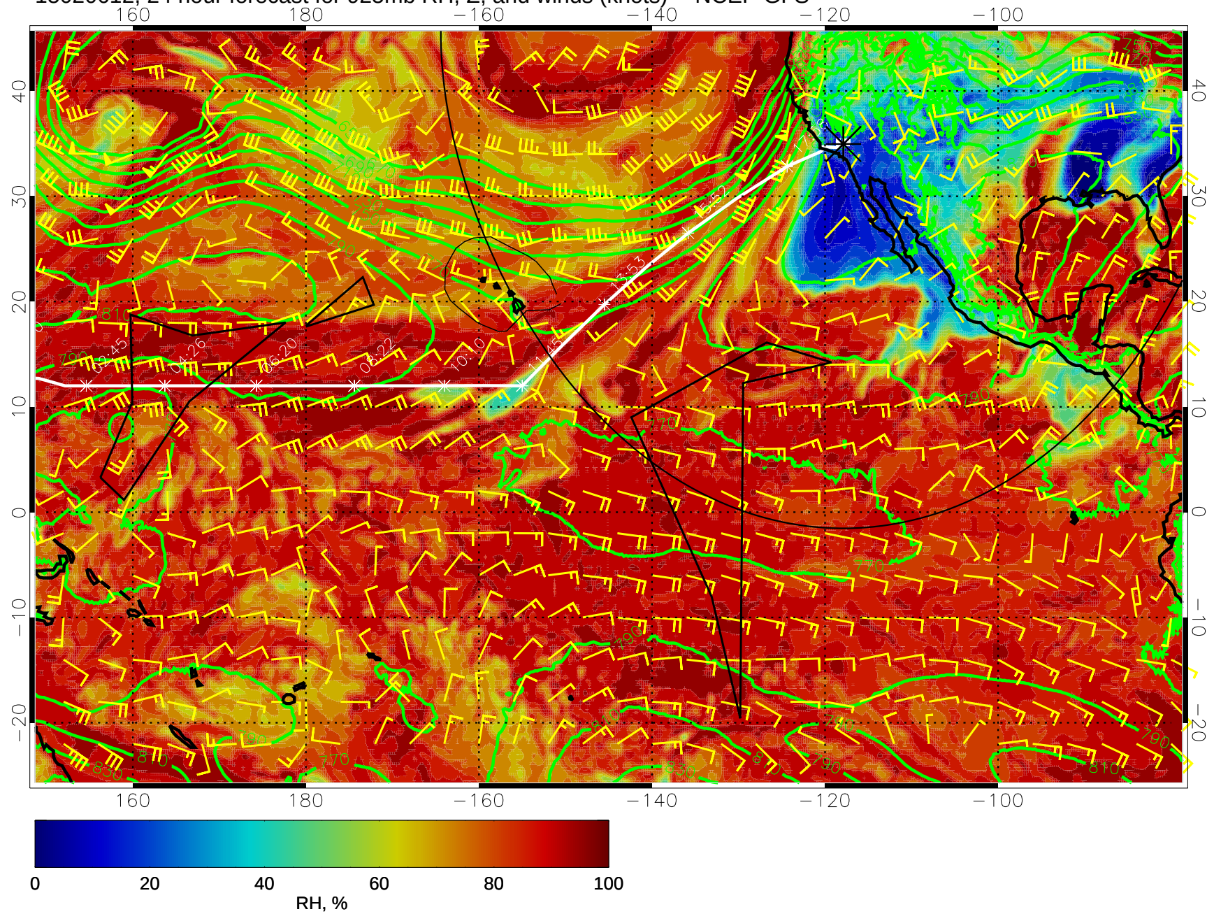
15020612, 24 hour forecast for 925mb RH, Z, and winds (knots) -- NCEP GFS
