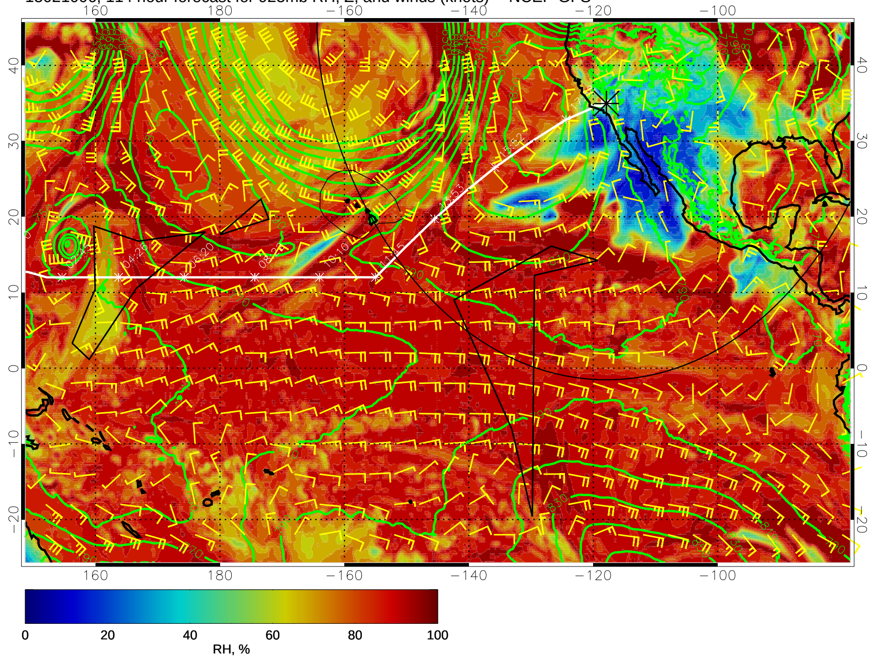
15021006, 114 hour forecast for 925mb RH, Z, and winds (knots) -- NCEP GFS
