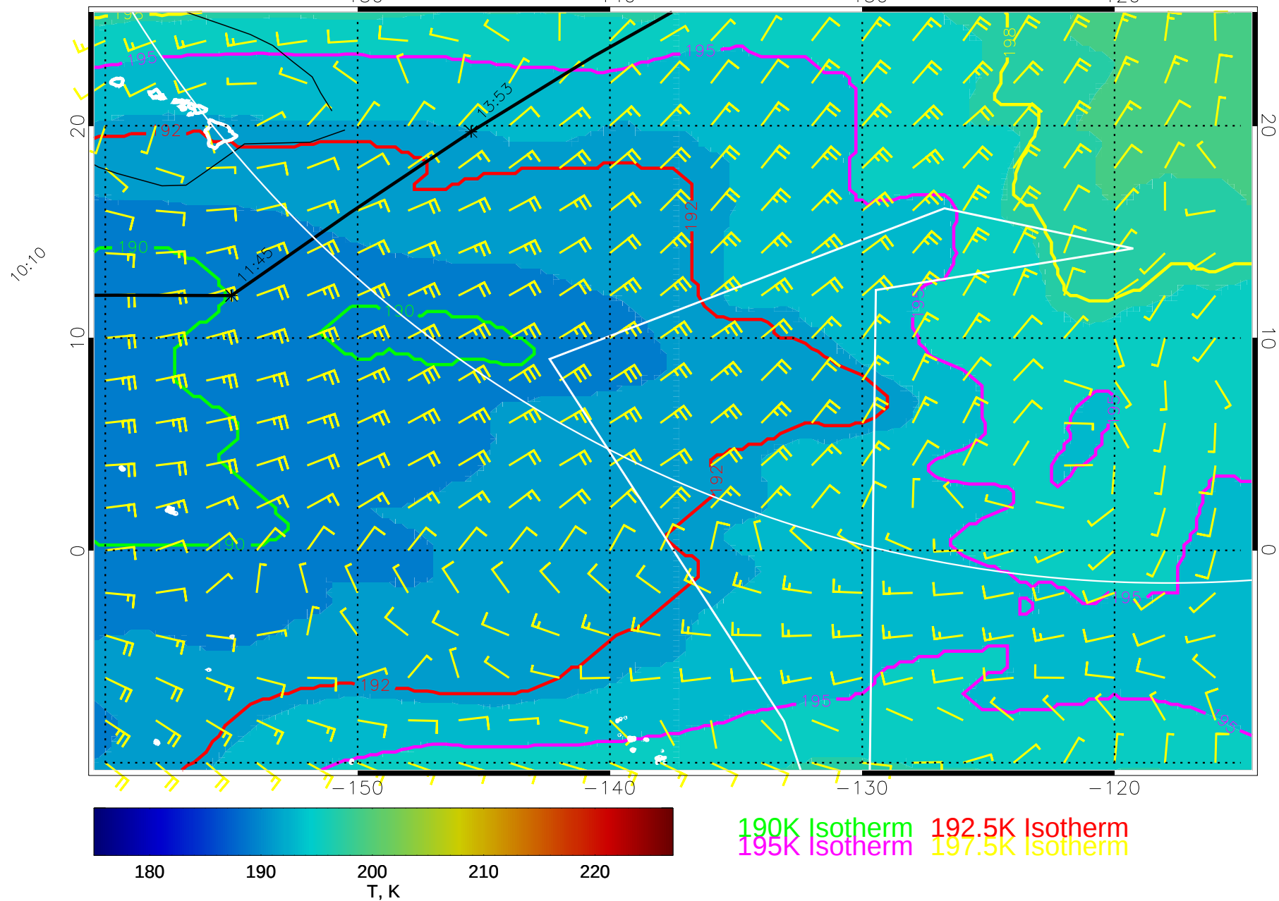
15020518, 6 hour forecast for 70mb T and winds (knots) -- NCEP GFS
