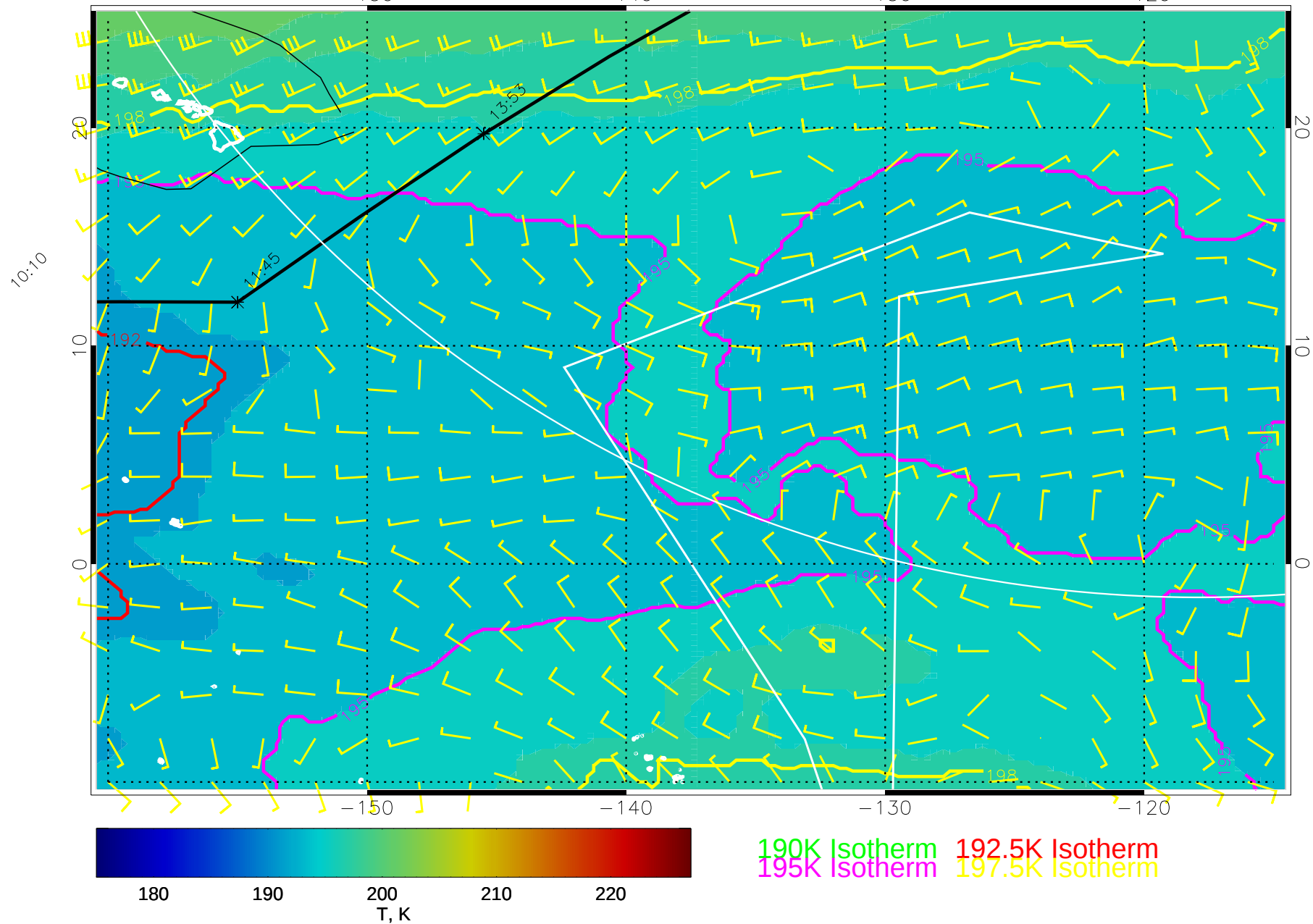
15021000, 108 hour forecast for 70mb T and winds (knots) -- NCEP GFS
