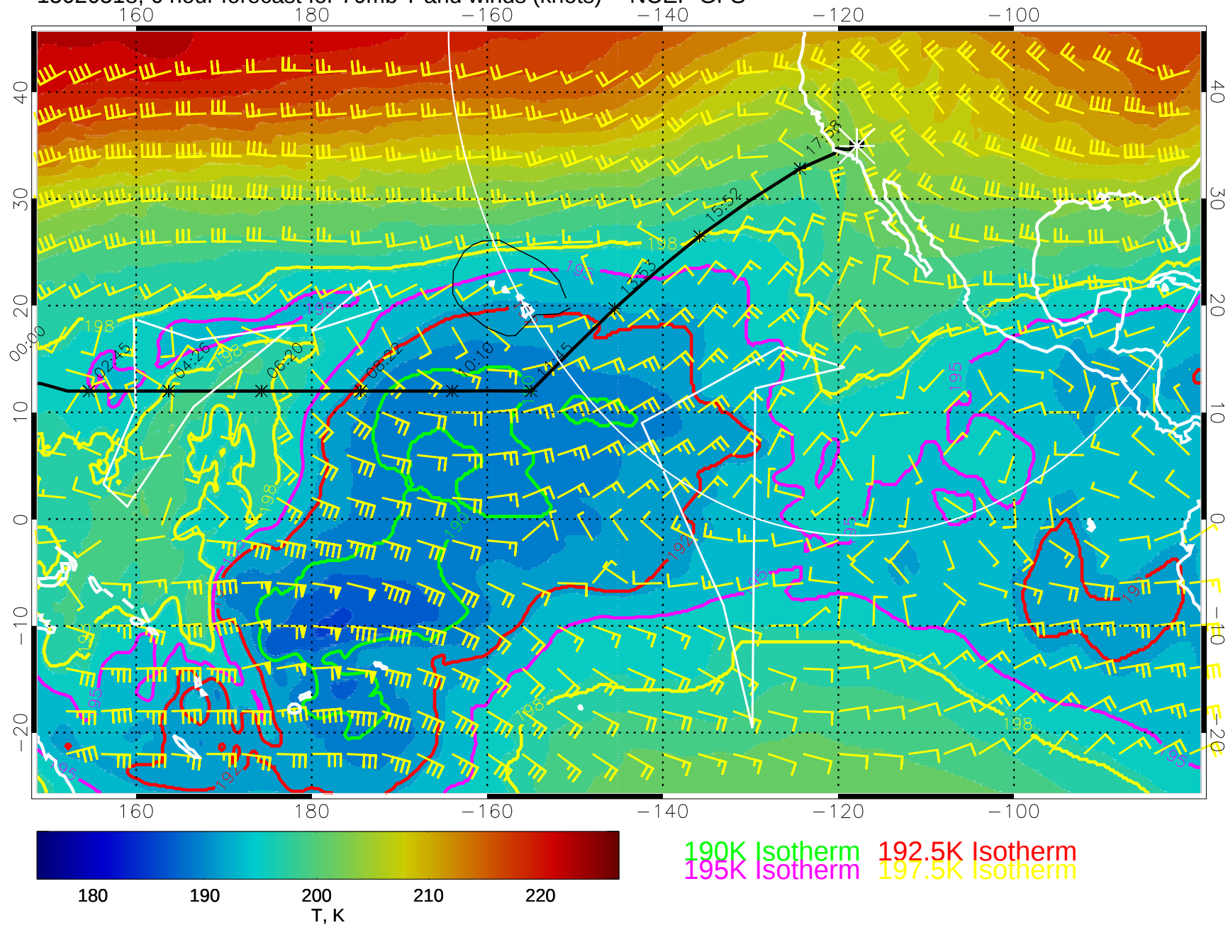
15020518, 6 hour forecast for 70mb T and winds (knots) -- NCEP GFS
