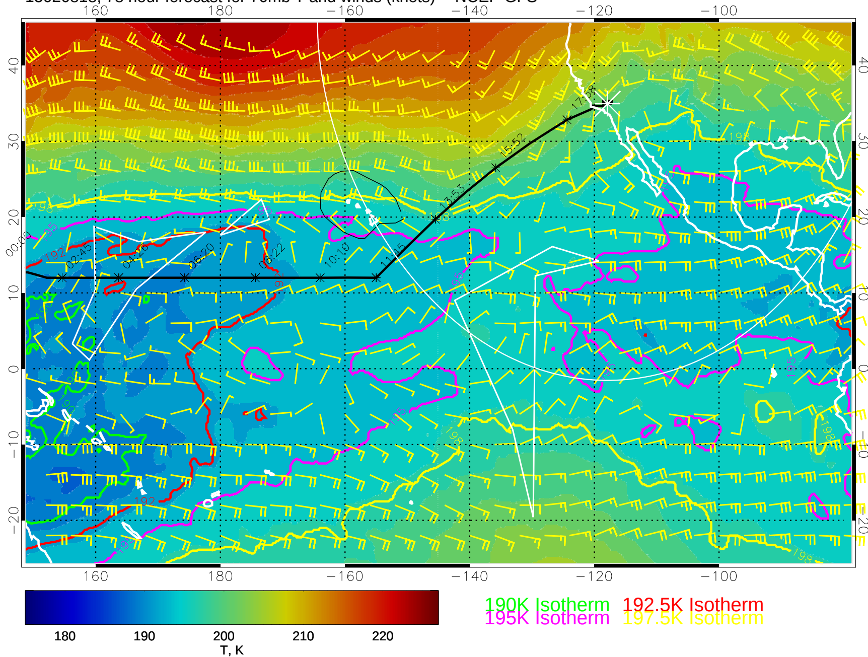
15020818, 78 hour forecast for 70mb T and winds (knots) -- NCEP GFS
