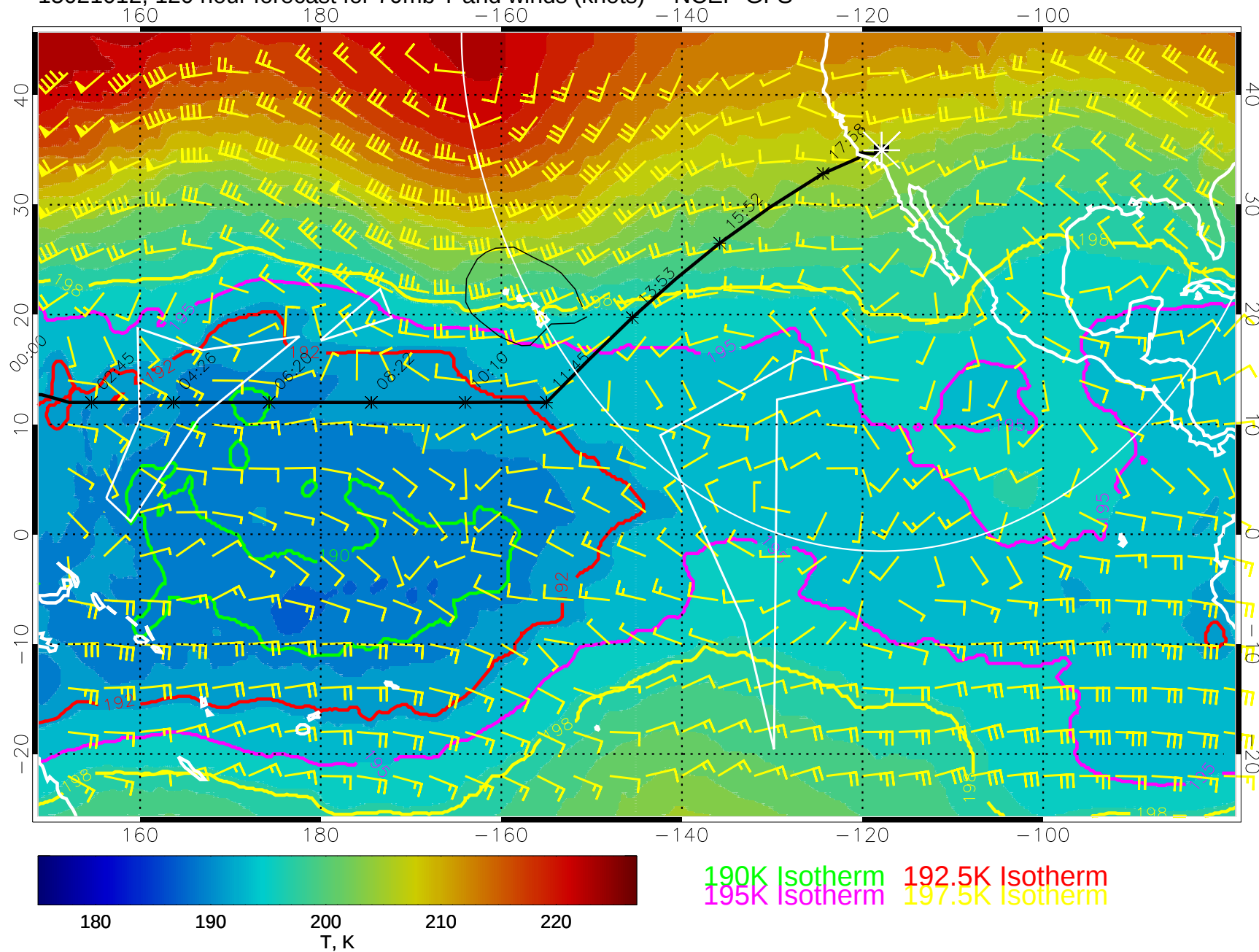
15021012, 120 hour forecast for 70mb T and winds (knots) -- NCEP GFS
