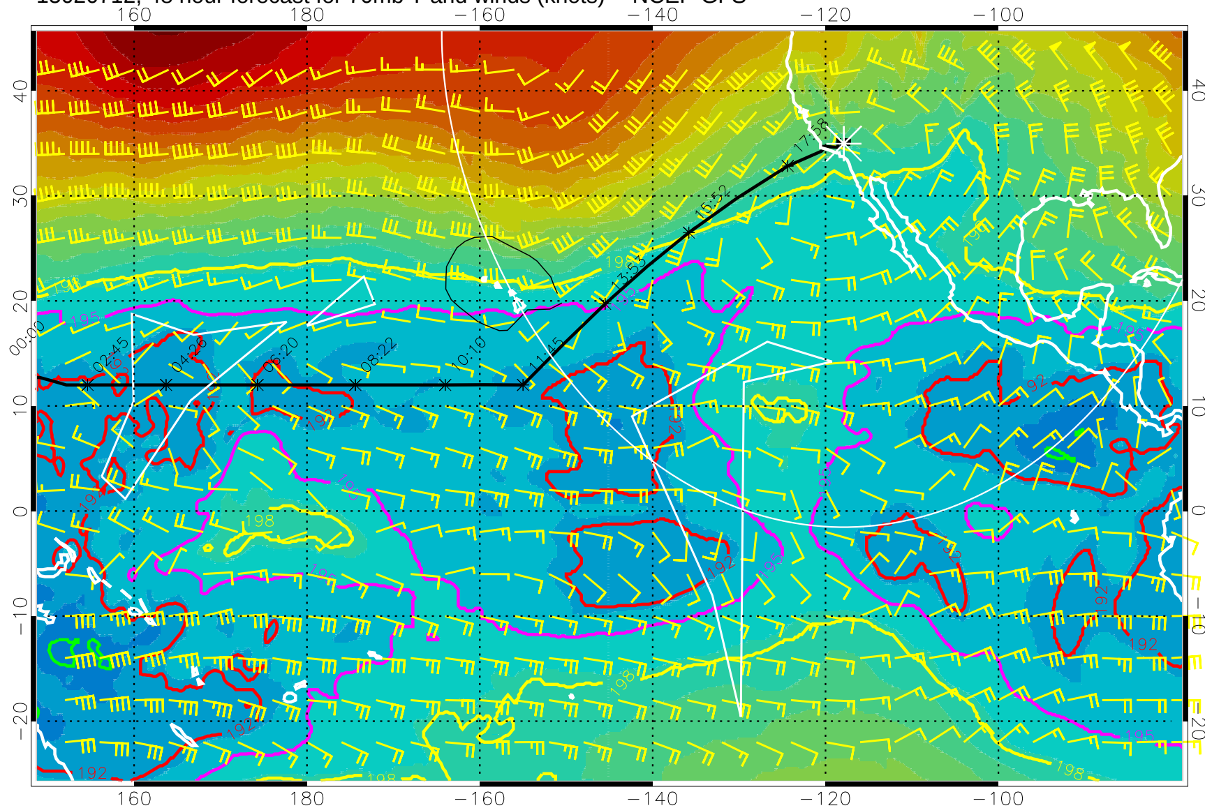
15020712, 48 hour forecast for 70mb T and winds (knots) -- NCEP GFS
