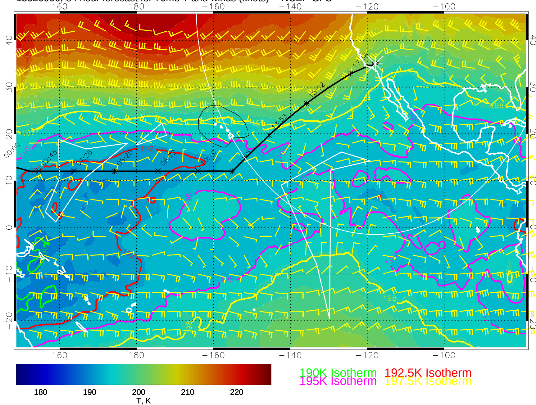
15020900, 84 hour forecast for 70mb T and winds (knots) -- NCEP GFS
