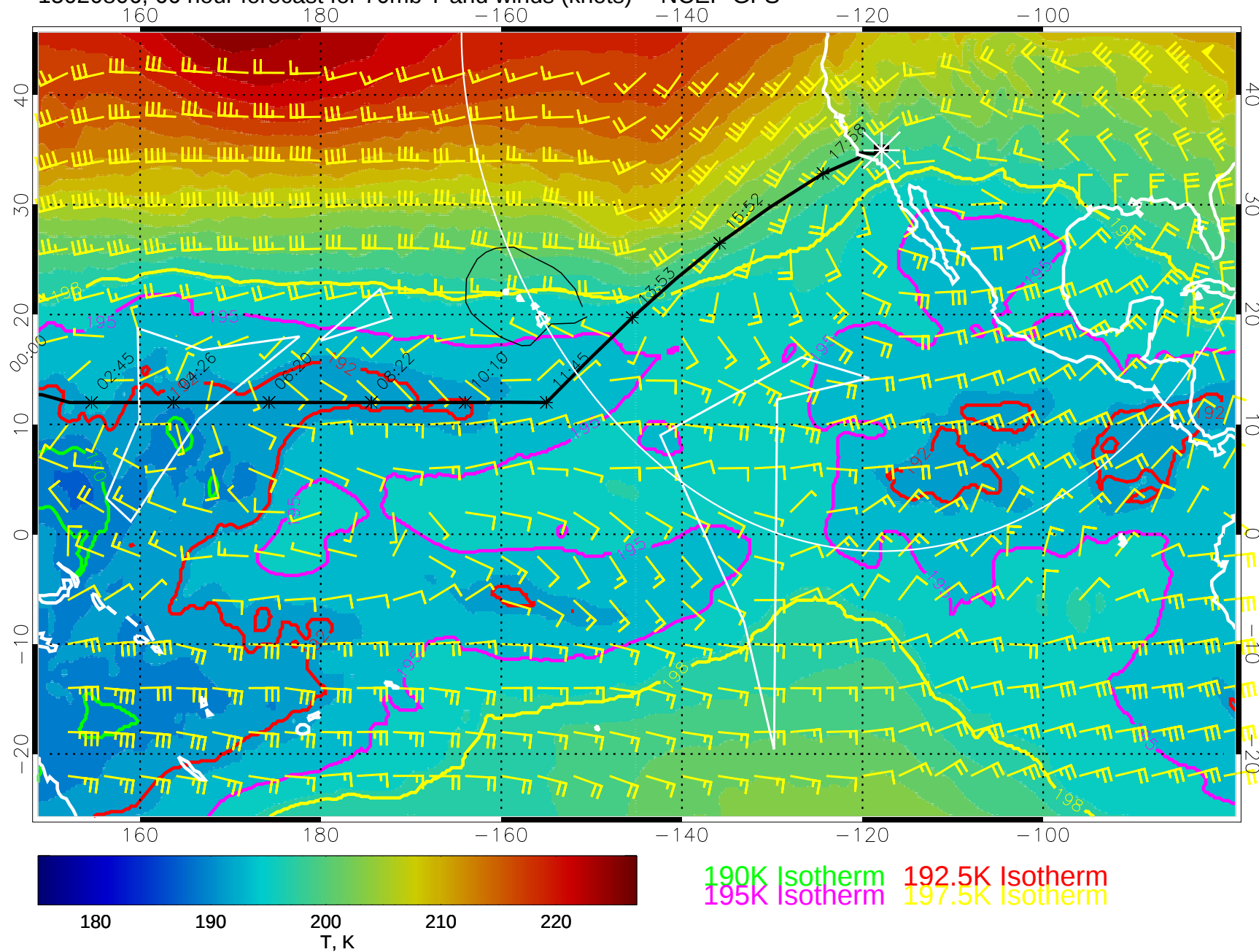
15020806, 66 hour forecast for 70mb T and winds (knots) -- NCEP GFS
