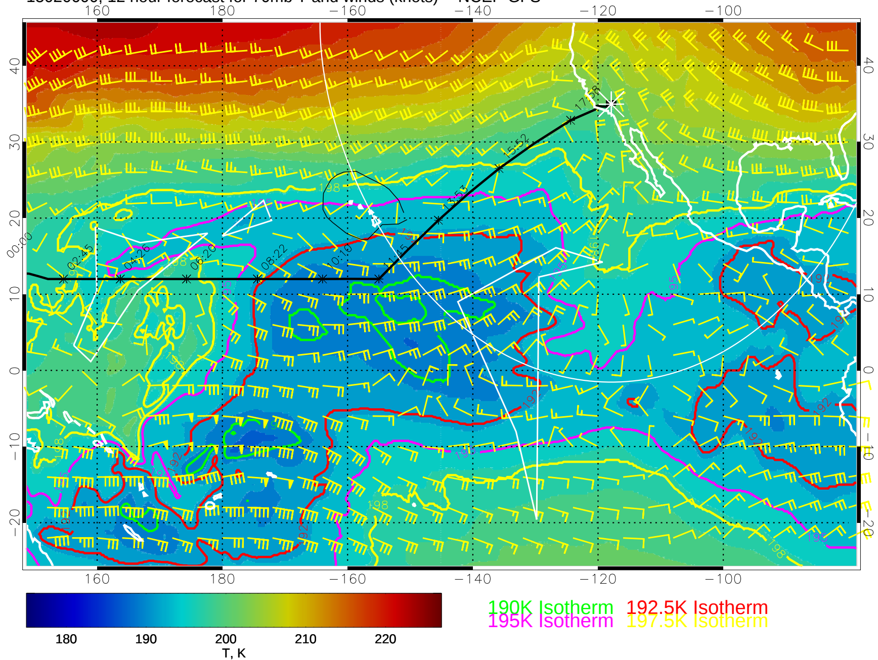
15020600, 12 hour forecast for 70mb T and winds (knots) -- NCEP GFS
