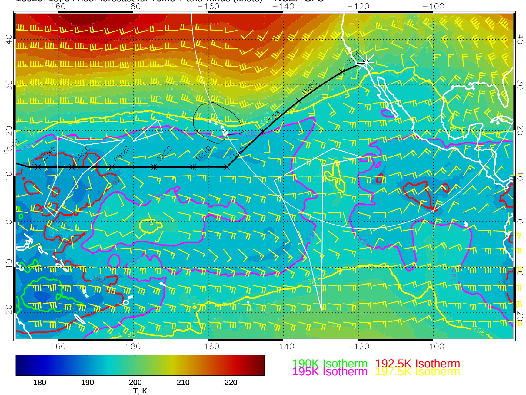
15020718, 54 hour forecast for 70mb T and winds (knots) -- NCEP GFS
