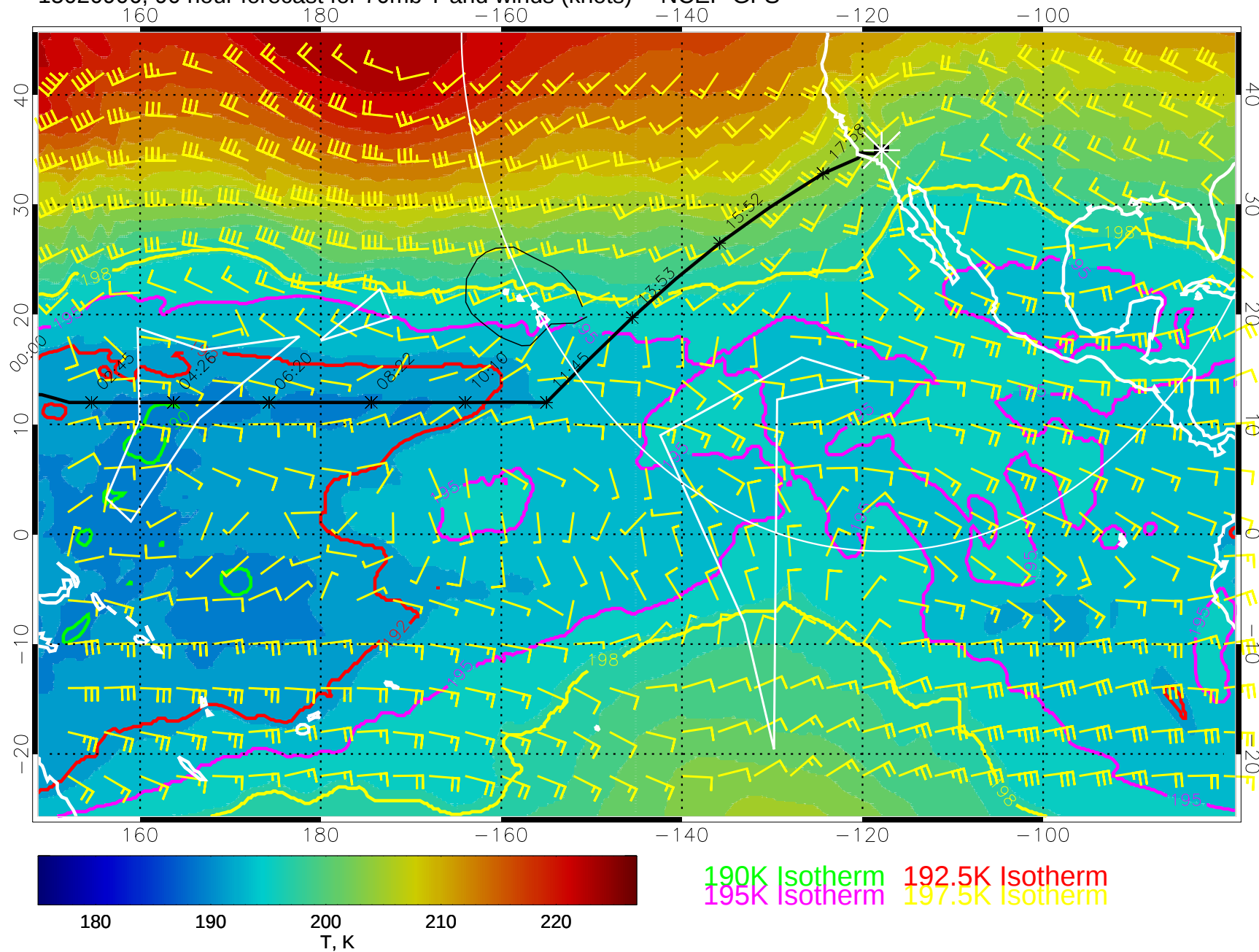
15020906, 90 hour forecast for 70mb T and winds (knots) -- NCEP GFS
