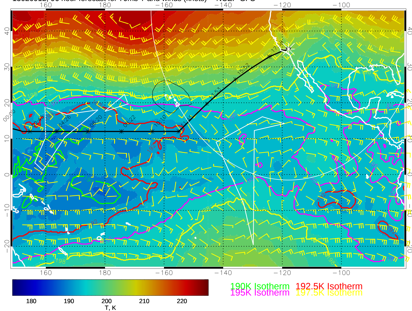
15020912, 96 hour forecast for 70mb T and winds (knots) -- NCEP GFS
