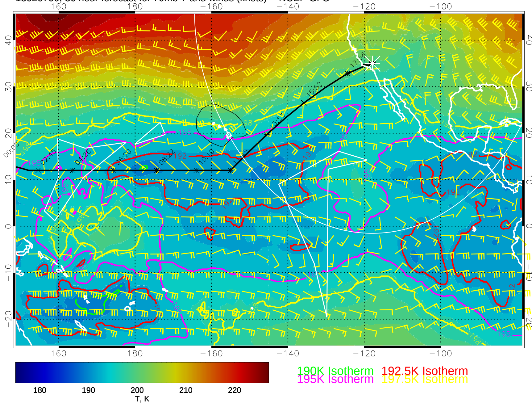
15020700, 36 hour forecast for 70mb T and winds (knots) -- NCEP GFS
