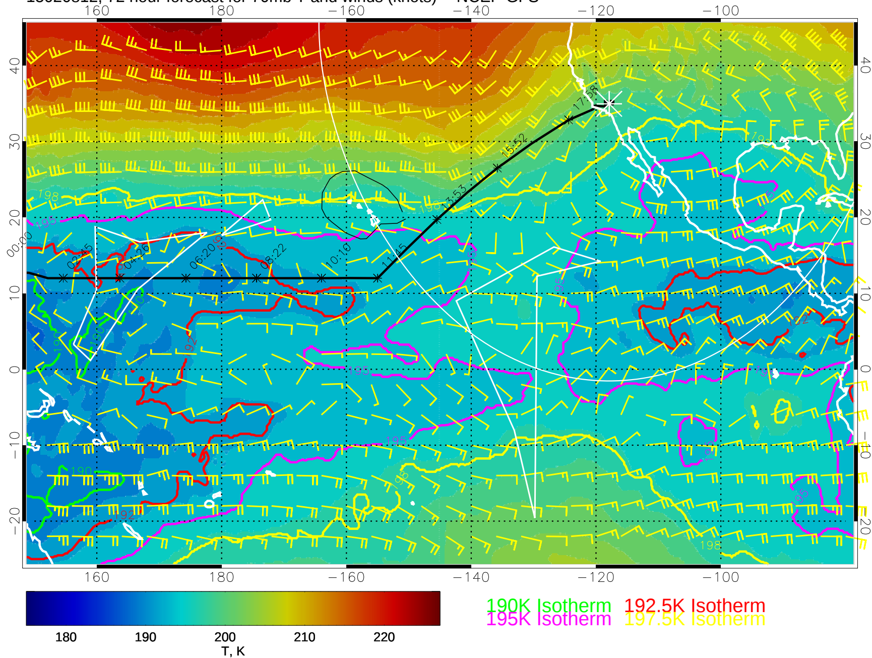
15020812, 72 hour forecast for 70mb T and winds (knots) -- NCEP GFS
