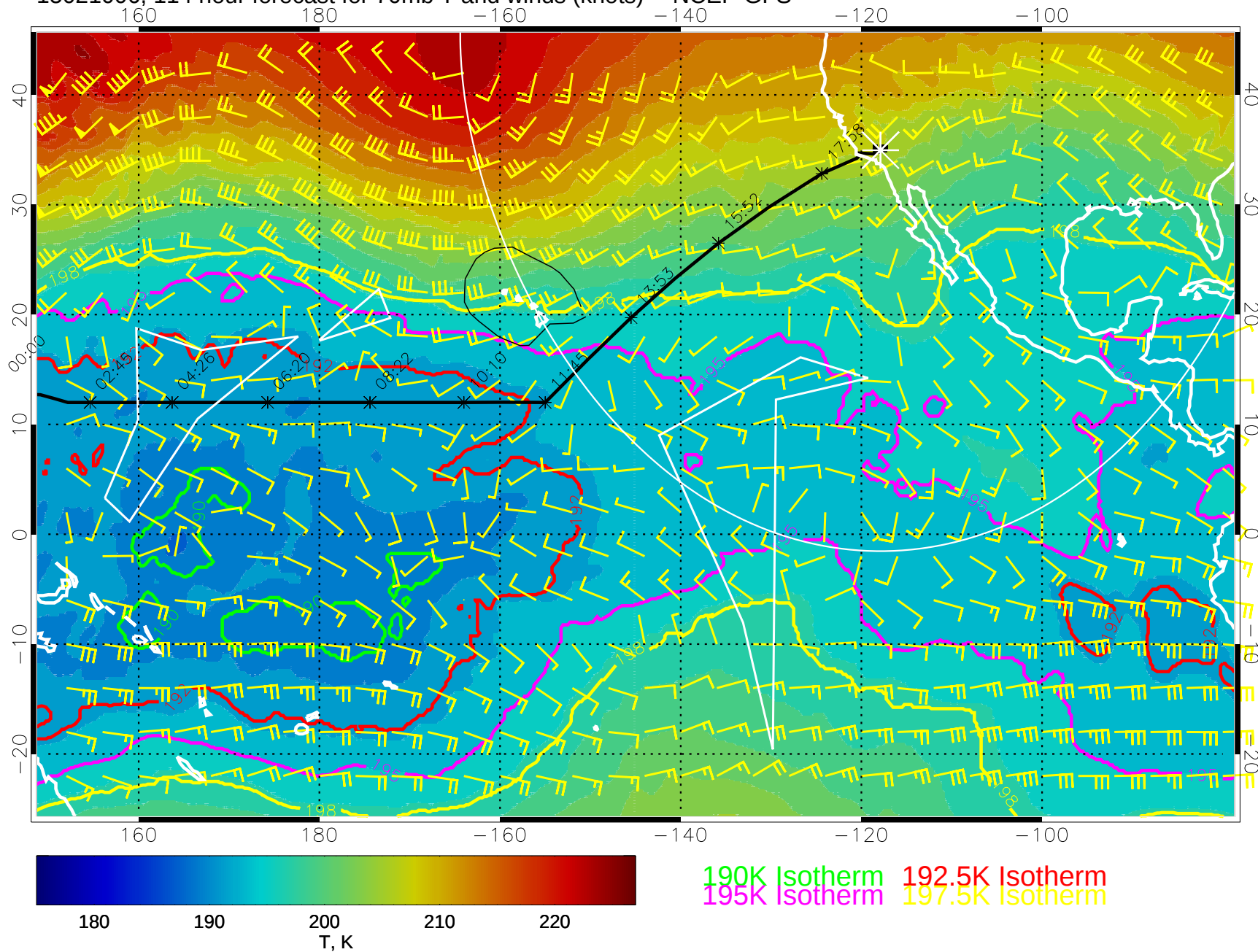
15021006, 114 hour forecast for 70mb T and winds (knots) -- NCEP GFS
