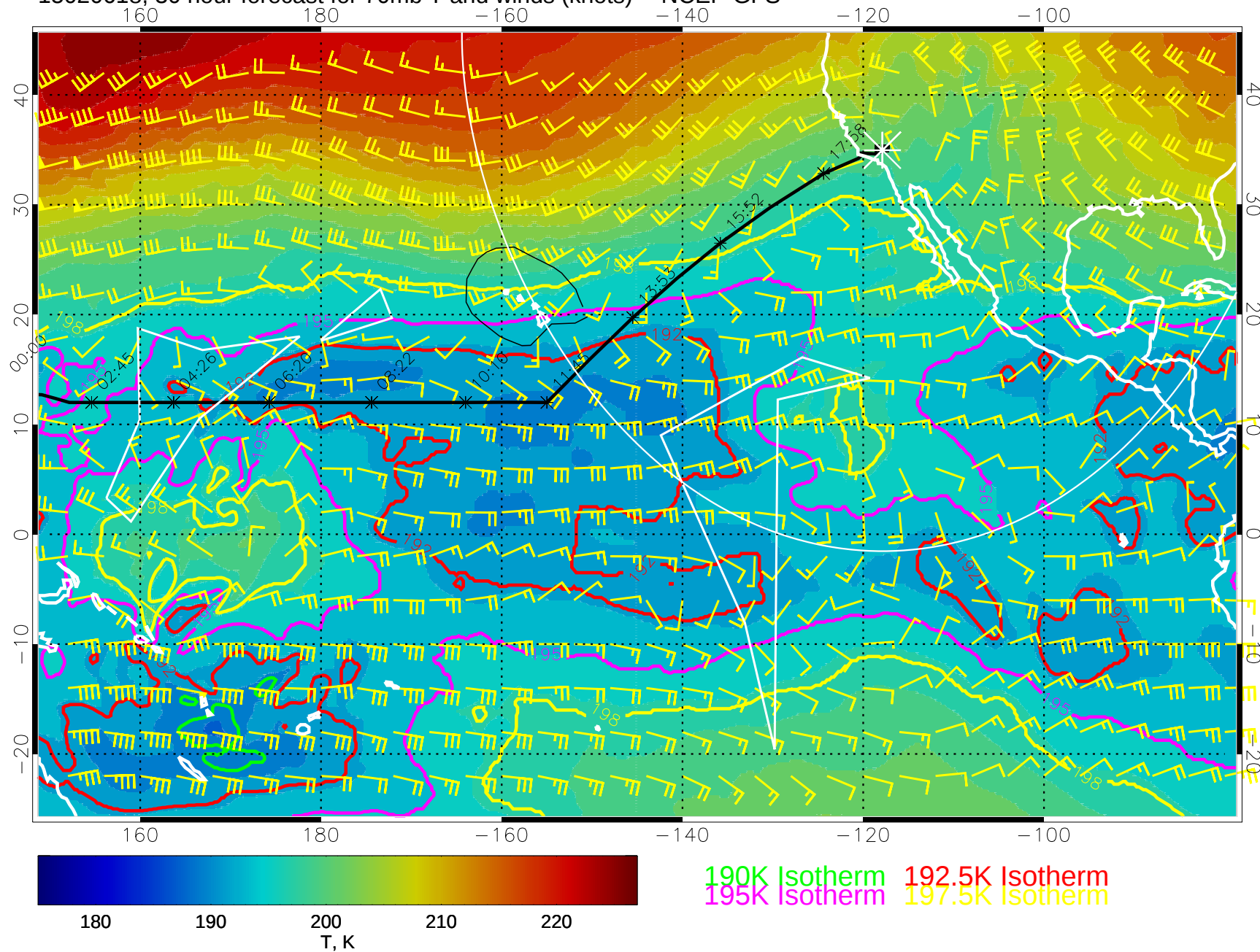
15020618, 30 hour forecast for 70mb T and winds (knots) -- NCEP GFS
