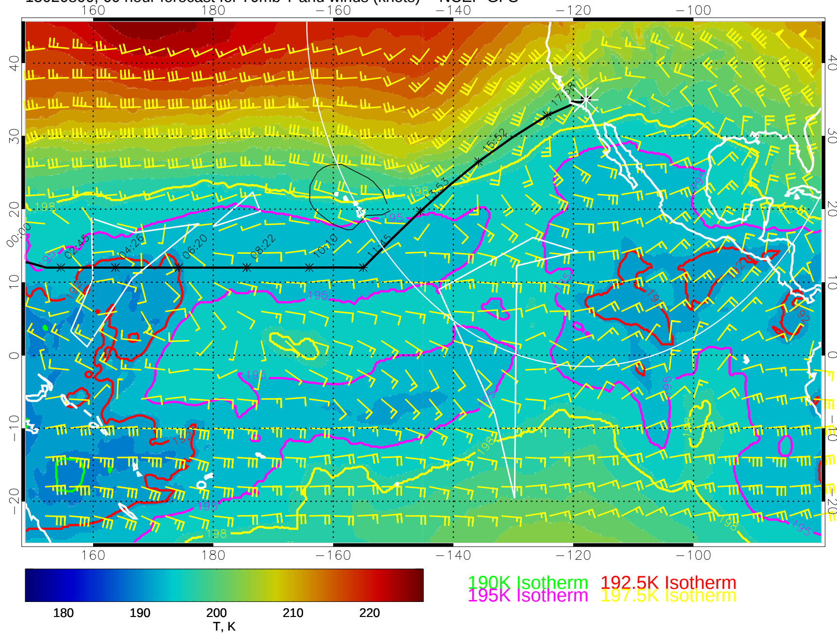
15020800, 60 hour forecast for 70mb T and winds (knots) -- NCEP GFS
