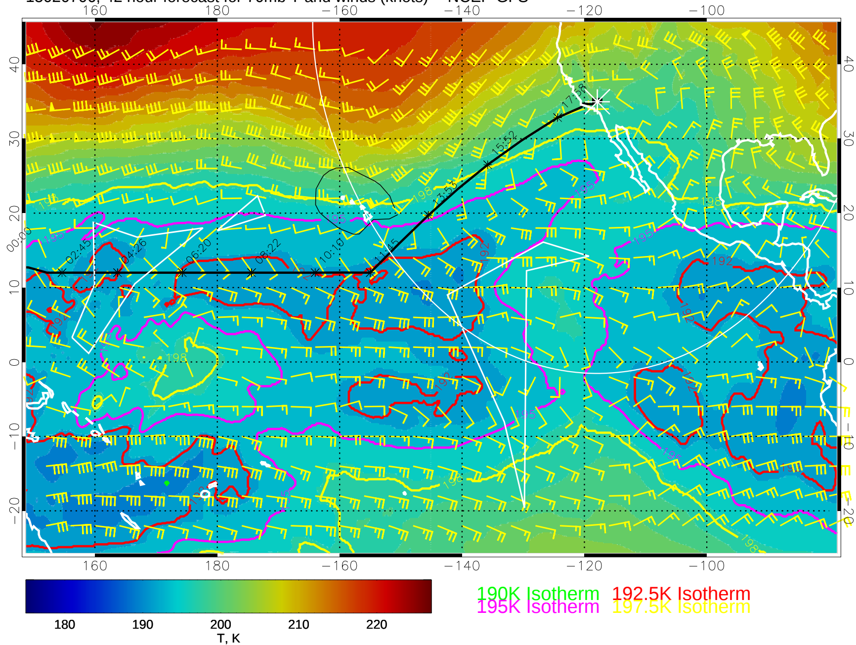
15020706, 42 hour forecast for 70mb T and winds (knots) -- NCEP GFS
