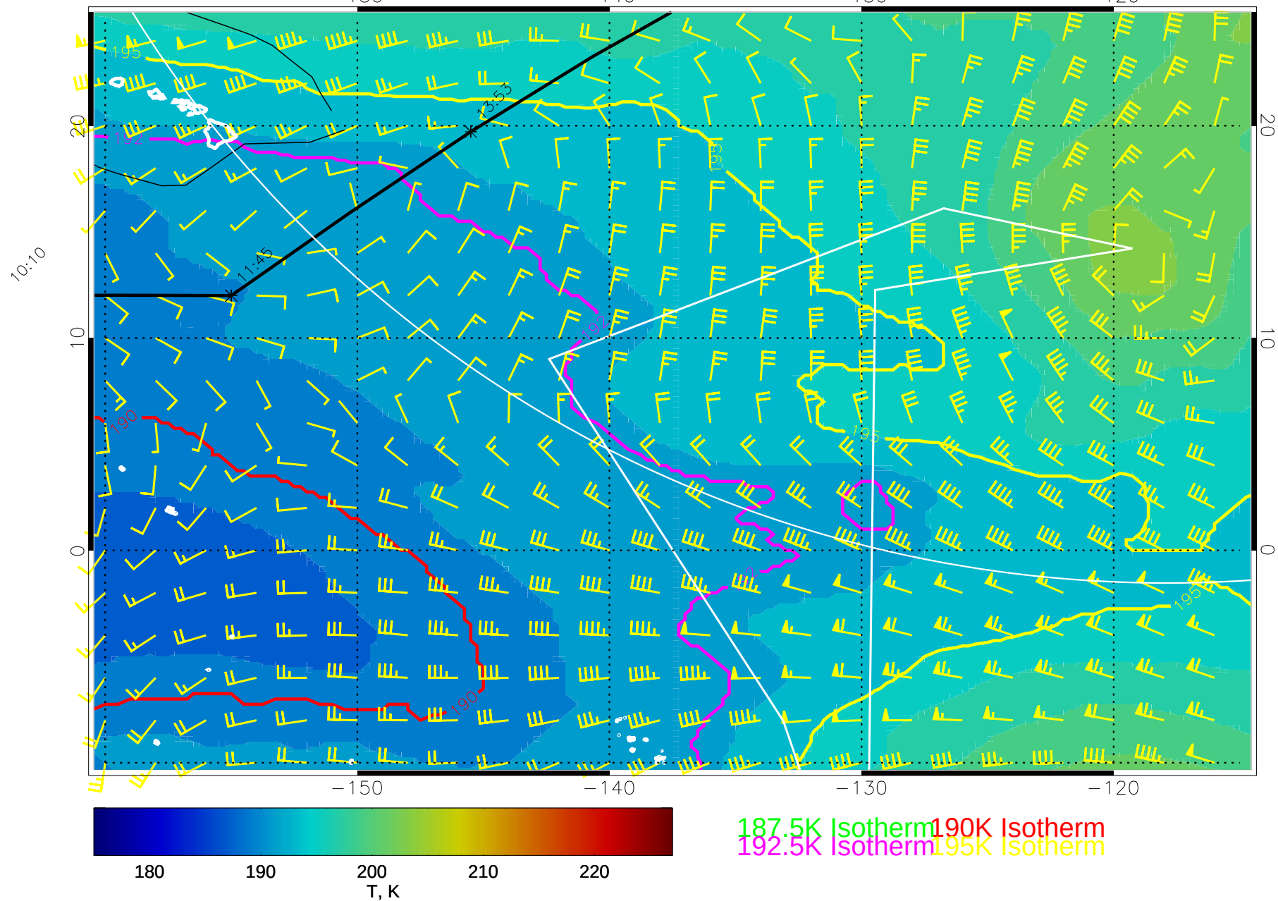
15020600, 12 hour forecast for 100mb T and winds (knots) -- NCEP GFS
