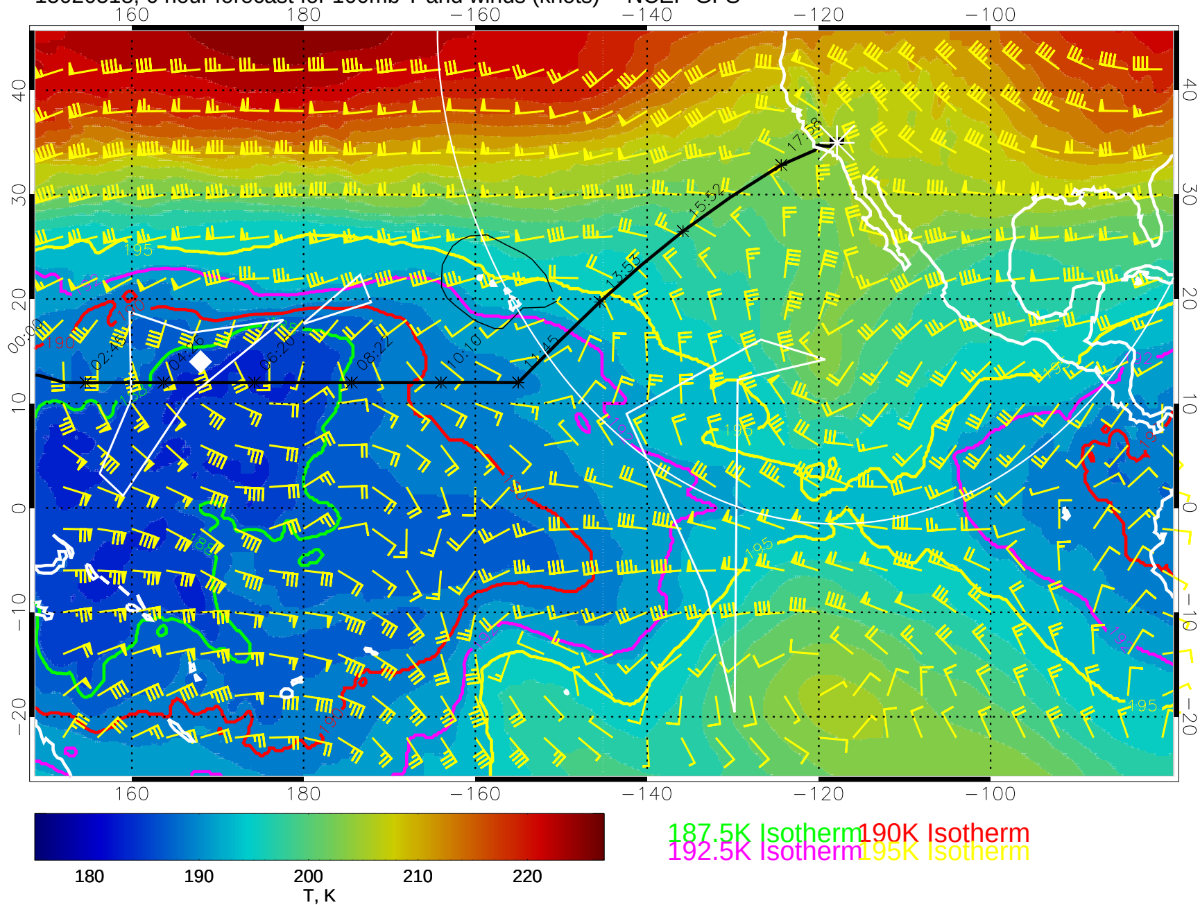
15020518, 6 hour forecast for 100mb T and winds (knots) -- NCEP GFS
