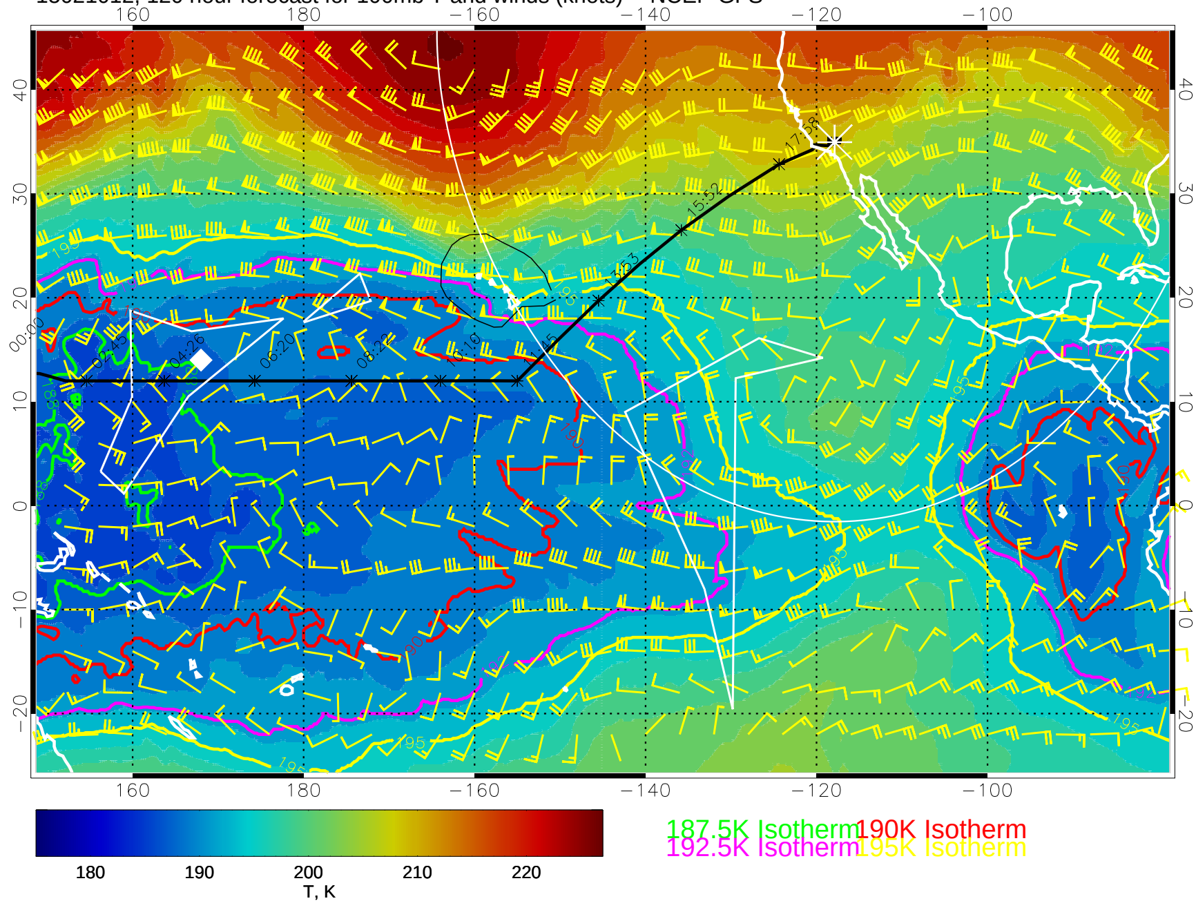
15021012, 120 hour forecast for 100mb T and winds (knots) -- NCEP GFS
