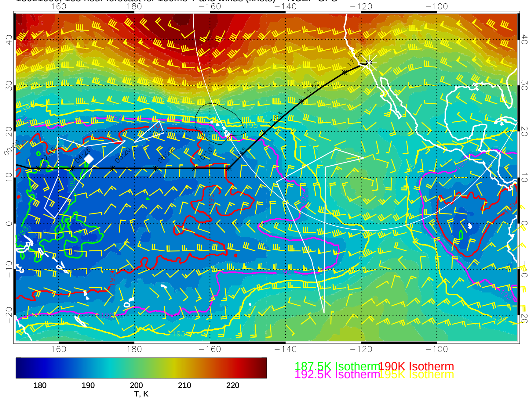
15021000, 108 hour forecast for 100mb T and winds (knots) -- NCEP GFS
