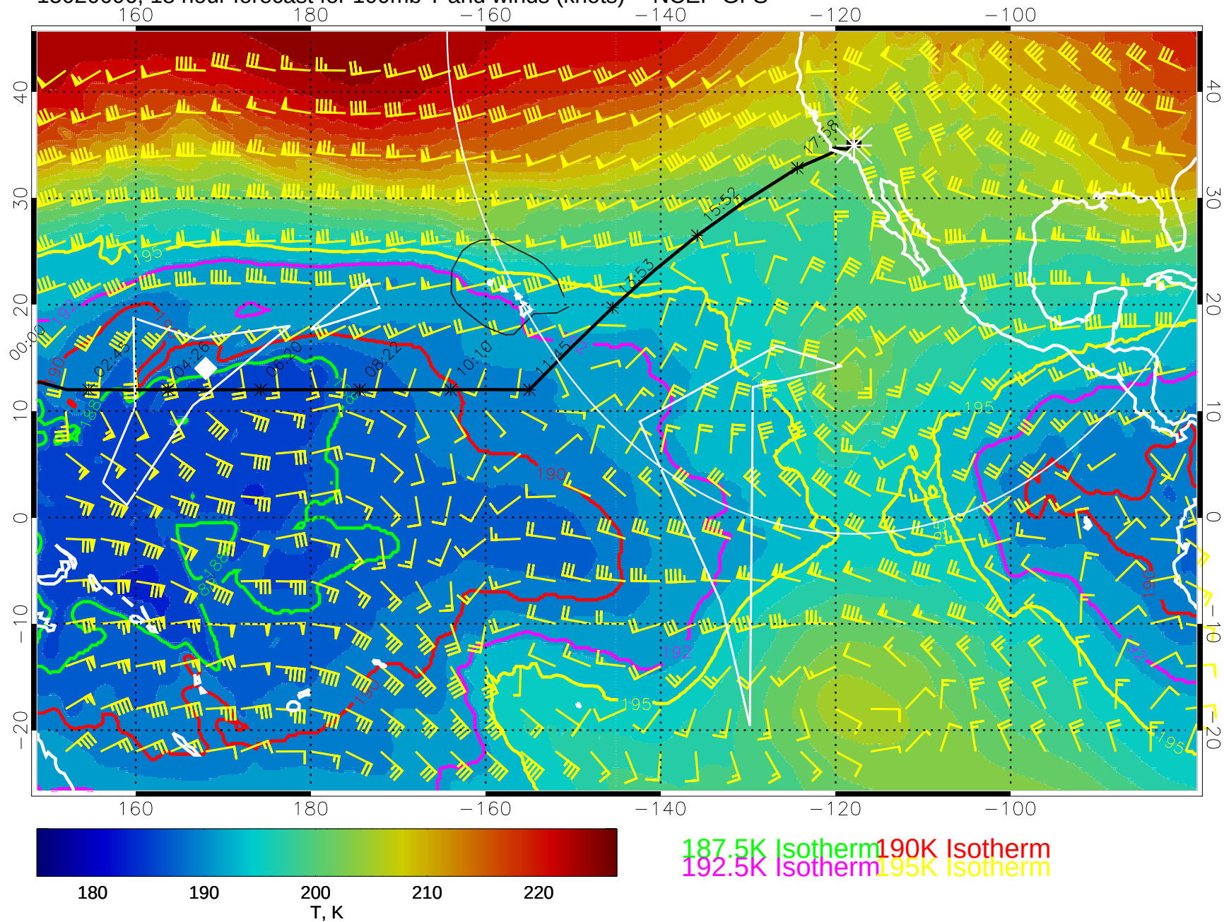
15020606, 18 hour forecast for 100mb T and winds (knots) -- NCEP GFS
