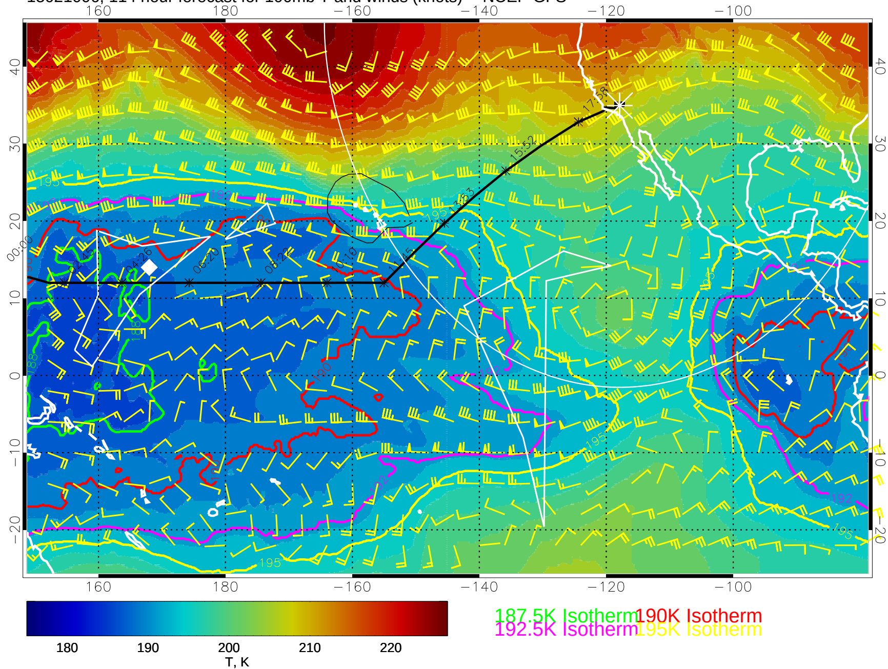
15021006, 114 hour forecast for 100mb T and winds (knots) -- NCEP GFS
