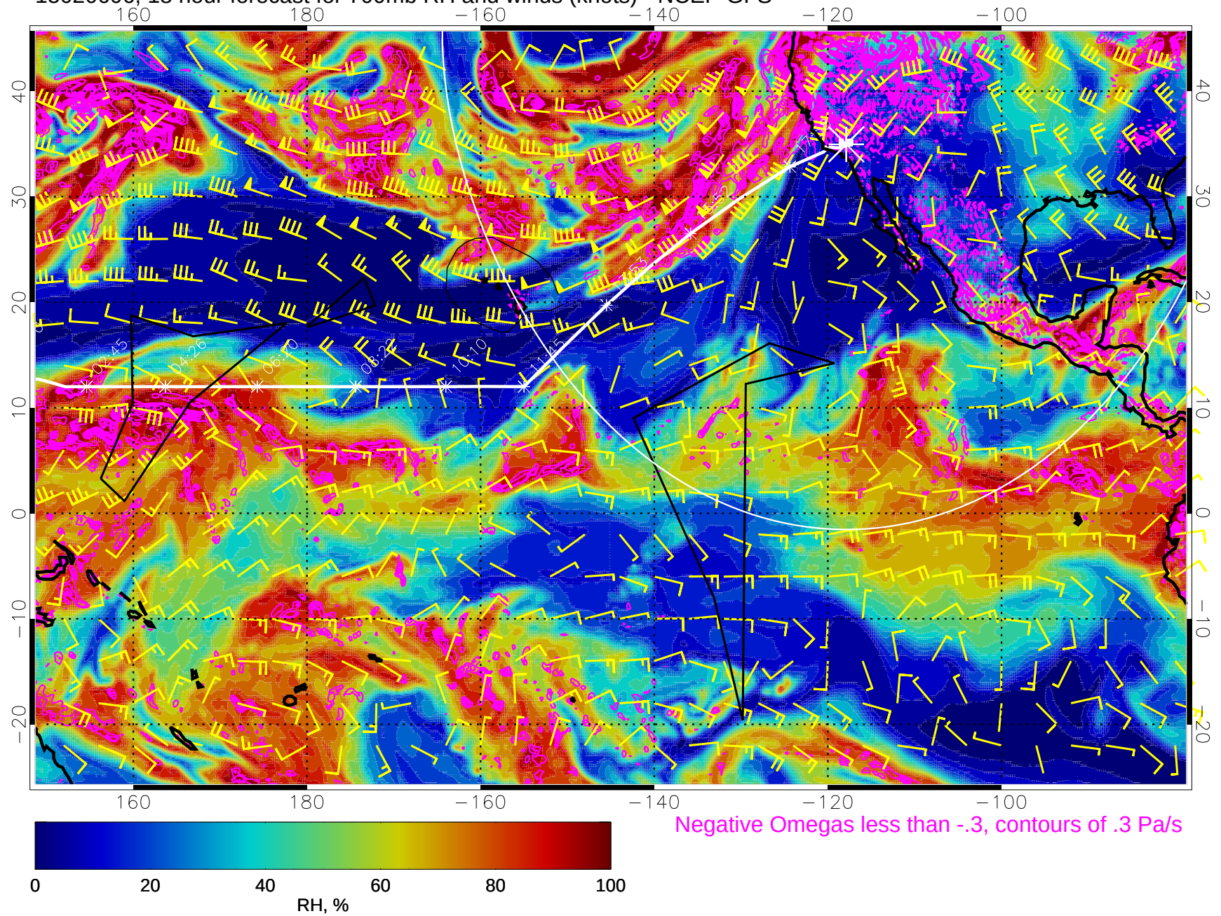
15020606, 18 hour forecast for 700mb RH and winds (knots) - NCEP GFS
