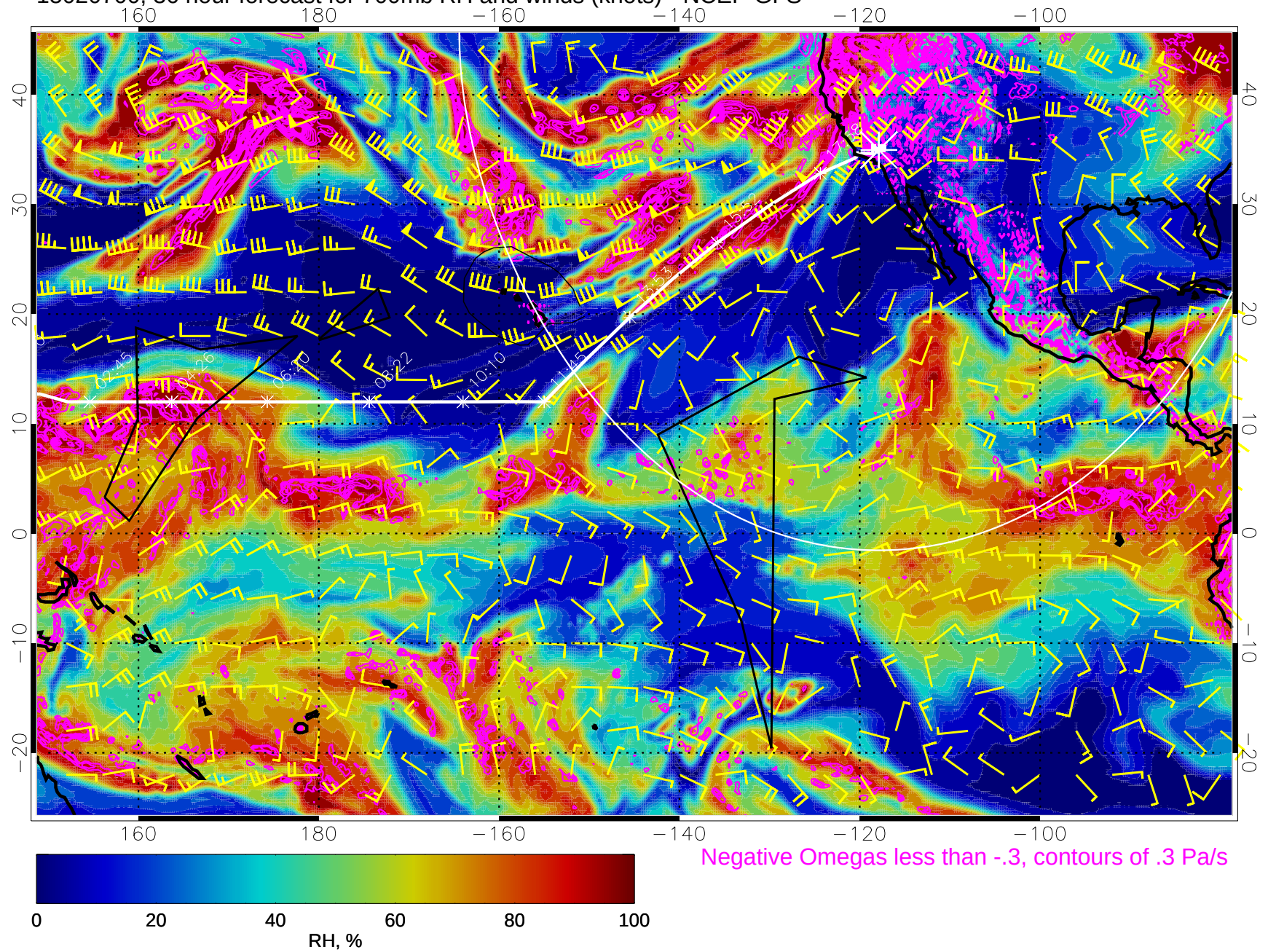
15020700, 36 hour forecast for 700mb RH and winds (knots) - NCEP GFS
