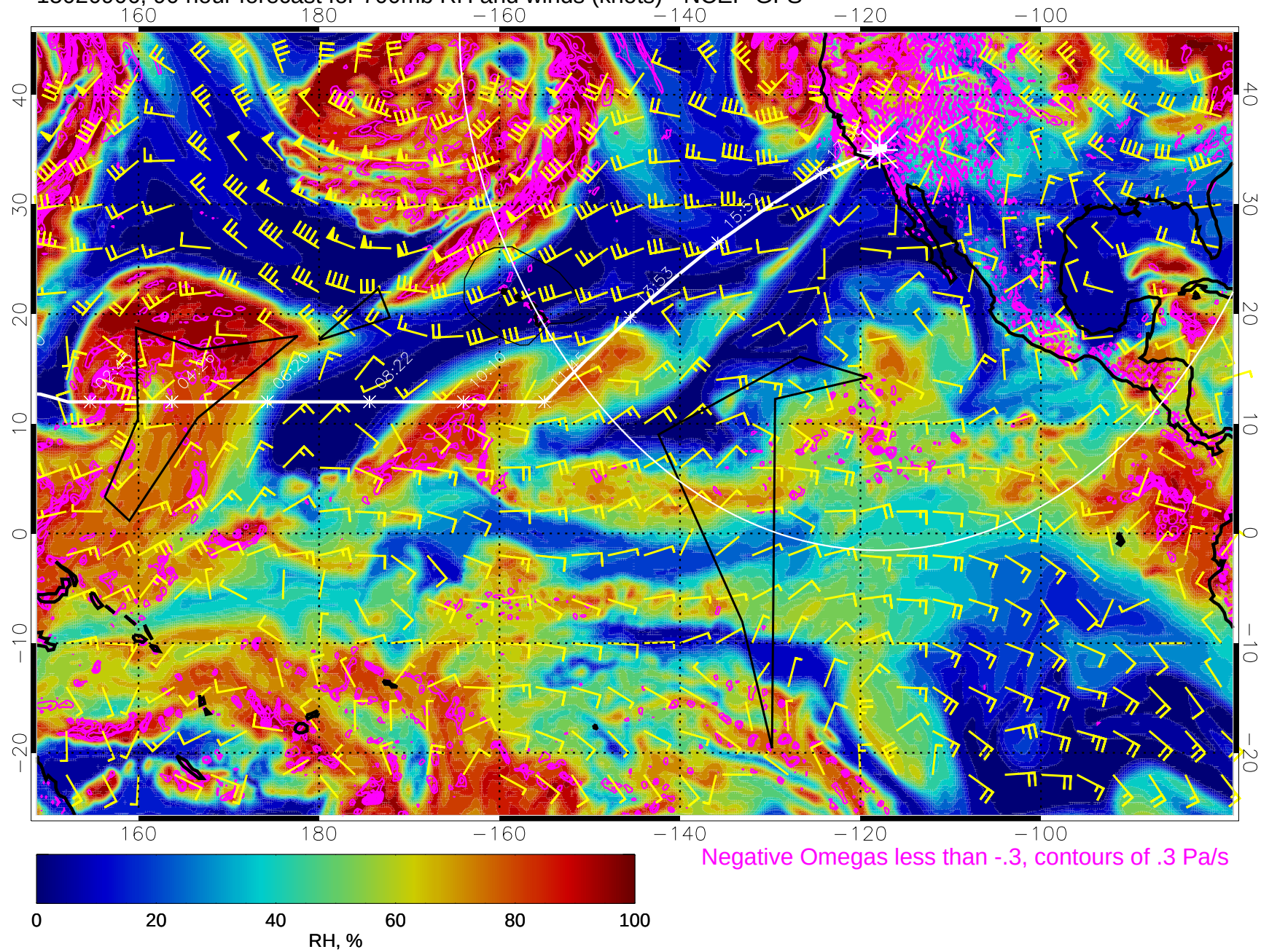
15020906, 90 hour forecast for 700mb RH and winds (knots) - NCEP GFS
