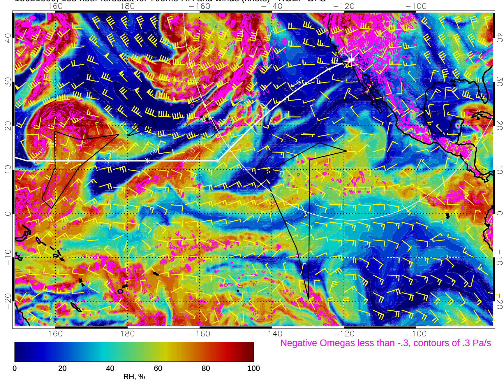
15021000, 108 hour forecast for 700mb RH and winds (knots) - NCEP GFS
