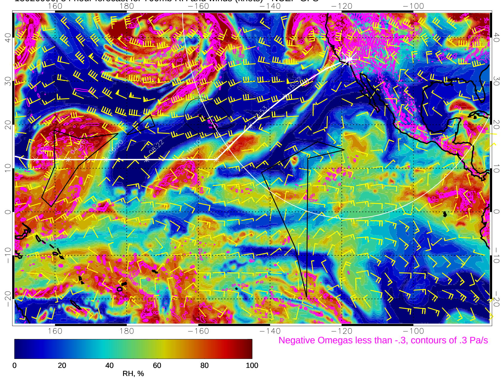
15020900, 84 hour forecast for 700mb RH and winds (knots) - NCEP GFS
