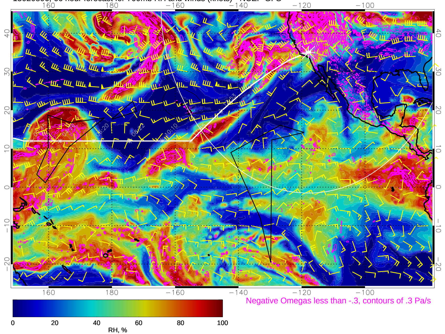
15020806, 66 hour forecast for 700mb RH and winds (knots) - NCEP GFS
