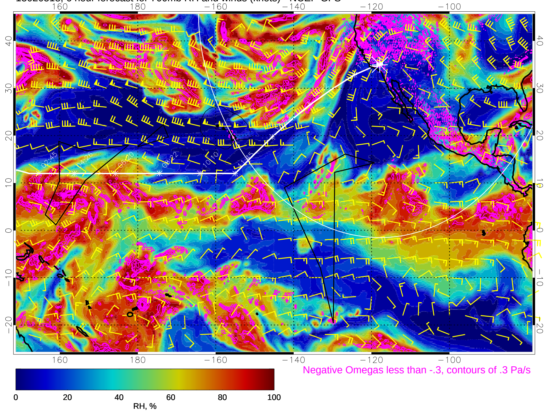
15020518, 6 hour forecast for 700mb RH and winds (knots) - NCEP GFS
