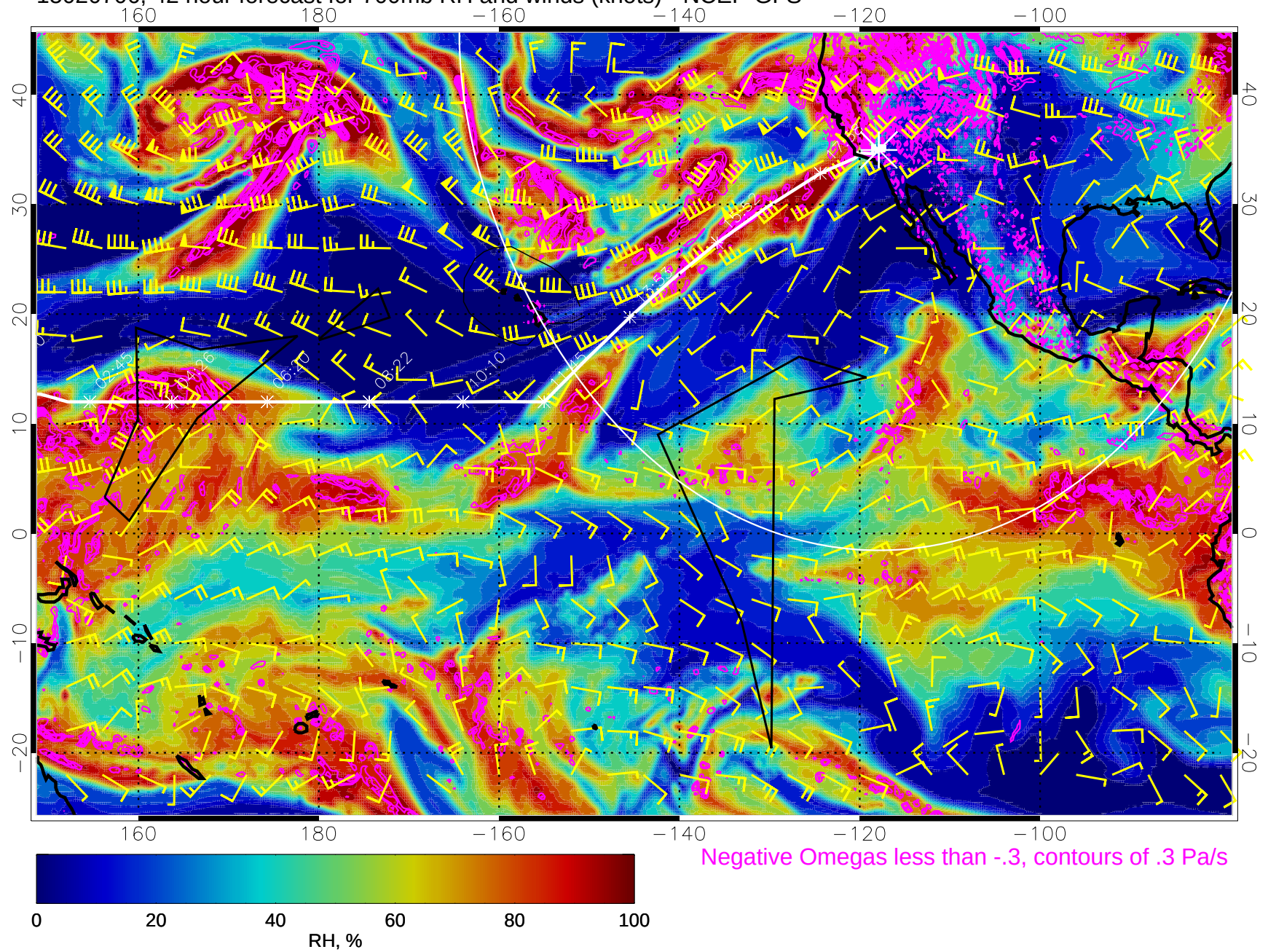
15020706, 42 hour forecast for 700mb RH and winds (knots) - NCEP GFS
