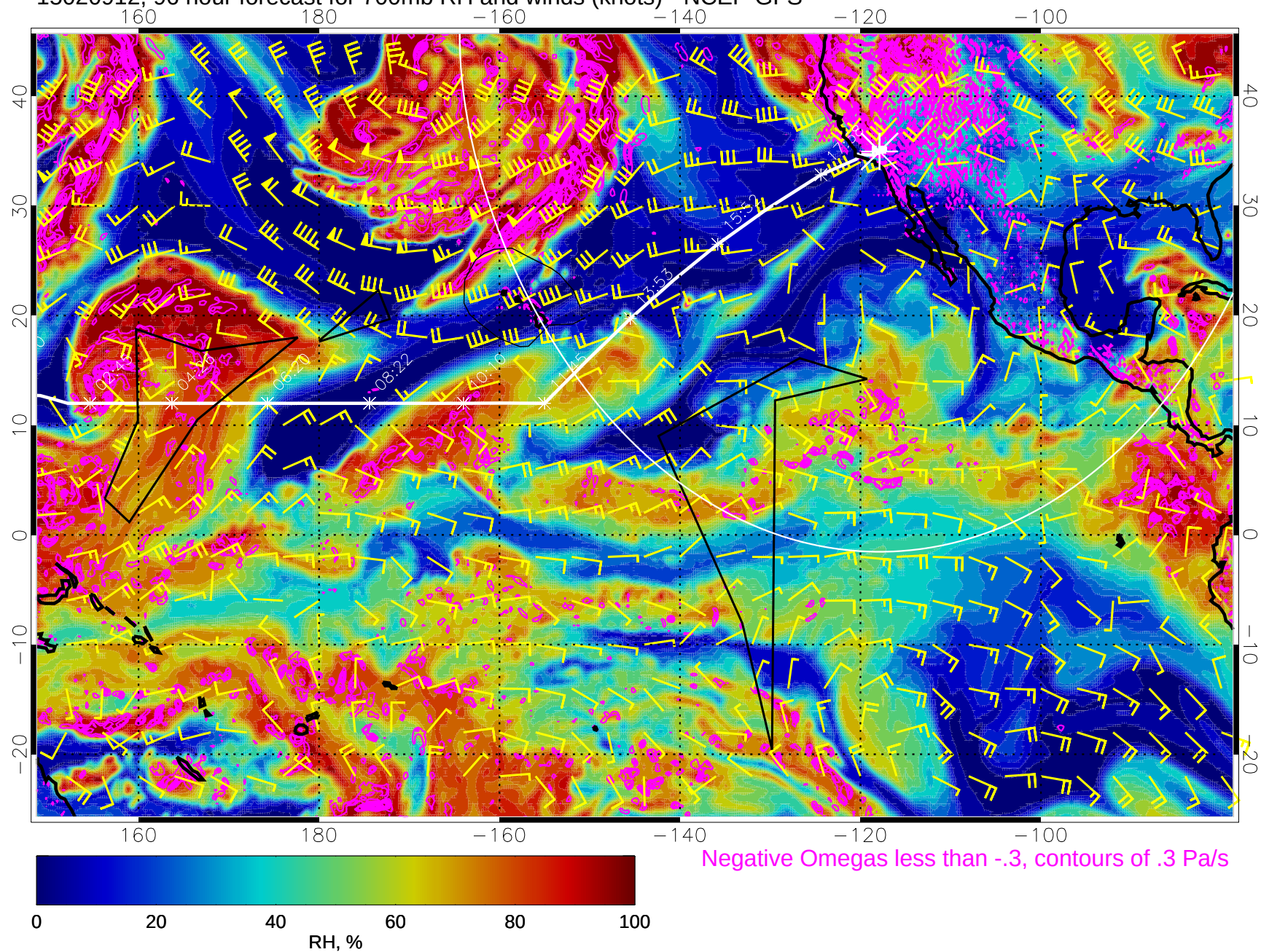
15020912, 96 hour forecast for 700mb RH and winds (knots) - NCEP GFS
