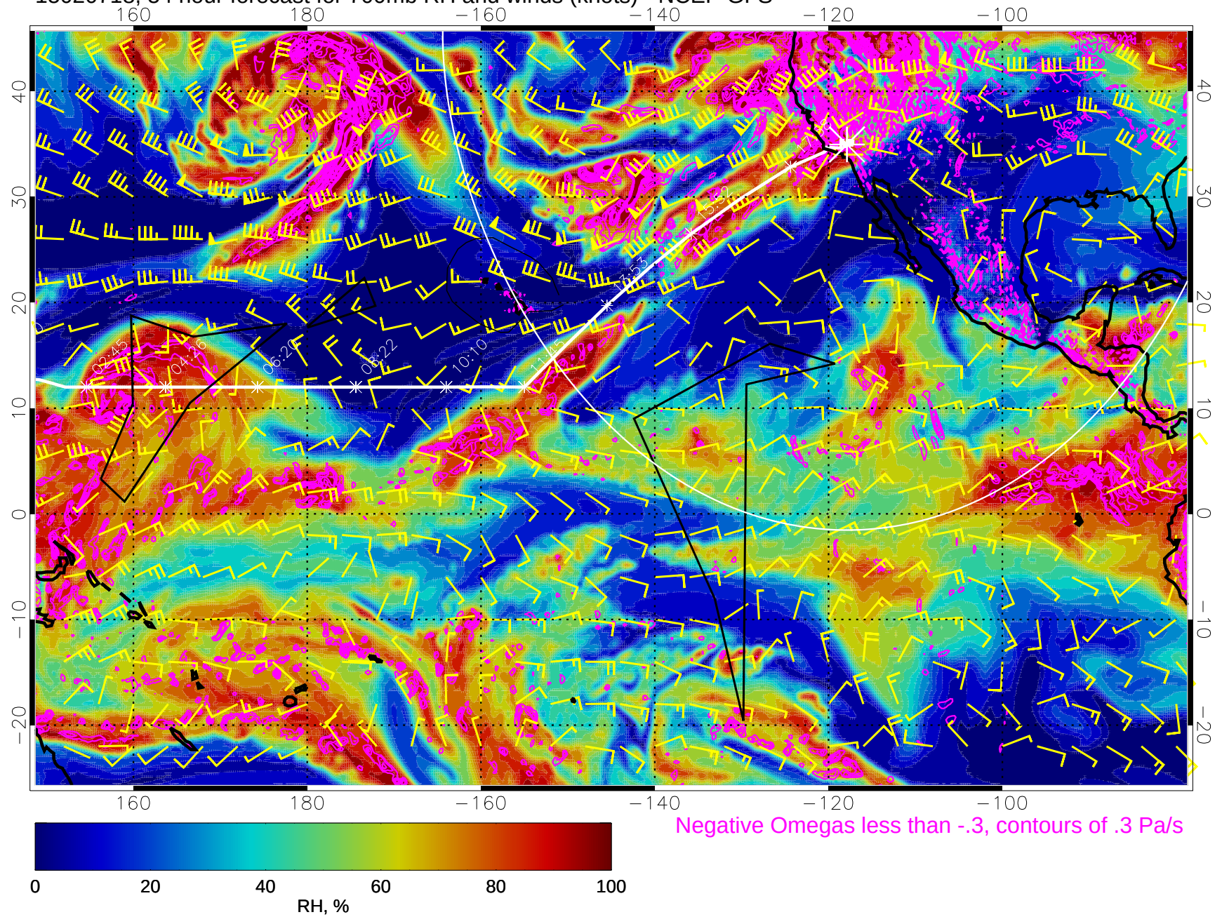
15020718, 54 hour forecast for 700mb RH and winds (knots) - NCEP GFS
