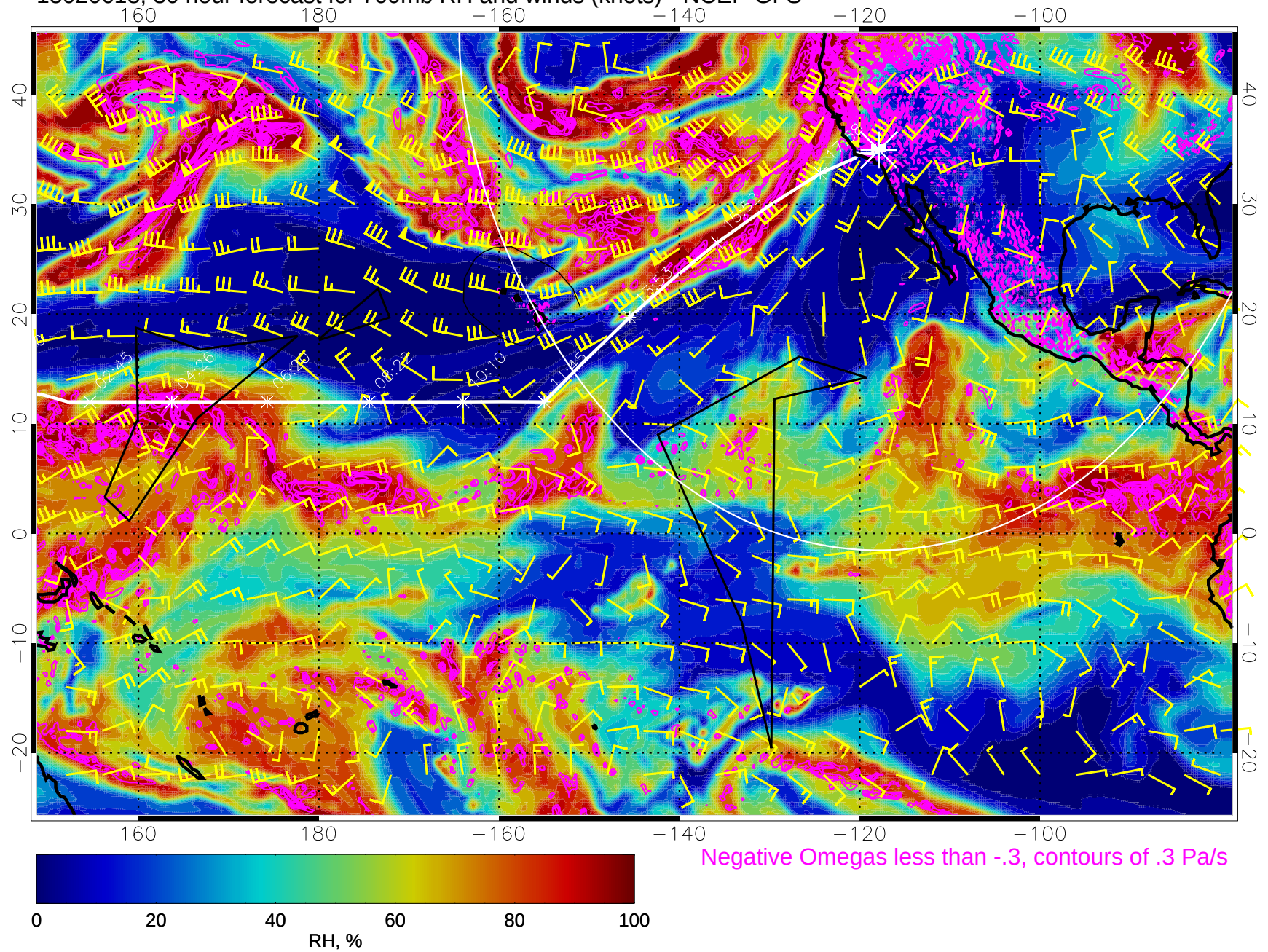
15020618, 30 hour forecast for 700mb RH and winds (knots) - NCEP GFS
