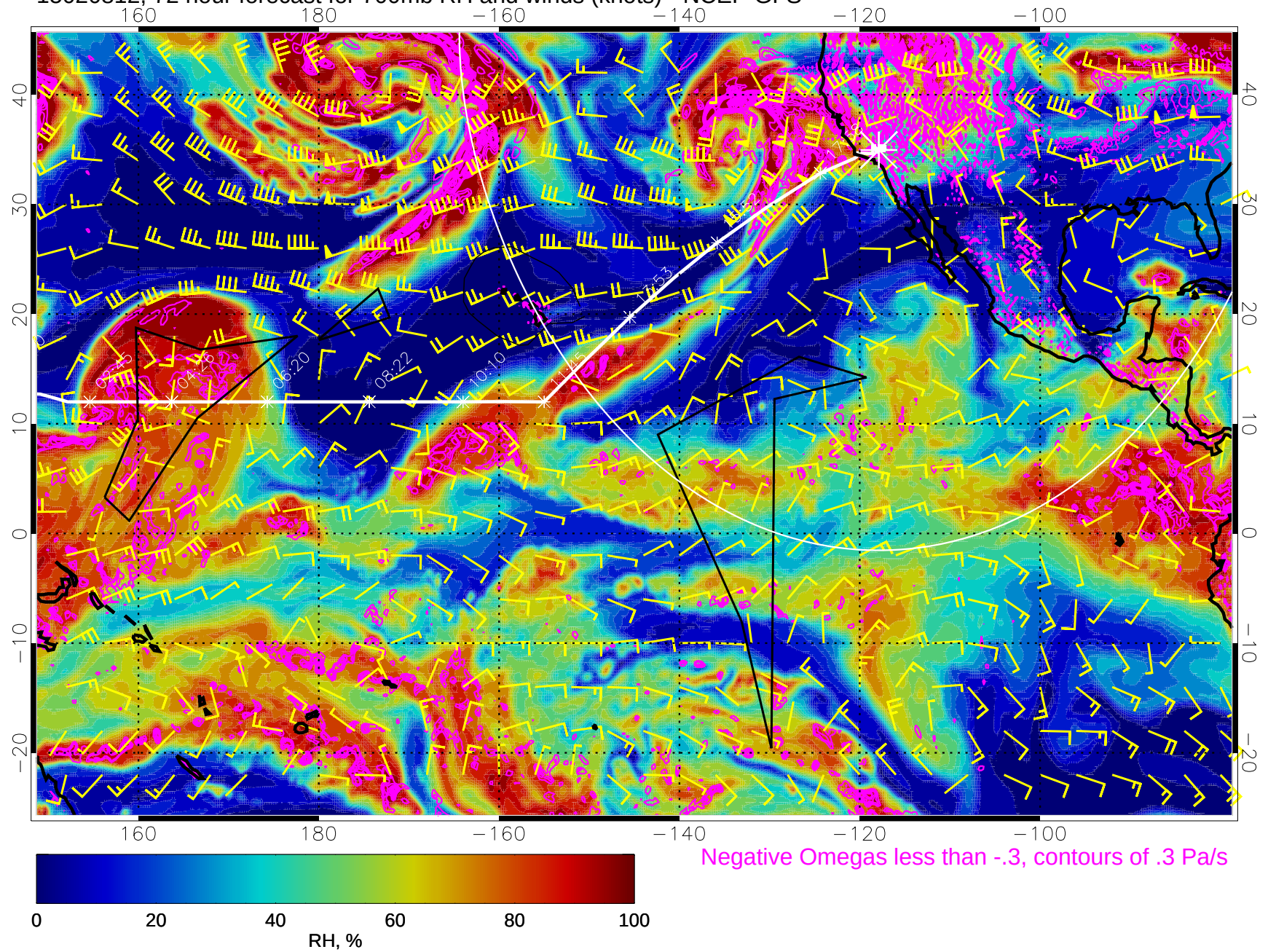
15020812, 72 hour forecast for 700mb RH and winds (knots) - NCEP GFS
