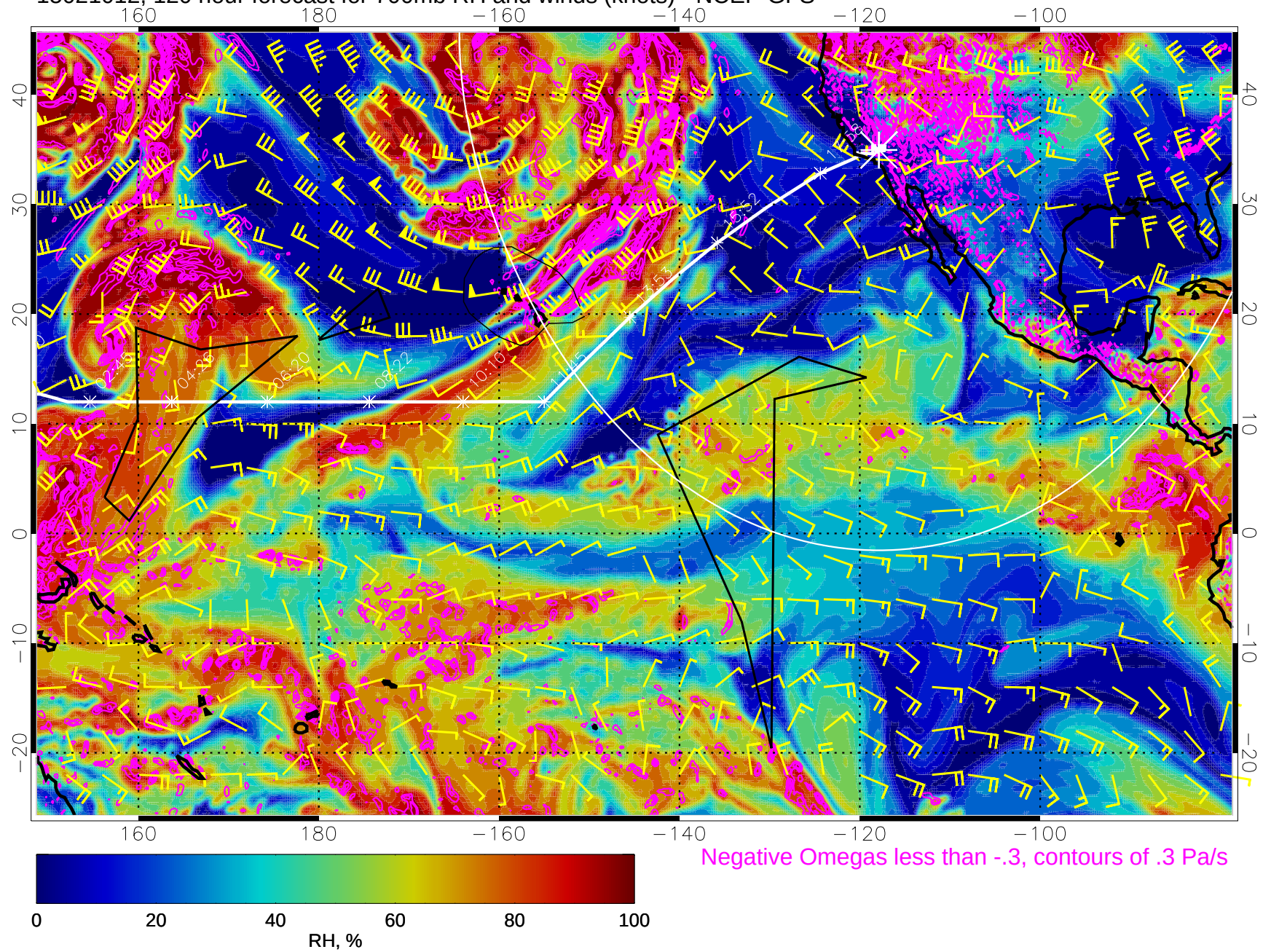
15021012, 120 hour forecast for 700mb RH and winds (knots) - NCEP GFS
