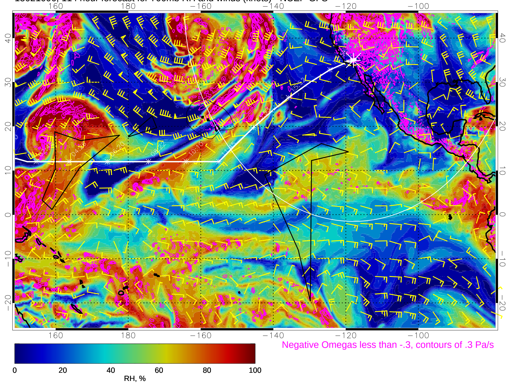
15021006, 114 hour forecast for 700mb RH and winds (knots) - NCEP GFS
