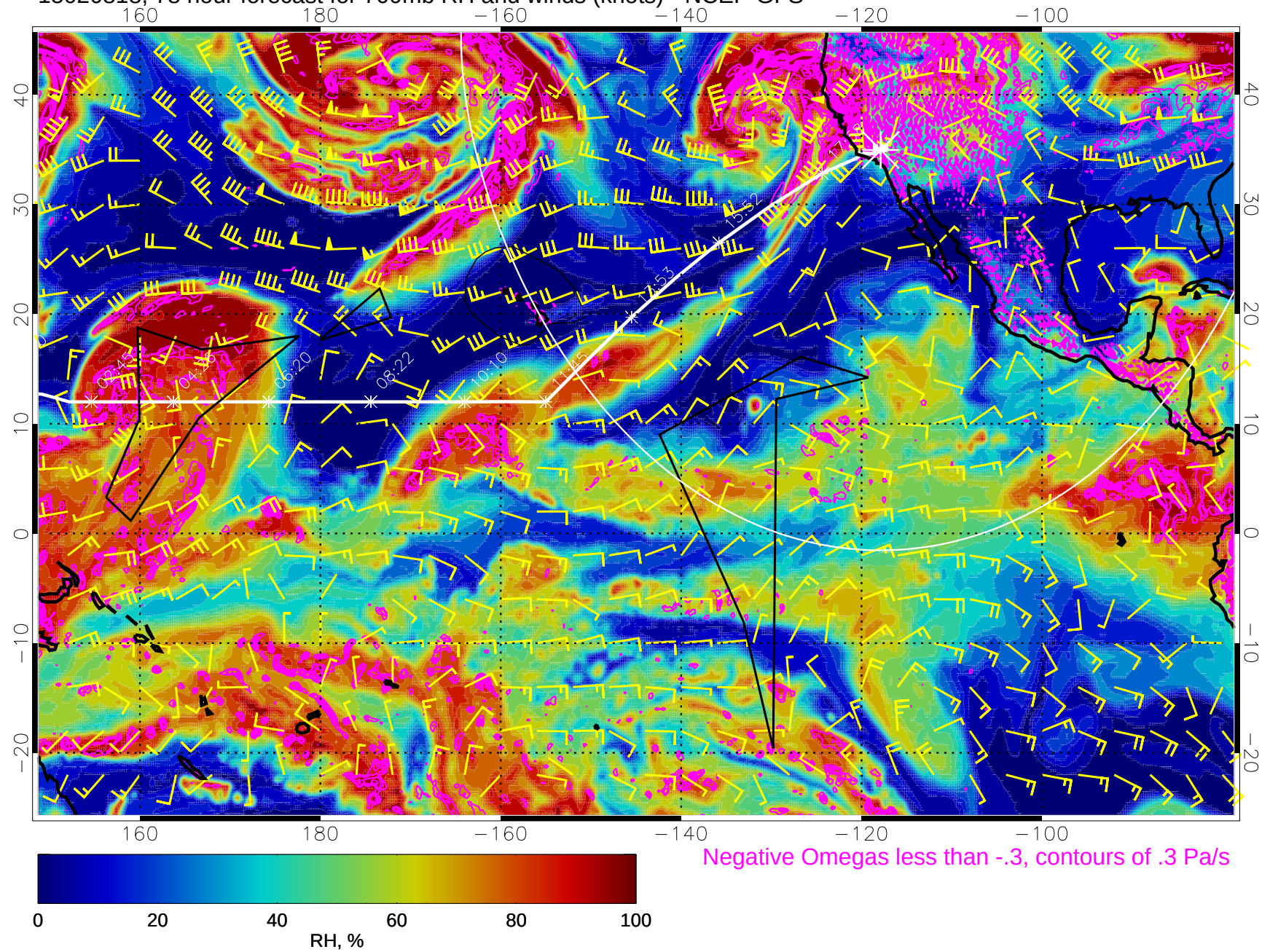
15020818, 78 hour forecast for 700mb RH and winds (knots) - NCEP GFS
