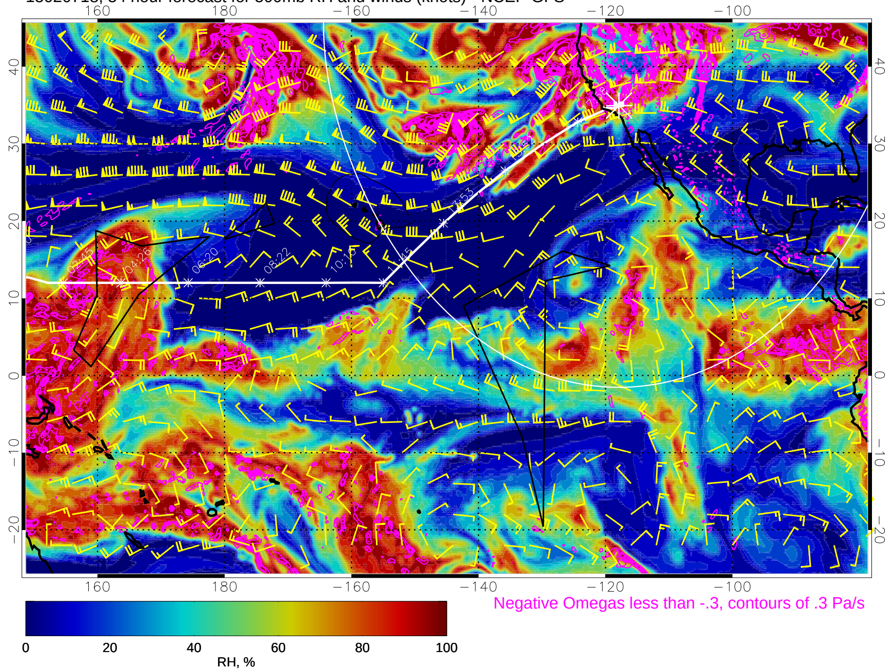
15020718, 54 hour forecast for 500mb RH and winds (knots) - NCEP GFS
