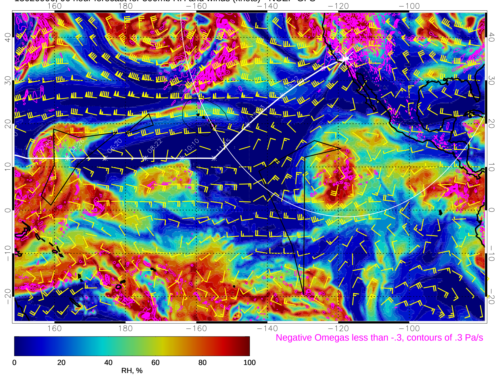
15020906, 90 hour forecast for 500mb RH and winds (knots) - NCEP GFS
