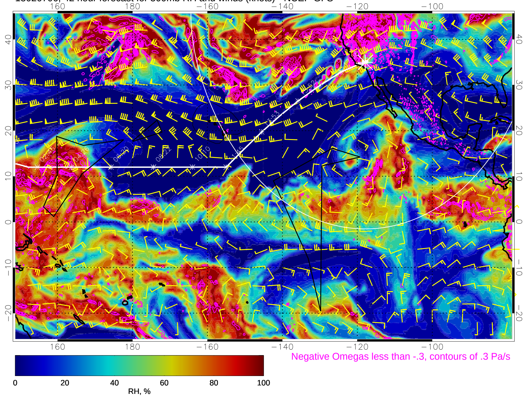
15020706, 42 hour forecast for 500mb RH and winds (knots) - NCEP GFS
