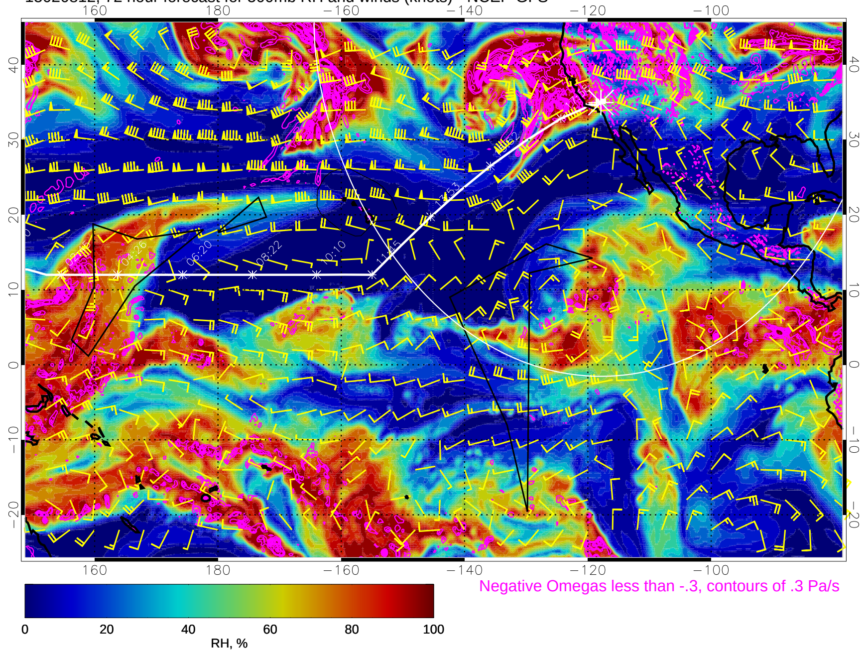
15020812, 72 hour forecast for 500mb RH and winds (knots) - NCEP GFS
