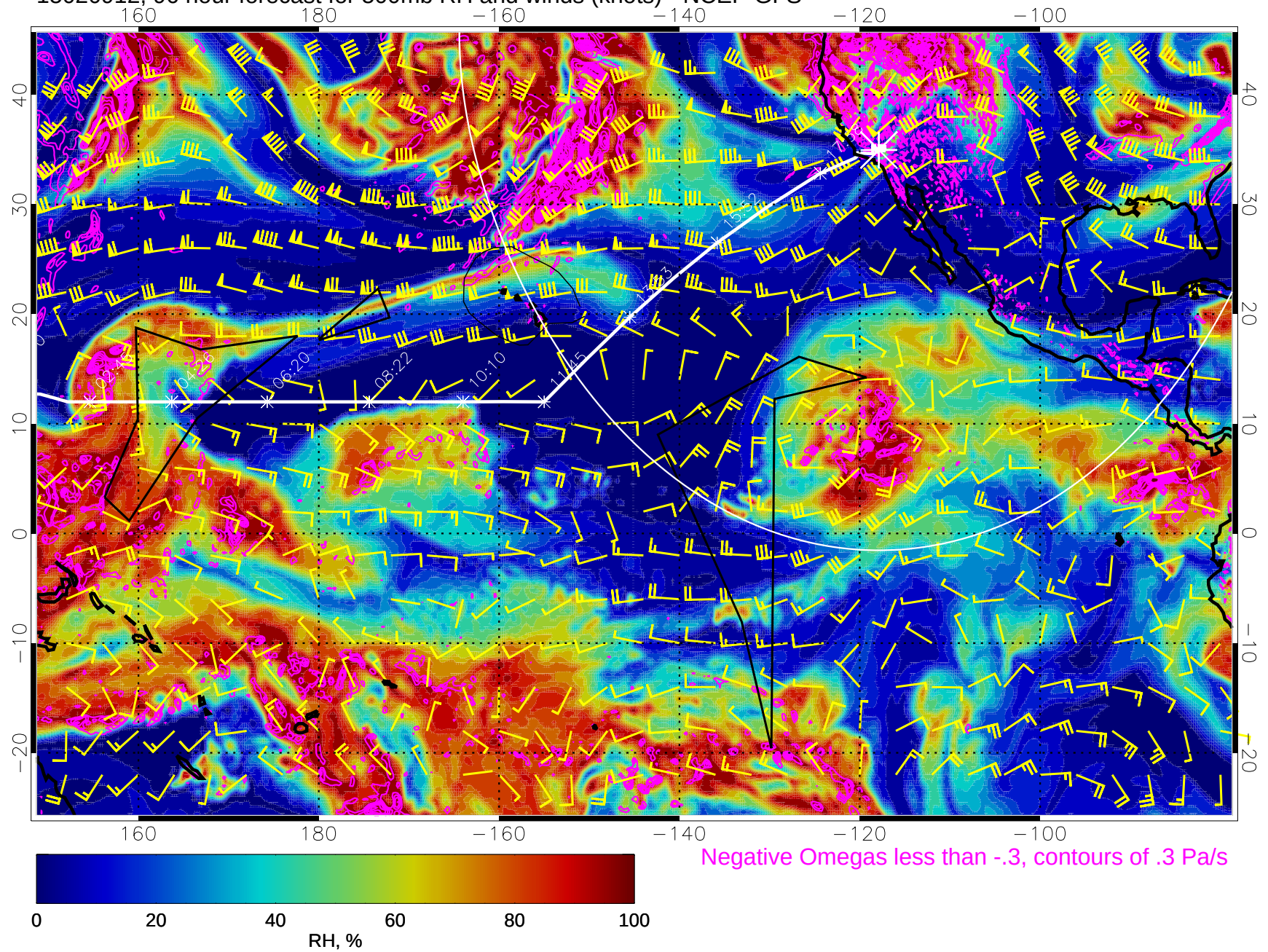
15020912, 96 hour forecast for 500mb RH and winds (knots) - NCEP GFS
