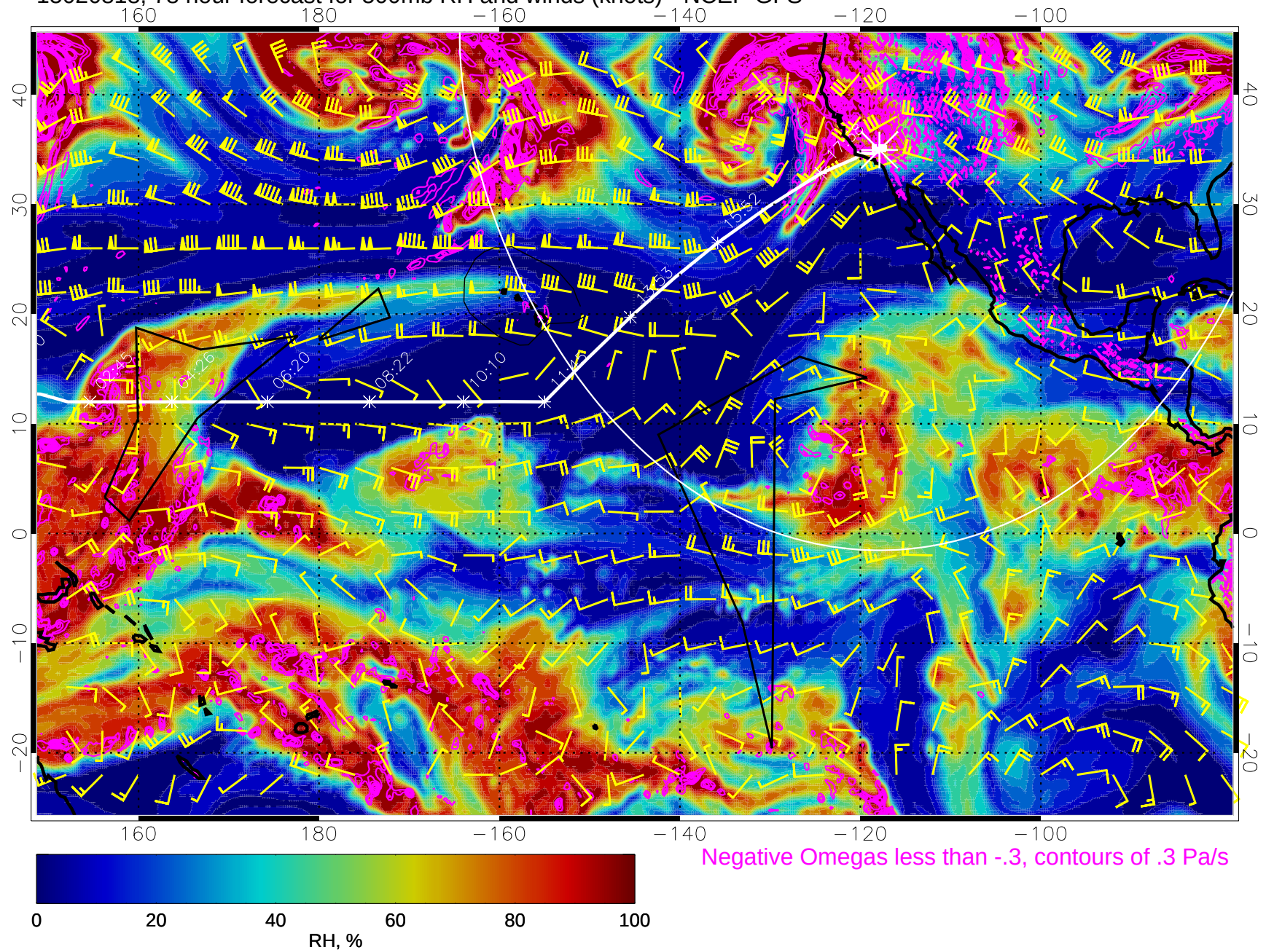
15020818, 78 hour forecast for 500mb RH and winds (knots) - NCEP GFS
