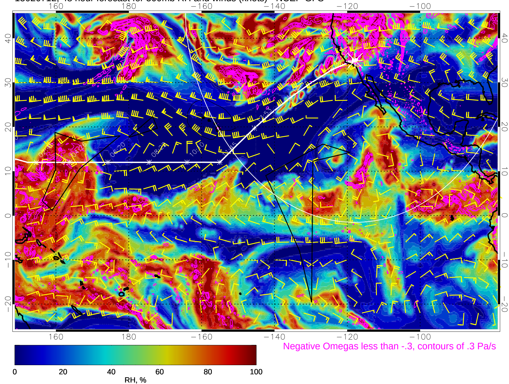
15020712, 48 hour forecast for 500mb RH and winds (knots) - NCEP GFS
