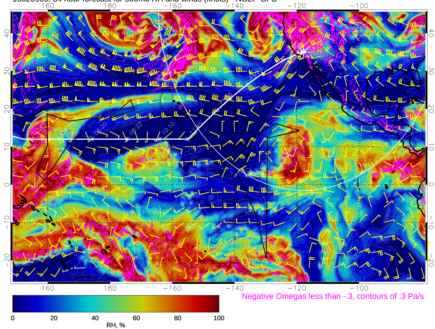
15020900, 84 hour forecast for 500mb RH and winds (knots) - NCEP GFS
