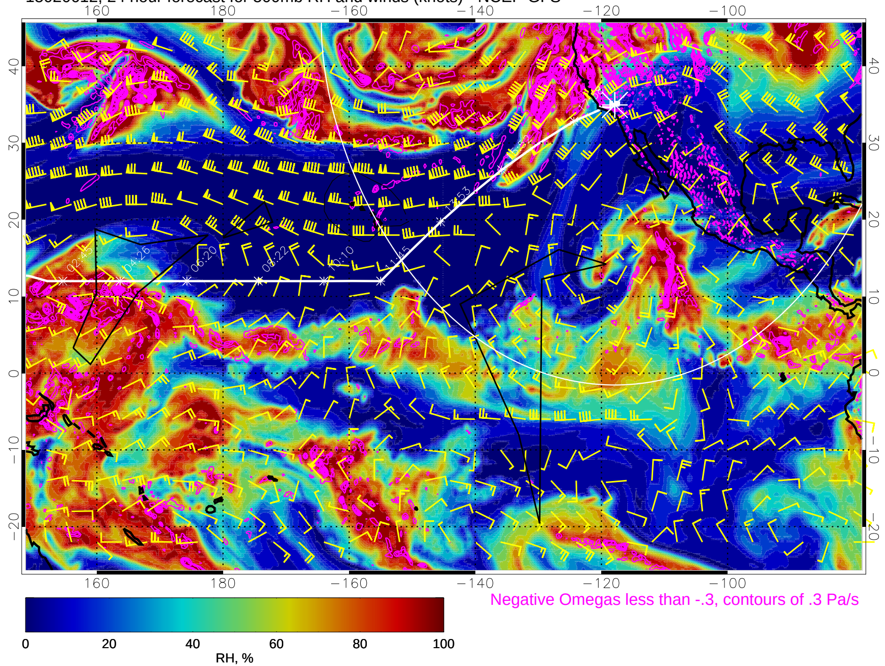
15020612, 24 hour forecast for 500mb RH and winds (knots) - NCEP GFS
