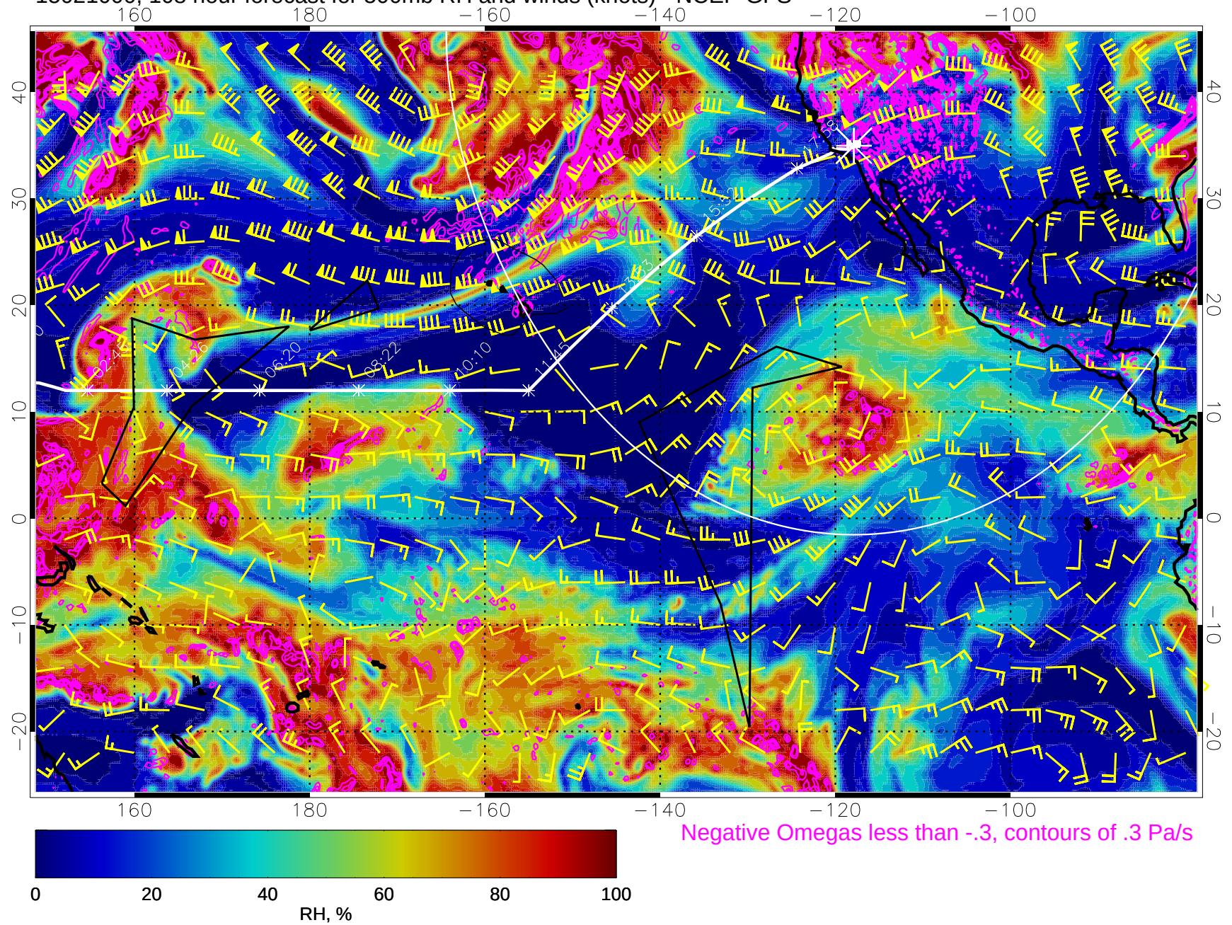
15021000, 108 hour forecast for 500mb RH and winds (knots) - NCEP GFS
