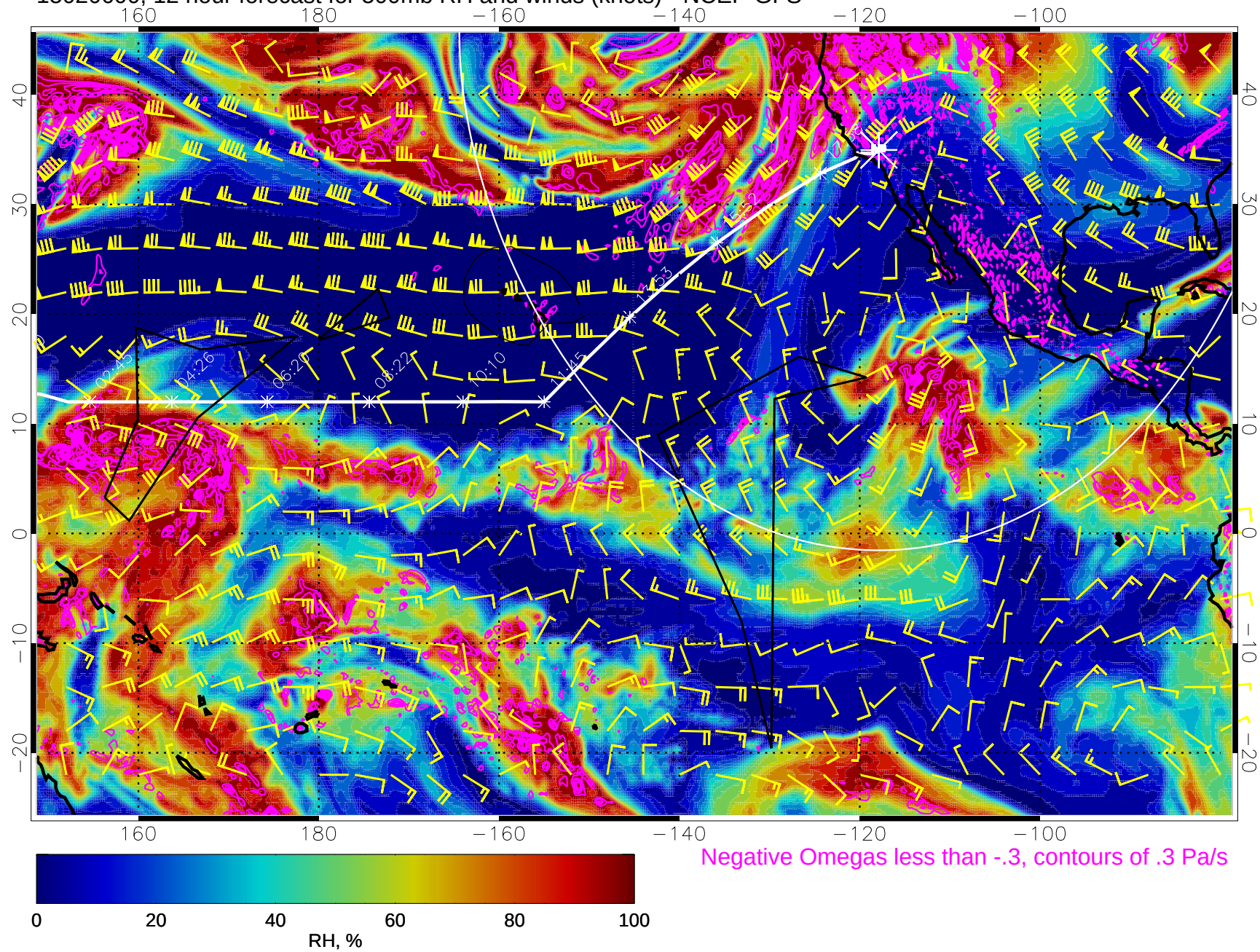
15020600, 12 hour forecast for 500mb RH and winds (knots) - NCEP GFS
