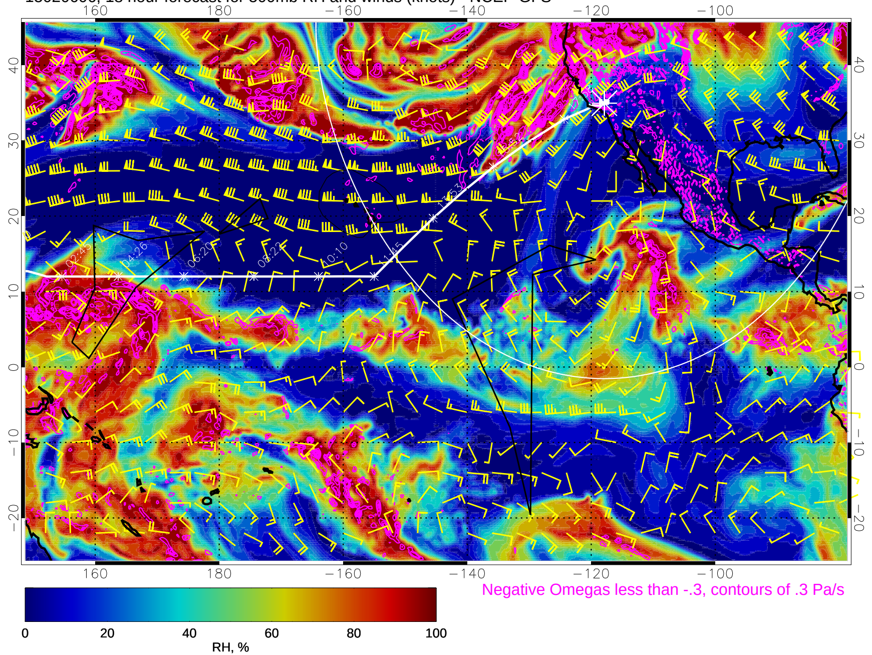
15020606, 18 hour forecast for 500mb RH and winds (knots) - NCEP GFS
