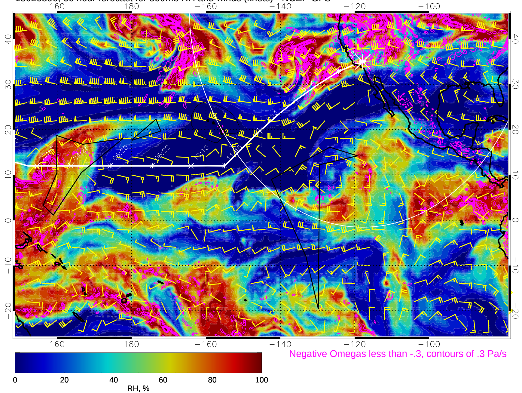
15020806, 66 hour forecast for 500mb RH and winds (knots) - NCEP GFS
