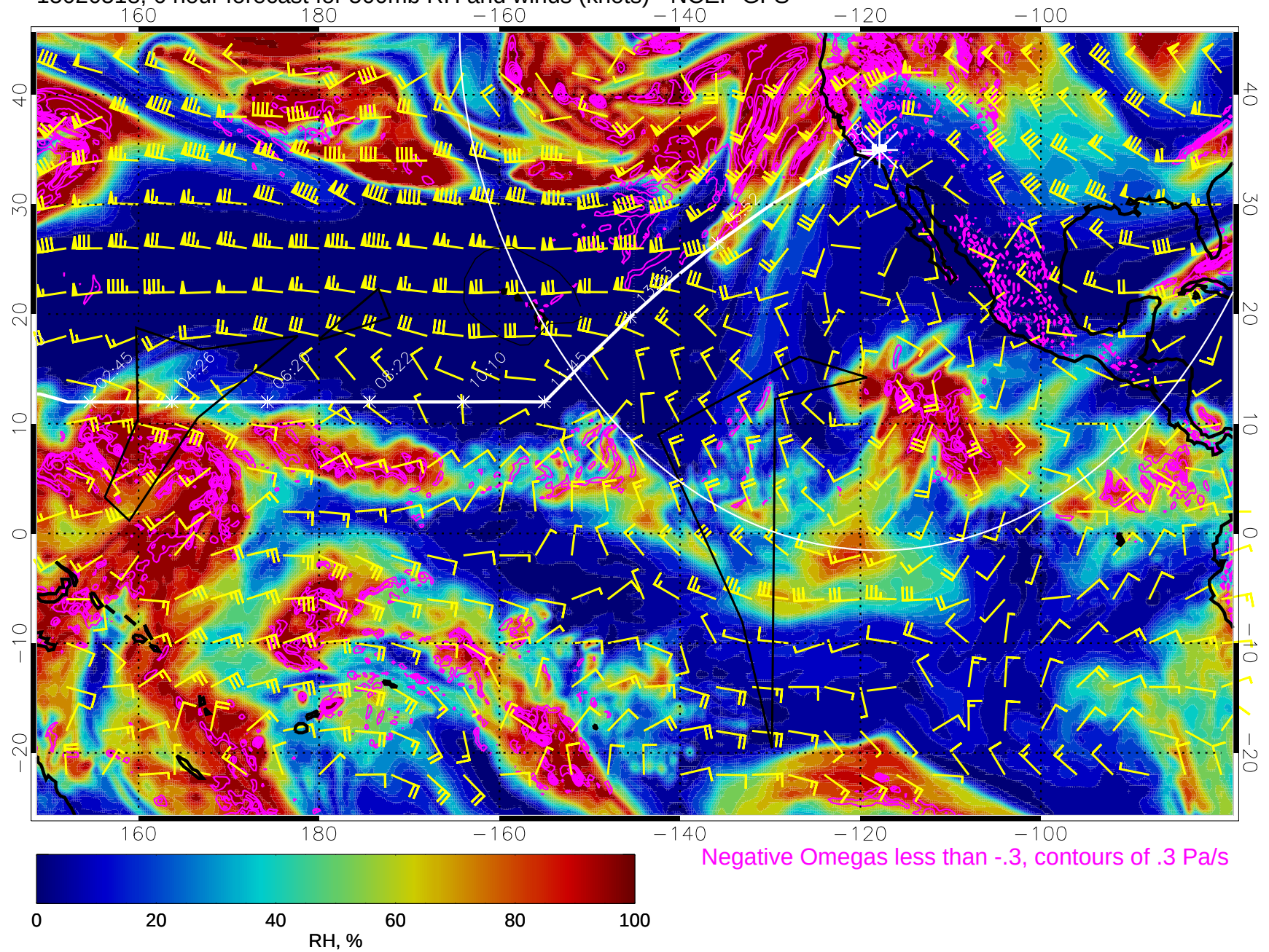
15020518, 6 hour forecast for 500mb RH and winds (knots) - NCEP GFS
