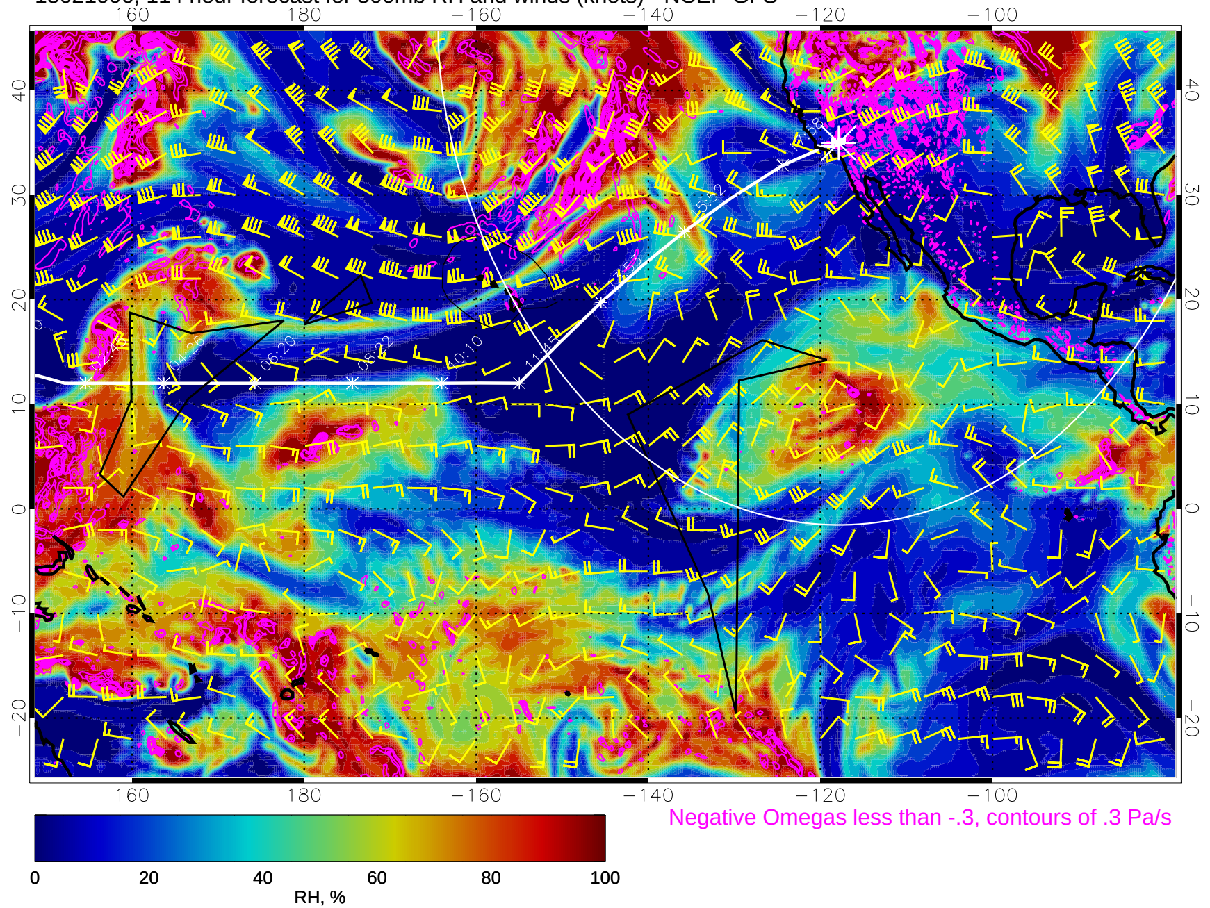
15021006, 114 hour forecast for 500mb RH and winds (knots) - NCEP GFS
