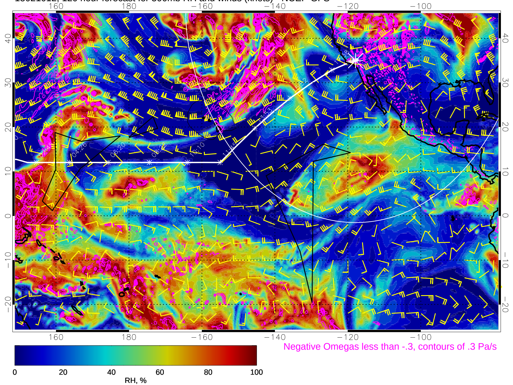
15021012, 120 hour forecast for 500mb RH and winds (knots) - NCEP GFS
