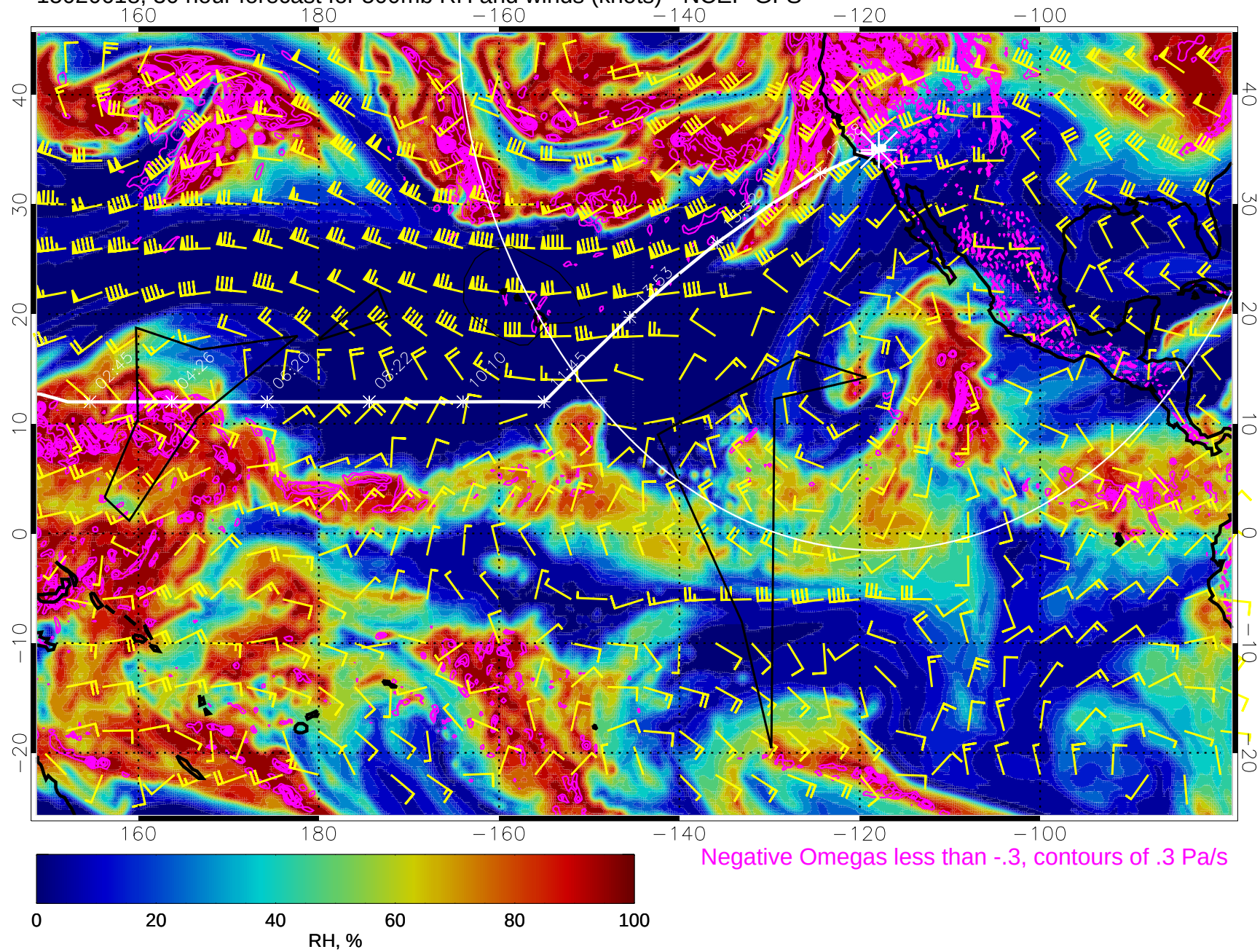
15020618, 30 hour forecast for 500mb RH and winds (knots) - NCEP GFS
