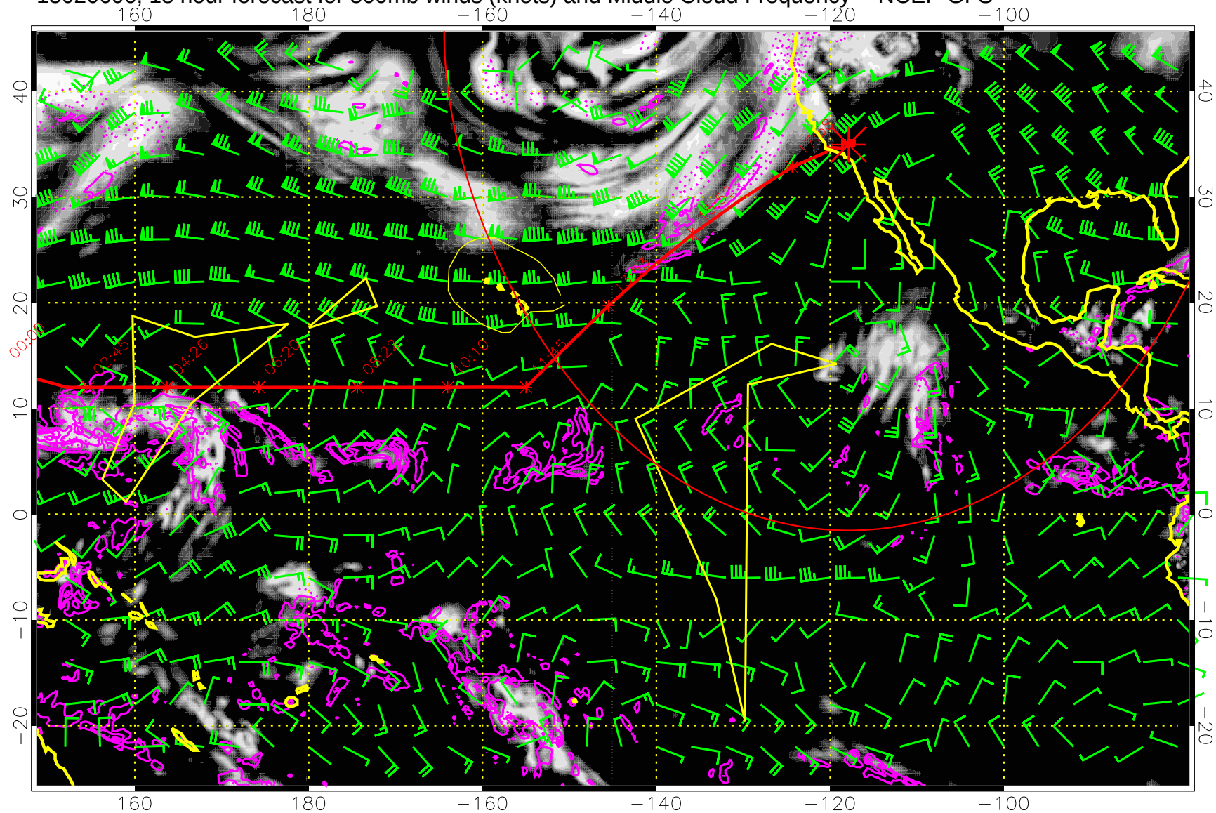
15020606, 18 hour forecast for 500mb winds (knots) and Middle Cloud Frequency -- NCEP GFS
