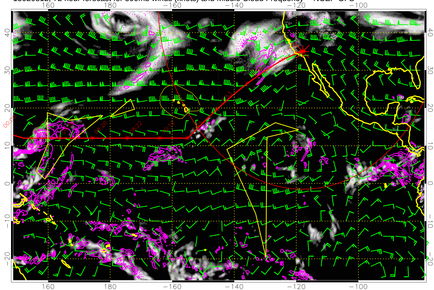
15020812, 72 hour forecast for 500mb winds (knots) and Middle Cloud Frequency -- NCEP GFS
