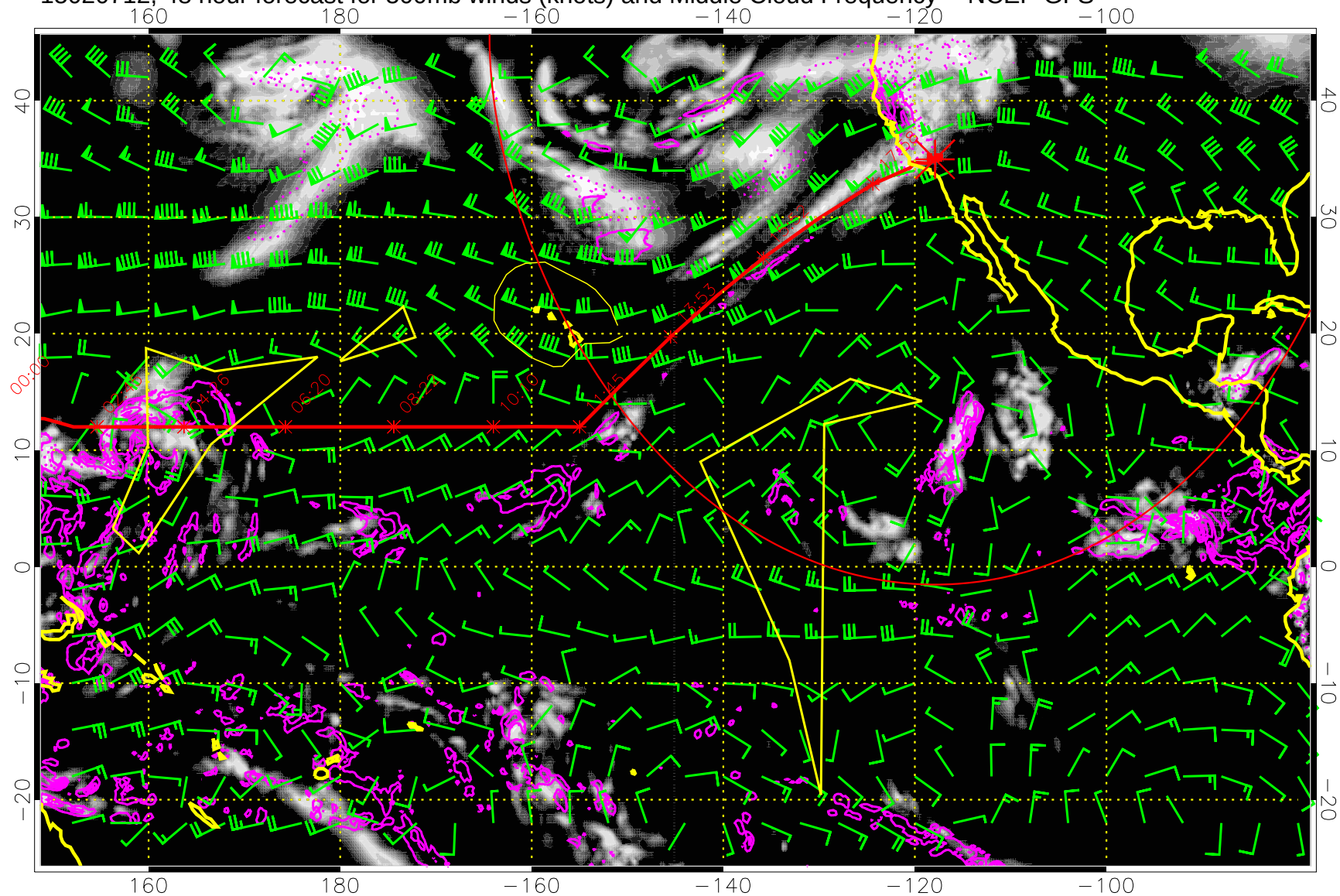
15020712, 48 hour forecast for 500mb winds (knots) and Middle Cloud Frequency -- NCEP GFS
