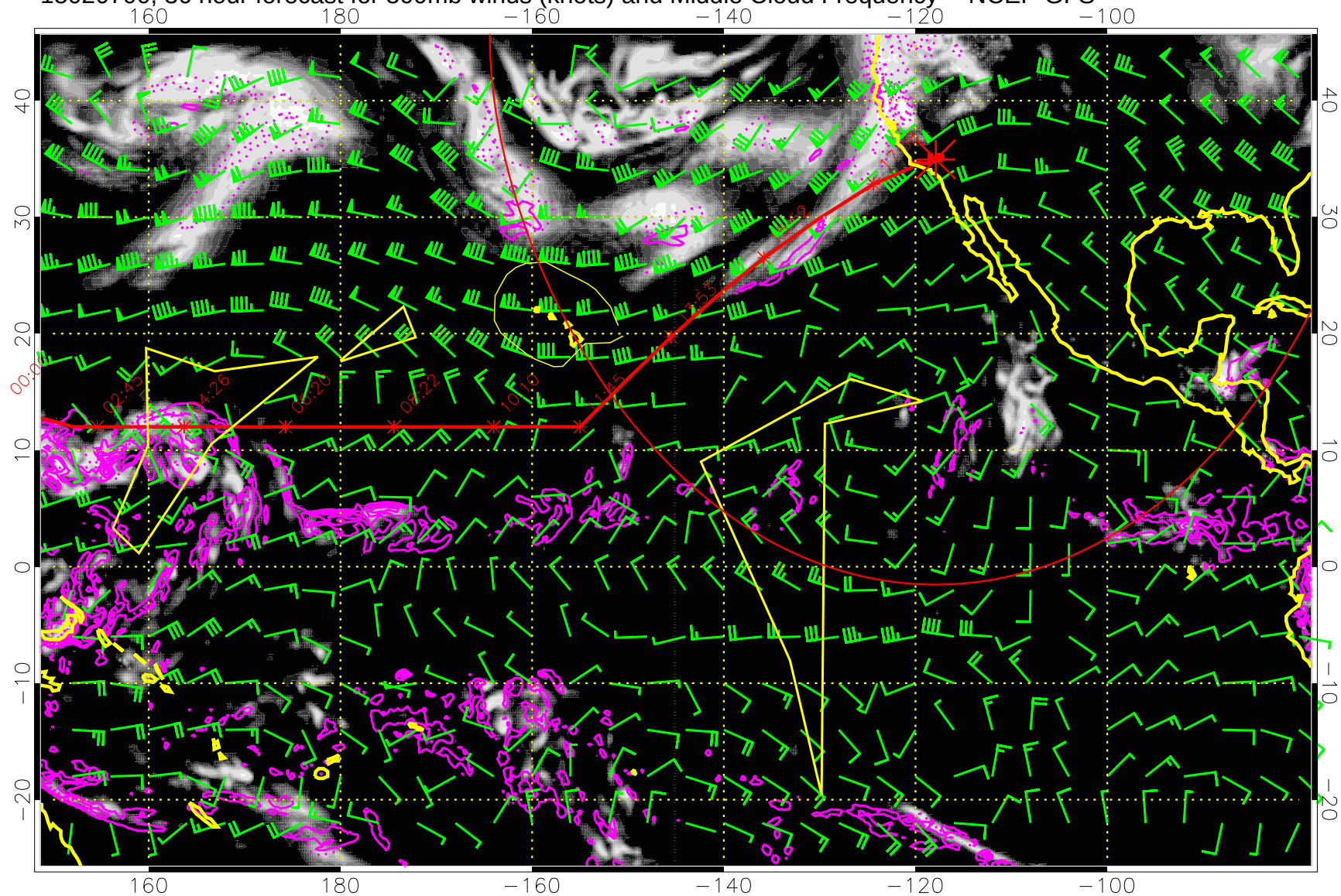
15020700, 36 hour forecast for 500mb winds (knots) and Middle Cloud Frequency -- NCEP GFS
