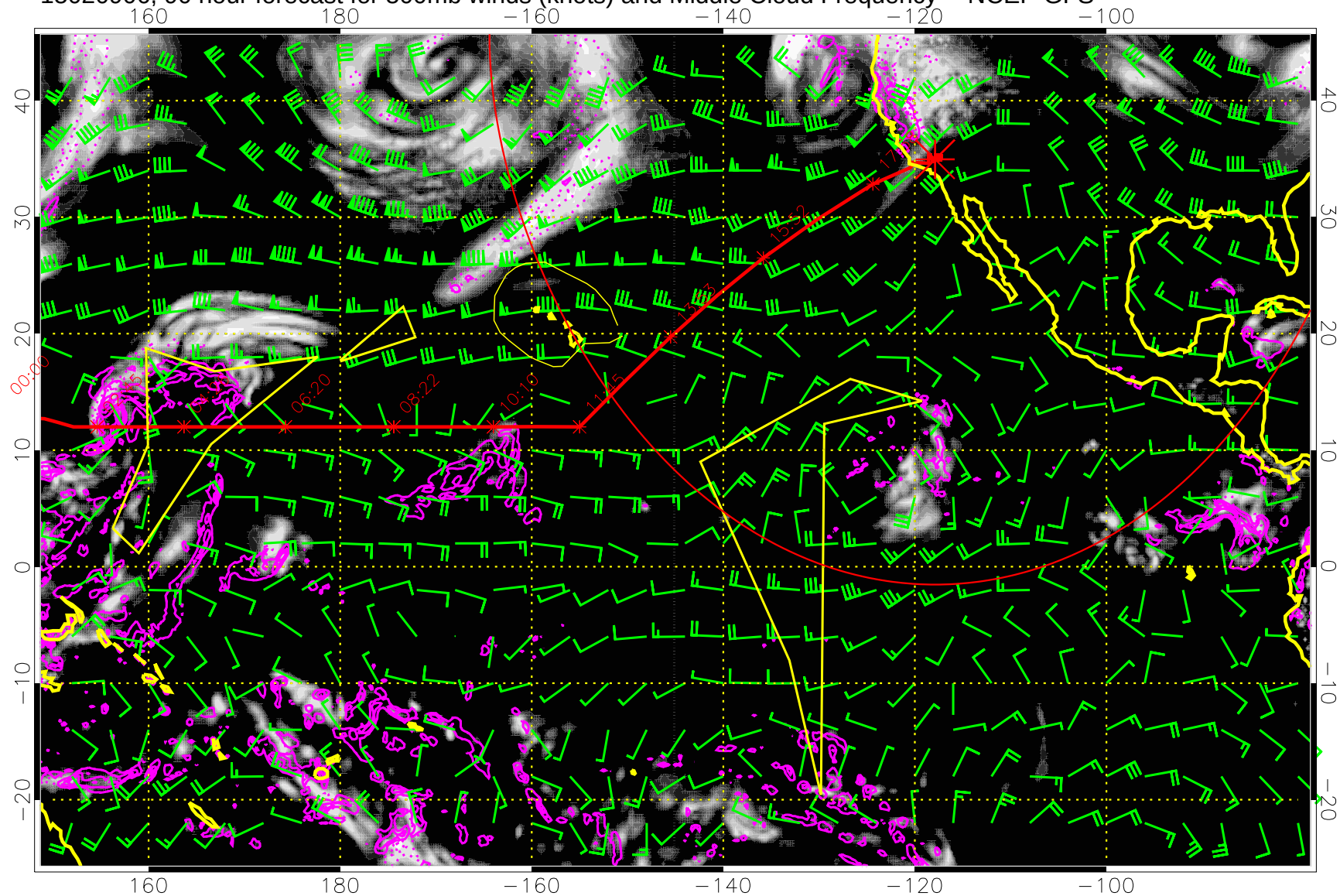
15020906, 90 hour forecast for 500mb winds (knots) and Middle Cloud Frequency -- NCEP GFS
