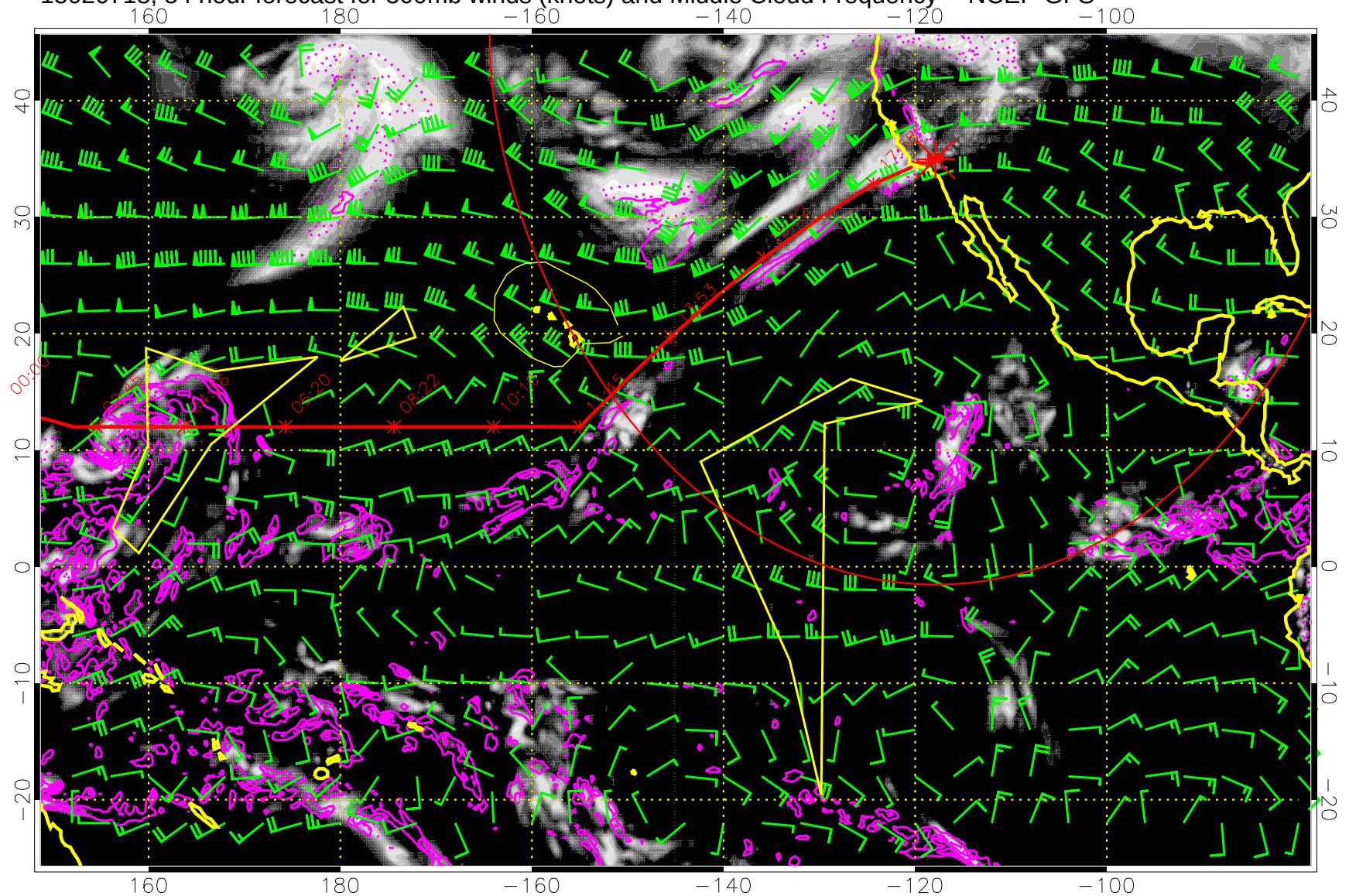
15020718, 54 hour forecast for 500mb winds (knots) and Middle Cloud Frequency -- NCEP GFS
