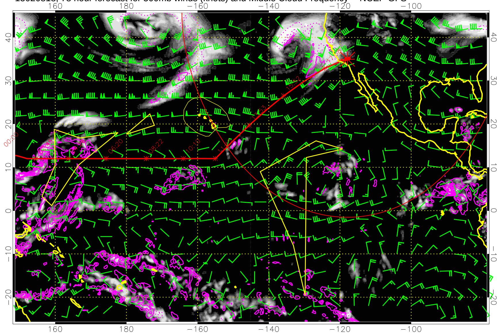
15020818, 78 hour forecast for 500mb winds (knots) and Middle Cloud Frequency -- NCEP GFS
