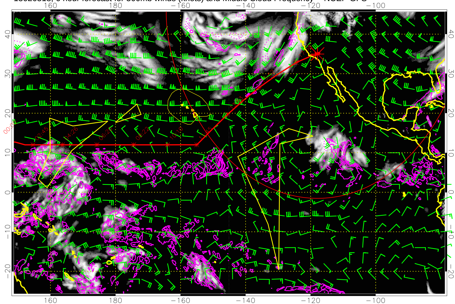
15020518, 6 hour forecast for 500mb winds (knots) and Middle Cloud Frequency -- NCEP GFS
