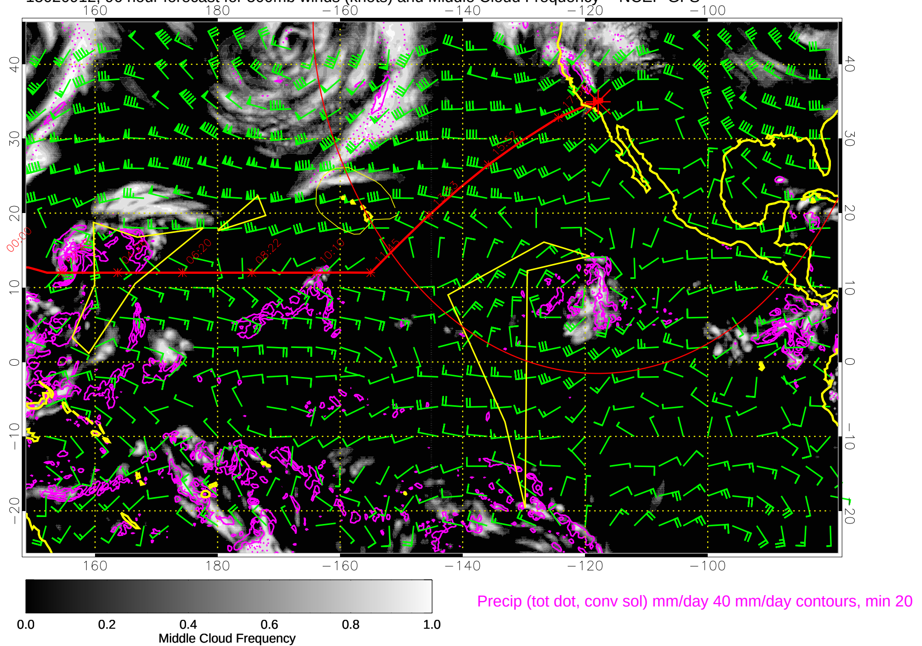
15020912, 96 hour forecast for 500mb winds (knots) and Middle Cloud Frequency -- NCEP GFS
