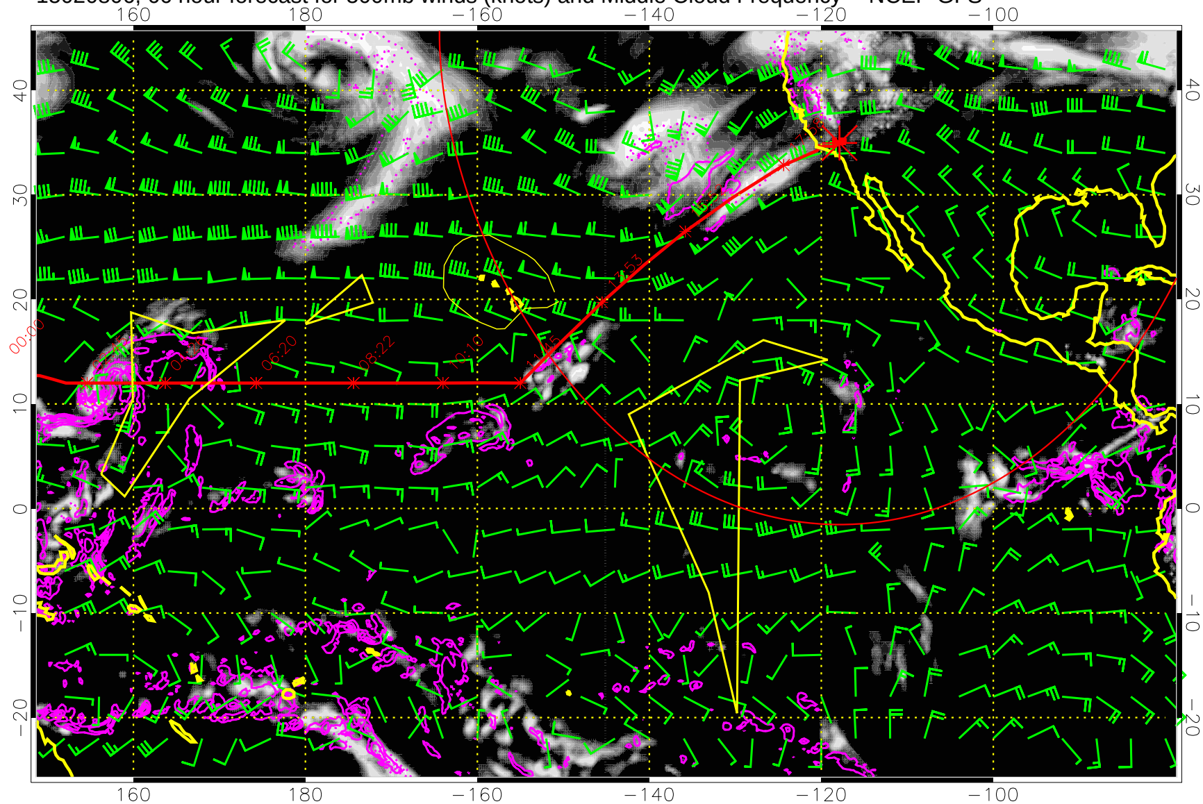
15020806, 66 hour forecast for 500mb winds (knots) and Middle Cloud Frequency -- NCEP GFS
