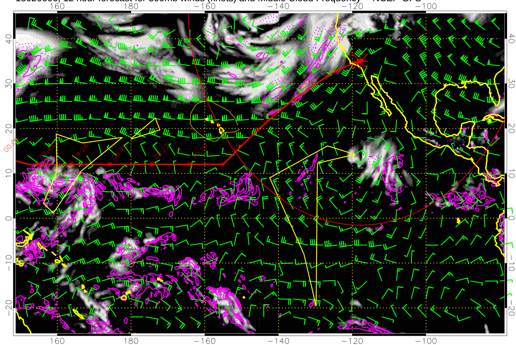
15020600, 12 hour forecast for 500mb winds (knots) and Middle Cloud Frequency -- NCEP GFS
