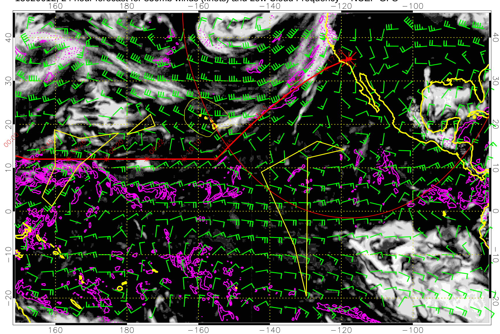
15020612, 24 hour forecast for 850mb winds (knots) and Low Cloud Frequency -- NCEP GFS
