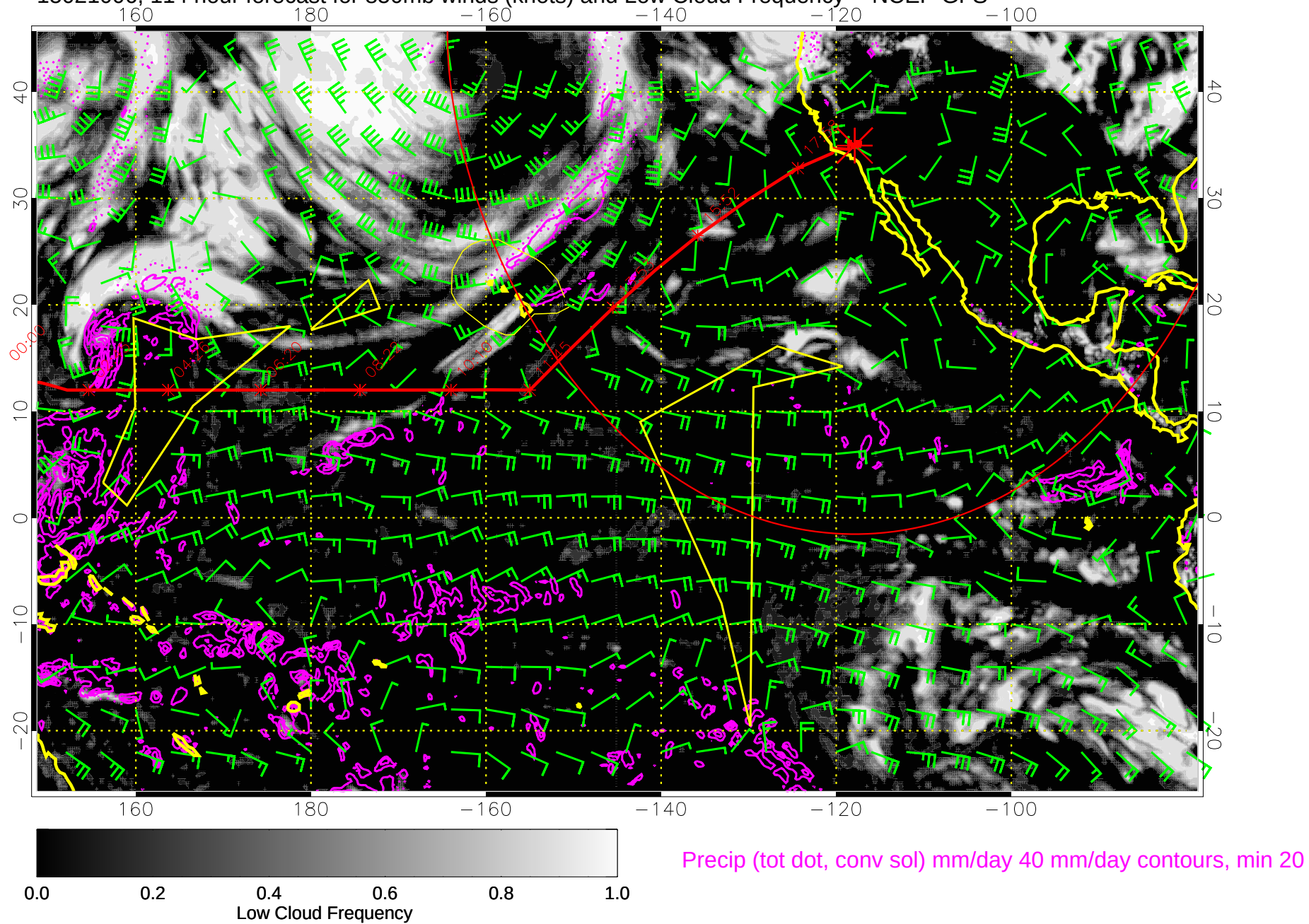
15021006, 114 hour forecast for 850mb winds (knots) and Low Cloud Frequency -- NCEP GFS
