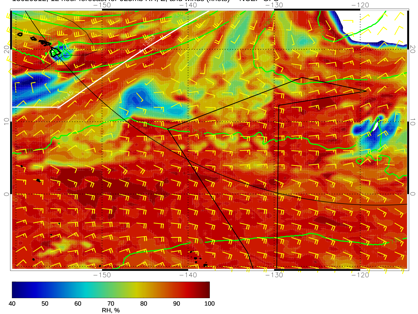
15020512, 12 hour forecast for 925mb RH, Z, and winds (knots) -- NCEP GFS
