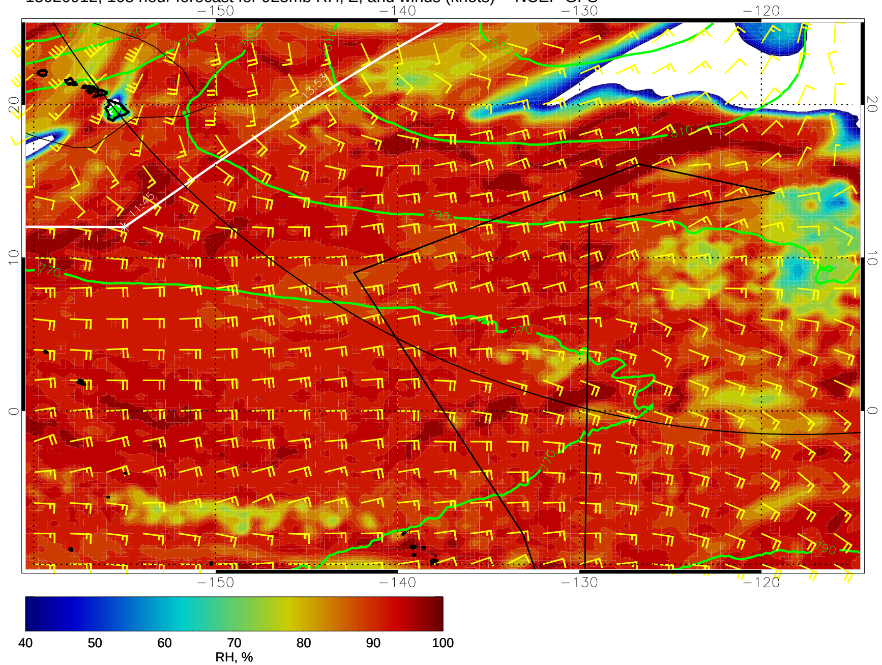
15020912, 108 hour forecast for 925mb RH, Z, and winds (knots) -- NCEP GFS
