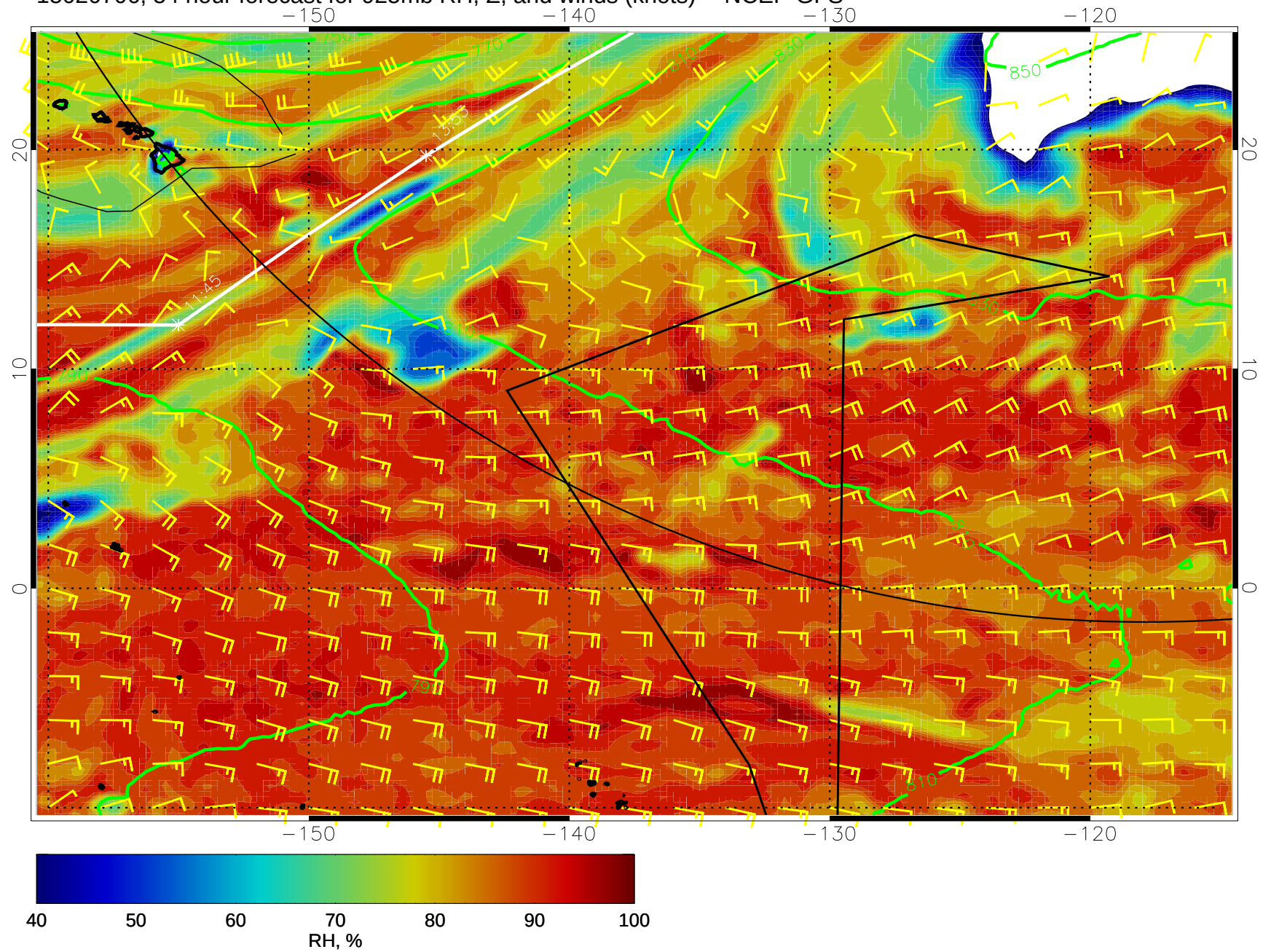
15020706, 54 hour forecast for 925mb RH, Z, and winds (knots) -- NCEP GFS
