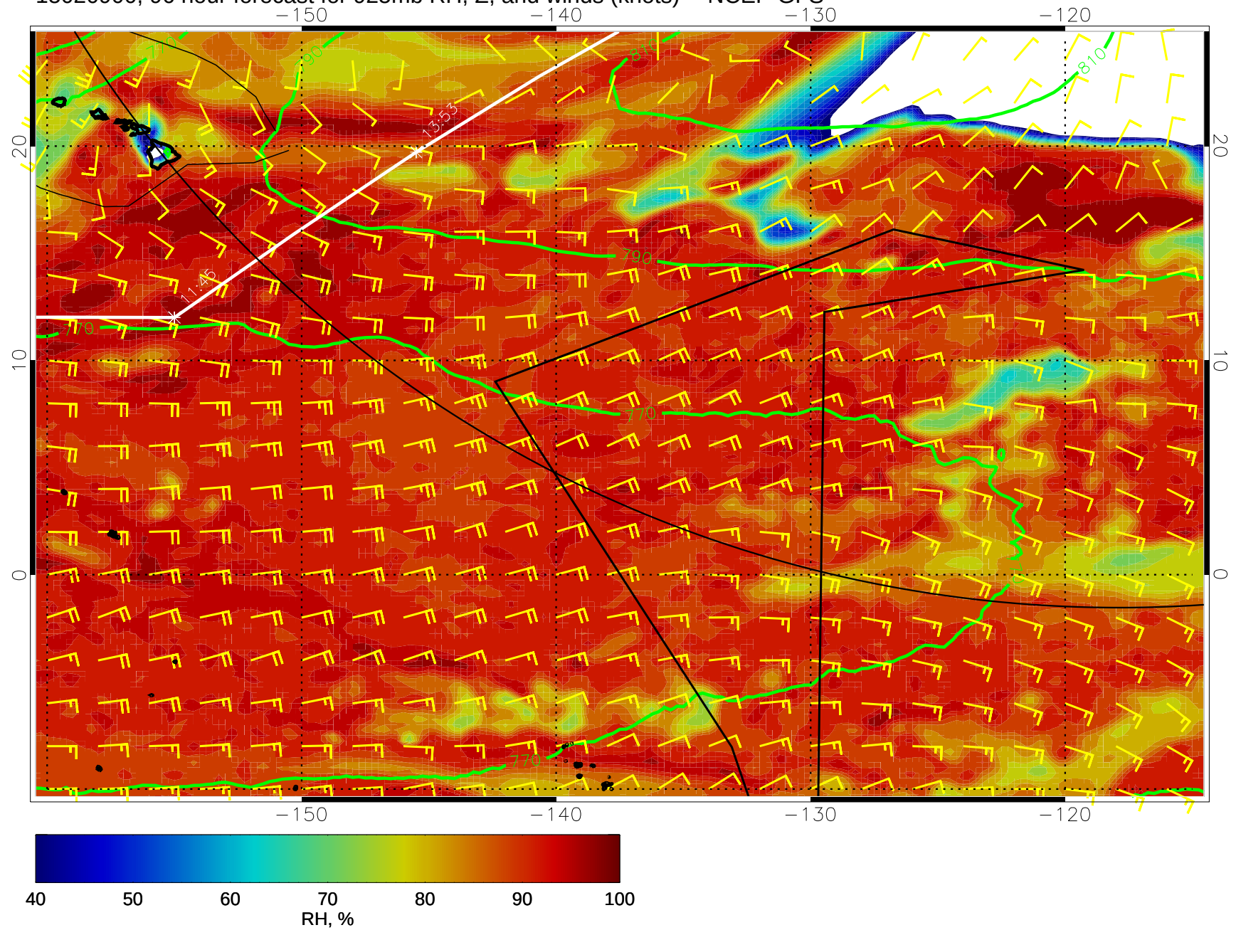
15020900, 96 hour forecast for 925mb RH, Z, and winds (knots) -- NCEP GFS
