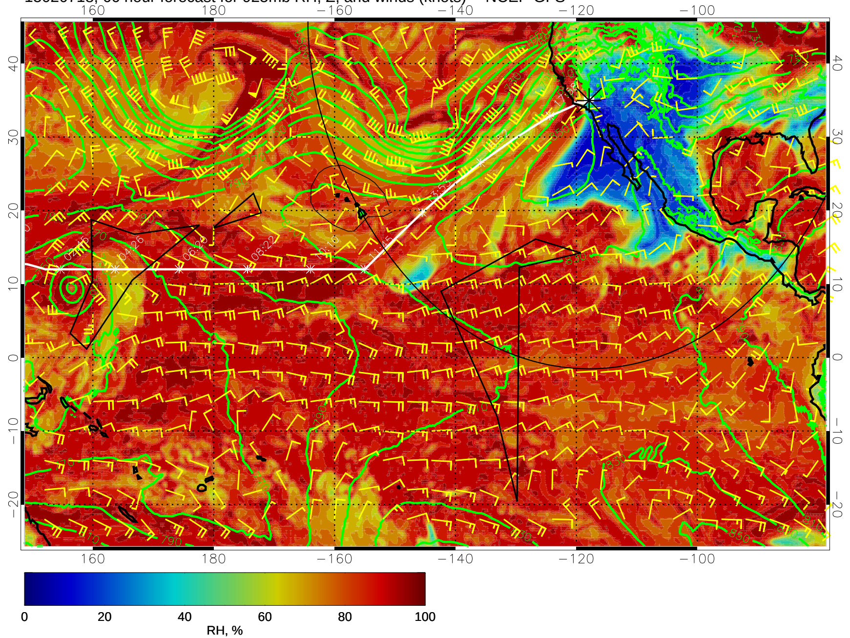
15020718, 66 hour forecast for 925mb RH, Z, and winds (knots) -- NCEP GFS
