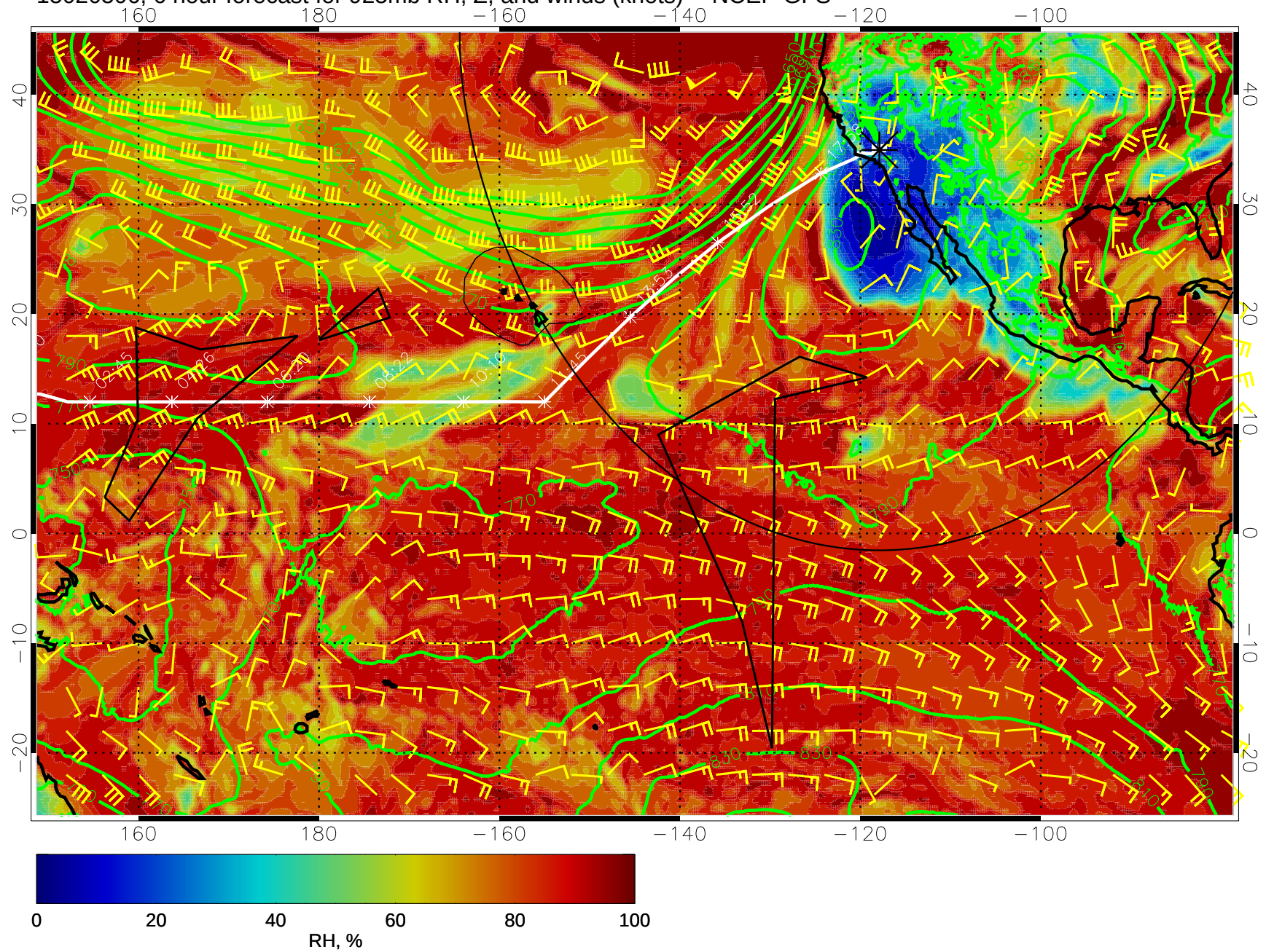
15020506, 6 hour forecast for 925mb RH, Z, and winds (knots) -- NCEP GFS
