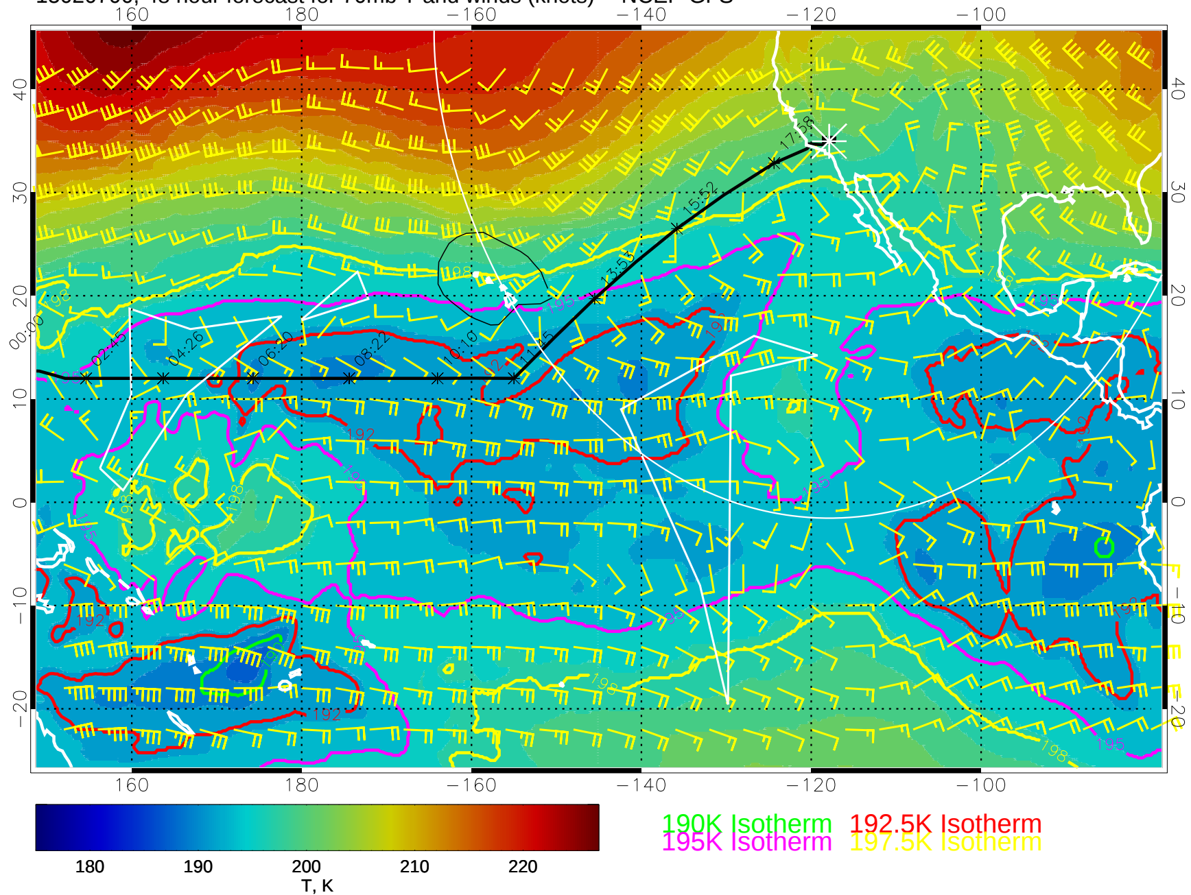
15020700, 48 hour forecast for 70mb T and winds (knots) -- NCEP GFS
