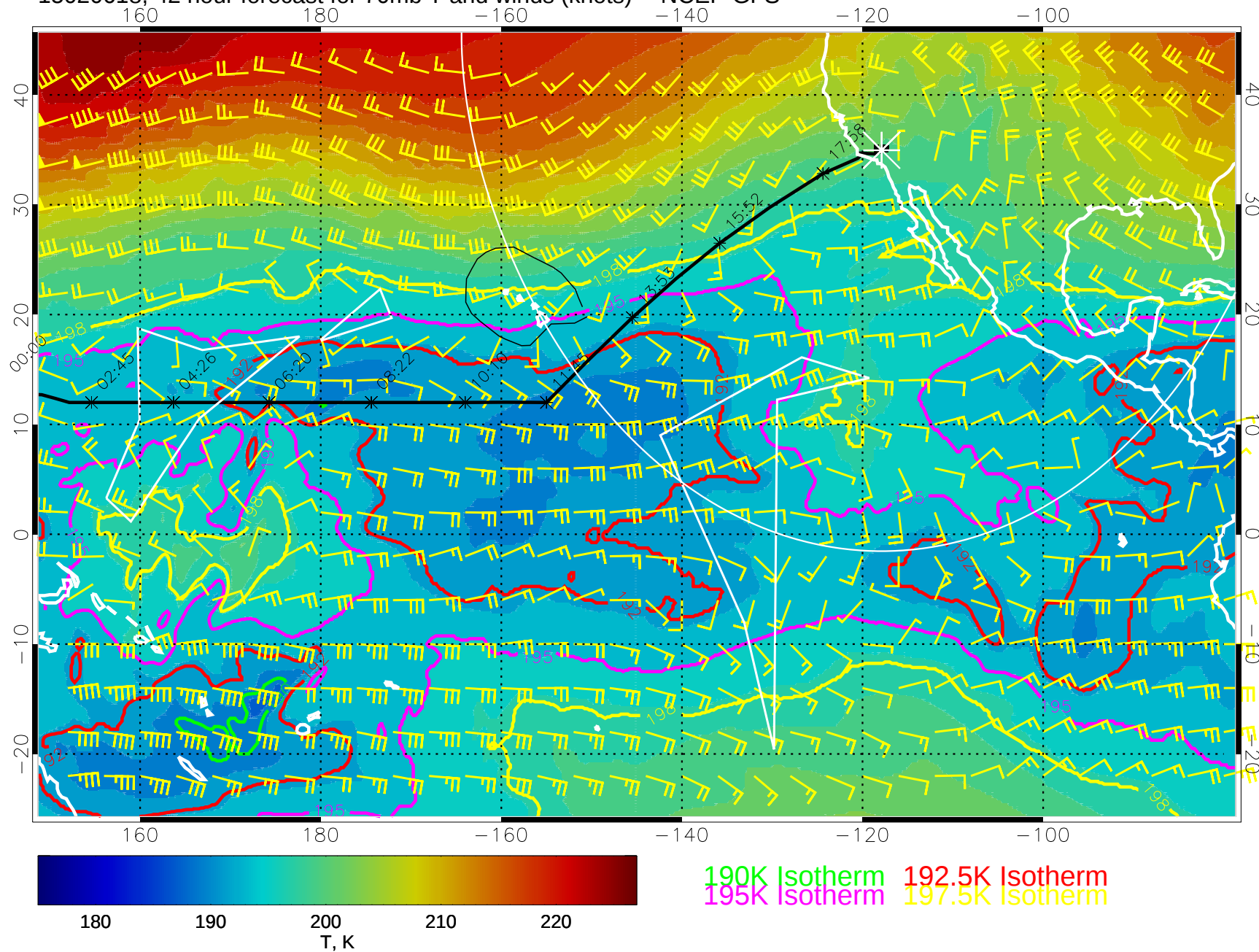
15020618, 42 hour forecast for 70mb T and winds (knots) -- NCEP GFS
