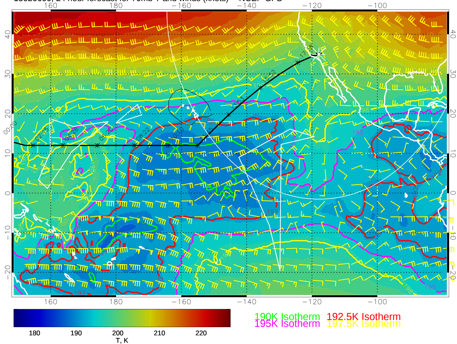
15020600, 24 hour forecast for 70mb T and winds (knots) -- NCEP GFS
