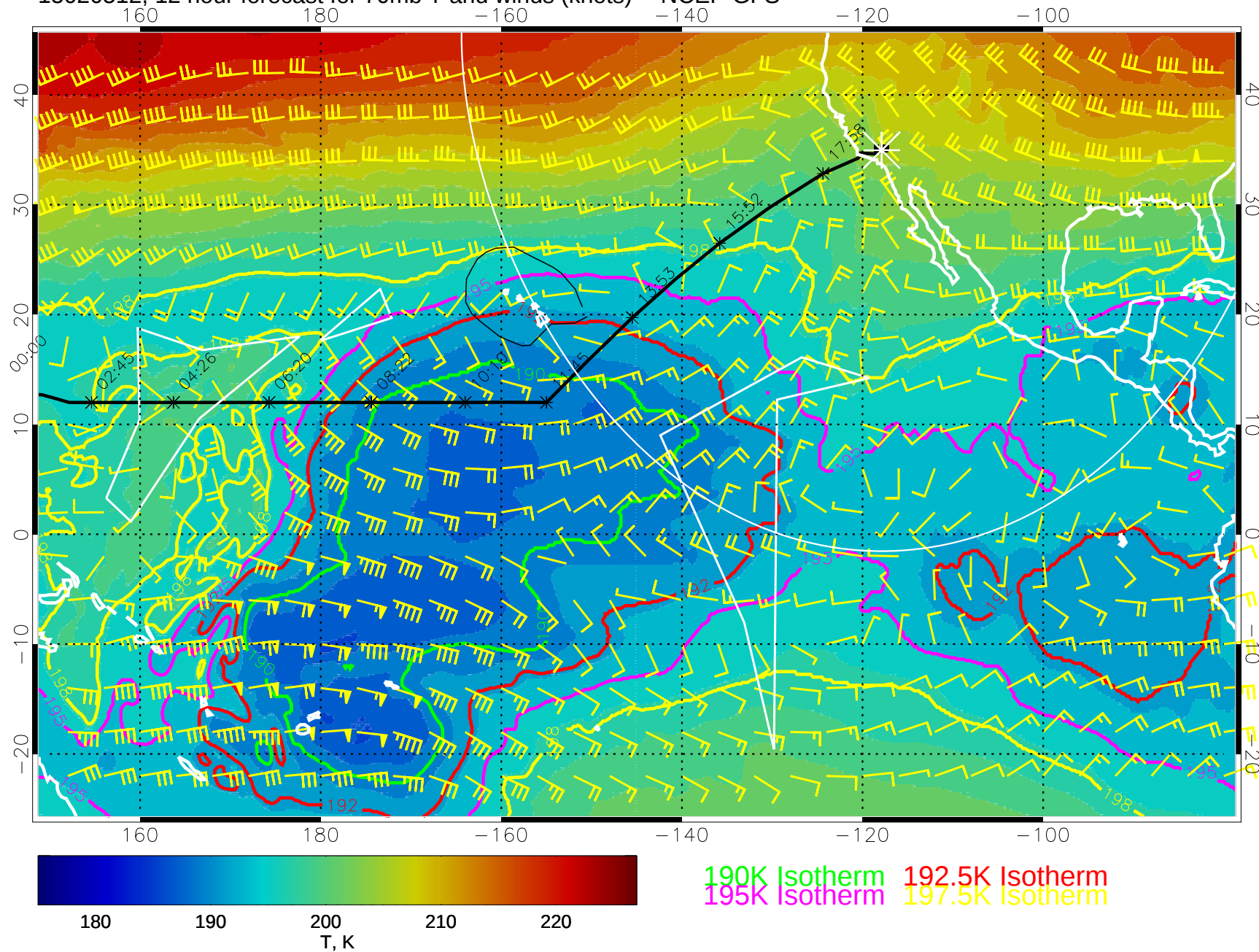
15020512, 12 hour forecast for 70mb T and winds (knots) -- NCEP GFS
