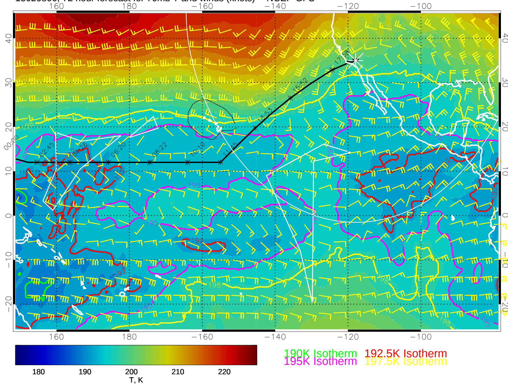
15020800, 72 hour forecast for 70mb T and winds (knots) -- NCEP GFS
