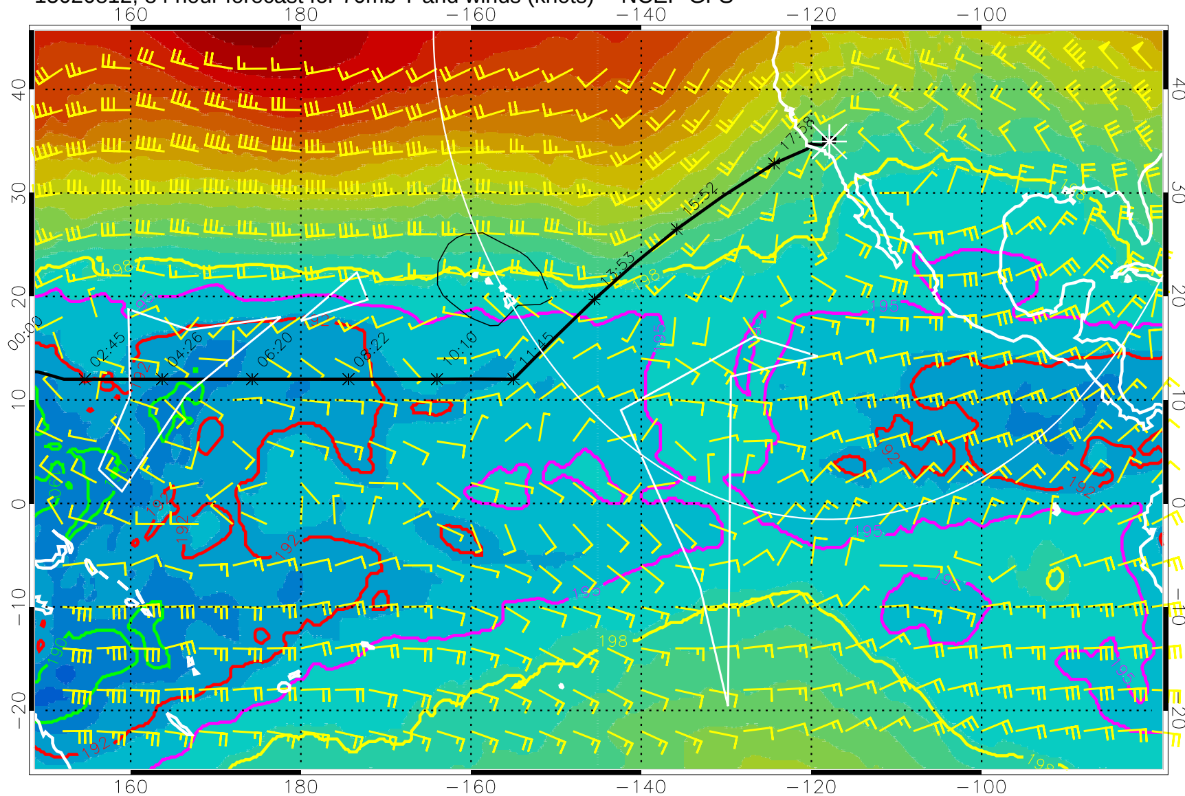
15020812, 84 hour forecast for 70mb T and winds (knots) -- NCEP GFS
