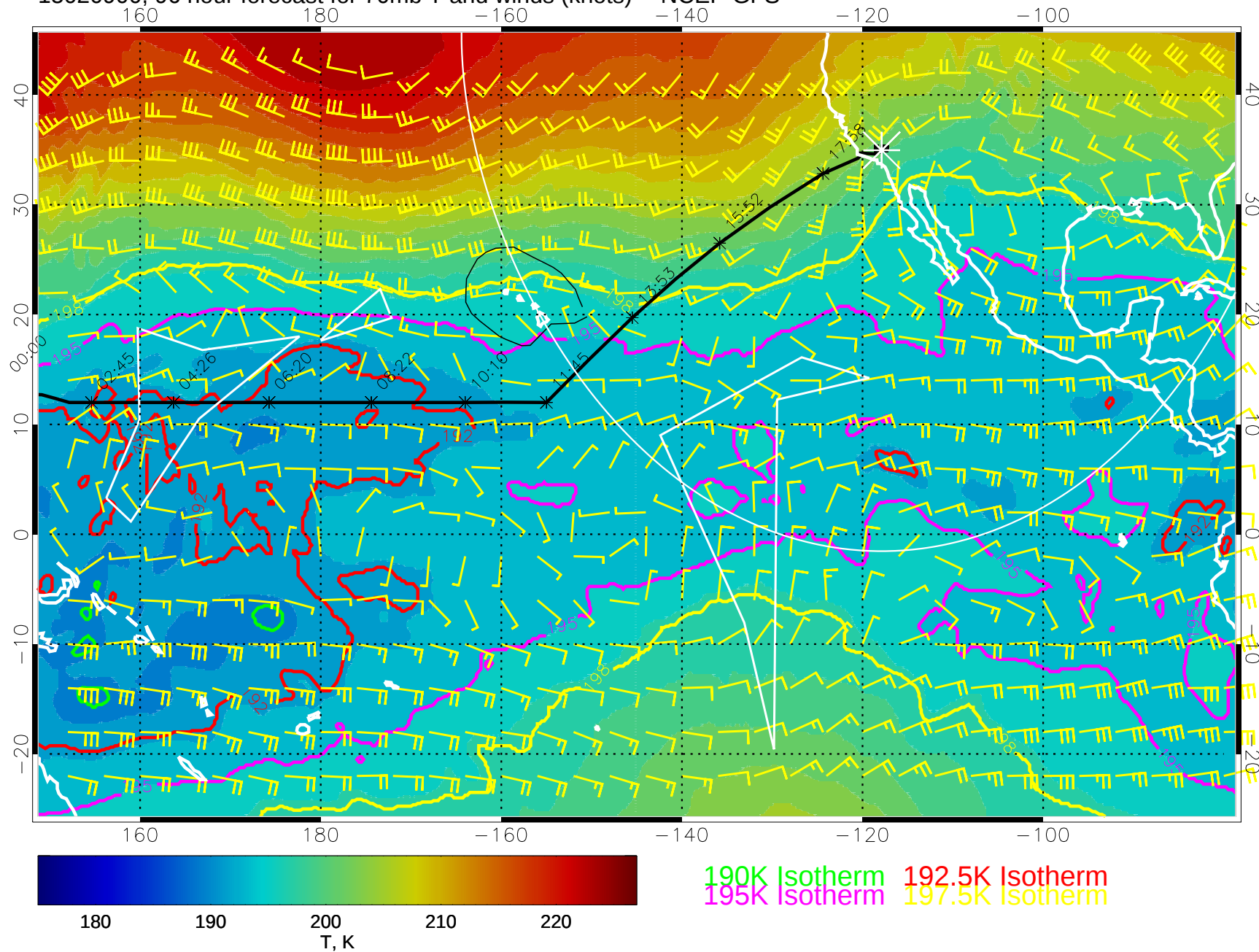
15020900, 96 hour forecast for 70mb T and winds (knots) -- NCEP GFS
