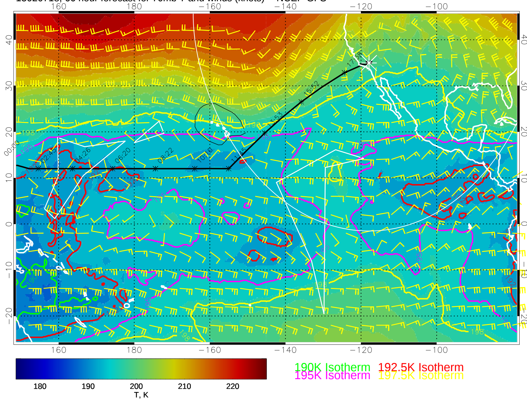
15020718, 66 hour forecast for 70mb T and winds (knots) -- NCEP GFS
