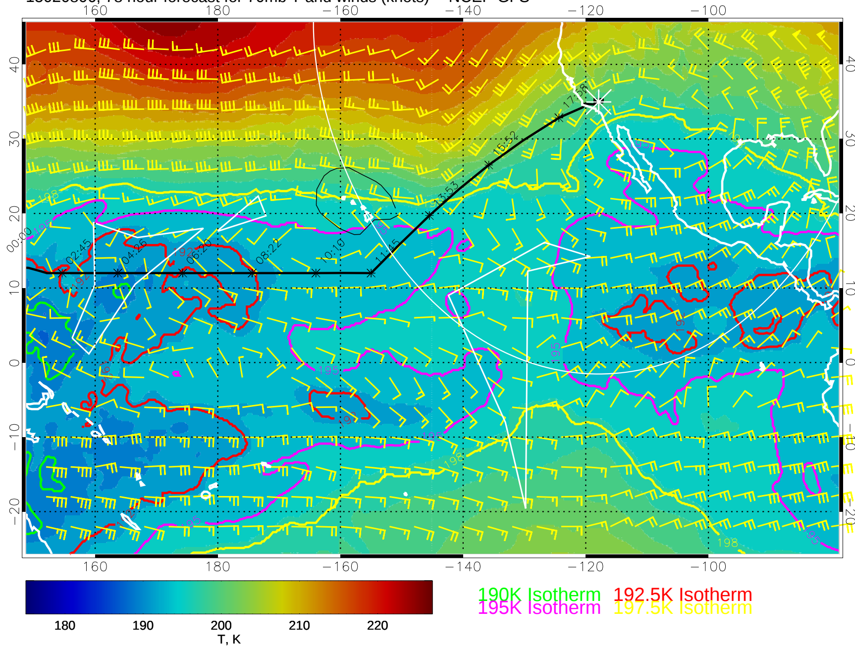
15020806, 78 hour forecast for 70mb T and winds (knots) -- NCEP GFS
