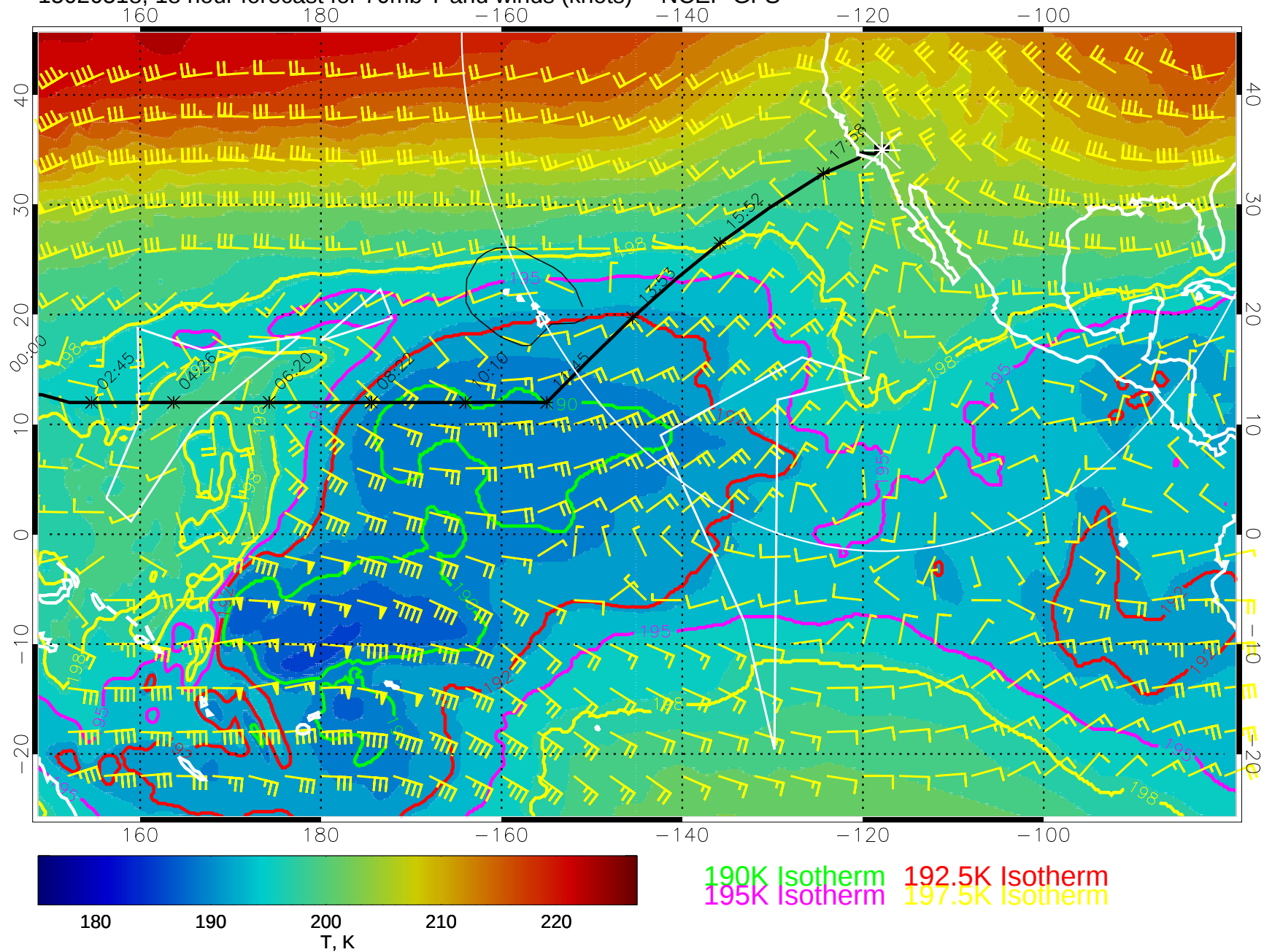
15020518, 18 hour forecast for 70mb T and winds (knots) -- NCEP GFS
