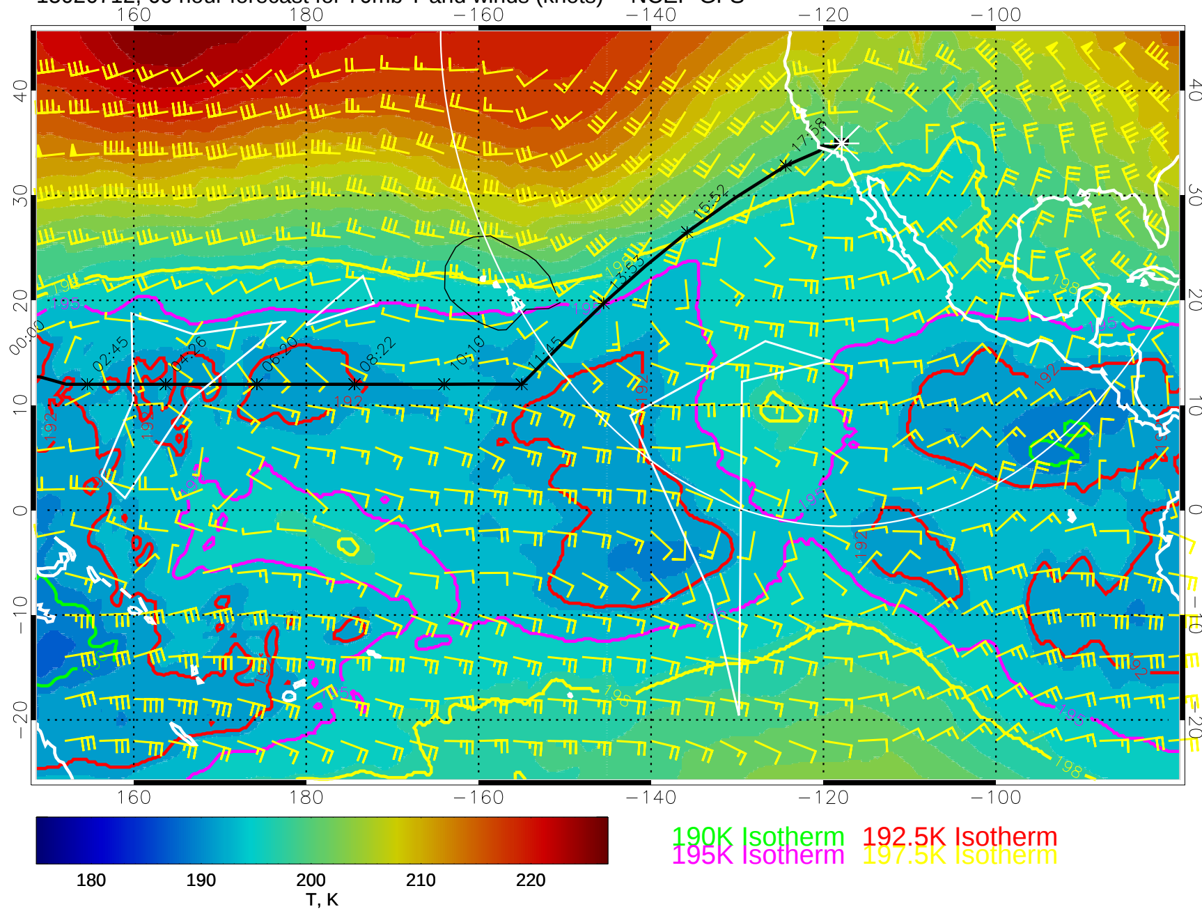
15020712, 60 hour forecast for 70mb T and winds (knots) -- NCEP GFS
