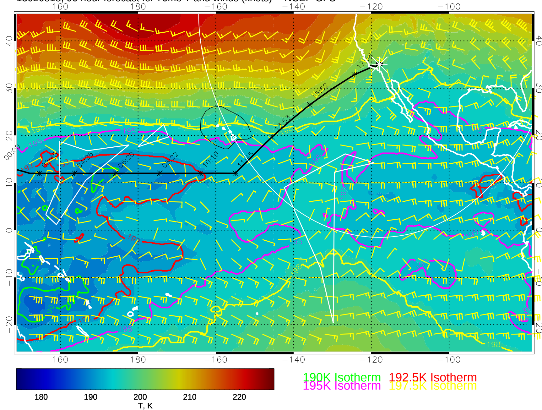
15020818, 90 hour forecast for 70mb T and winds (knots) -- NCEP GFS
