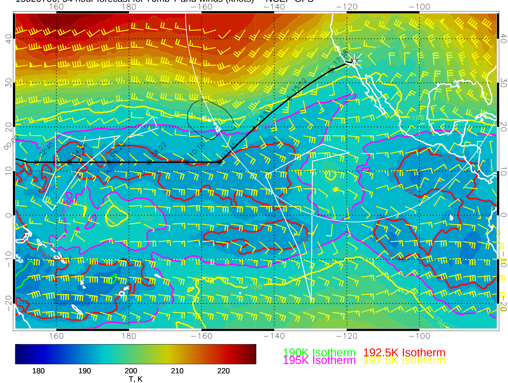
15020706, 54 hour forecast for 70mb T and winds (knots) -- NCEP GFS
