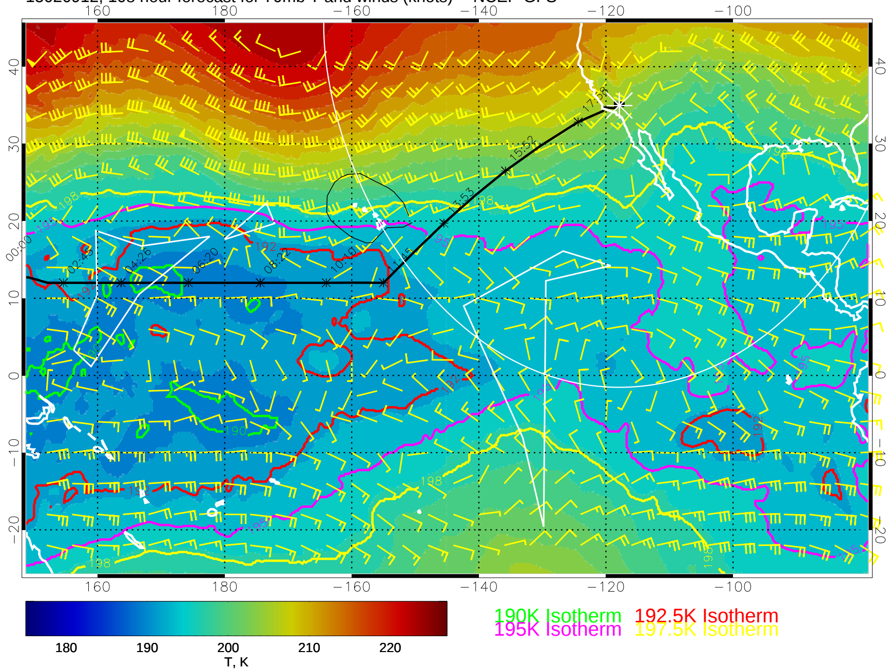
15020912, 108 hour forecast for 70mb T and winds (knots) -- NCEP GFS
