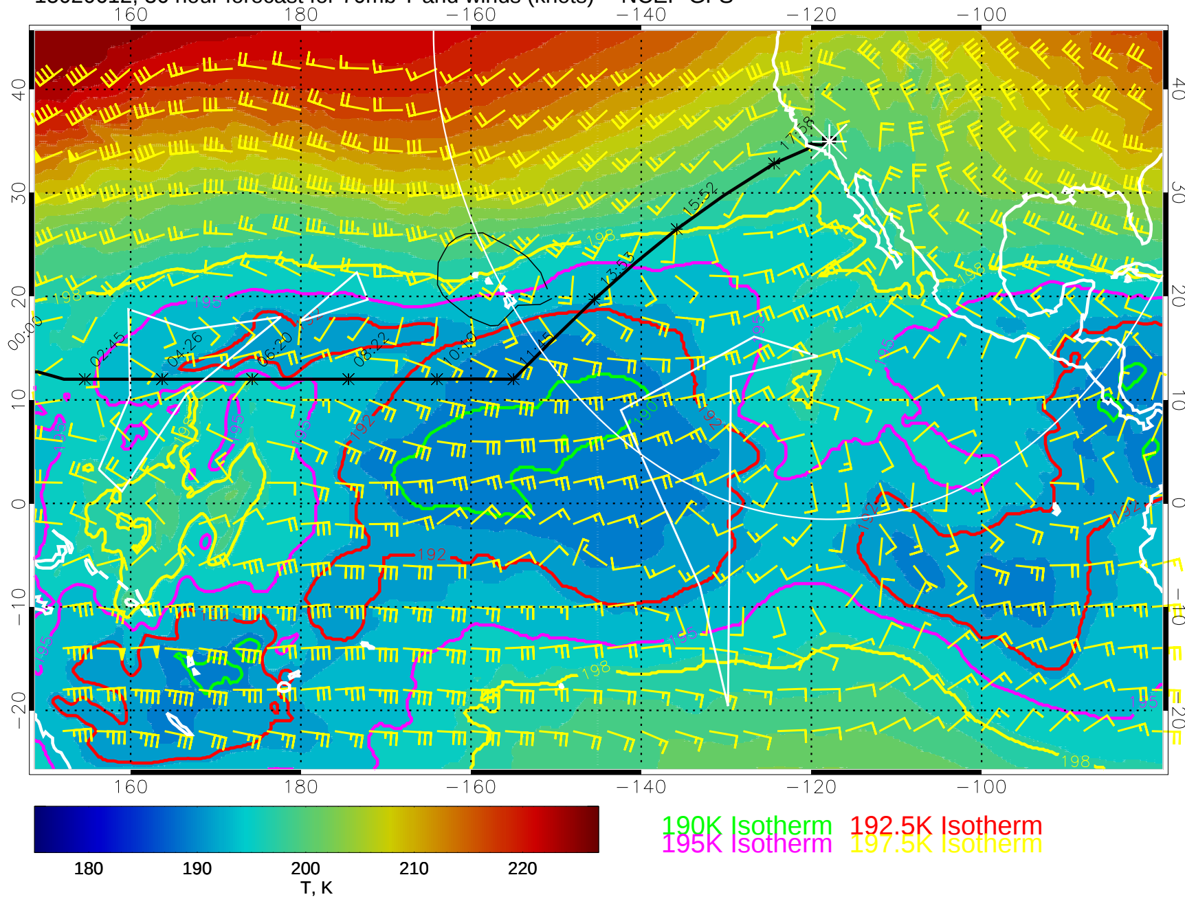
15020612, 36 hour forecast for 70mb T and winds (knots) -- NCEP GFS
