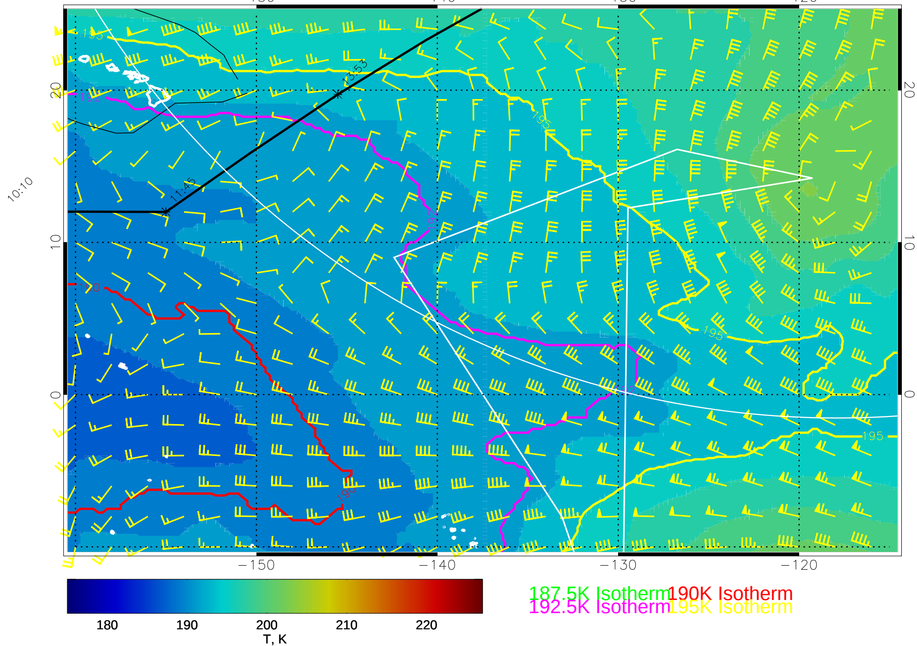
15020600, 24 hour forecast for 100mb T and winds (knots) -- NCEP GFS
