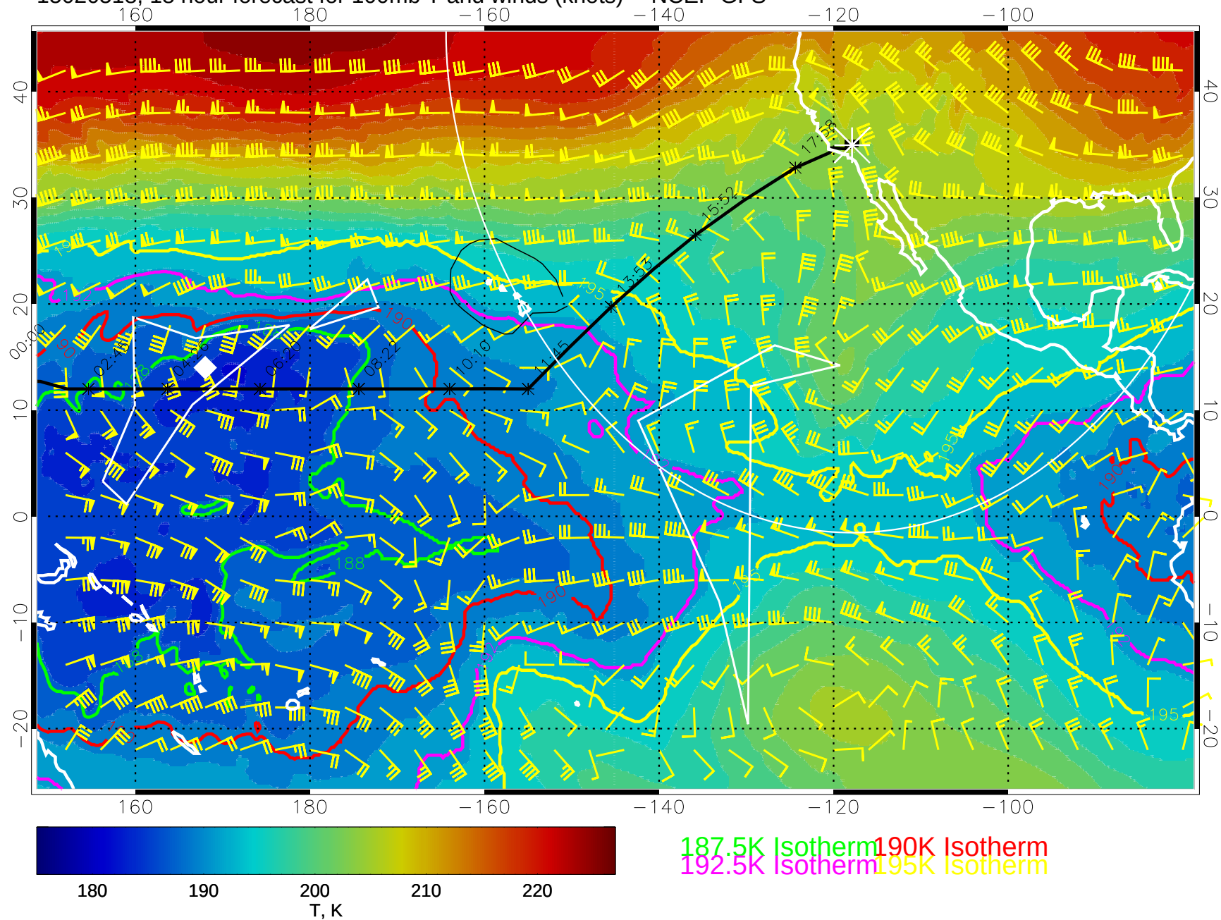
15020518, 18 hour forecast for 100mb T and winds (knots) -- NCEP GFS
