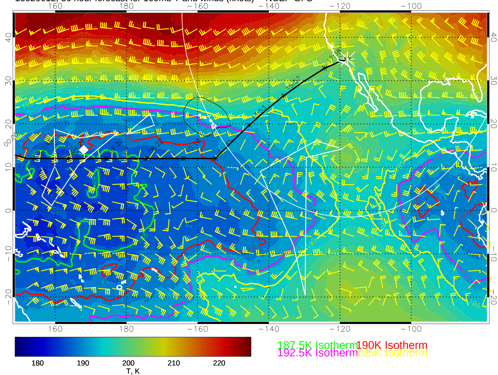
15020612, 36 hour forecast for 100mb T and winds (knots) -- NCEP GFS
