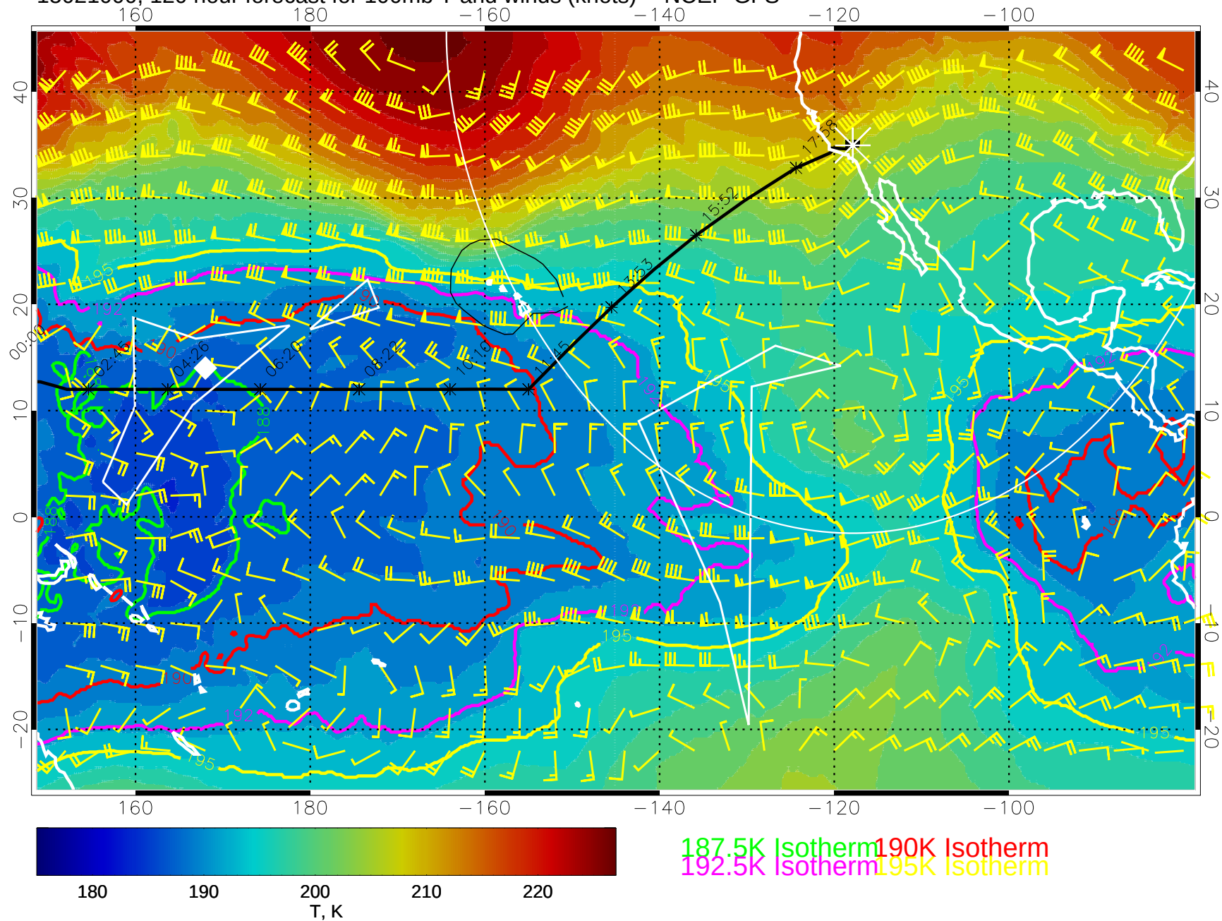
15021000, 120 hour forecast for 100mb T and winds (knots) -- NCEP GFS
