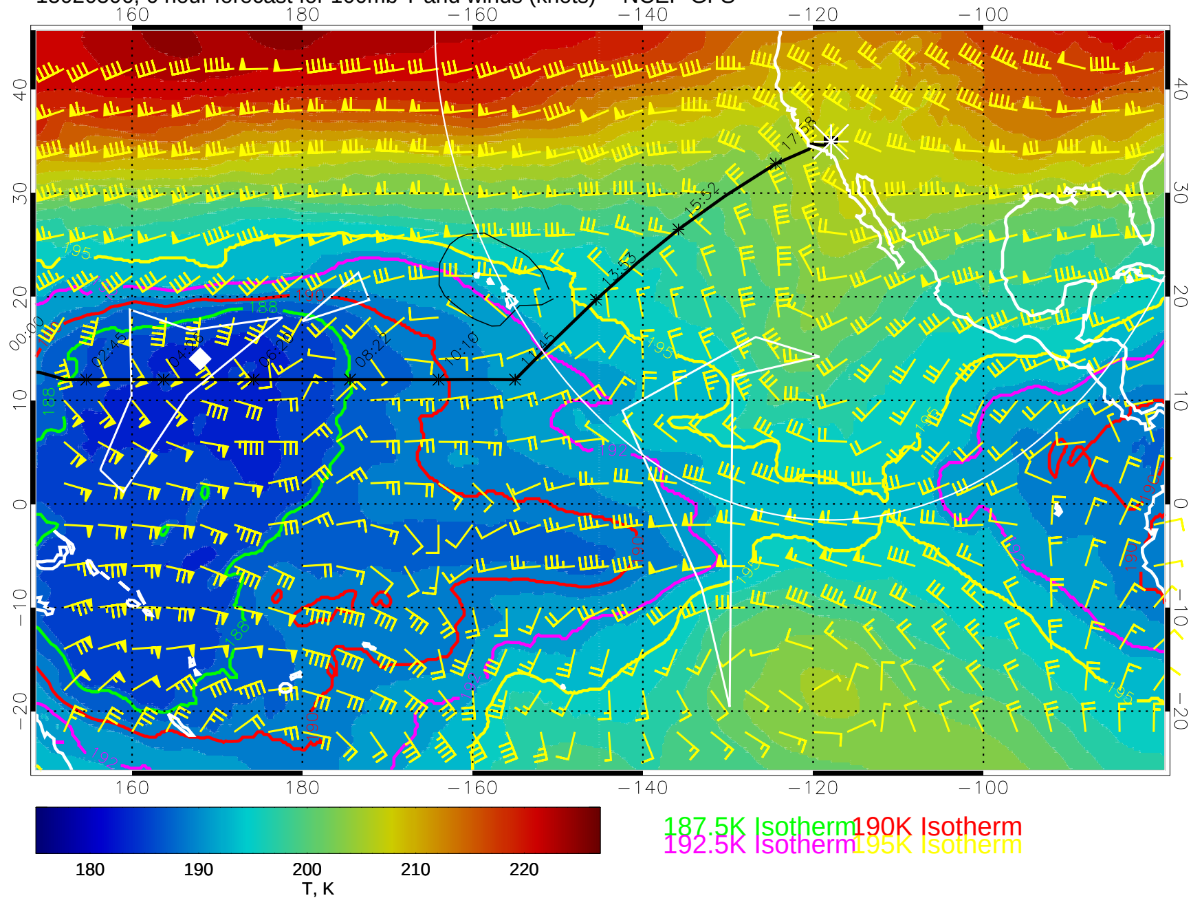
15020506, 6 hour forecast for 100mb T and winds (knots) -- NCEP GFS
