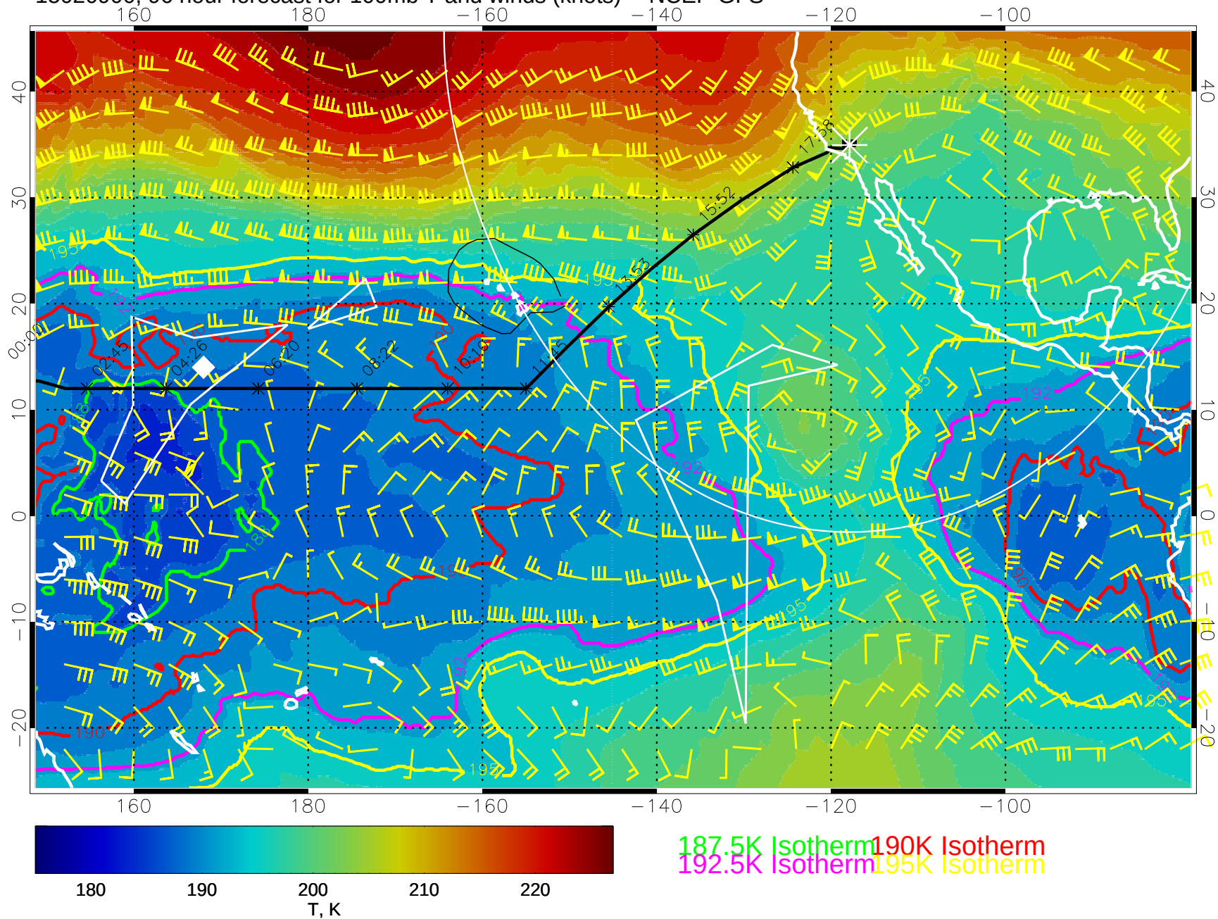
15020900, 96 hour forecast for 100mb T and winds (knots) -- NCEP GFS
