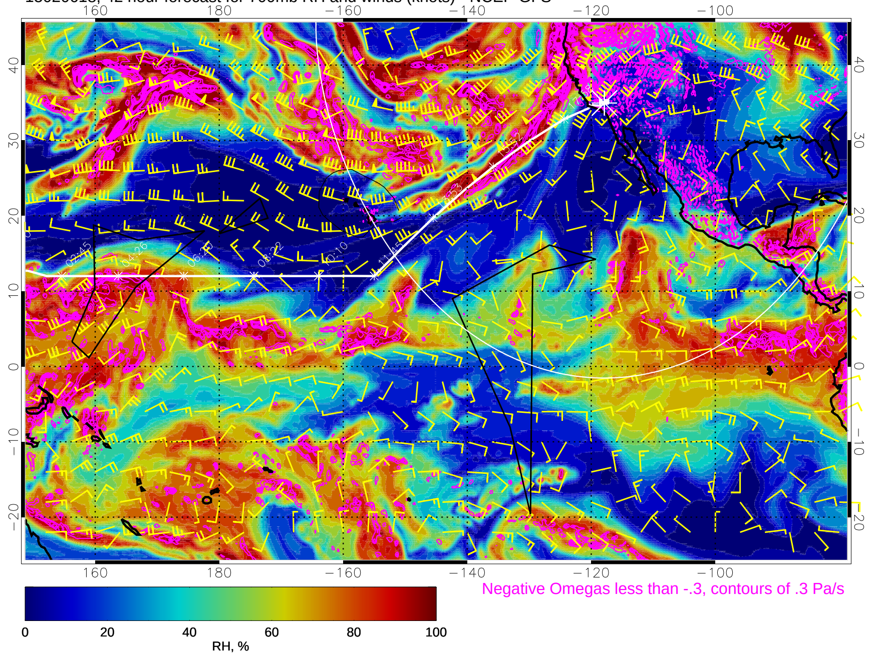
15020618, 42 hour forecast for 700mb RH and winds (knots) - NCEP GFS
