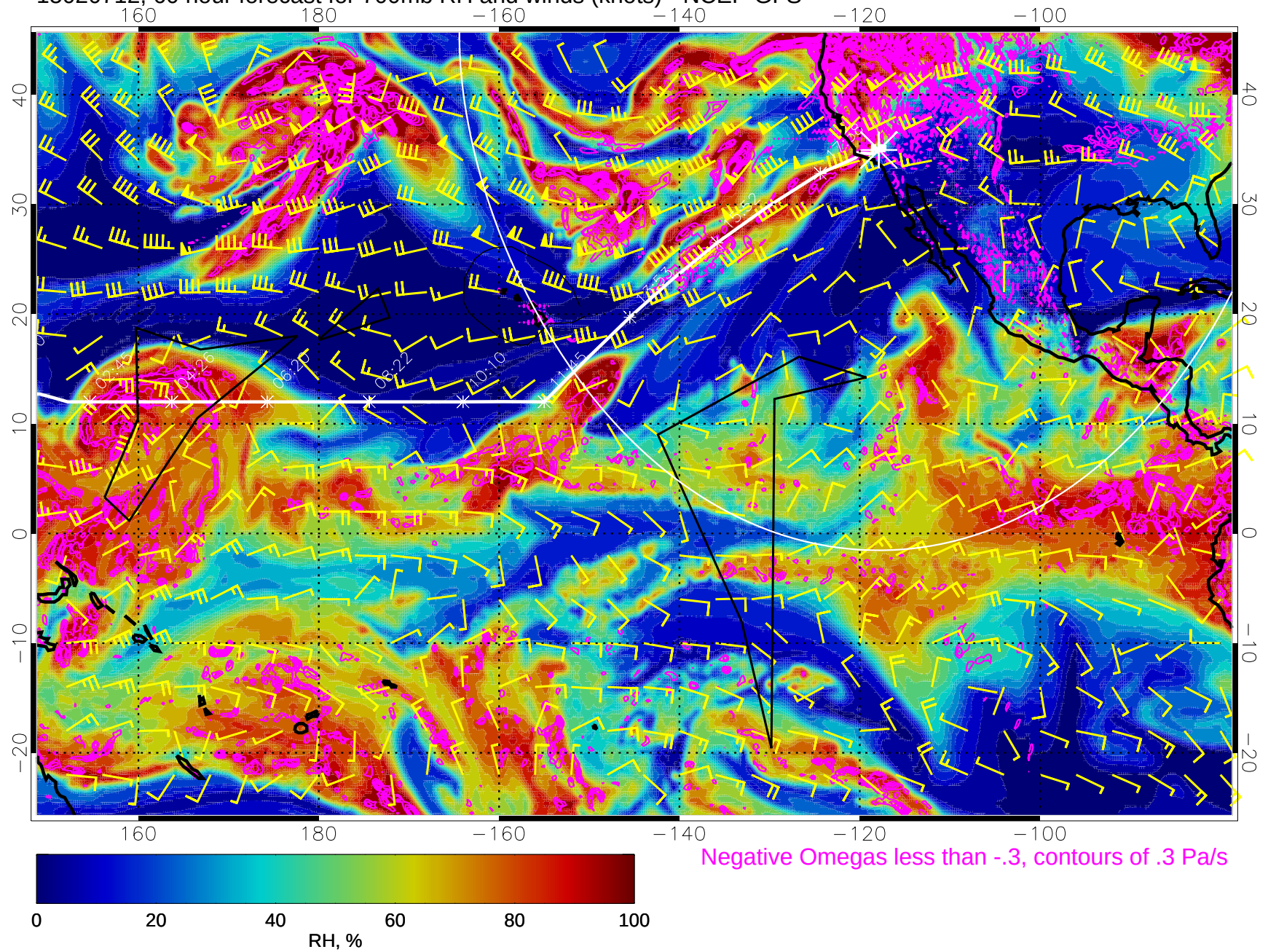
15020712, 60 hour forecast for 700mb RH and winds (knots) - NCEP GFS
