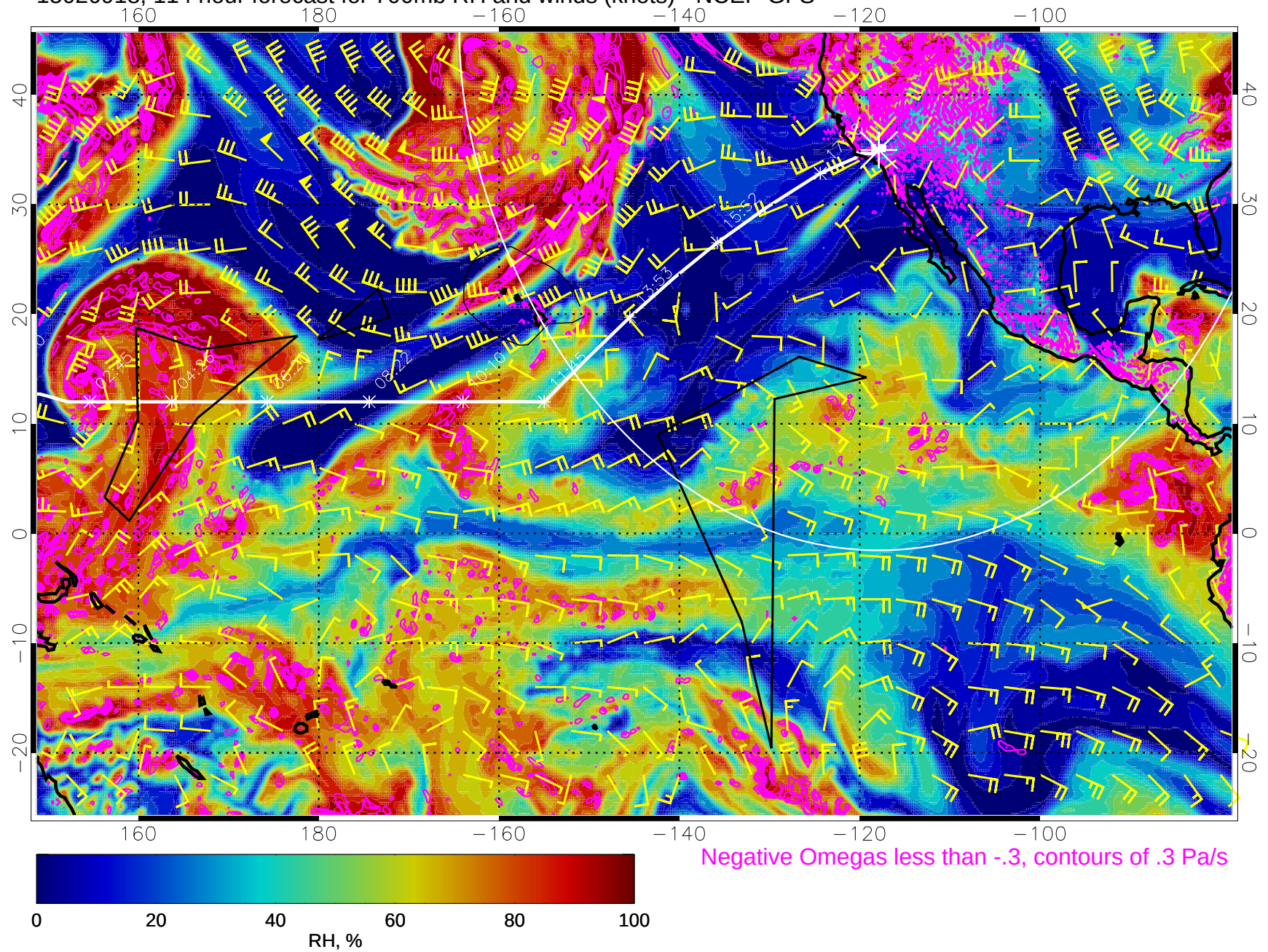
15020918, 114 hour forecast for 700mb RH and winds (knots) - NCEP GFS
