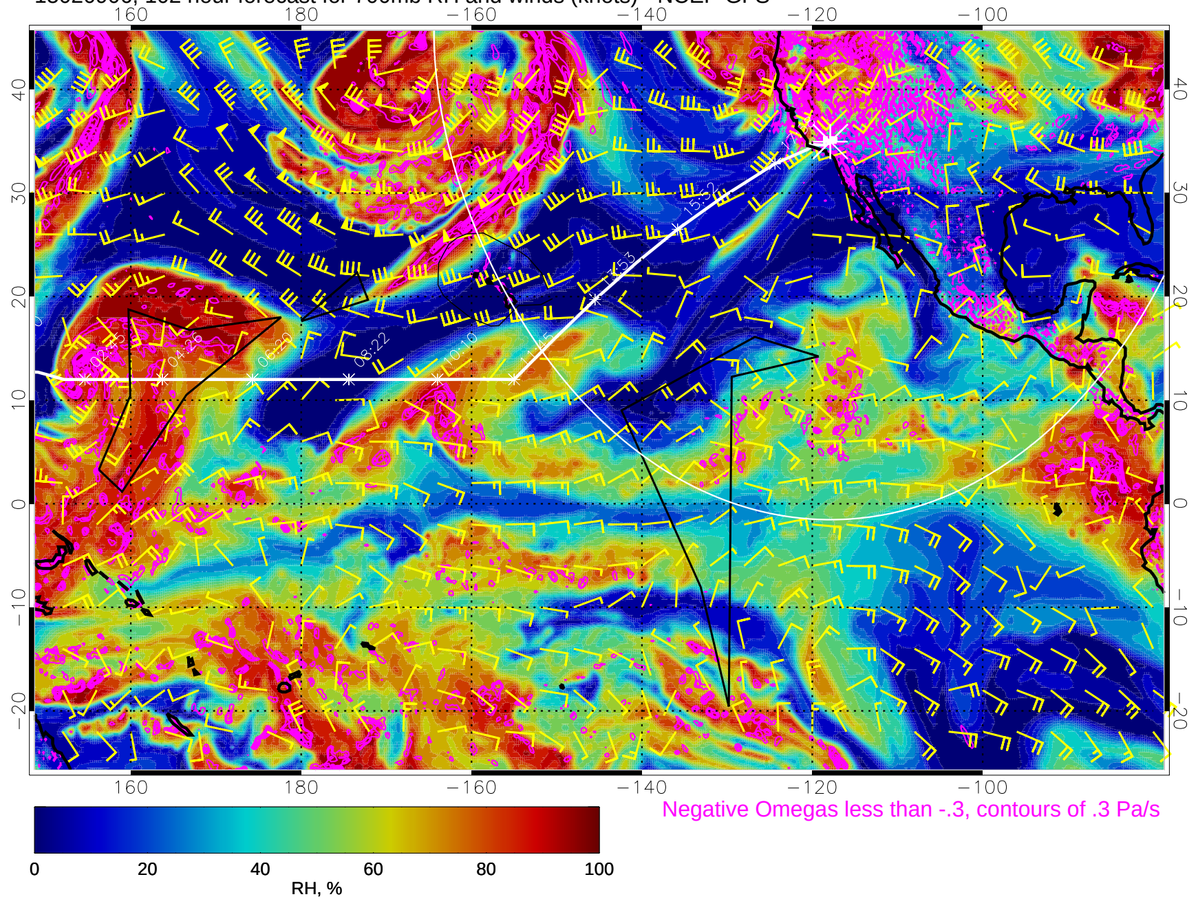
15020906, 102 hour forecast for 700mb RH and winds (knots) - NCEP GFS
