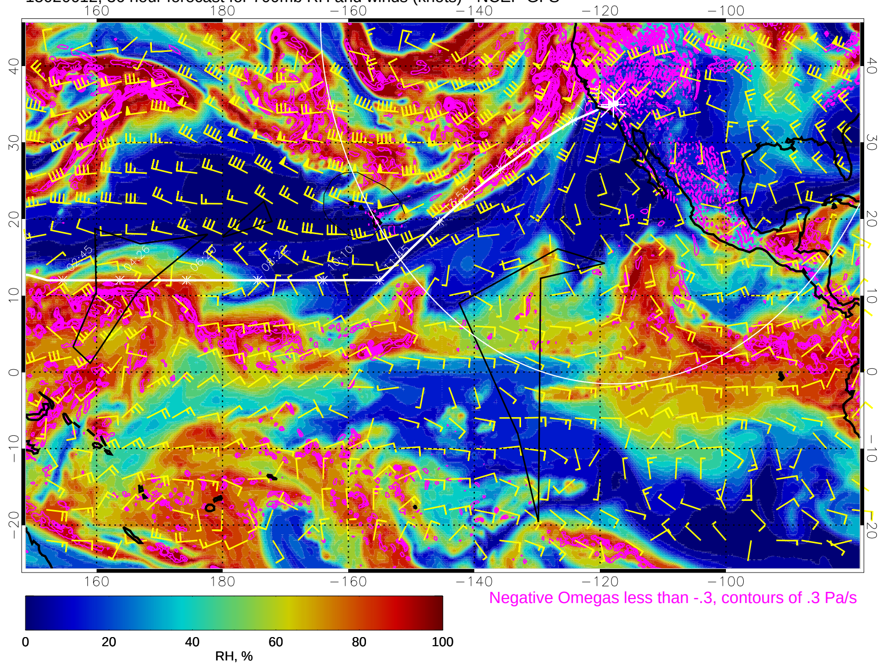
15020612, 36 hour forecast for 700mb RH and winds (knots) - NCEP GFS
