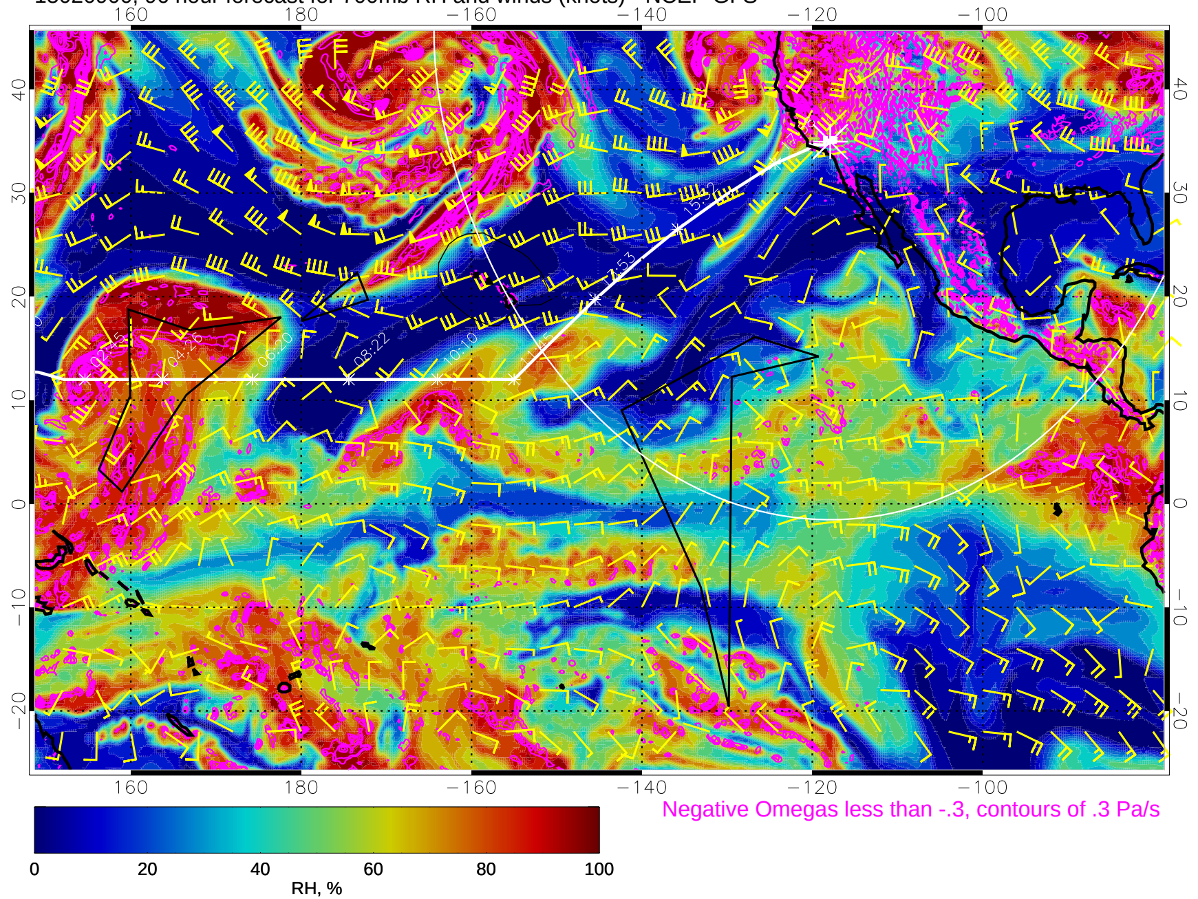
15020900, 96 hour forecast for 700mb RH and winds (knots) - NCEP GFS
