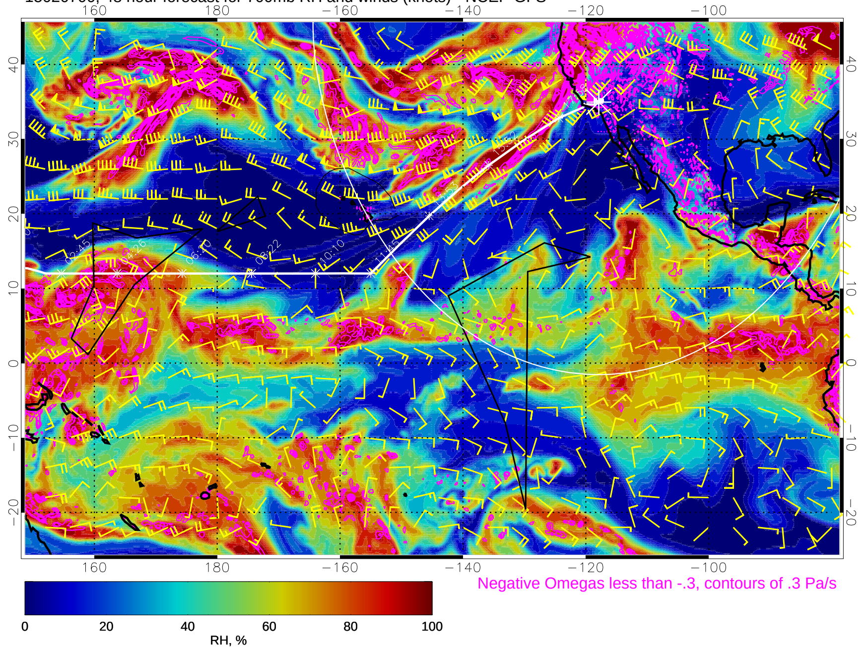
15020700, 48 hour forecast for 700mb RH and winds (knots) - NCEP GFS
