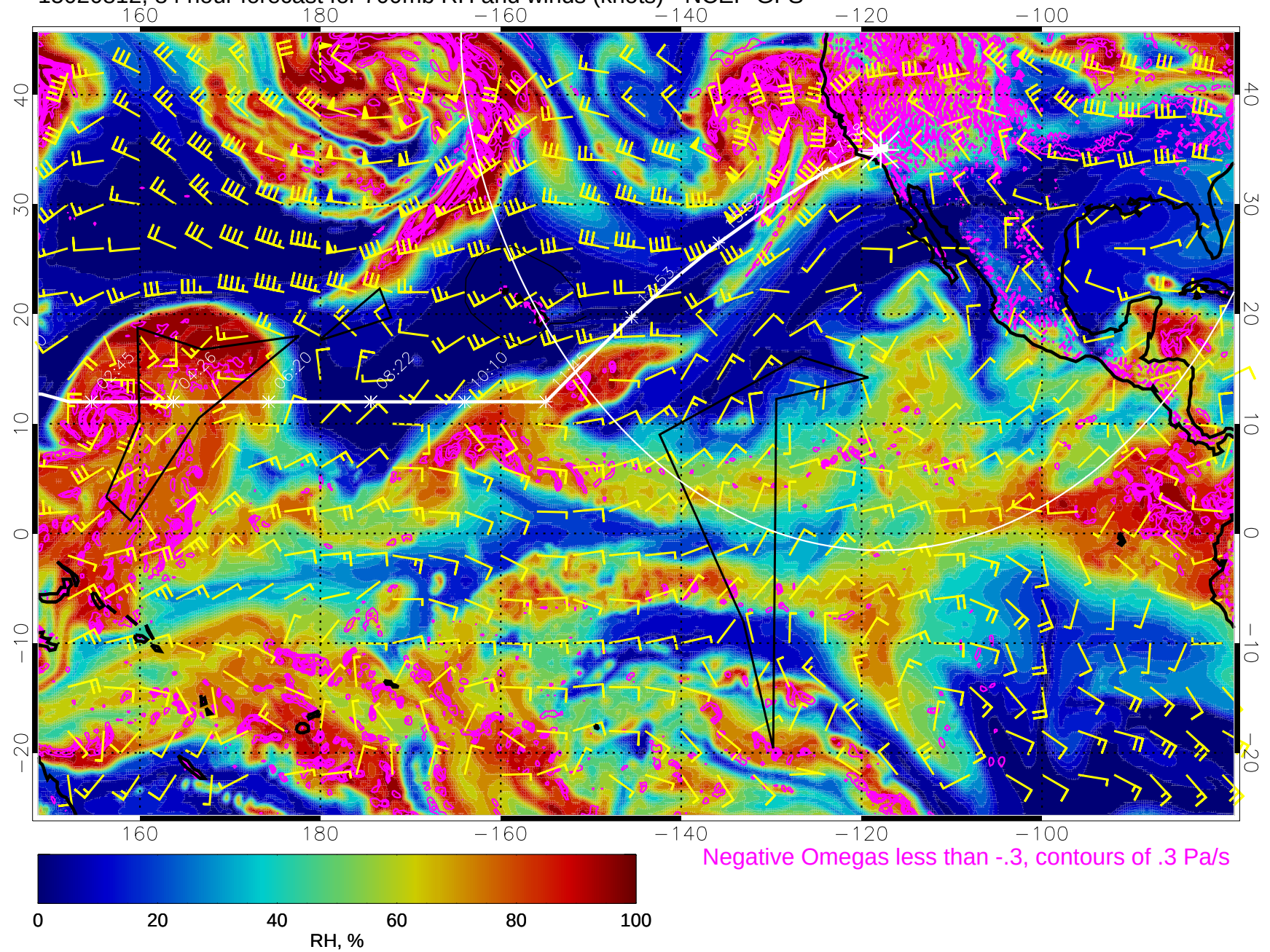
15020812, 84 hour forecast for 700mb RH and winds (knots) - NCEP GFS
