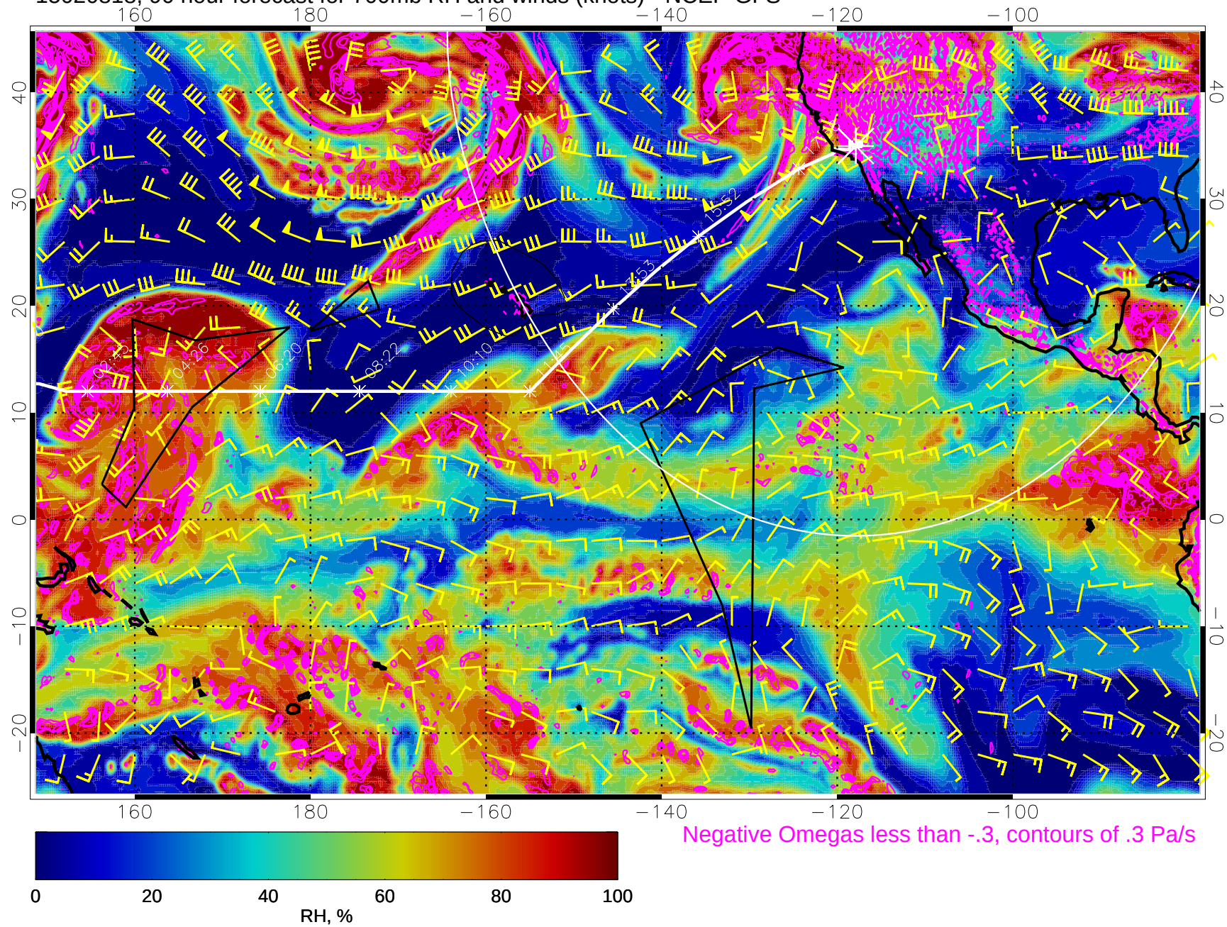
15020818, 90 hour forecast for 700mb RH and winds (knots) - NCEP GFS
