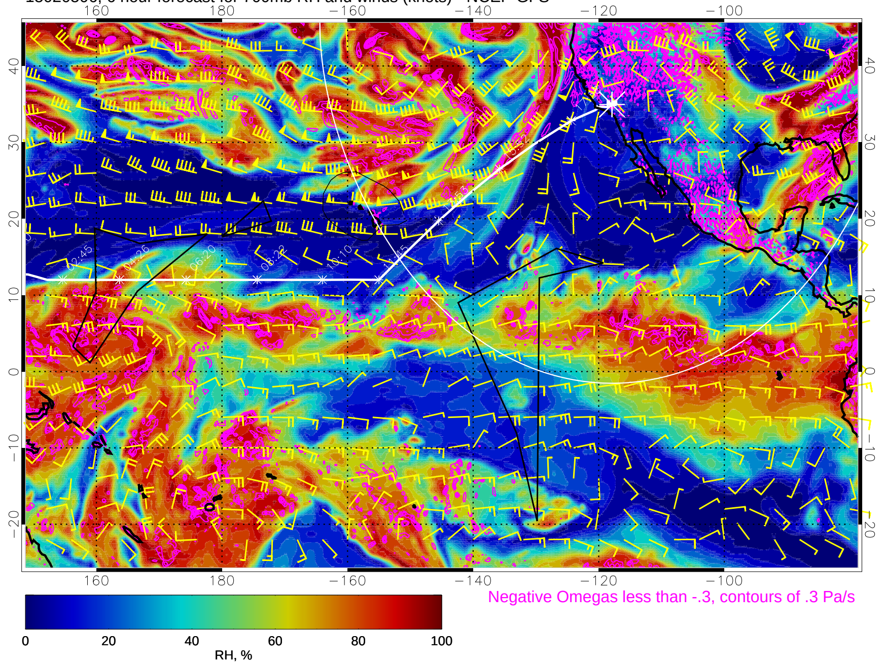
15020506, 6 hour forecast for 700mb RH and winds (knots) - NCEP GFS
