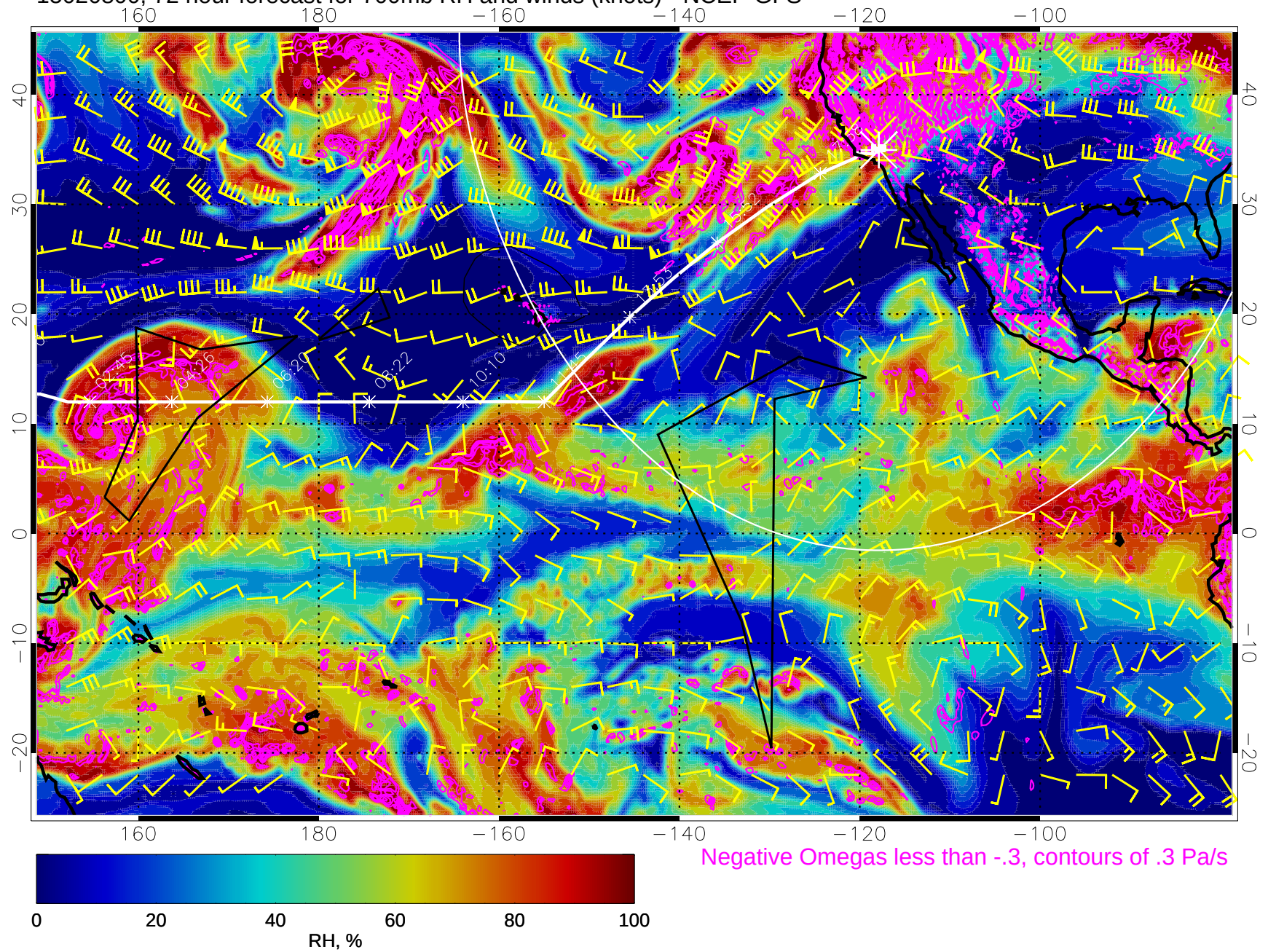
15020800, 72 hour forecast for 700mb RH and winds (knots) - NCEP GFS
