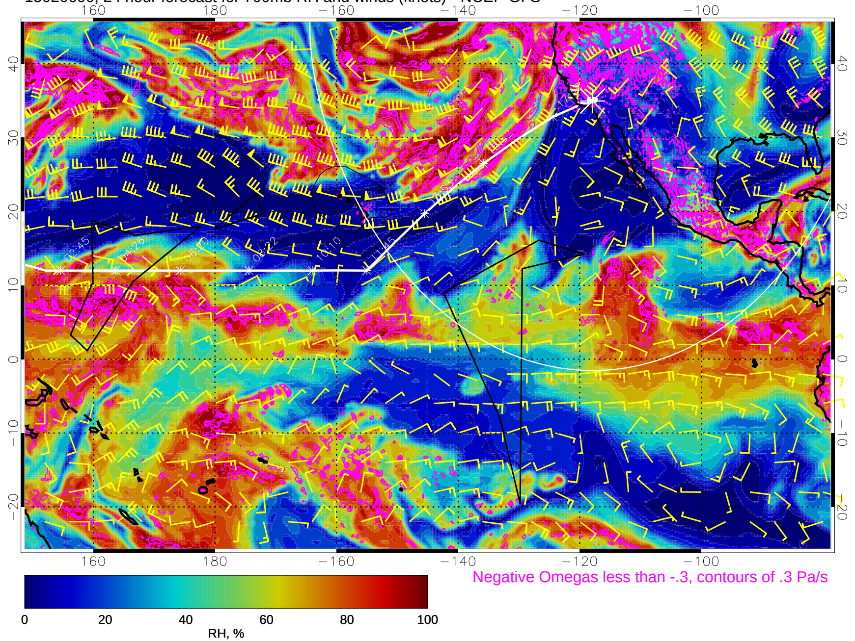
15020600, 24 hour forecast for 700mb RH and winds (knots) - NCEP GFS
