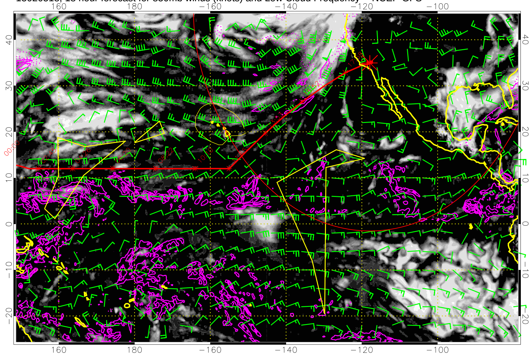
15020518, 18 hour forecast for 850mb winds (knots) and Low Cloud Frequency -- NCEP GFS
