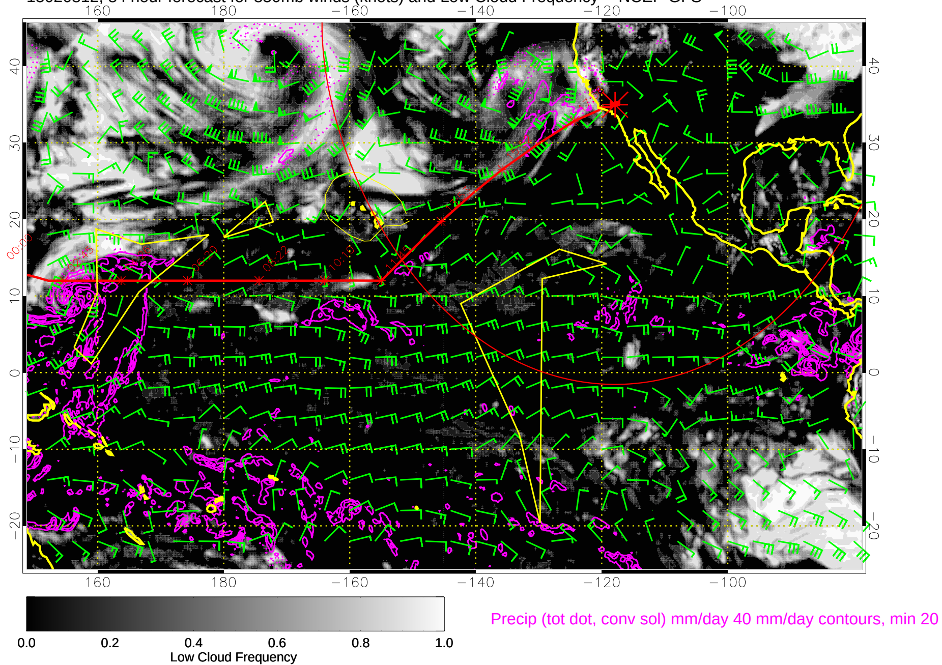
15020812, 84 hour forecast for 850mb winds (knots) and Low Cloud Frequency -- NCEP GFS
