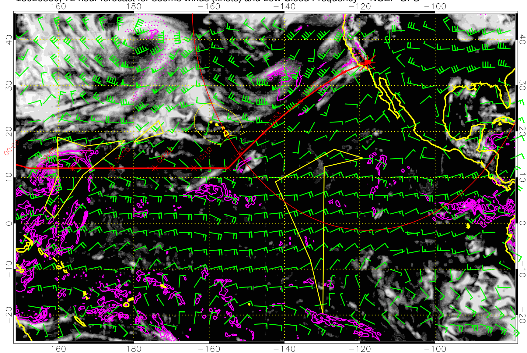
15020800, 72 hour forecast for 850mb winds (knots) and Low Cloud Frequency -- NCEP GFS
