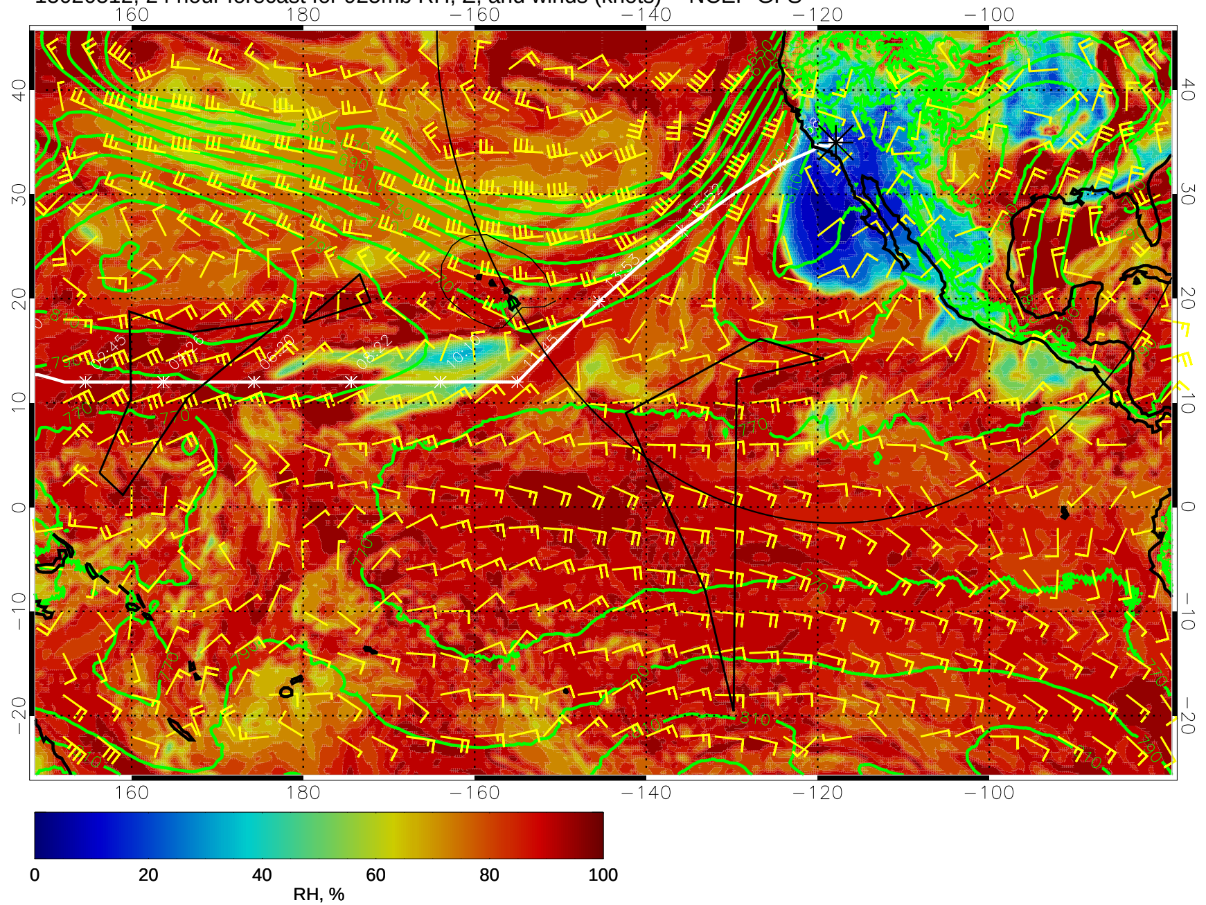
15020512, 24 hour forecast for 925mb RH, Z, and winds (knots) -- NCEP GFS
