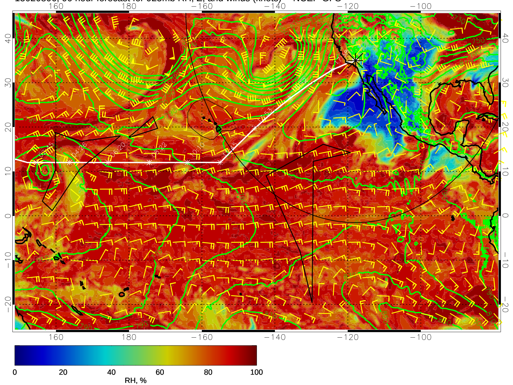
15020806, 90 hour forecast for 925mb RH, Z, and winds (knots) -- NCEP GFS
