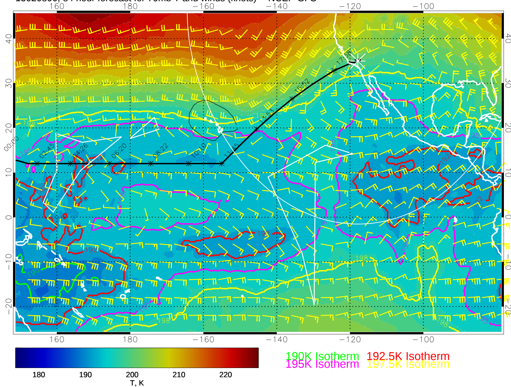
15020800, 84 hour forecast for 70mb T and winds (knots) -- NCEP GFS
