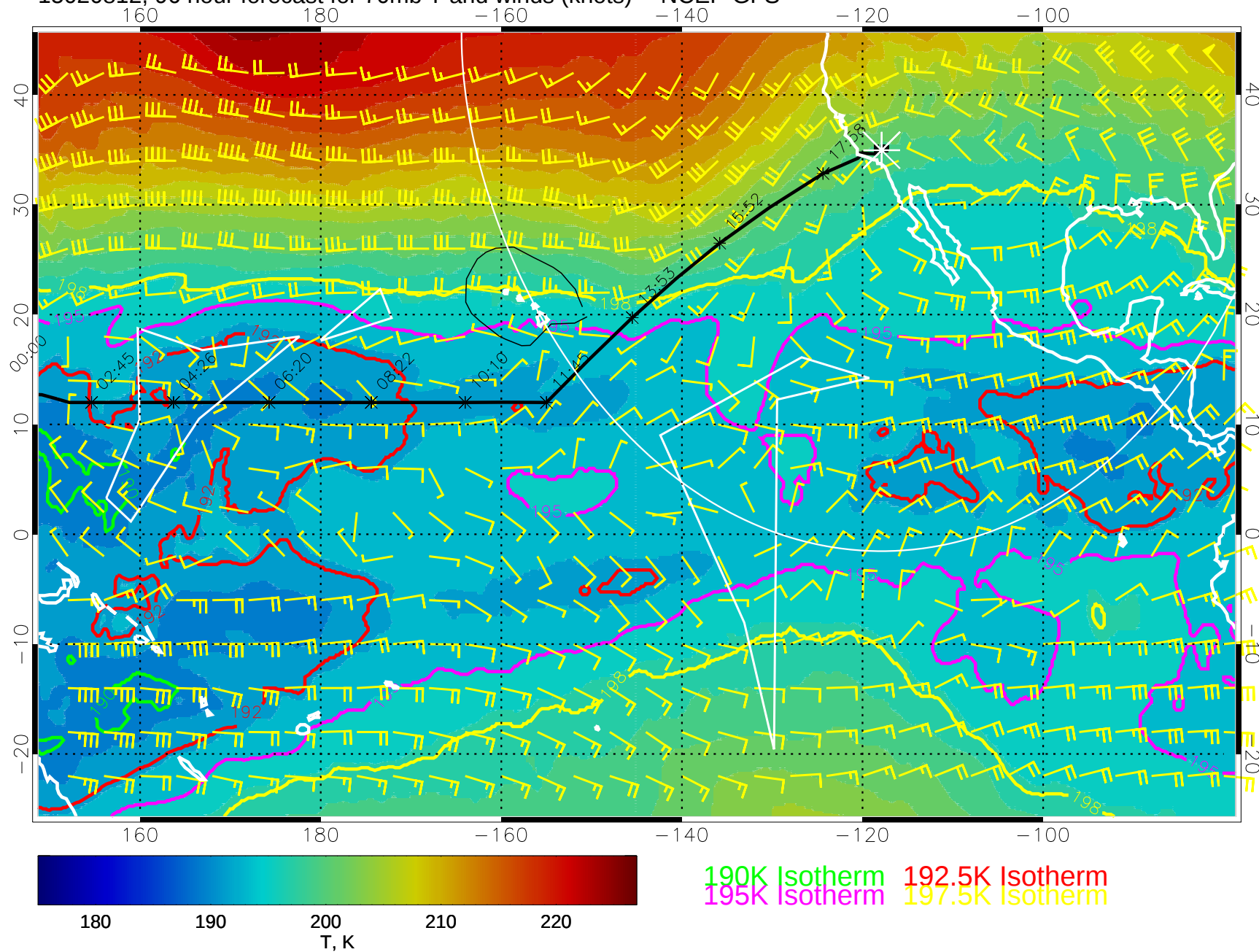
15020812, 96 hour forecast for 70mb T and winds (knots) -- NCEP GFS
