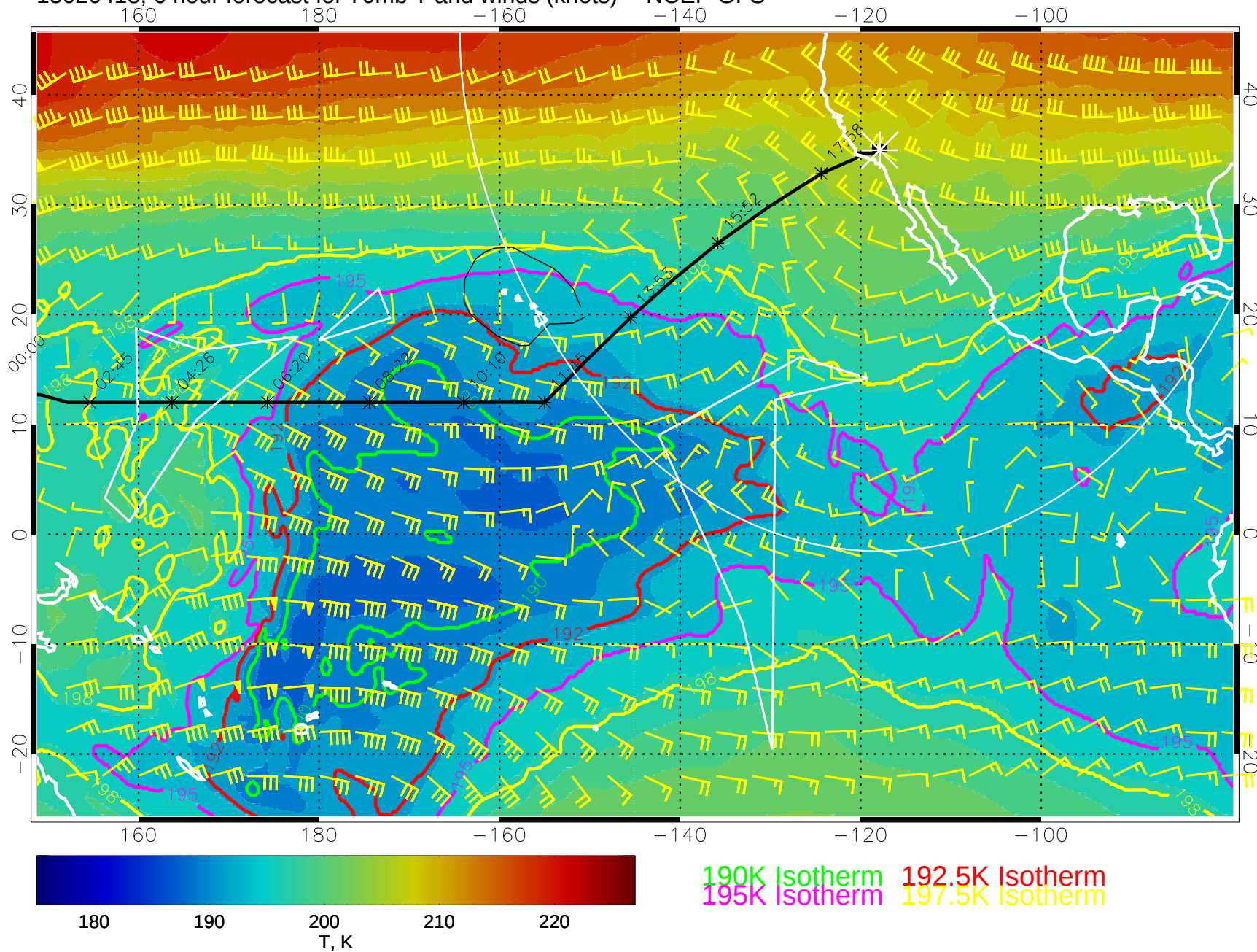
15020418, 6 hour forecast for 70mb T and winds (knots) -- NCEP GFS
