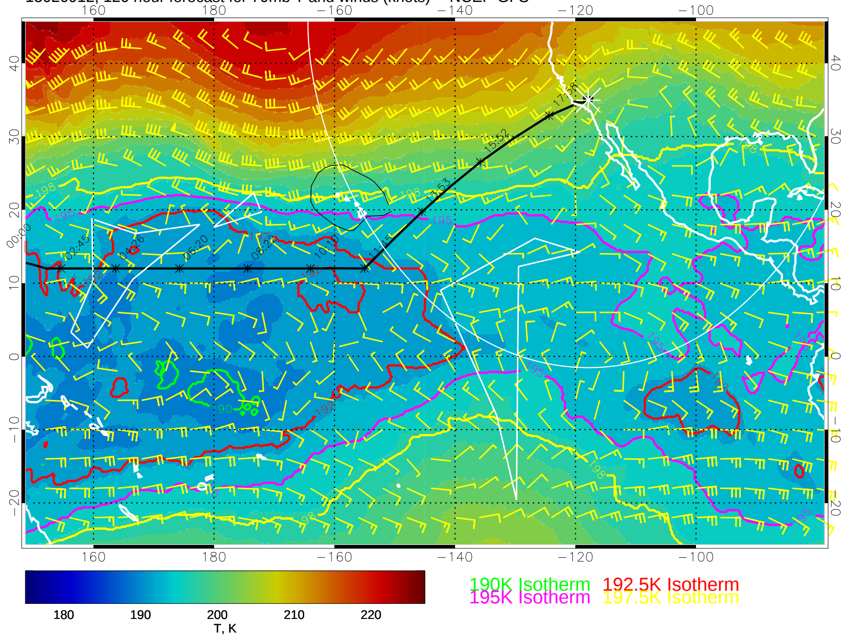
15020912, 120 hour forecast for 70mb T and winds (knots) -- NCEP GFS
