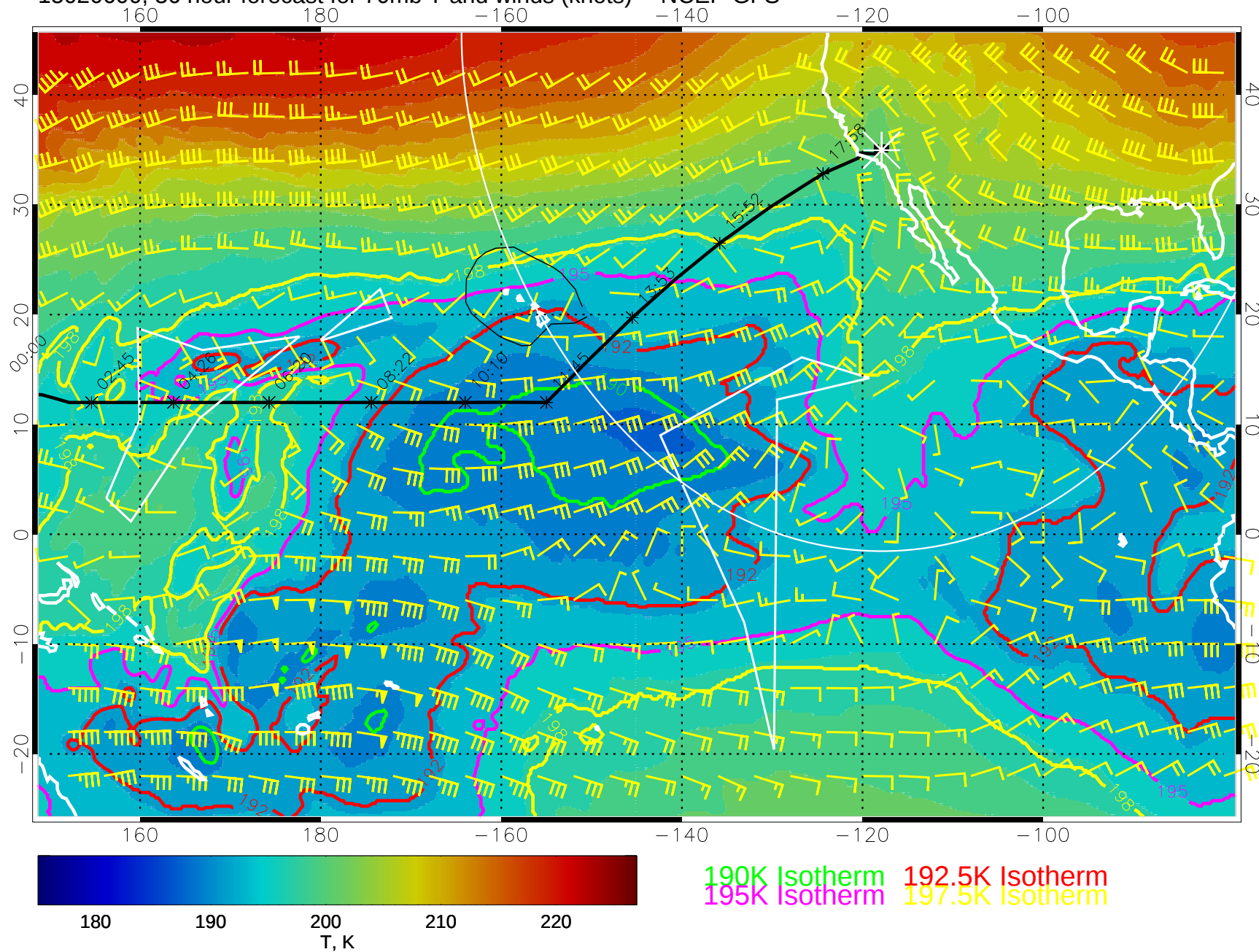
15020600, 36 hour forecast for 70mb T and winds (knots) -- NCEP GFS
