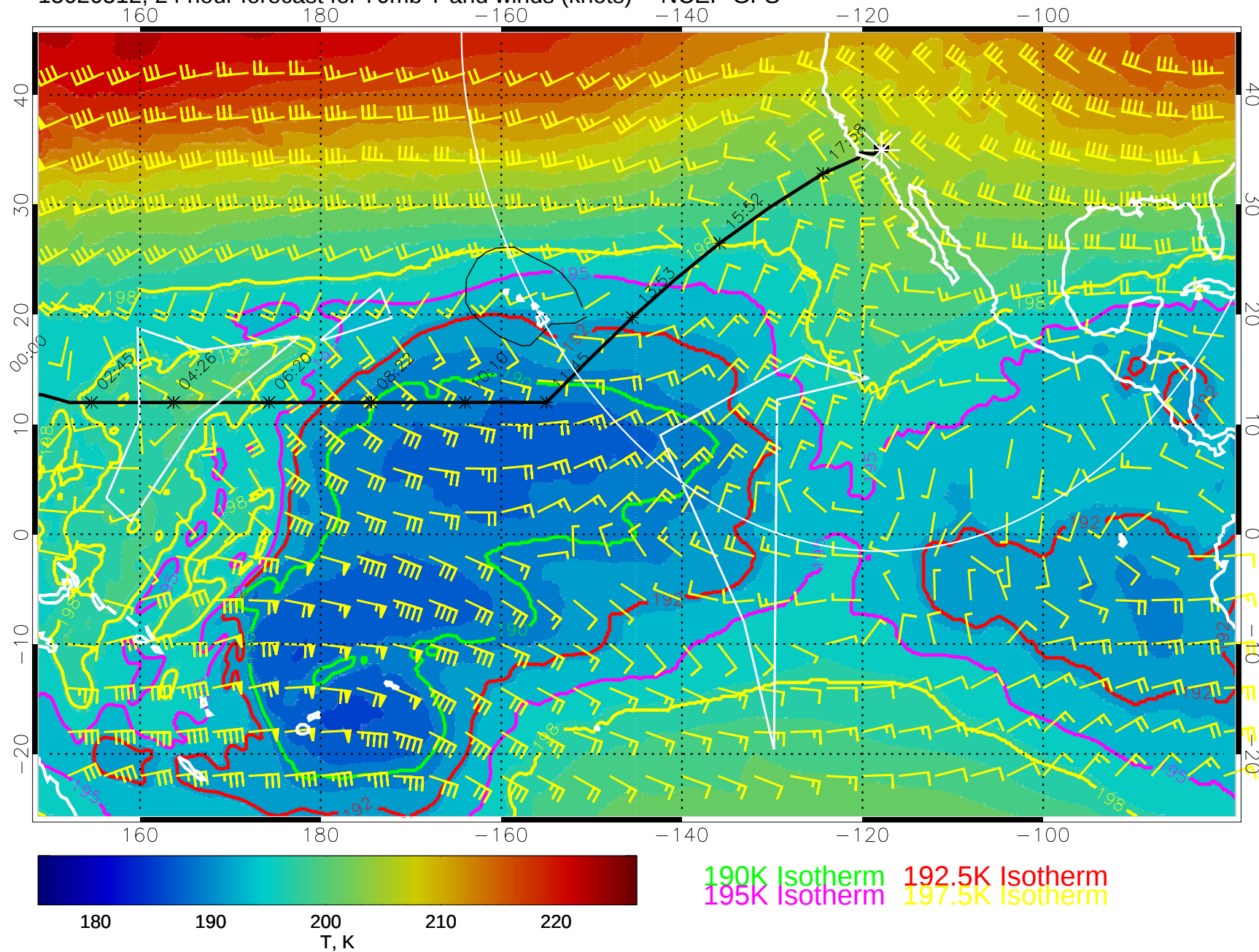
15020512, 24 hour forecast for 70mb T and winds (knots) -- NCEP GFS
