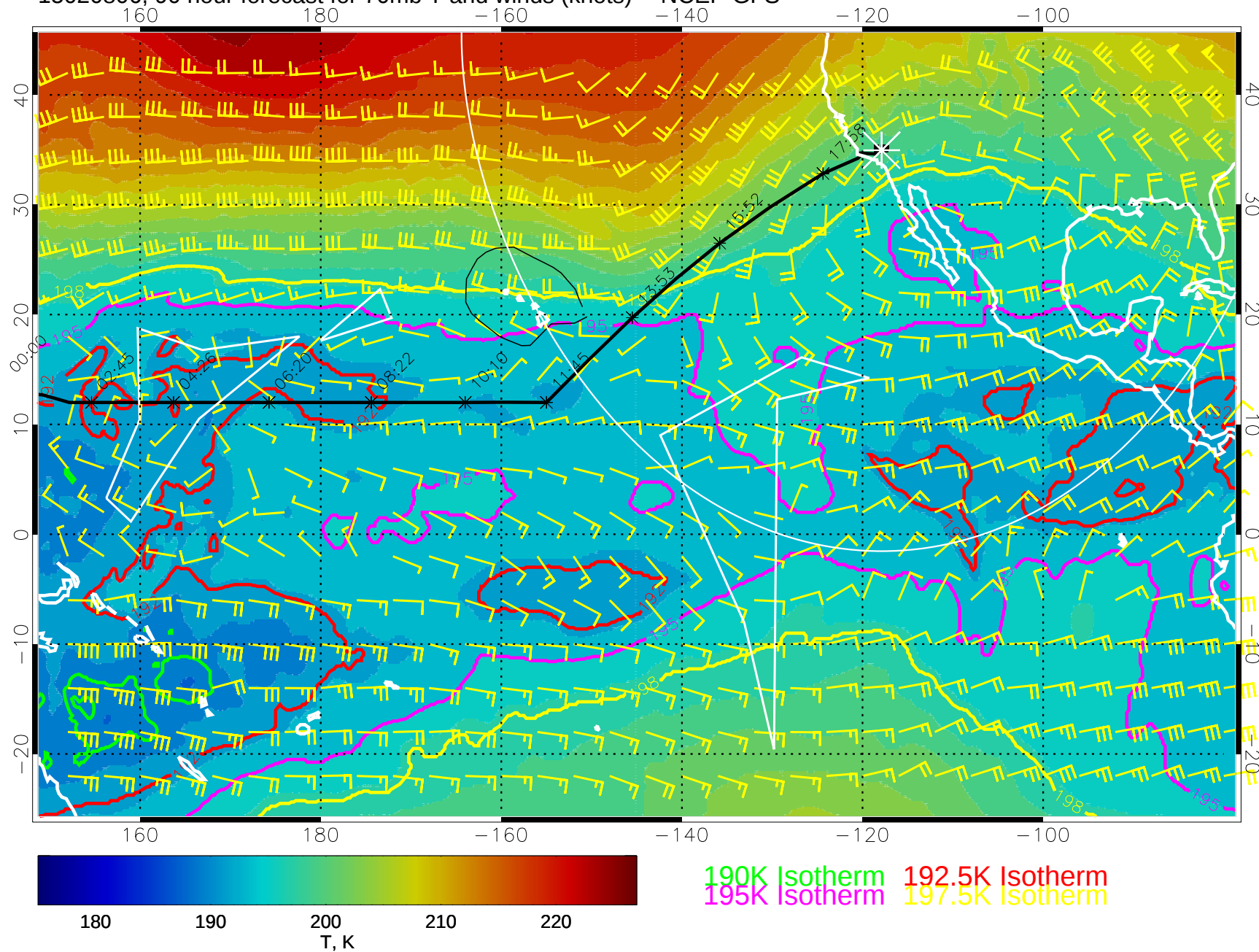
15020806, 90 hour forecast for 70mb T and winds (knots) -- NCEP GFS
