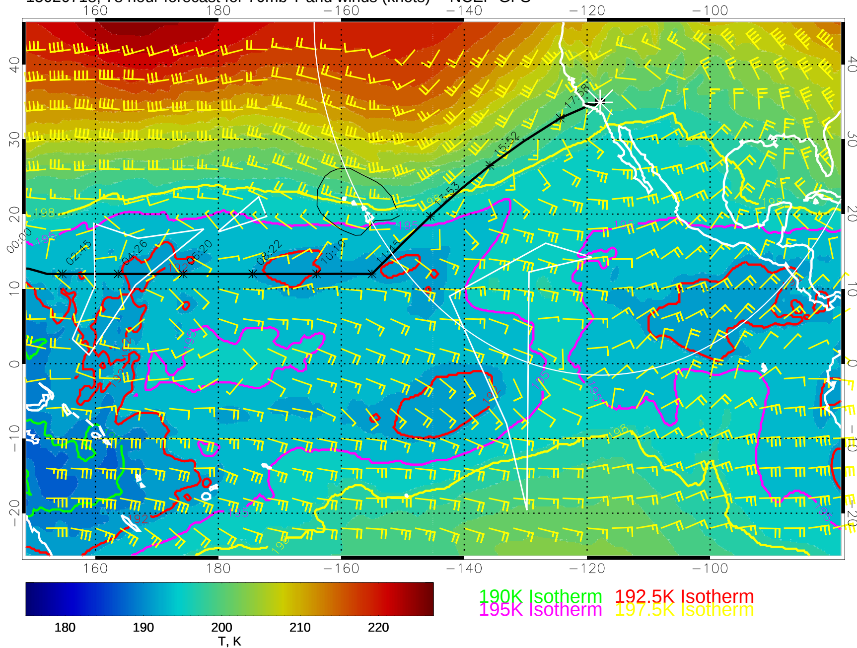
15020718, 78 hour forecast for 70mb T and winds (knots) -- NCEP GFS
