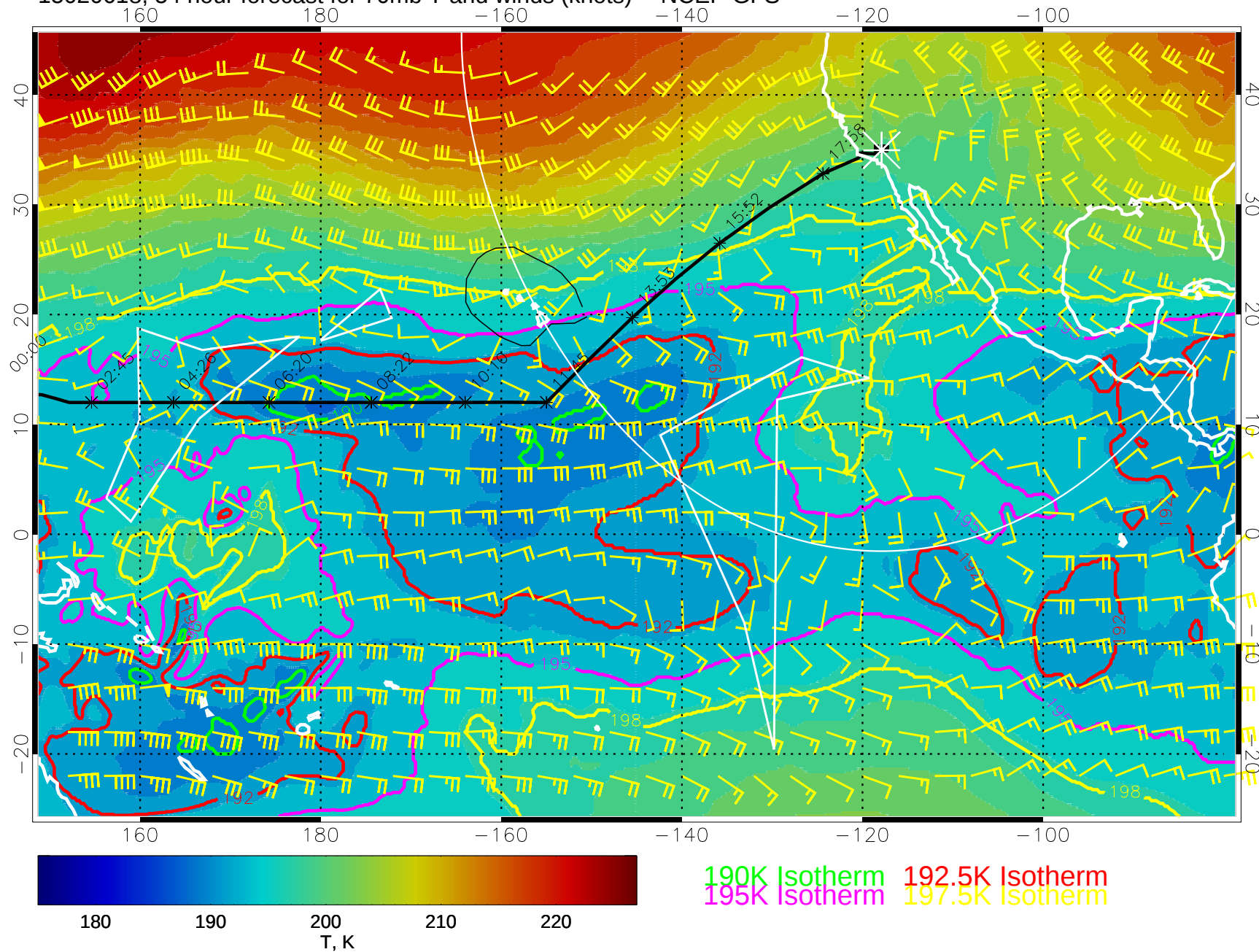
15020618, 54 hour forecast for 70mb T and winds (knots) -- NCEP GFS
