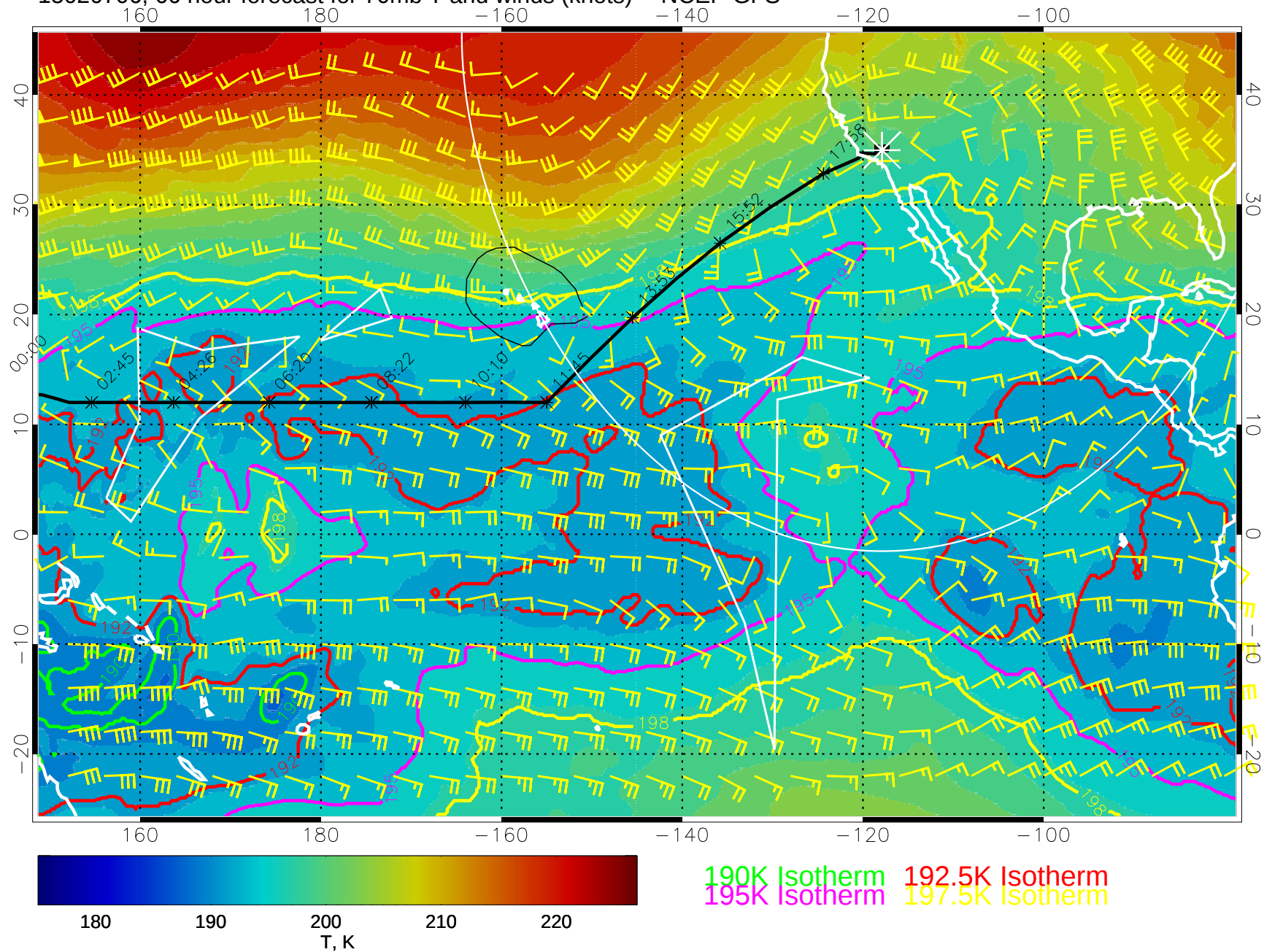
15020706, 66 hour forecast for 70mb T and winds (knots) -- NCEP GFS
