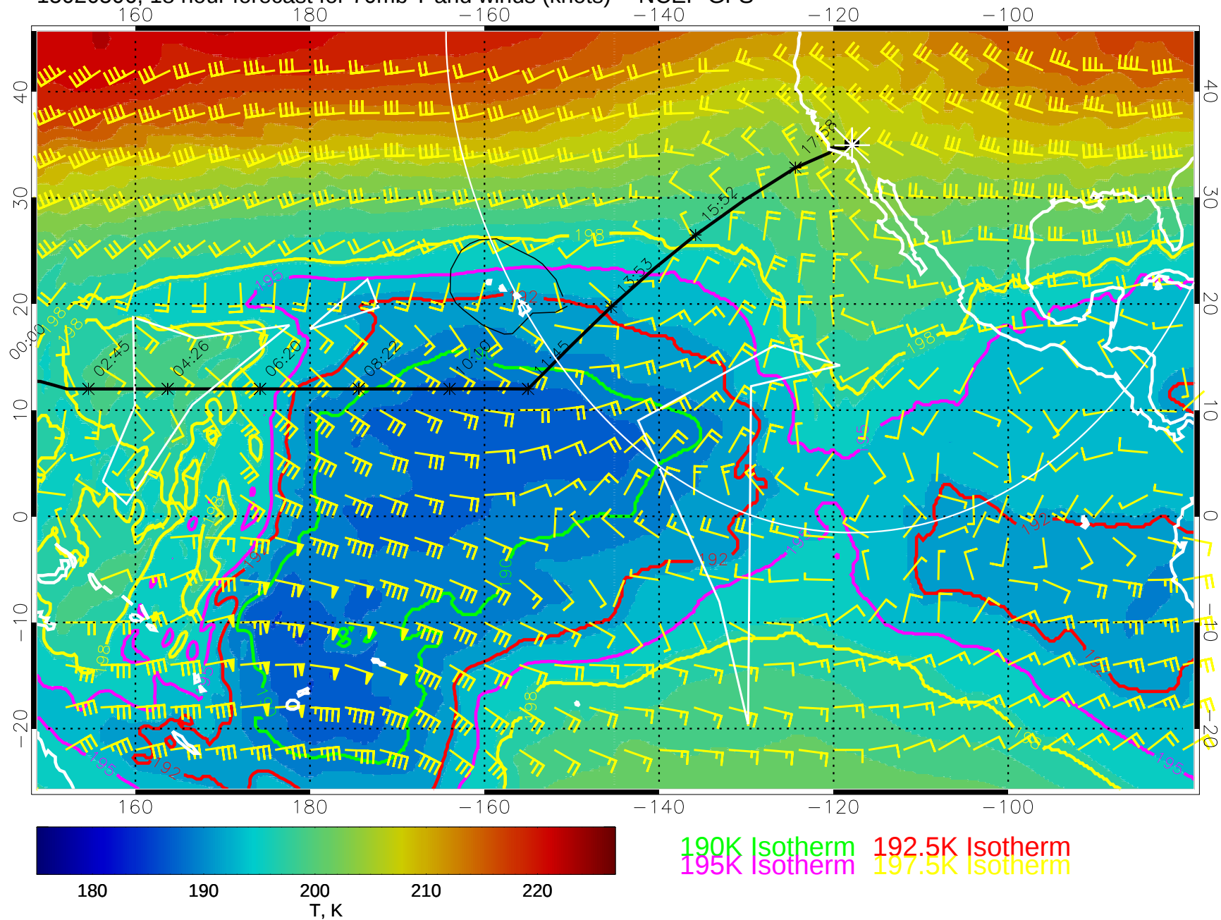
15020506, 18 hour forecast for 70mb T and winds (knots) -- NCEP GFS
