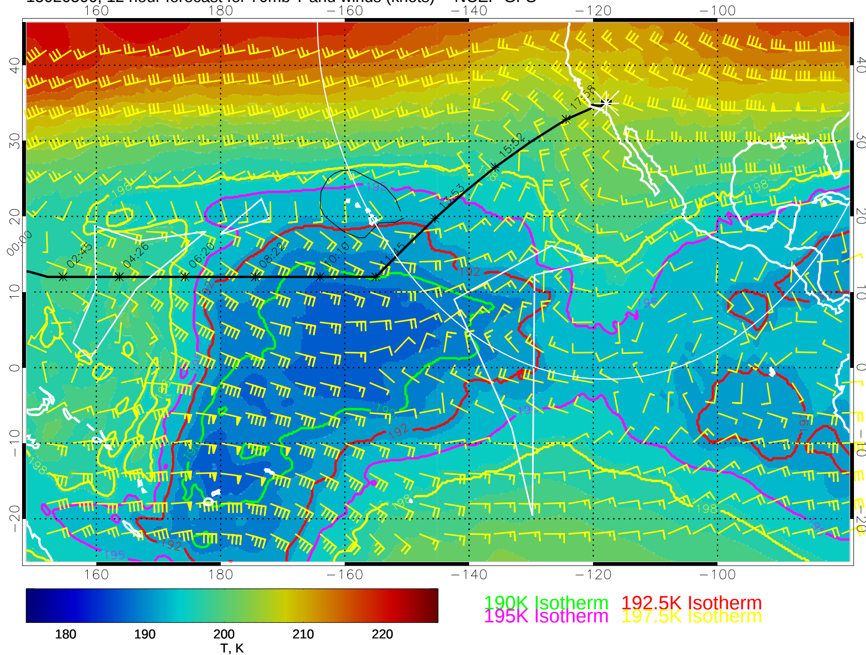
15020500, 12 hour forecast for 70mb T and winds (knots) -- NCEP GFS
