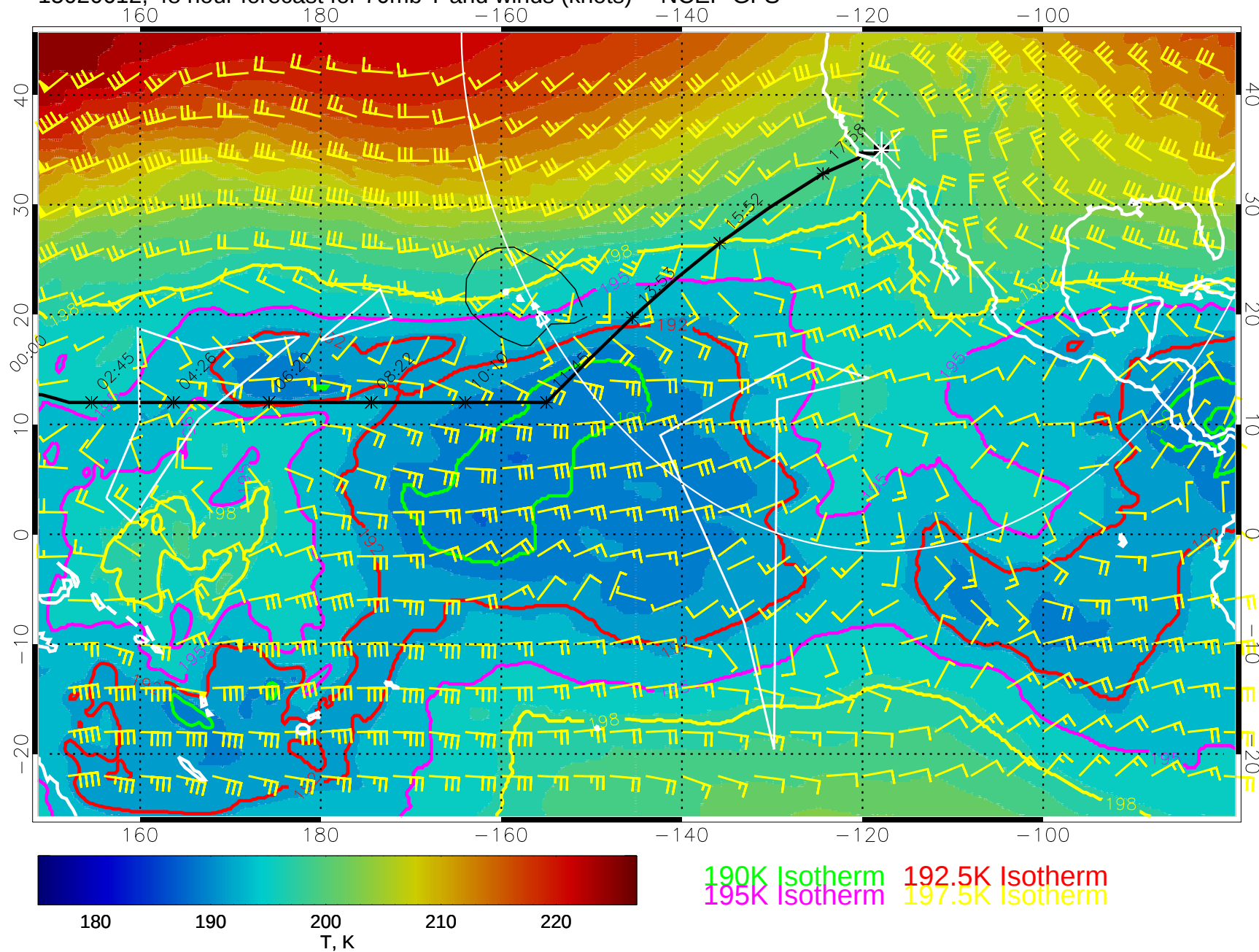
15020612, 48 hour forecast for 70mb T and winds (knots) -- NCEP GFS
