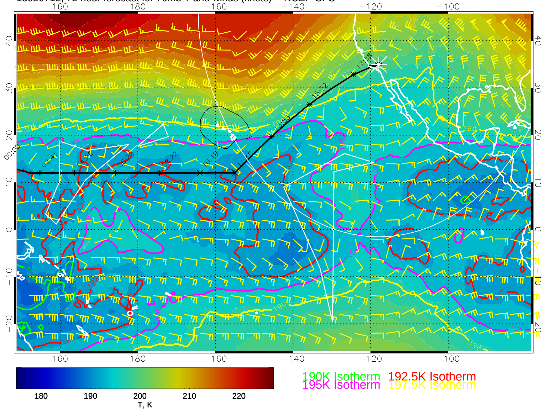
15020712, 72 hour forecast for 70mb T and winds (knots) -- NCEP GFS
