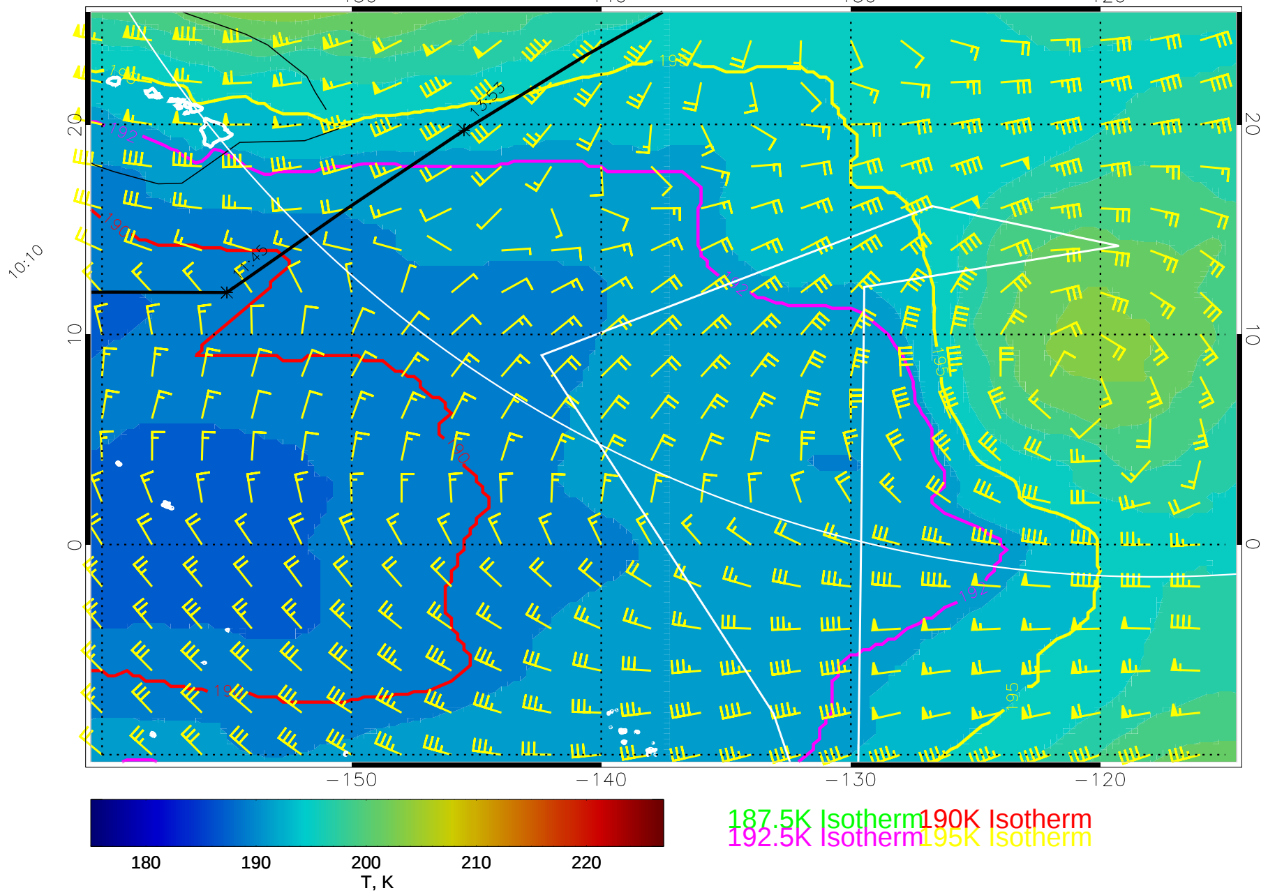
15020706, 66 hour forecast for 100mb T and winds (knots) -- NCEP GFS
