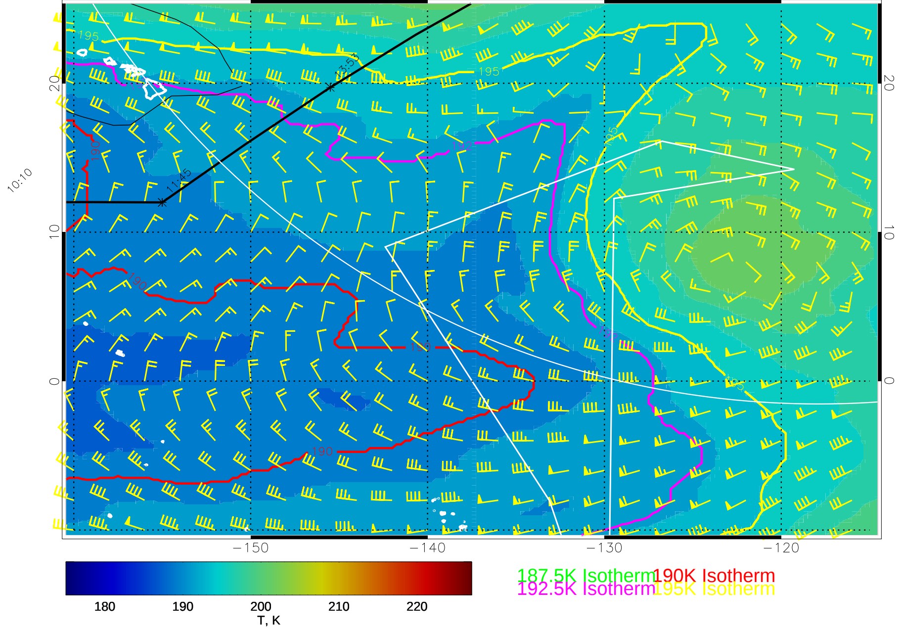
15020812, 96 hour forecast for 100mb T and winds (knots) -- NCEP GFS
