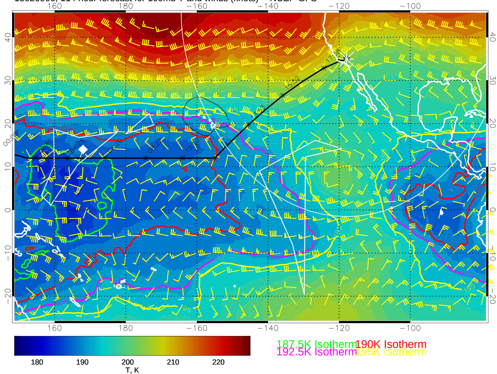
15020906, 114 hour forecast for 100mb T and winds (knots) -- NCEP GFS
