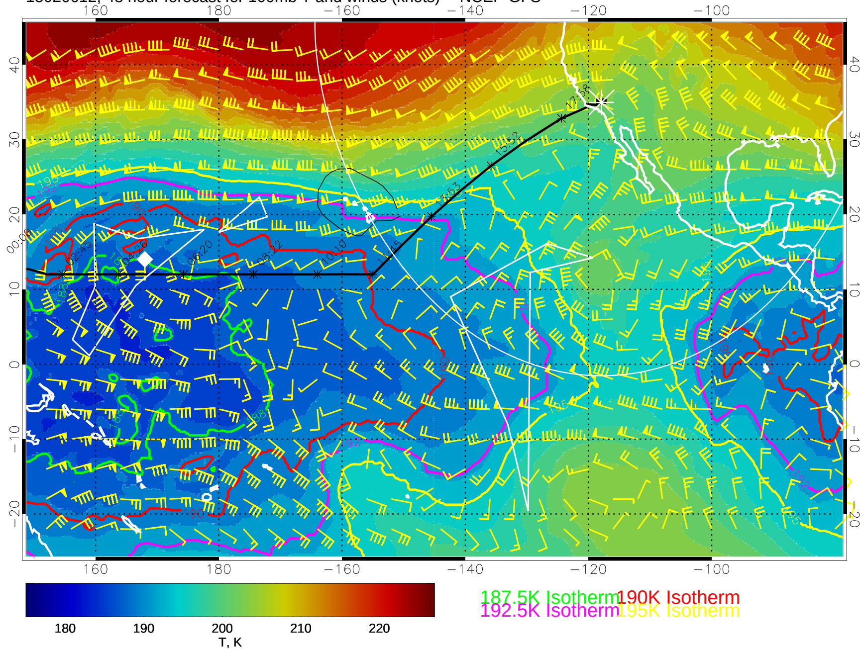
15020612, 48 hour forecast for 100mb T and winds (knots) -- NCEP GFS
