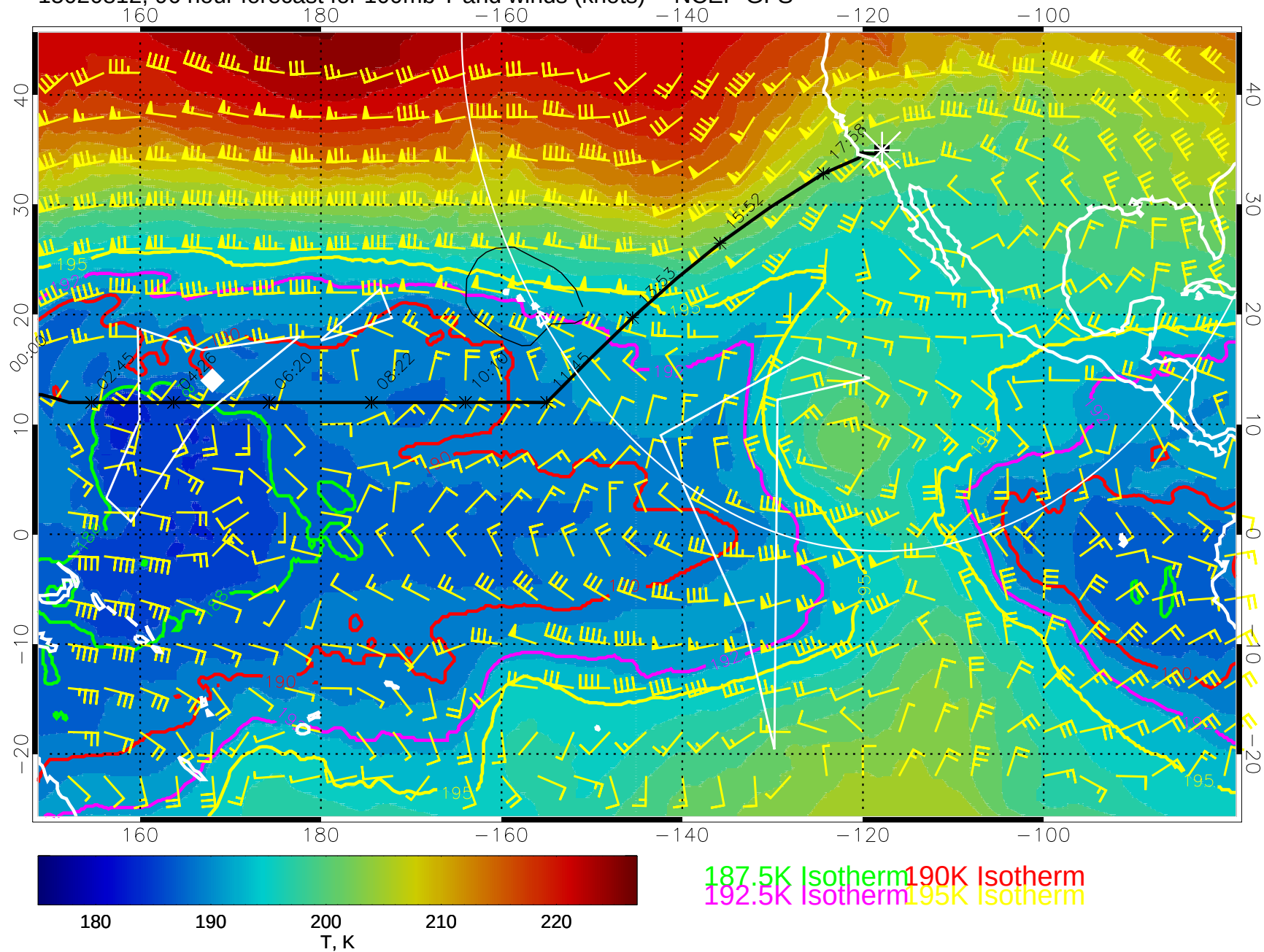
15020812, 96 hour forecast for 100mb T and winds (knots) -- NCEP GFS
