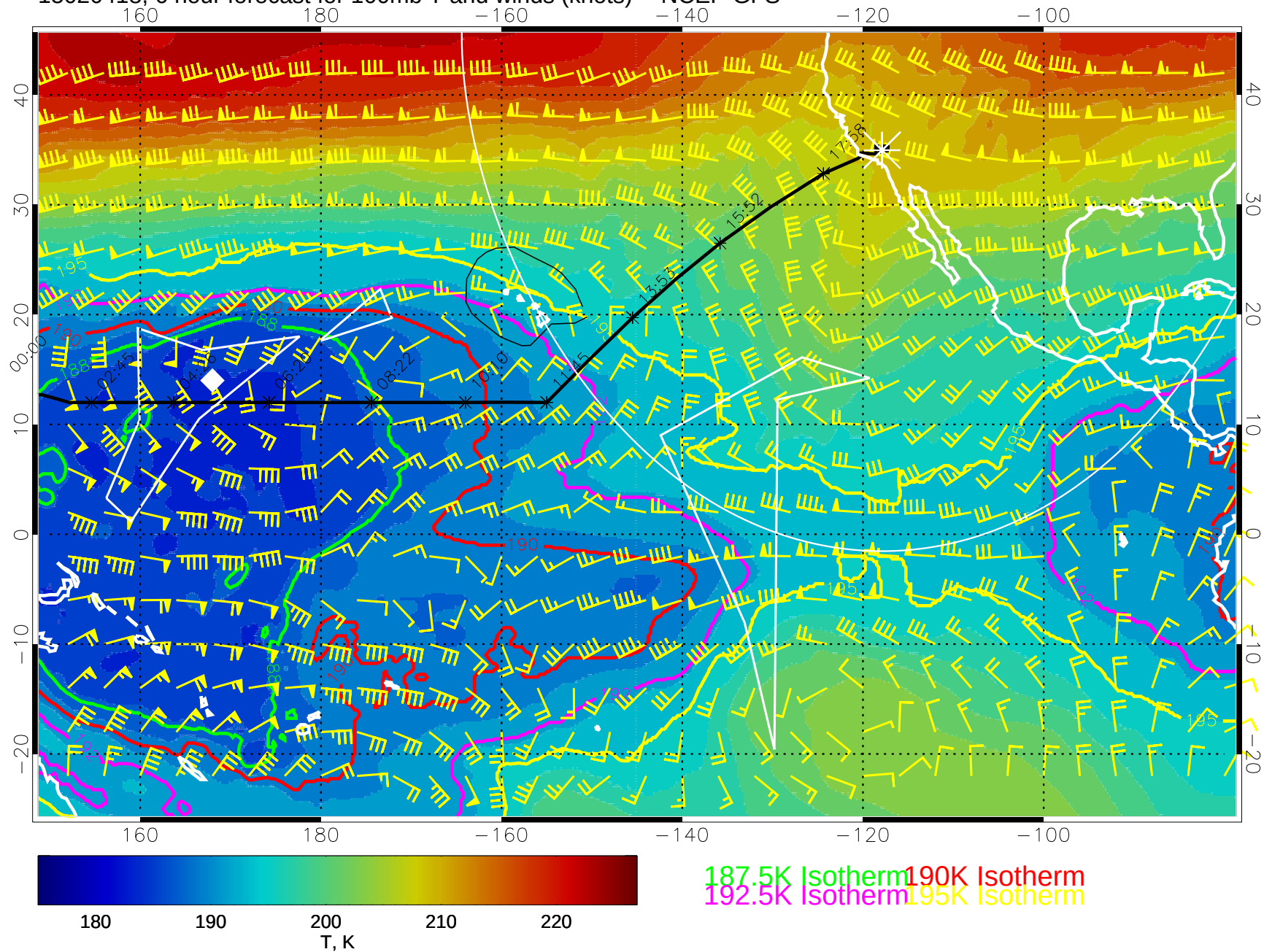
15020418, 6 hour forecast for 100mb T and winds (knots) -- NCEP GFS
