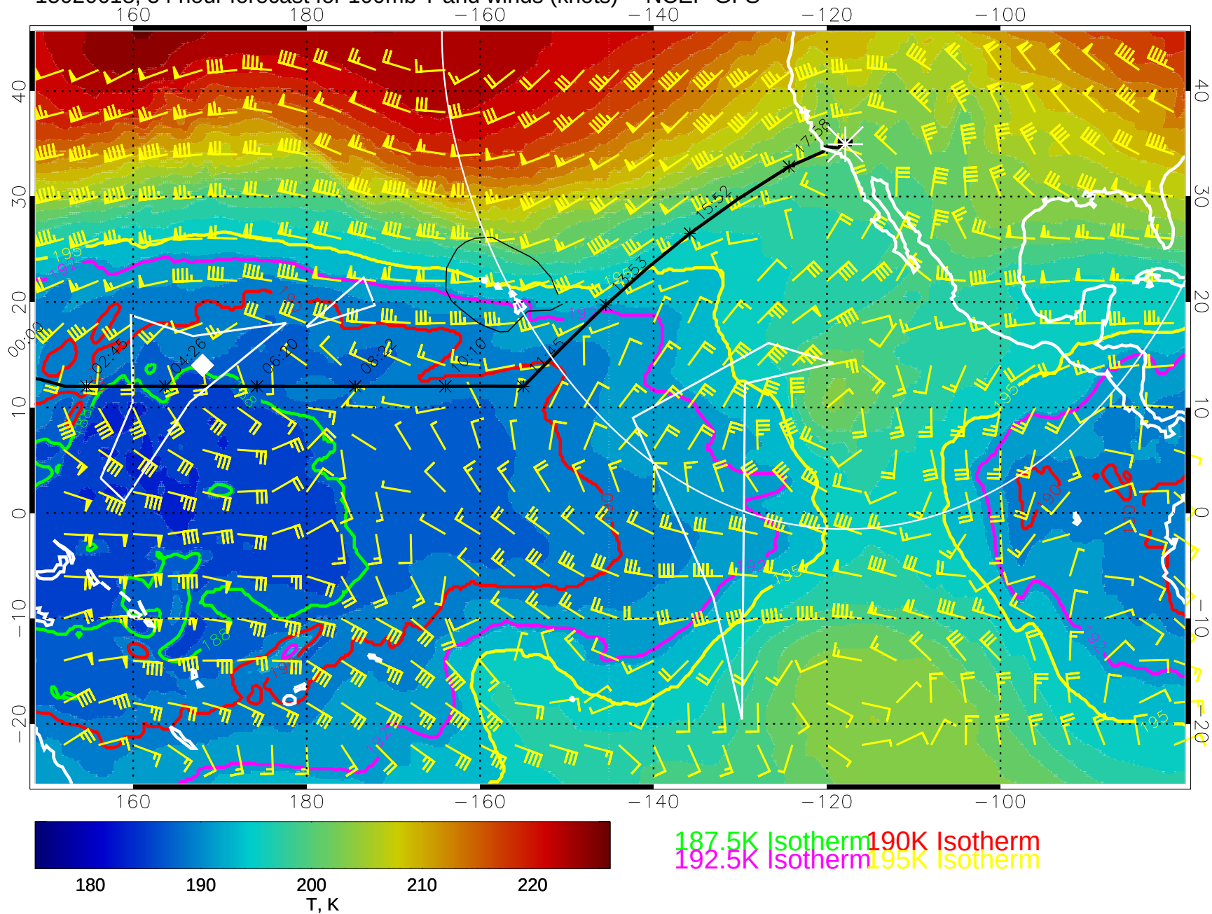
15020618, 54 hour forecast for 100mb T and winds (knots) -- NCEP GFS
