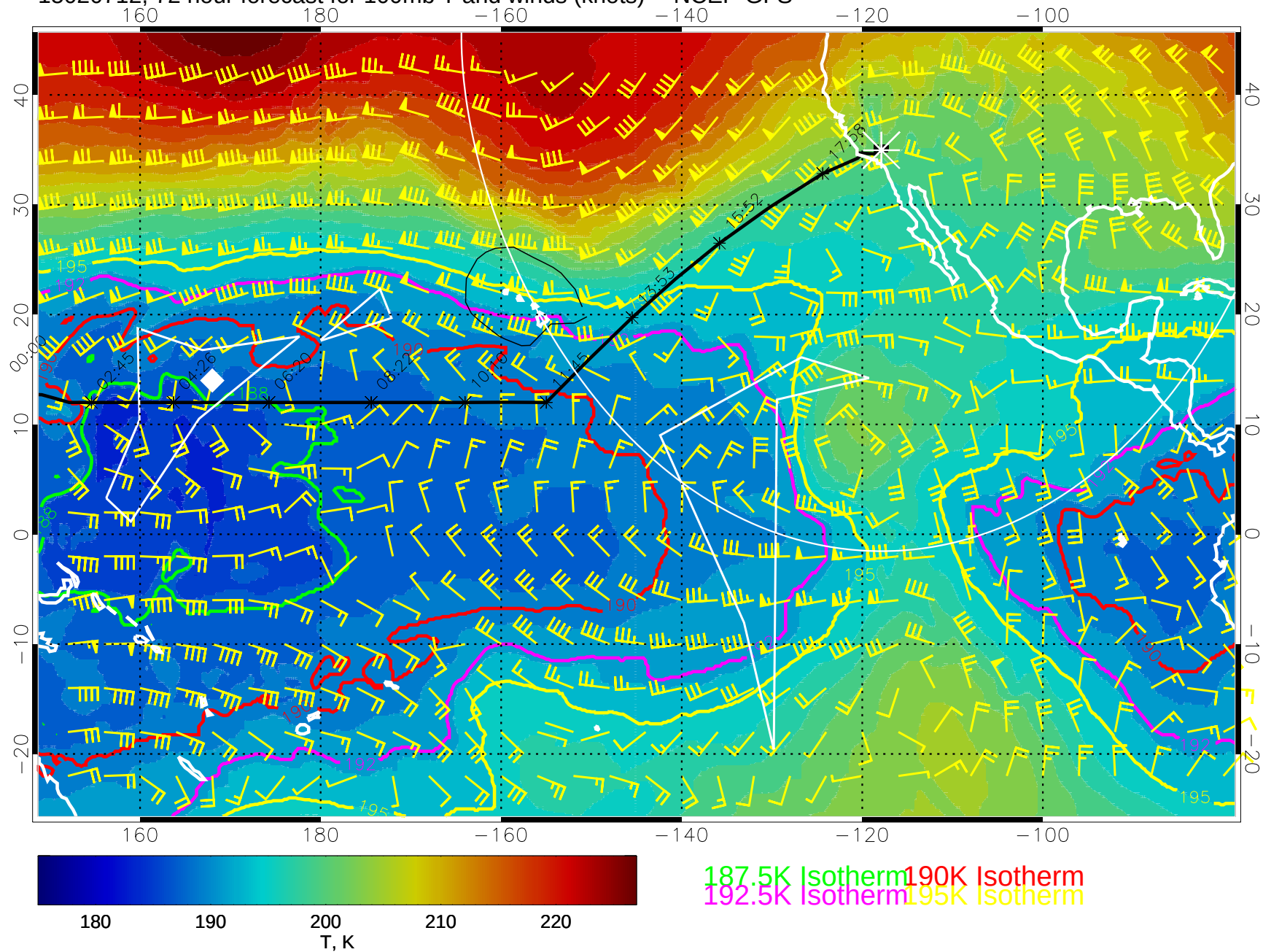
15020712, 72 hour forecast for 100mb T and winds (knots) -- NCEP GFS
