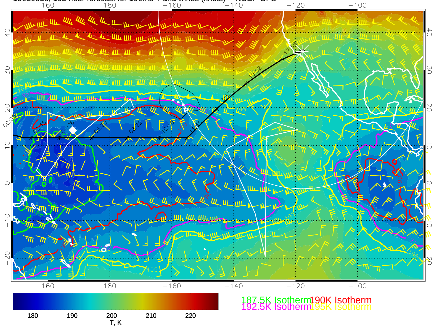
15020818, 102 hour forecast for 100mb T and winds (knots) -- NCEP GFS
