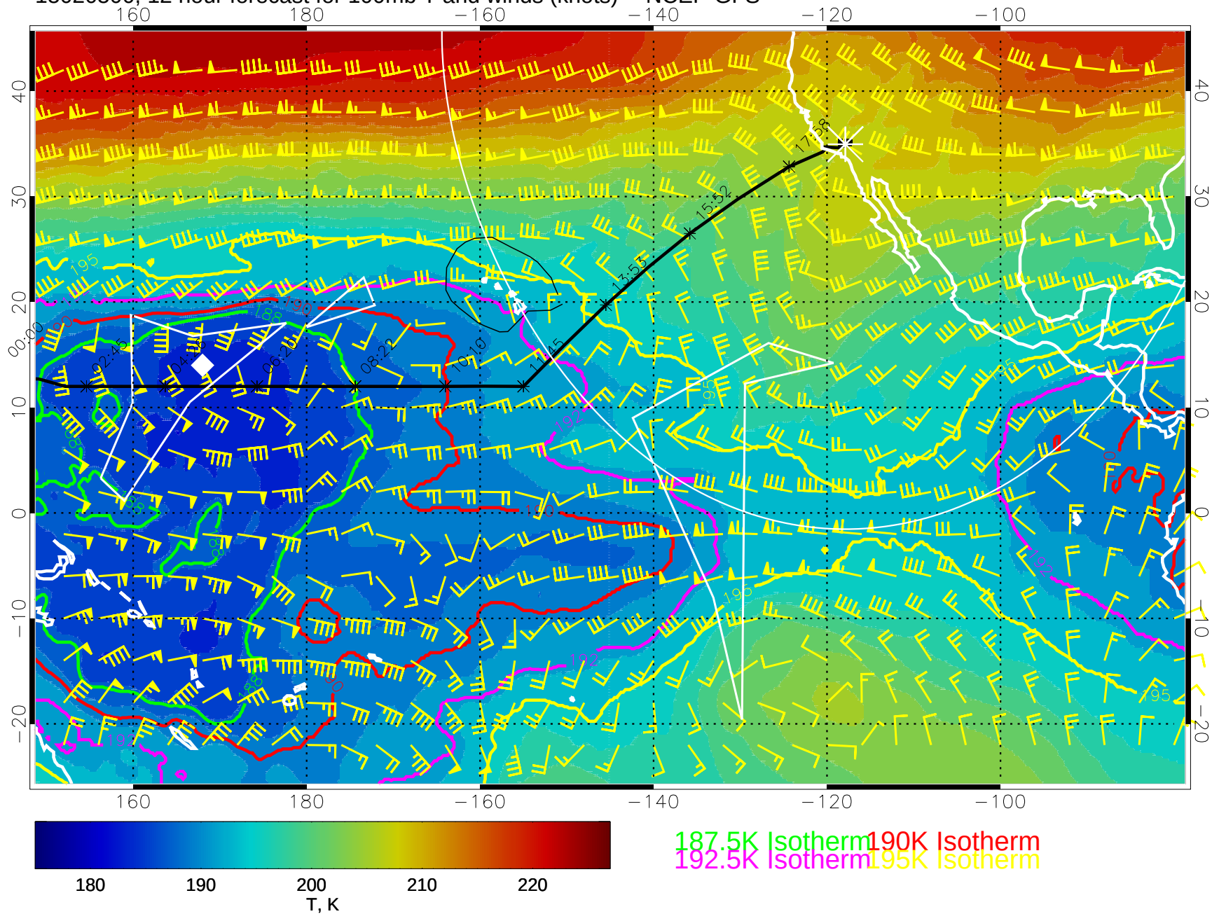
15020500, 12 hour forecast for 100mb T and winds (knots) -- NCEP GFS
