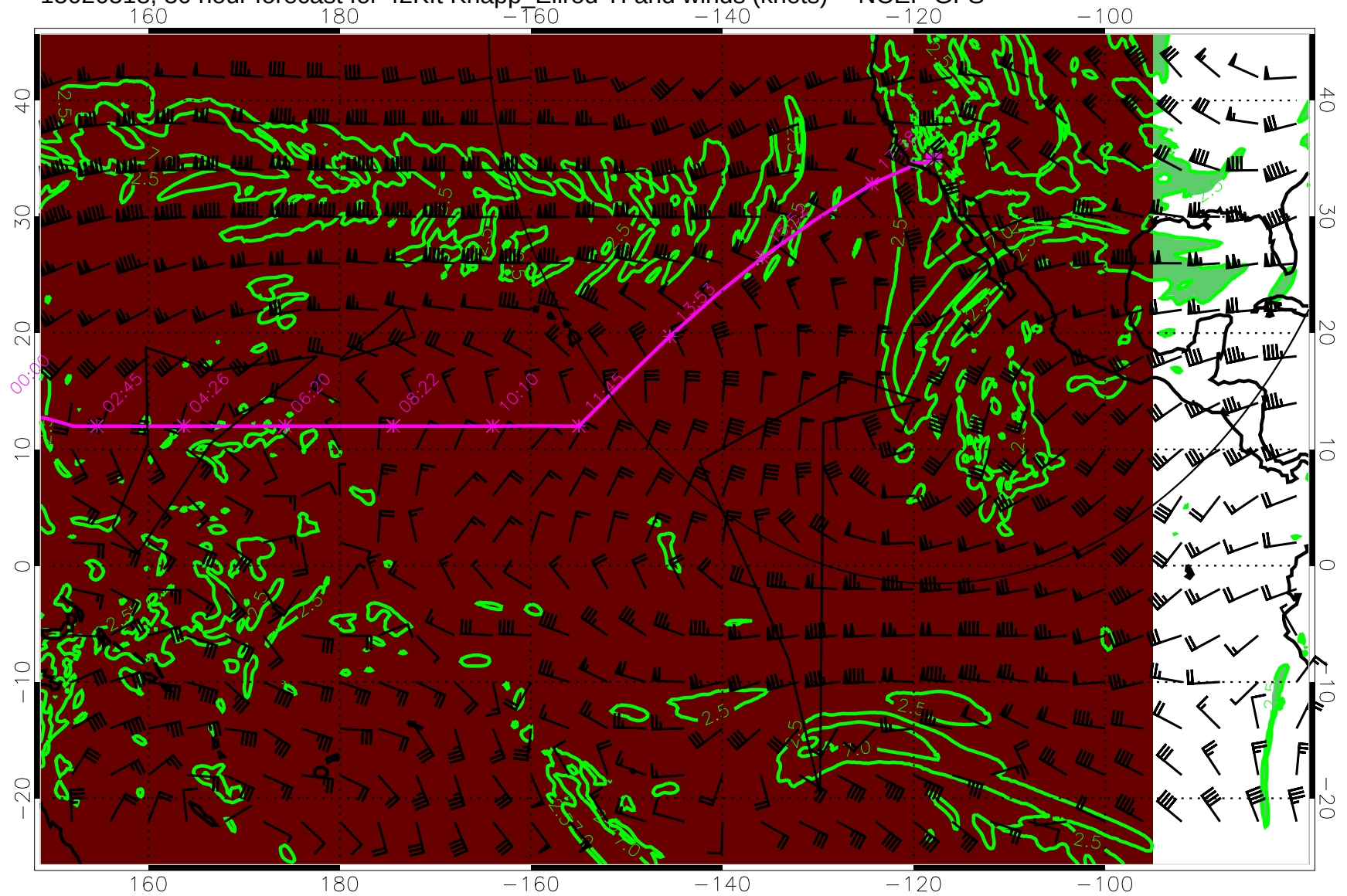
15020518, 30 hour forecast for 42Kft Knapp_Ellrod TI and winds (knots) -- NCEP GFS
