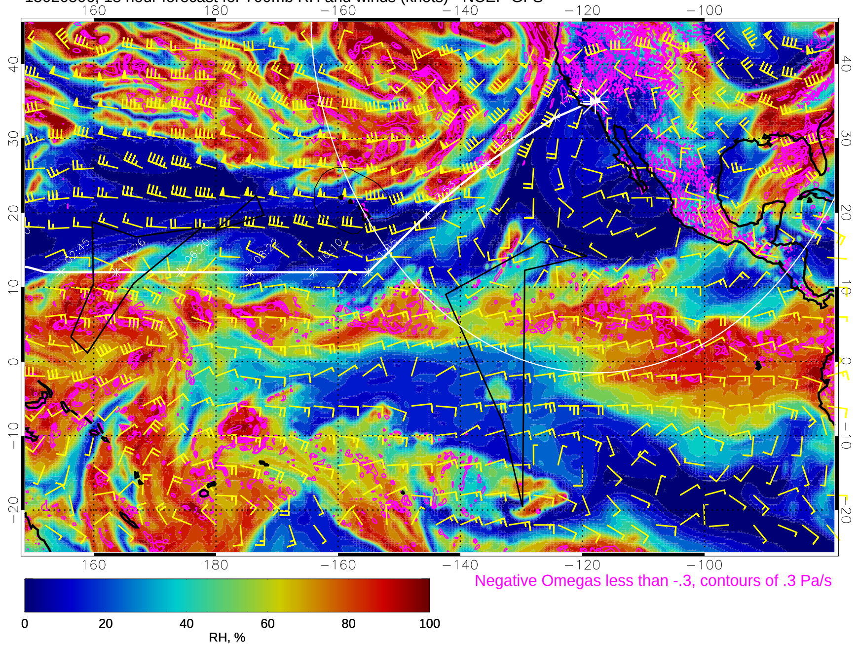
15020506, 18 hour forecast for 700mb RH and winds (knots) - NCEP GFS
