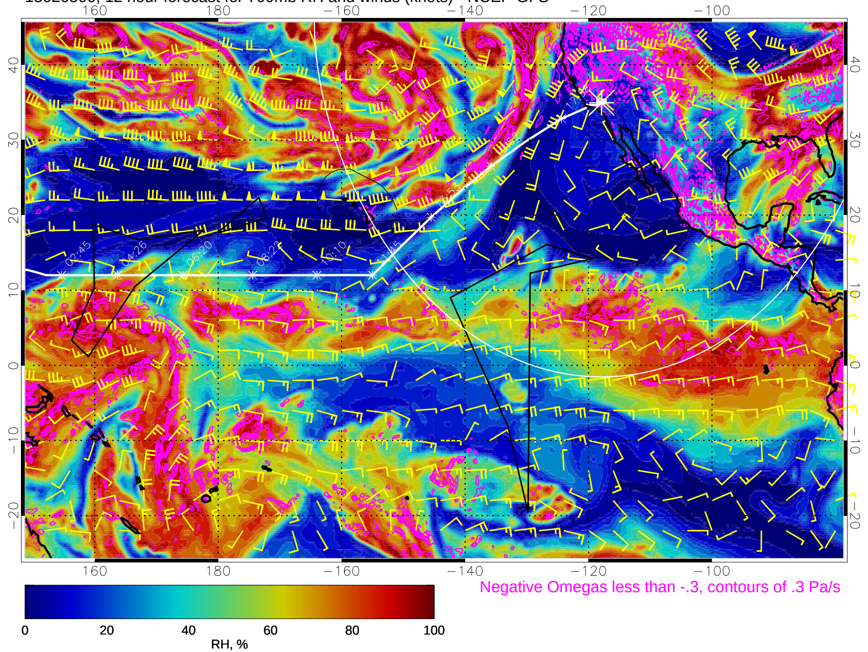
15020500, 12 hour forecast for 700mb RH and winds (knots) - NCEP GFS
