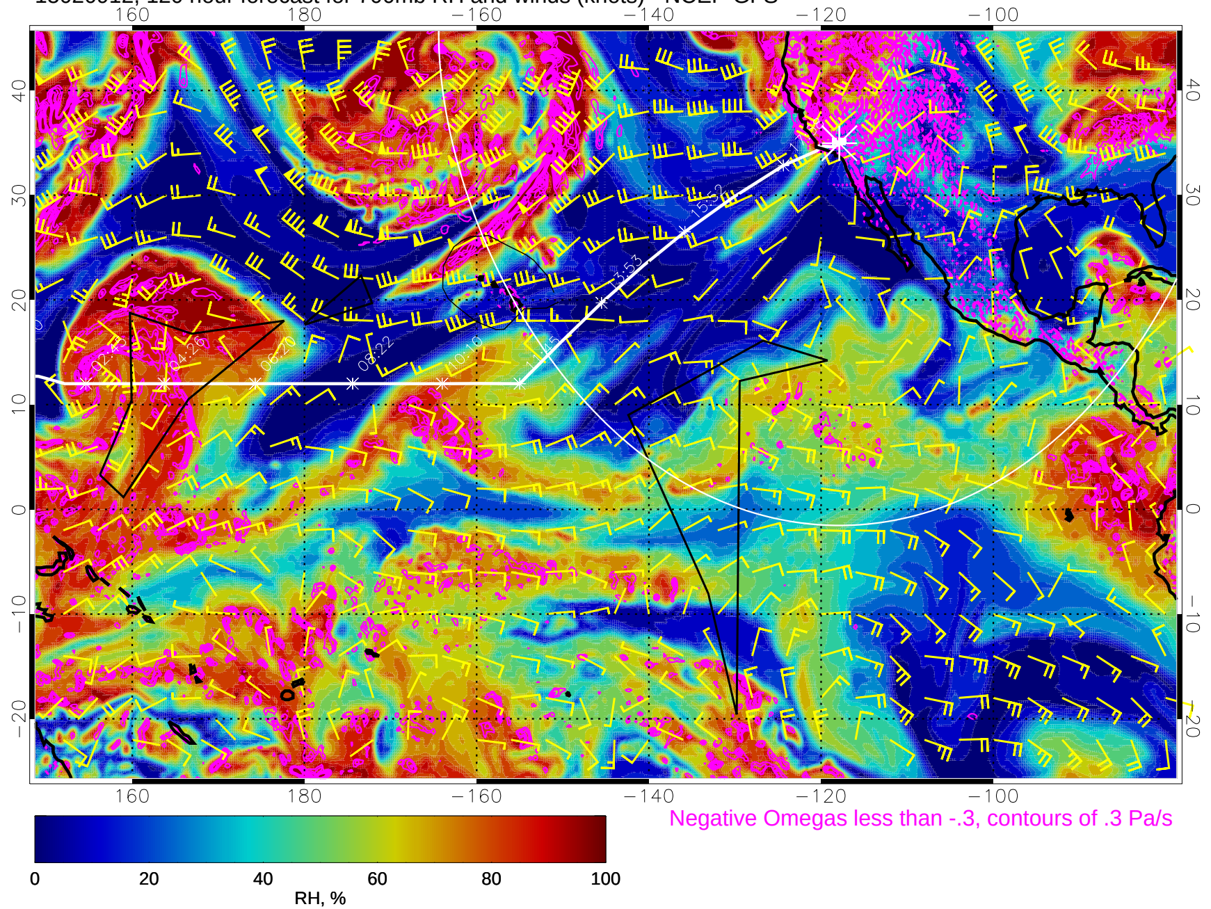
15020912, 120 hour forecast for 700mb RH and winds (knots) - NCEP GFS
