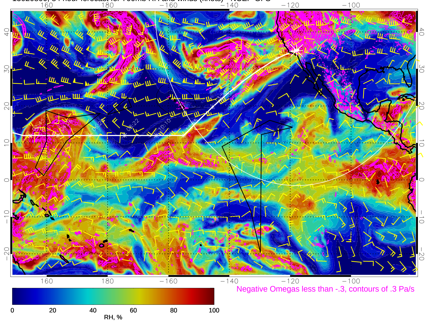
15020800, 84 hour forecast for 700mb RH and winds (knots) - NCEP GFS
