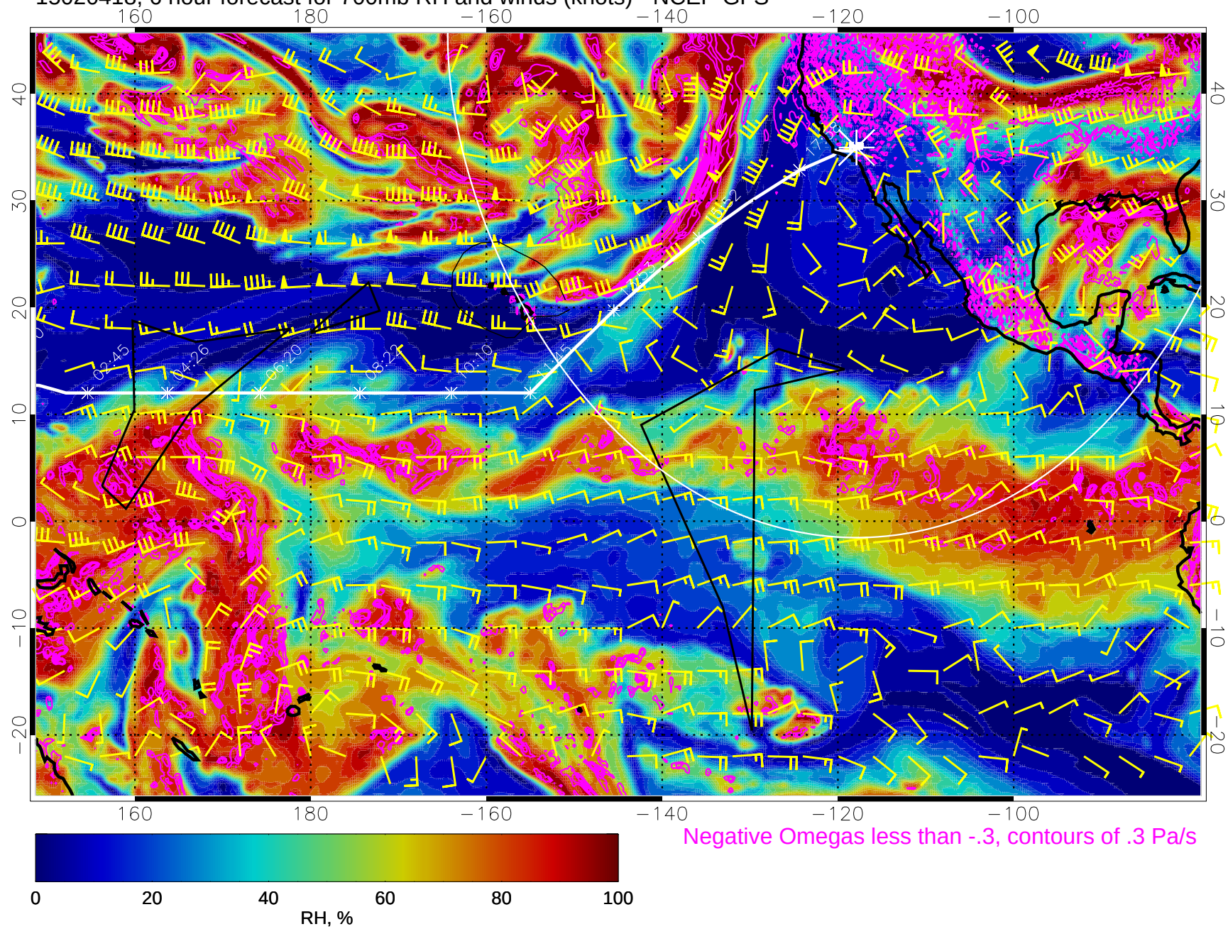
15020418, 6 hour forecast for 700mb RH and winds (knots) - NCEP GFS
