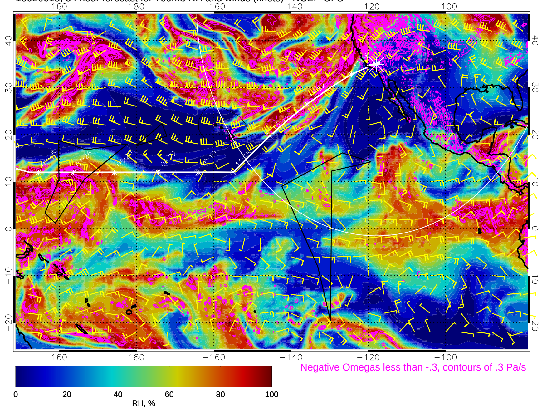
15020618, 54 hour forecast for 700mb RH and winds (knots) - NCEP GFS
