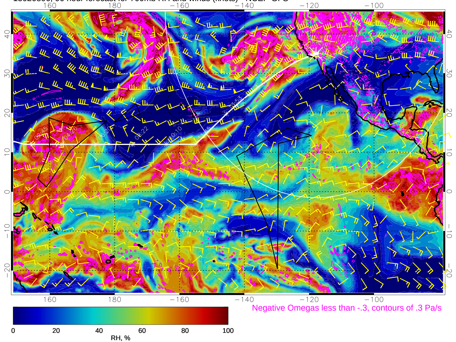
15020806, 90 hour forecast for 700mb RH and winds (knots) - NCEP GFS
