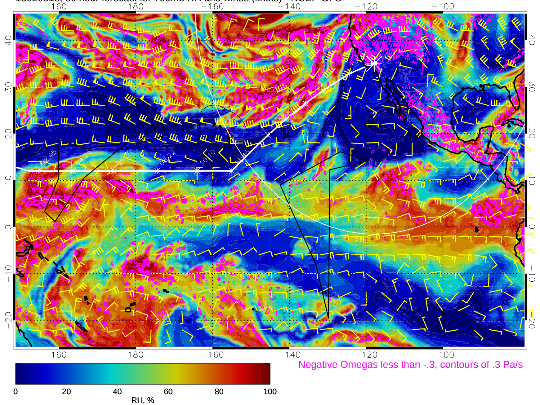
15020518, 30 hour forecast for 700mb RH and winds (knots) - NCEP GFS
