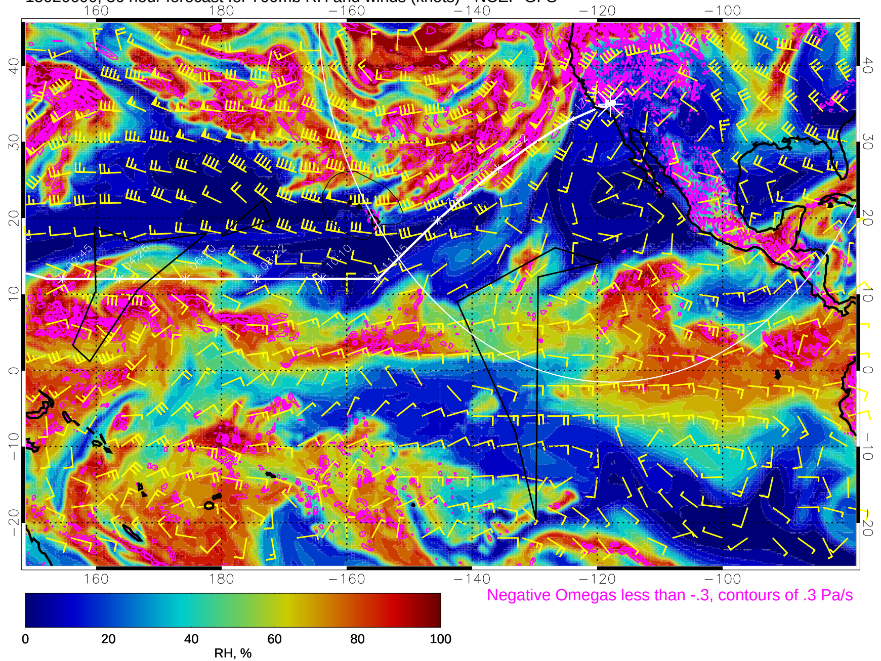
15020600, 36 hour forecast for 700mb RH and winds (knots) - NCEP GFS
