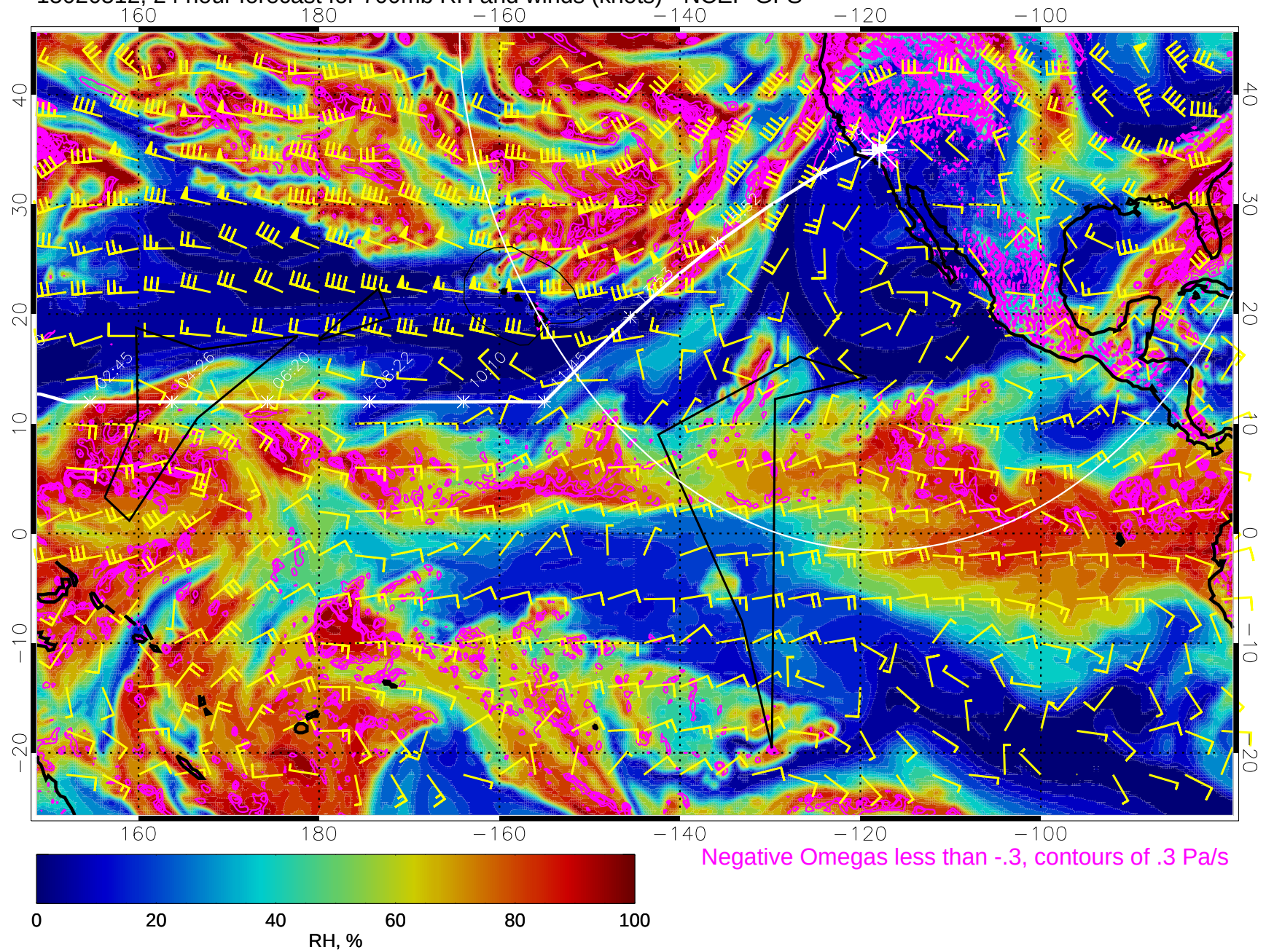
15020512, 24 hour forecast for 700mb RH and winds (knots) - NCEP GFS
