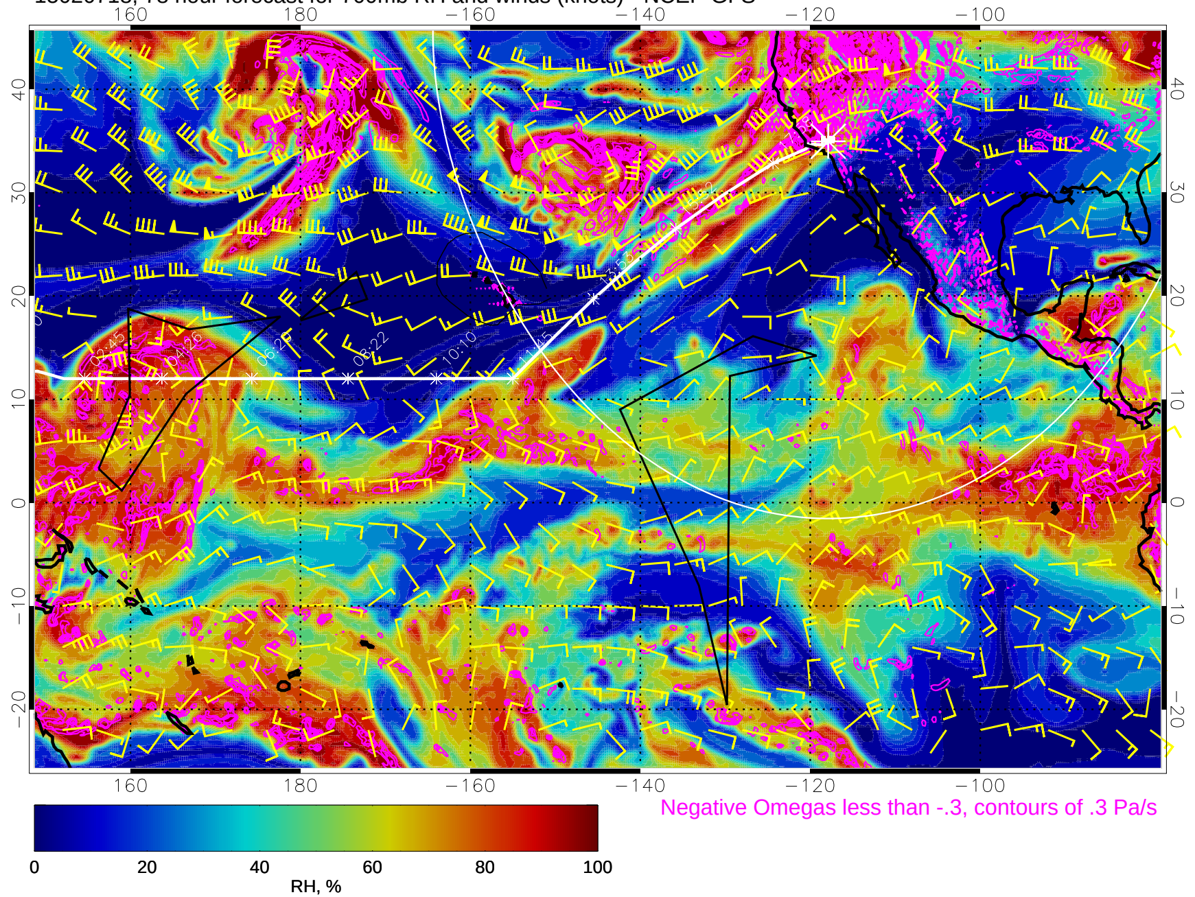
15020718, 78 hour forecast for 700mb RH and winds (knots) - NCEP GFS
