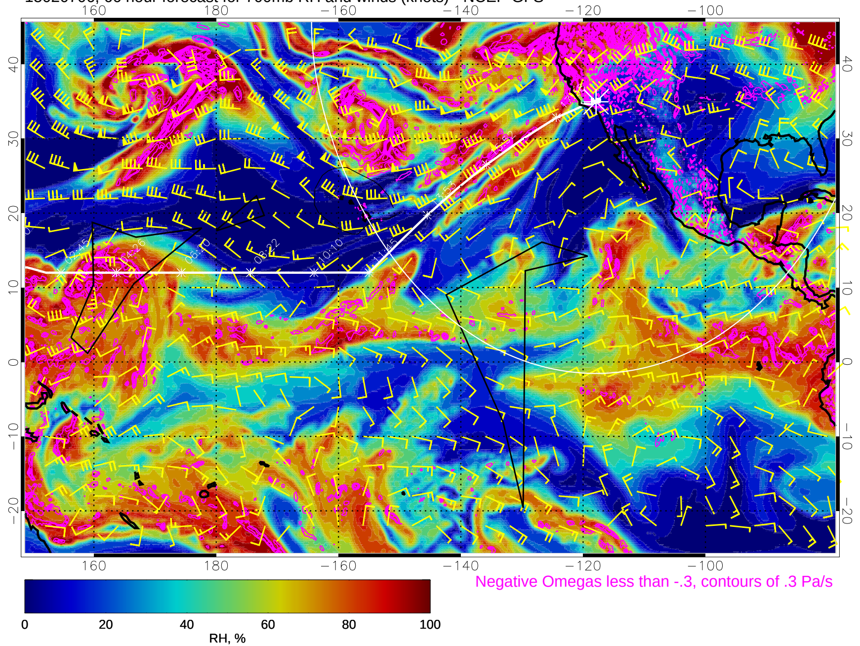
15020706, 66 hour forecast for 700mb RH and winds (knots) - NCEP GFS
