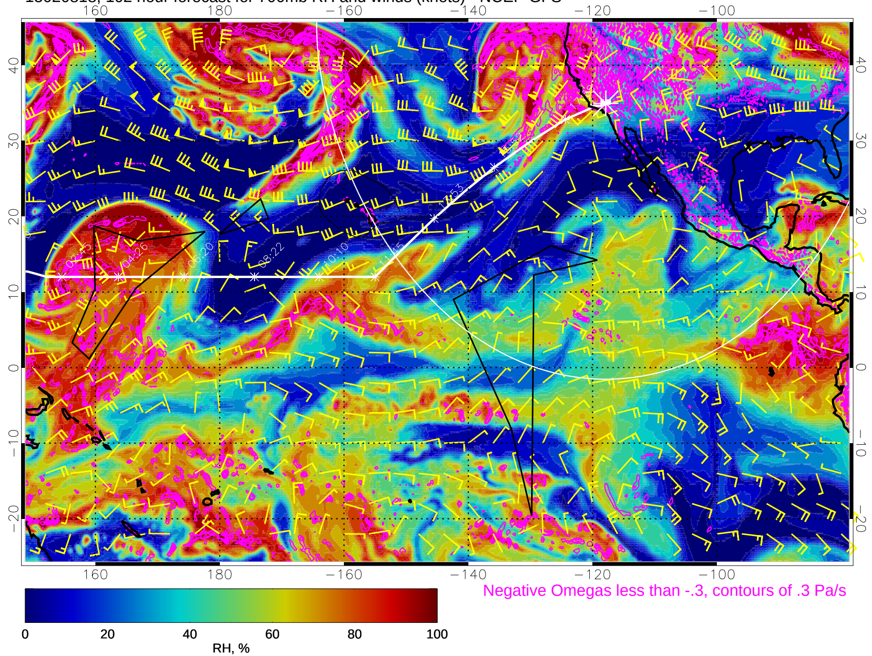
15020818, 102 hour forecast for 700mb RH and winds (knots) - NCEP GFS
