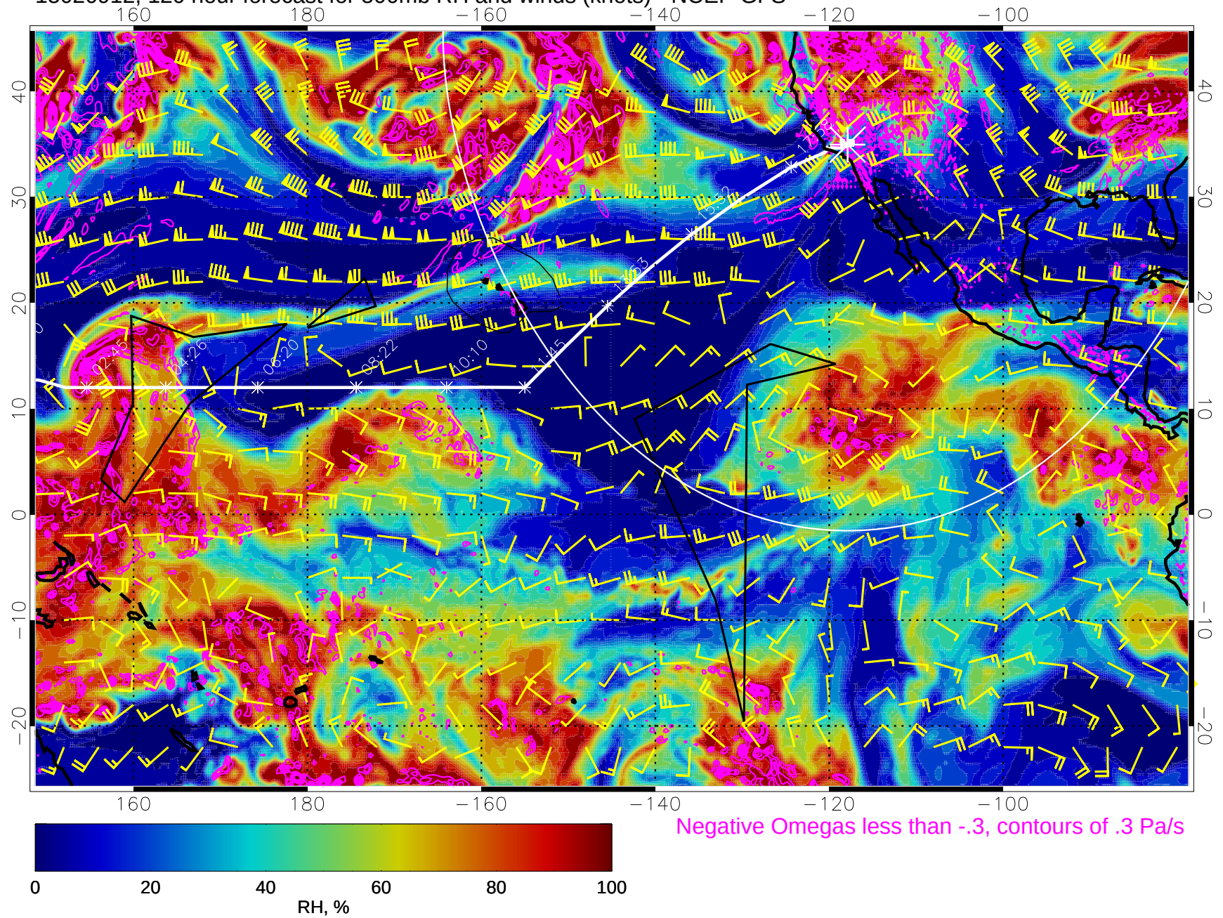
15020912, 120 hour forecast for 500mb RH and winds (knots) - NCEP GFS
