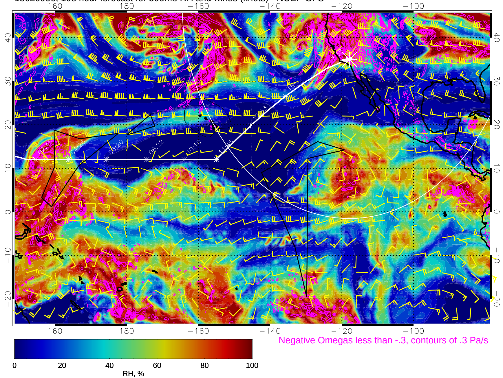
15020900, 108 hour forecast for 500mb RH and winds (knots) - NCEP GFS
