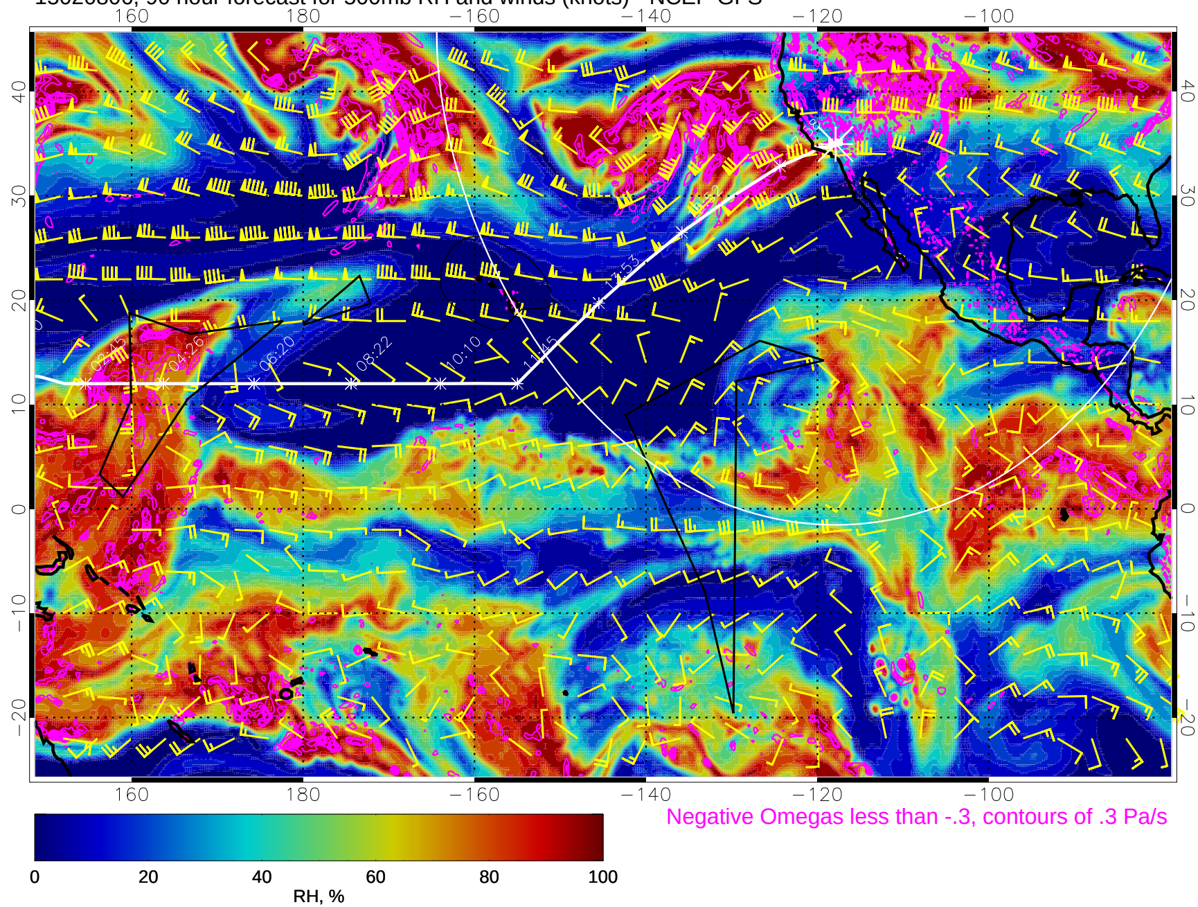
15020806, 90 hour forecast for 500mb RH and winds (knots) - NCEP GFS
