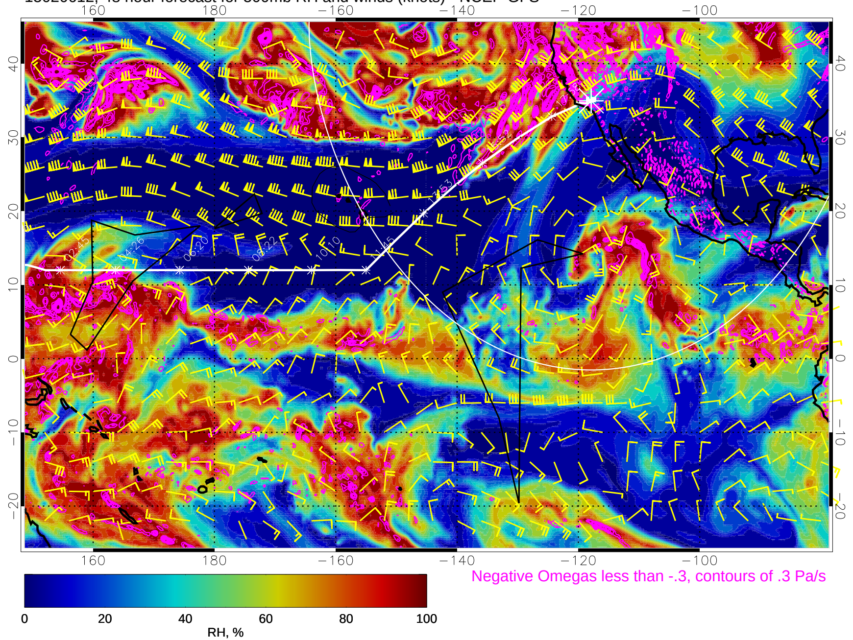
15020612, 48 hour forecast for 500mb RH and winds (knots) - NCEP GFS
