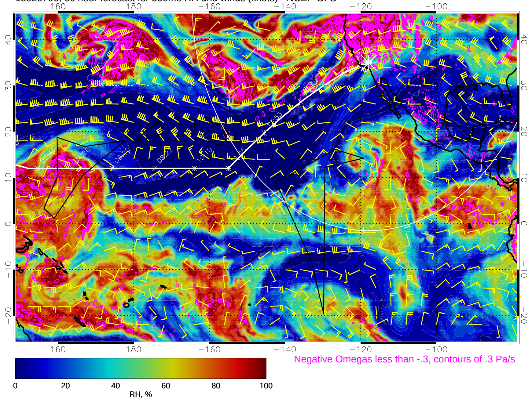
15020706, 66 hour forecast for 500mb RH and winds (knots) - NCEP GFS
