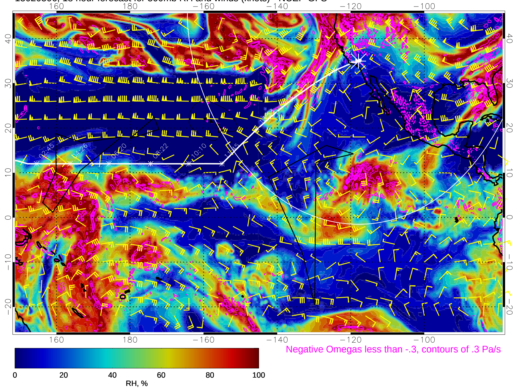
15020506, 18 hour forecast for 500mb RH and winds (knots) - NCEP GFS
