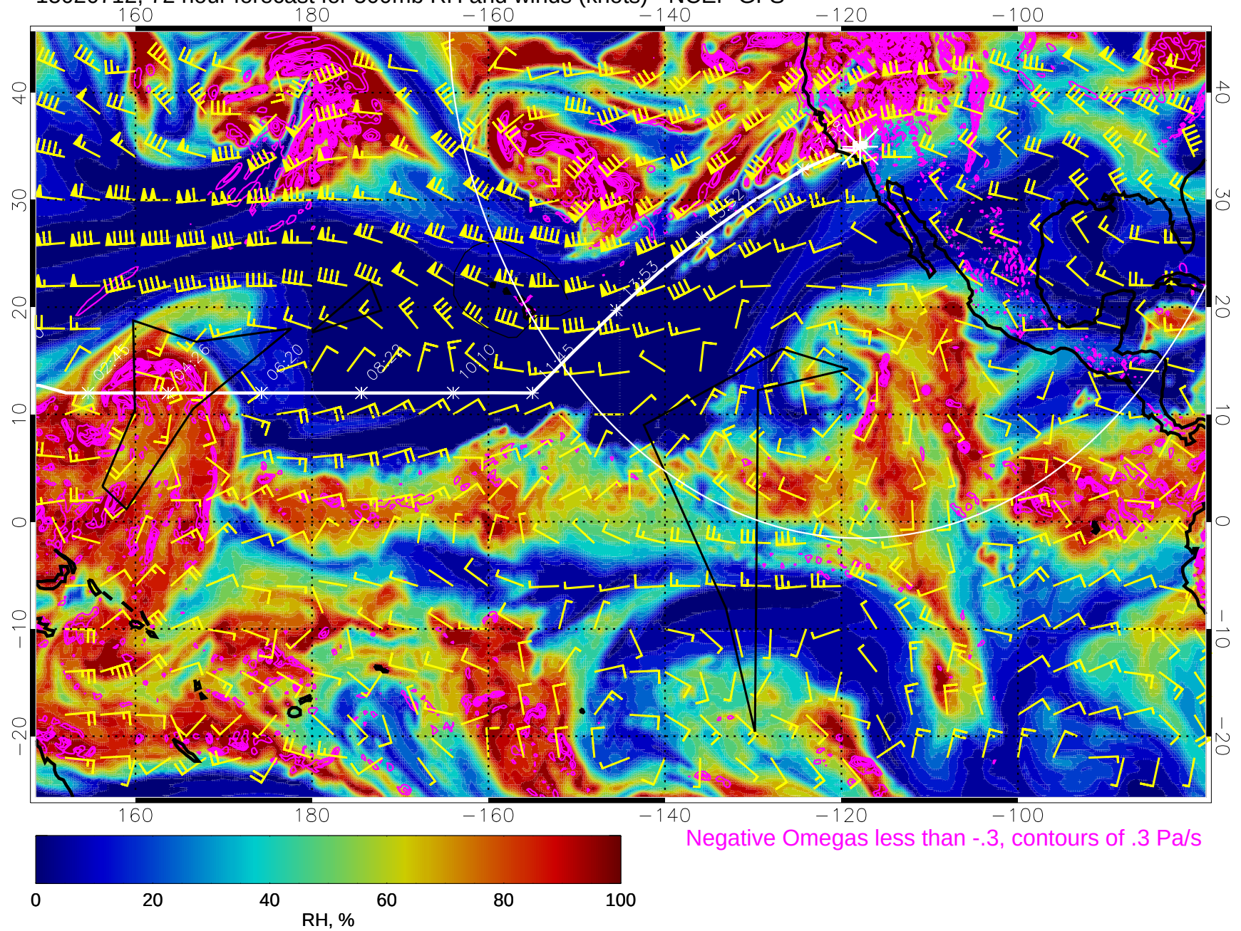
15020712, 72 hour forecast for 500mb RH and winds (knots) - NCEP GFS
