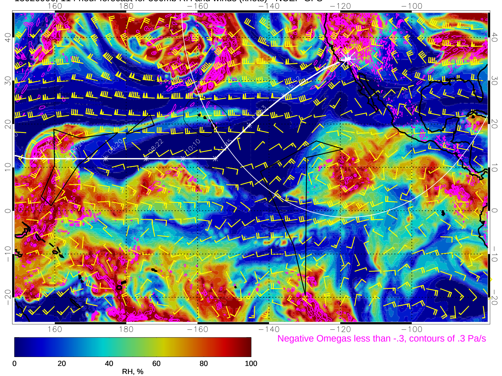
15020906, 114 hour forecast for 500mb RH and winds (knots) - NCEP GFS
