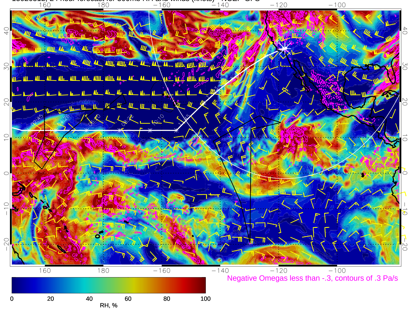
15020512, 24 hour forecast for 500mb RH and winds (knots) - NCEP GFS
