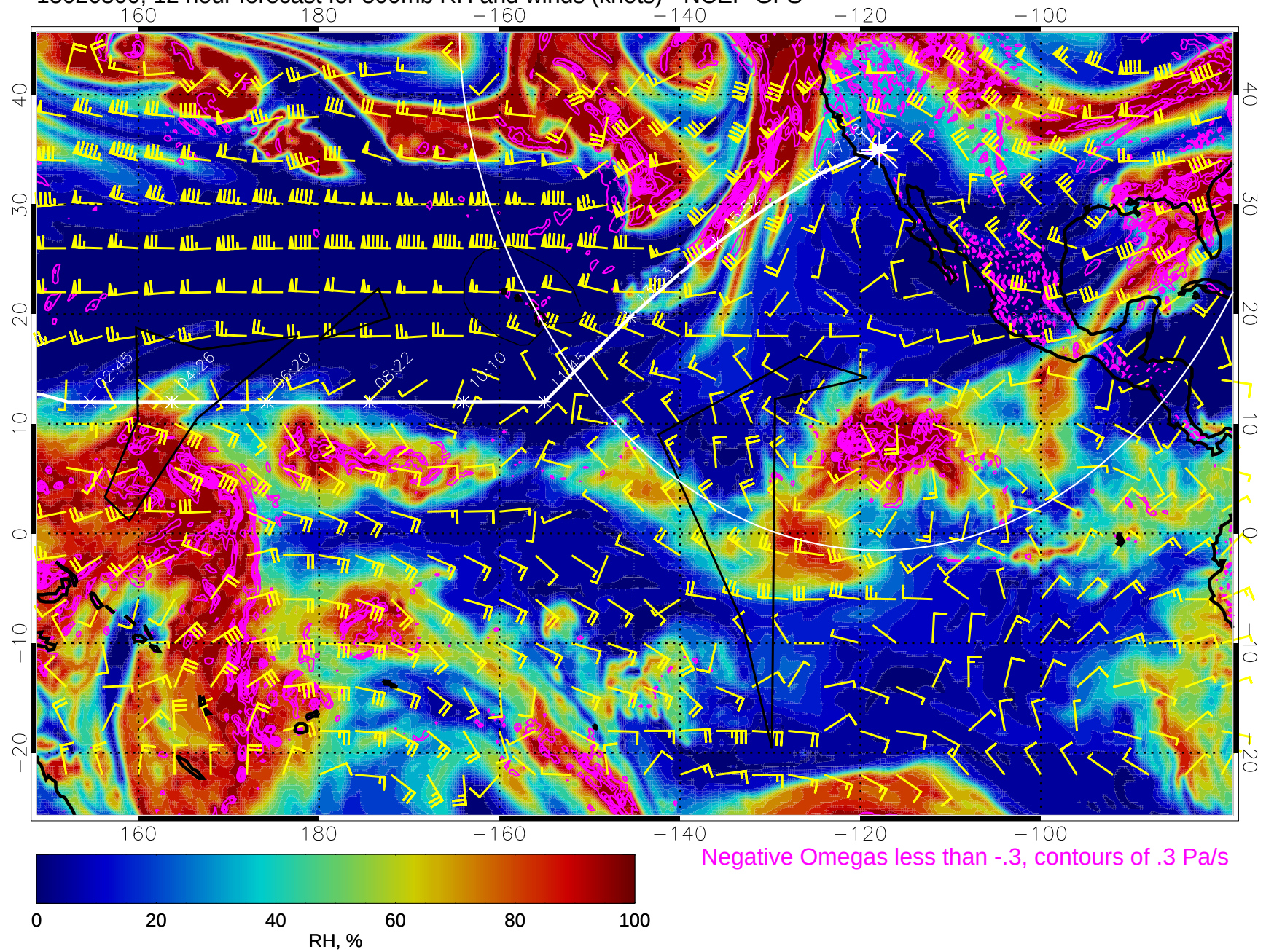
15020500, 12 hour forecast for 500mb RH and winds (knots) - NCEP GFS
