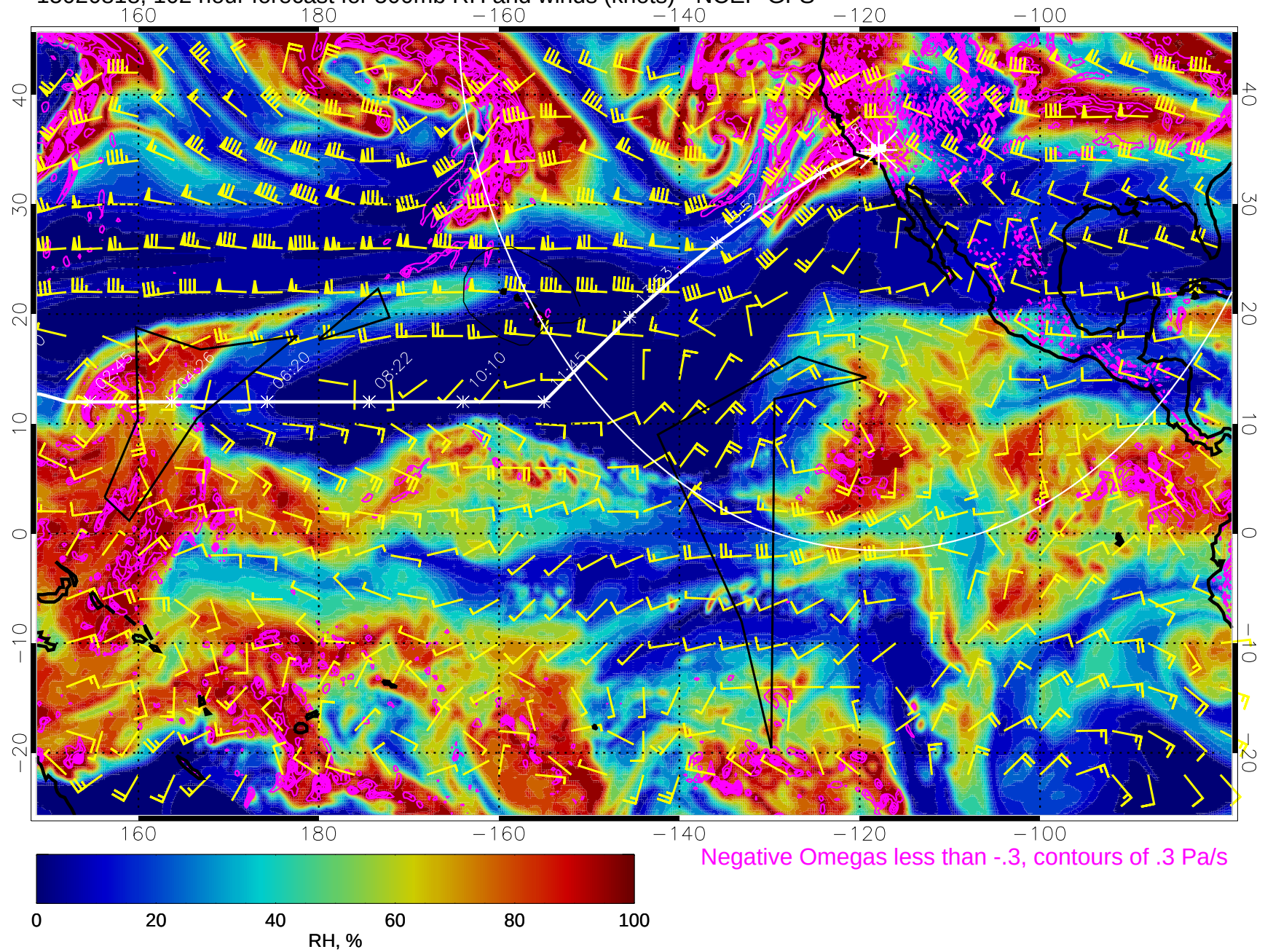
15020818, 102 hour forecast for 500mb RH and winds (knots) - NCEP GFS
