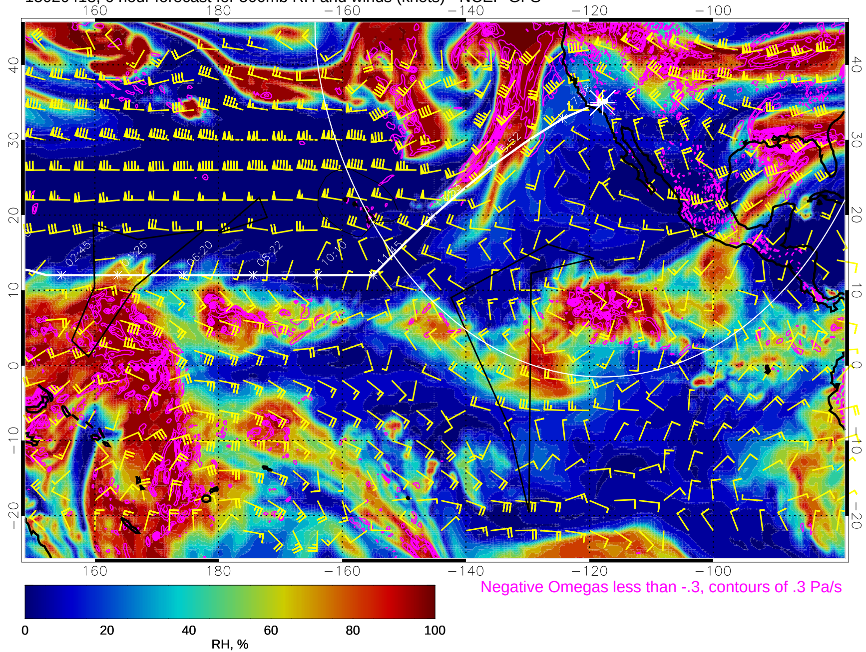
15020418, 6 hour forecast for 500mb RH and winds (knots) - NCEP GFS
