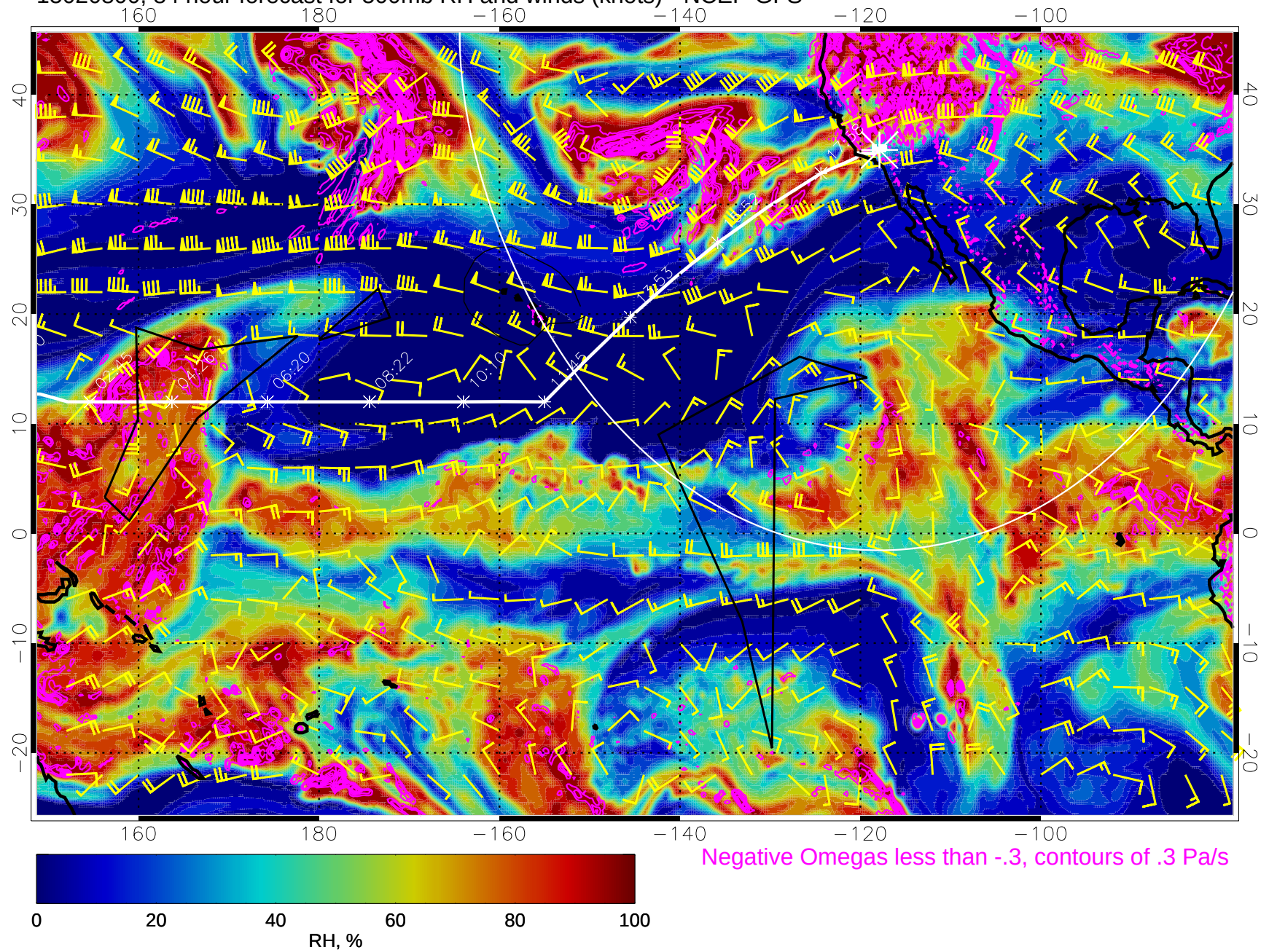
15020800, 84 hour forecast for 500mb RH and winds (knots) - NCEP GFS
