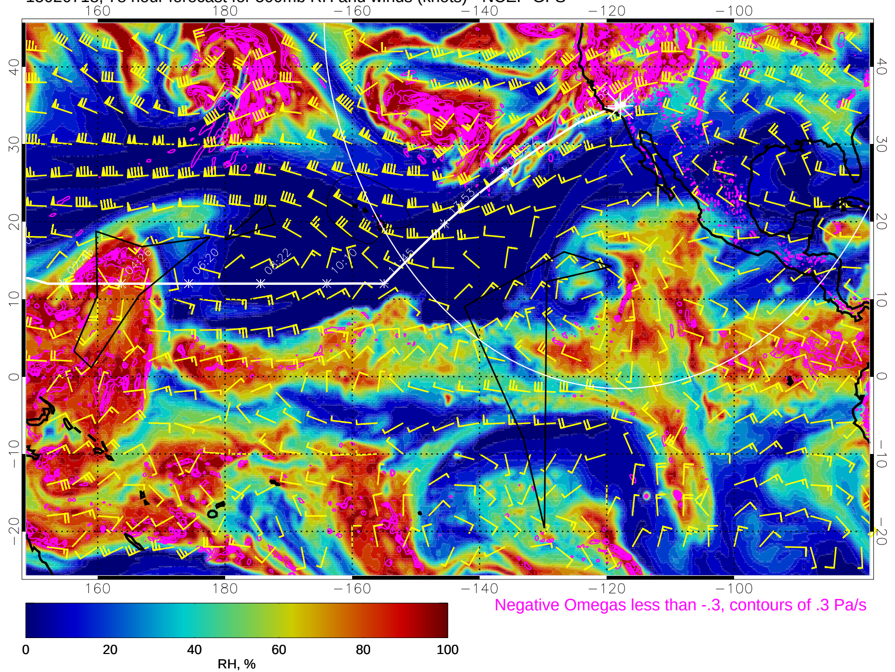
15020718, 78 hour forecast for 500mb RH and winds (knots) - NCEP GFS
