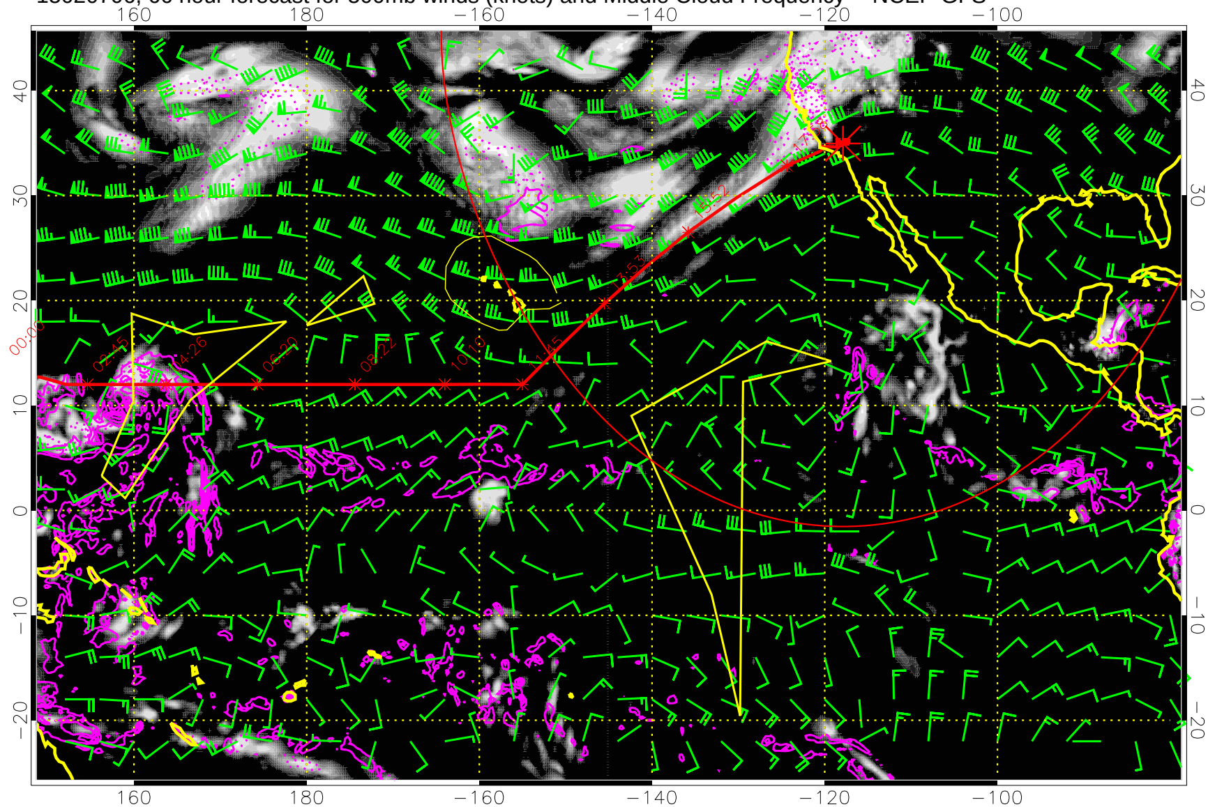
15020706, 66 hour forecast for 500mb winds (knots) and Middle Cloud Frequency -- NCEP GFS
