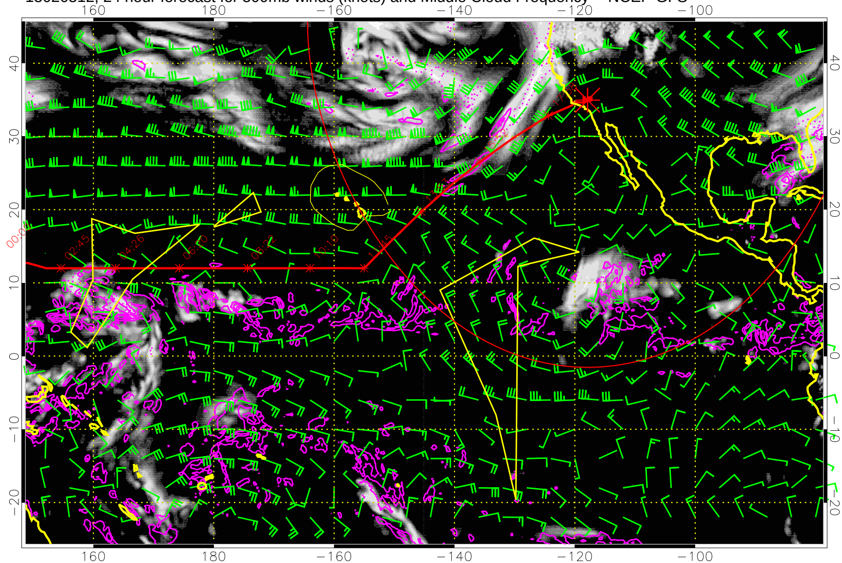
15020512, 24 hour forecast for 500mb winds (knots) and Middle Cloud Frequency -- NCEP GFS
