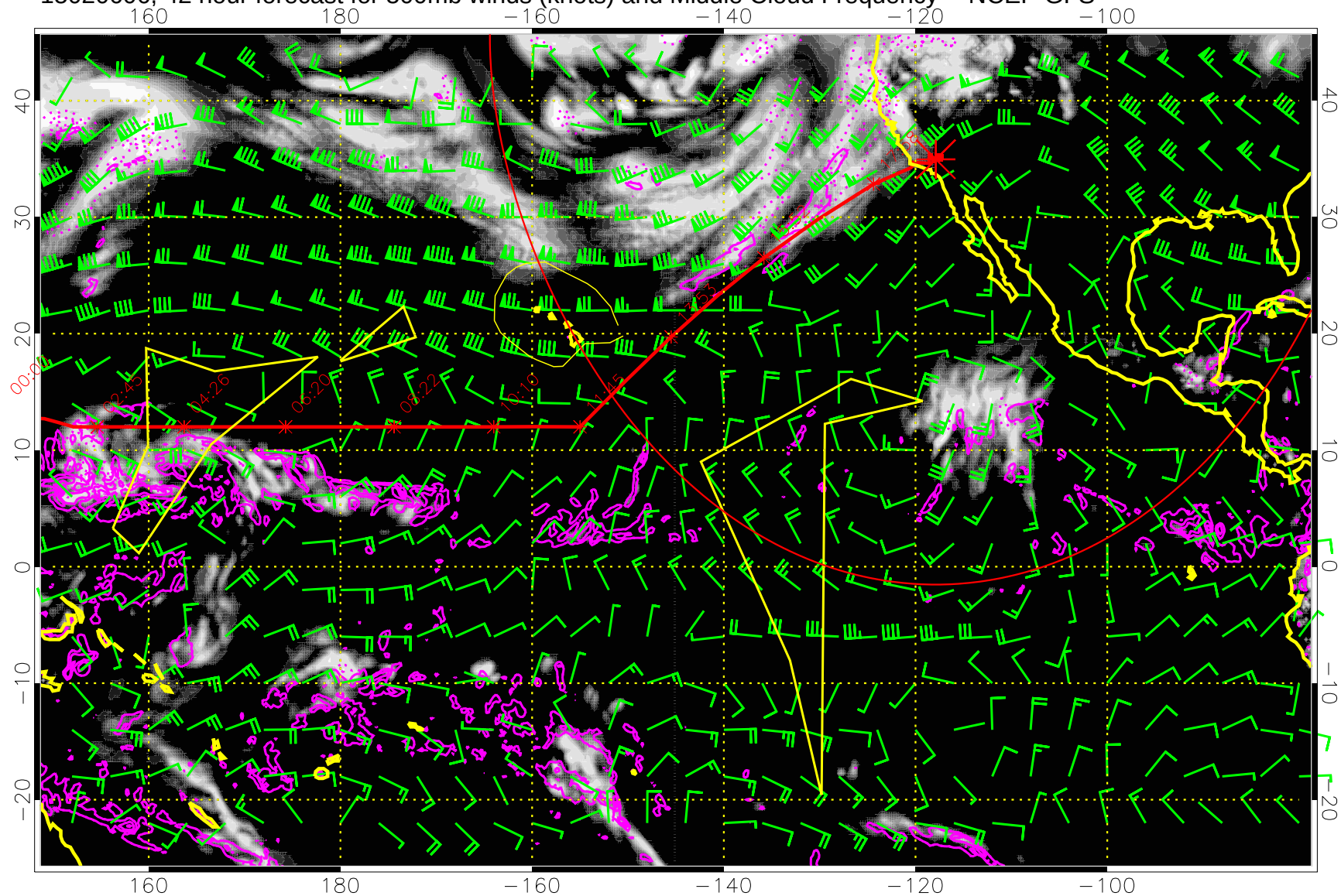
15020606, 42 hour forecast for 500mb winds (knots) and Middle Cloud Frequency -- NCEP GFS
