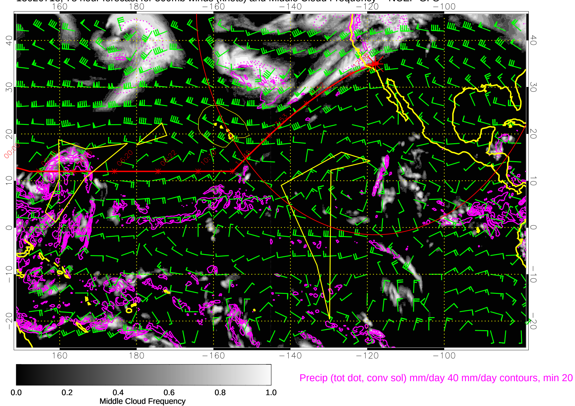
15020718, 78 hour forecast for 500mb winds (knots) and Middle Cloud Frequency -- NCEP GFS
