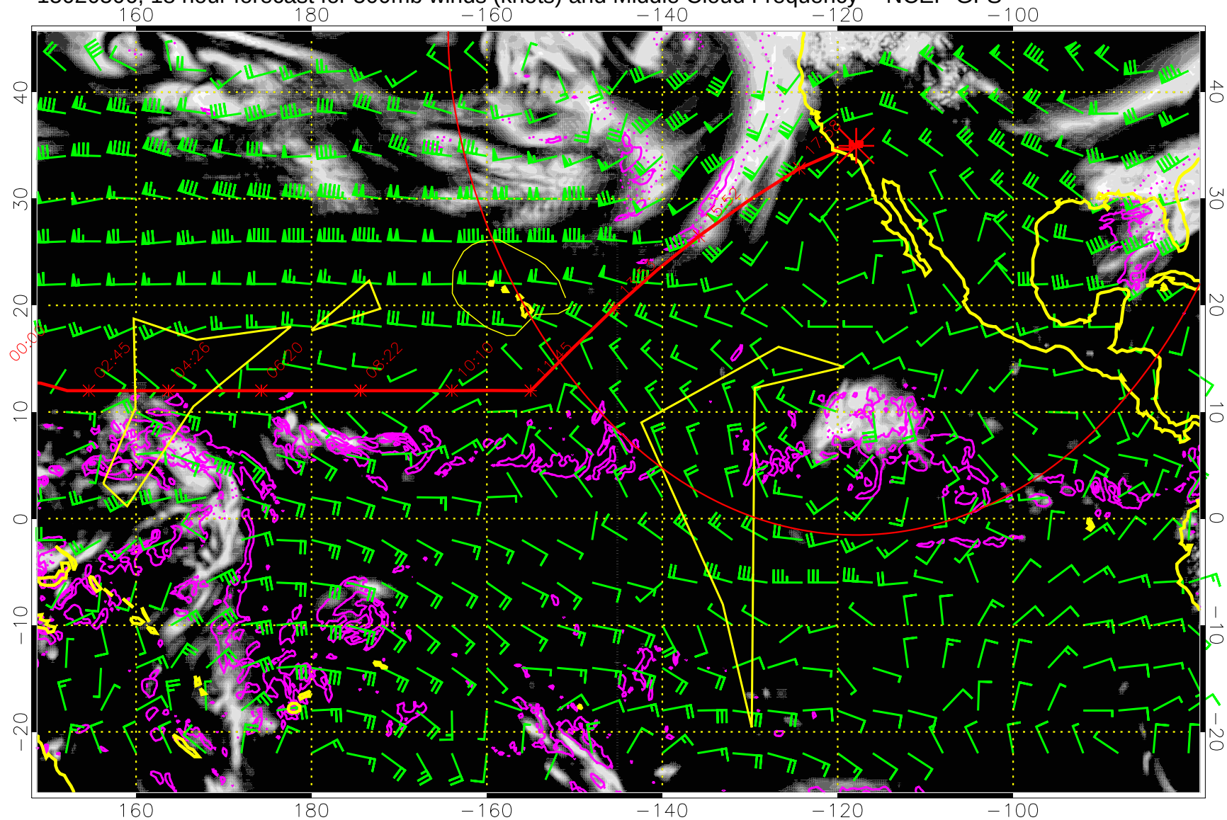
15020506, 18 hour forecast for 500mb winds (knots) and Middle Cloud Frequency -- NCEP GFS
