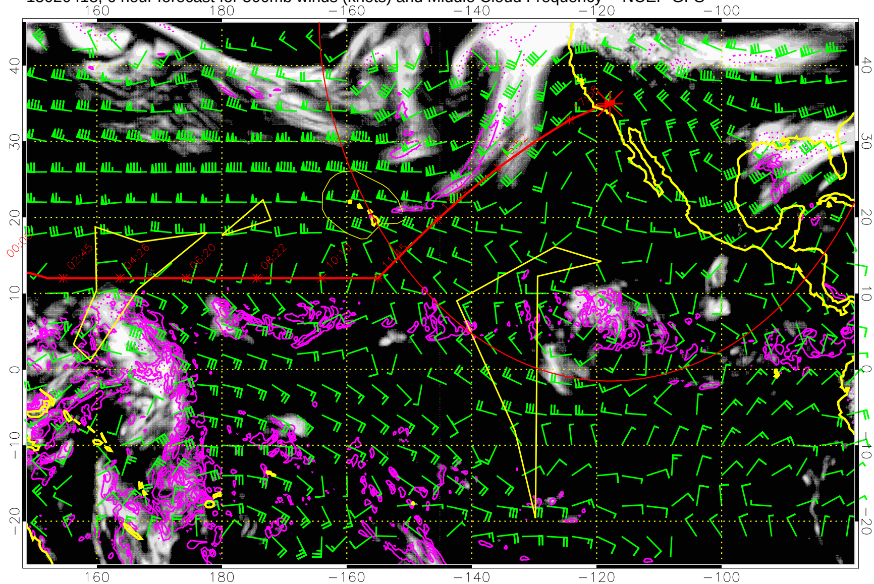
15020418, 6 hour forecast for 500mb winds (knots) and Middle Cloud Frequency -- NCEP GFS
