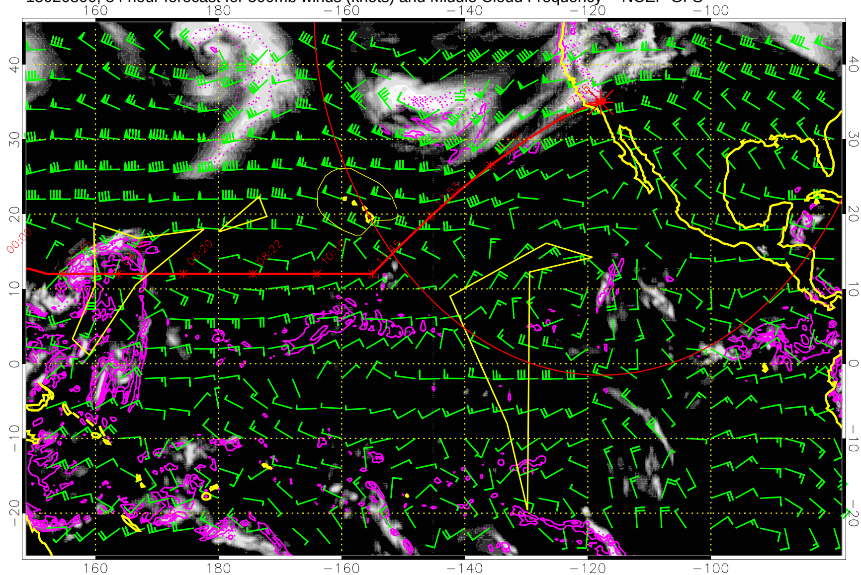
15020800, 84 hour forecast for 500mb winds (knots) and Middle Cloud Frequency -- NCEP GFS
