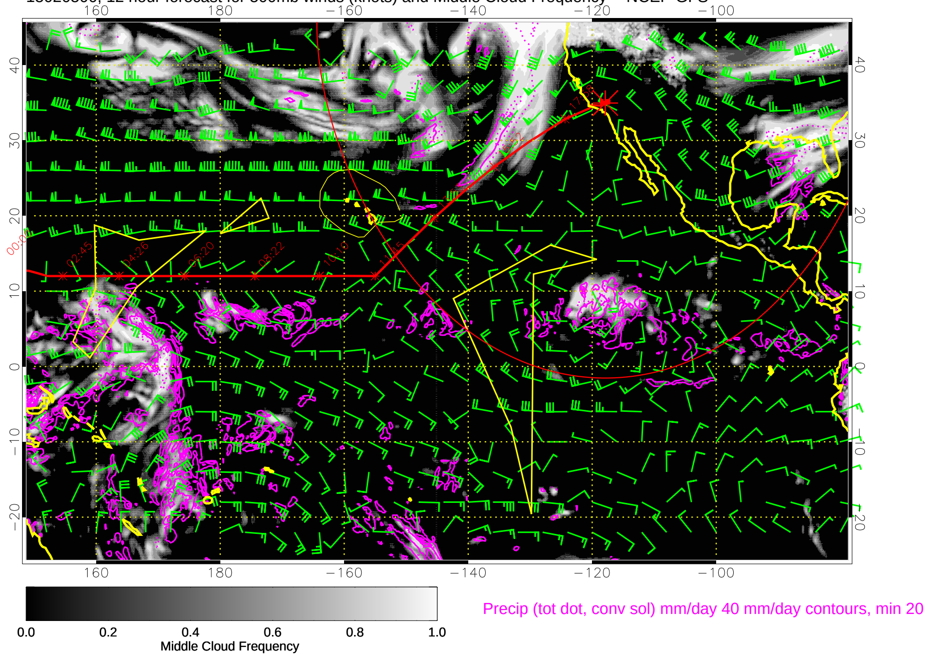
15020500, 12 hour forecast for 500mb winds (knots) and Middle Cloud Frequency -- NCEP GFS
