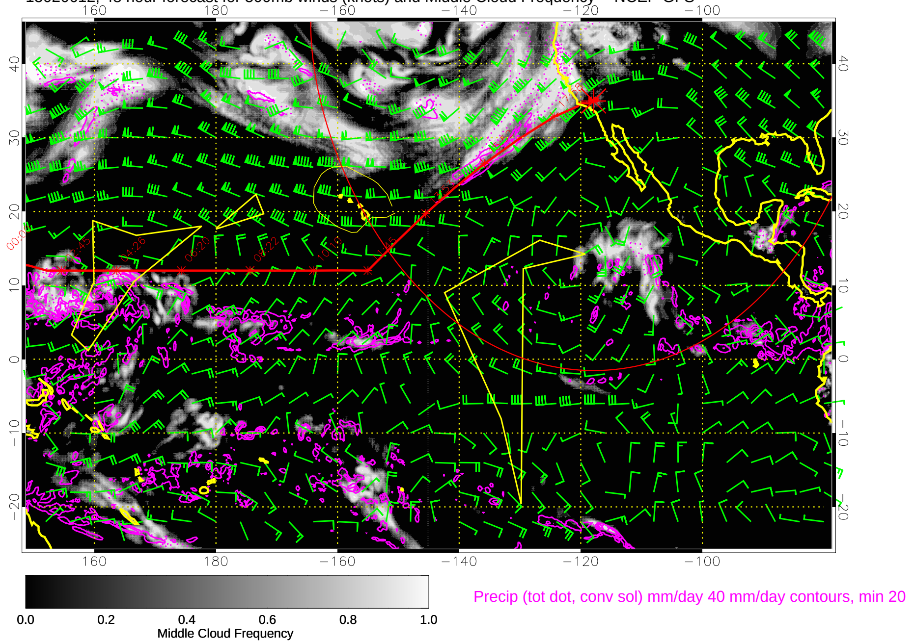
15020612, 48 hour forecast for 500mb winds (knots) and Middle Cloud Frequency -- NCEP GFS
