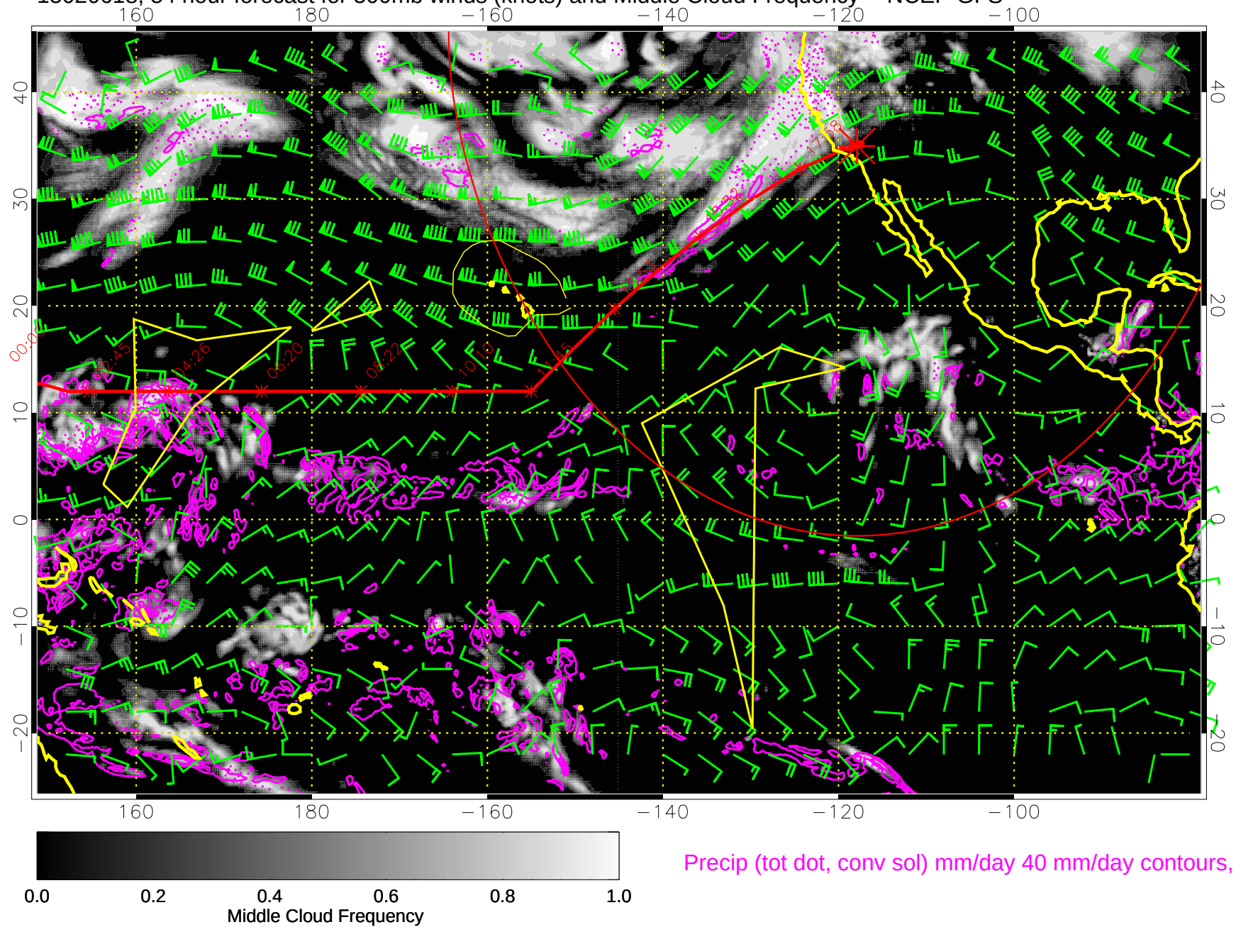
15020618, 54 hour forecast for 500mb winds (knots) and Middle Cloud Frequency -- NCEP GFS
