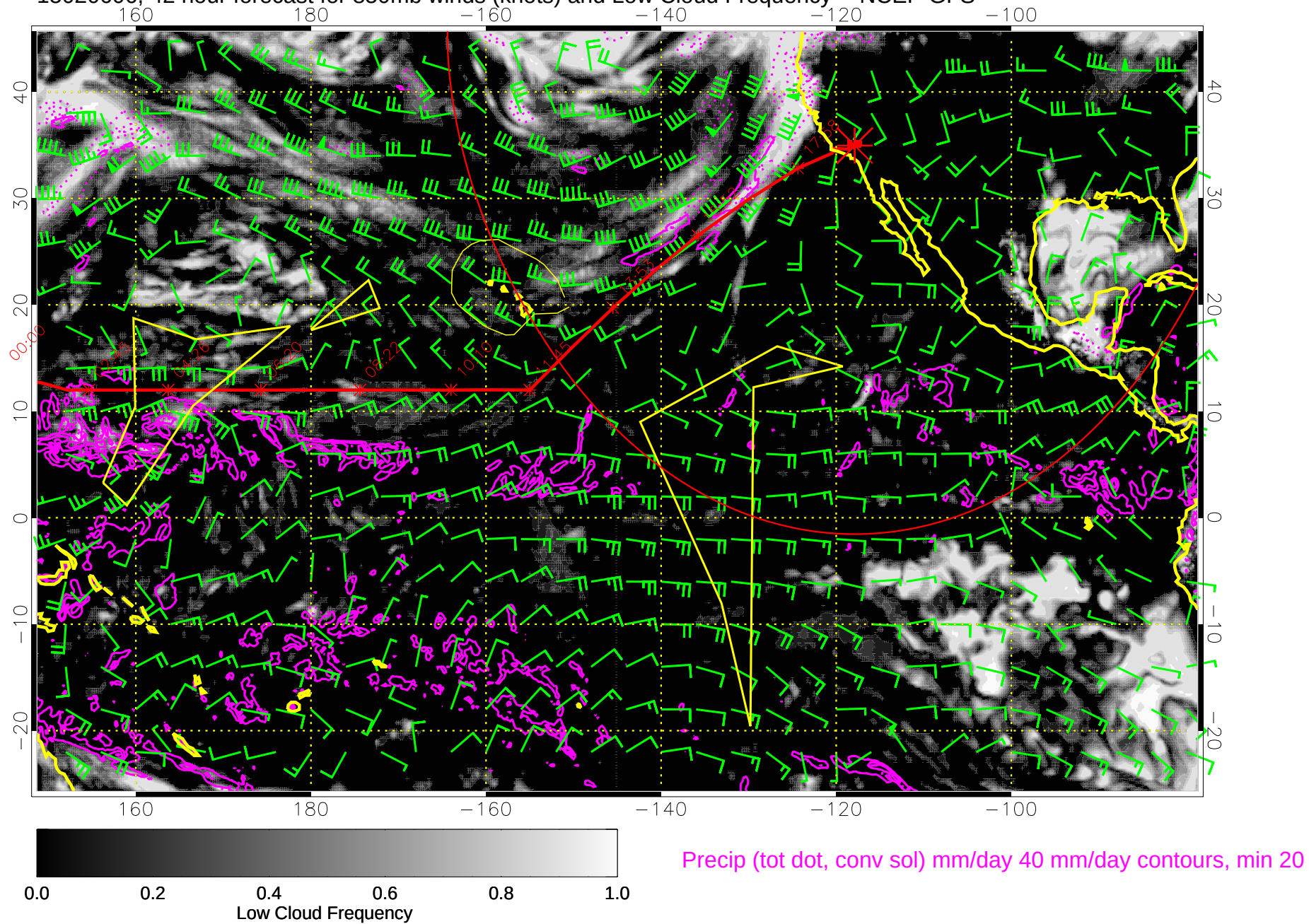
15020606, 42 hour forecast for 850mb winds (knots) and Low Cloud Frequency -- NCEP GFS
