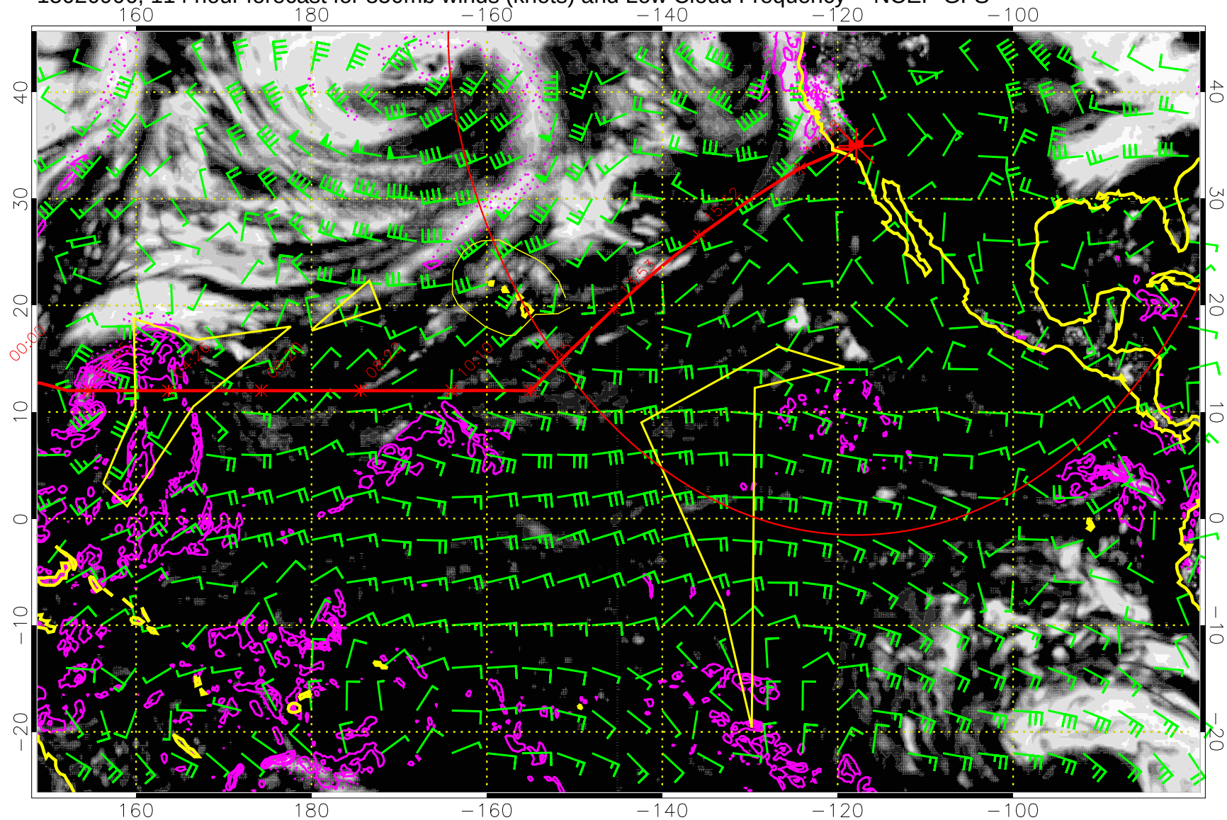
15020906, 114 hour forecast for 850mb winds (knots) and Low Cloud Frequency -- NCEP GFS
