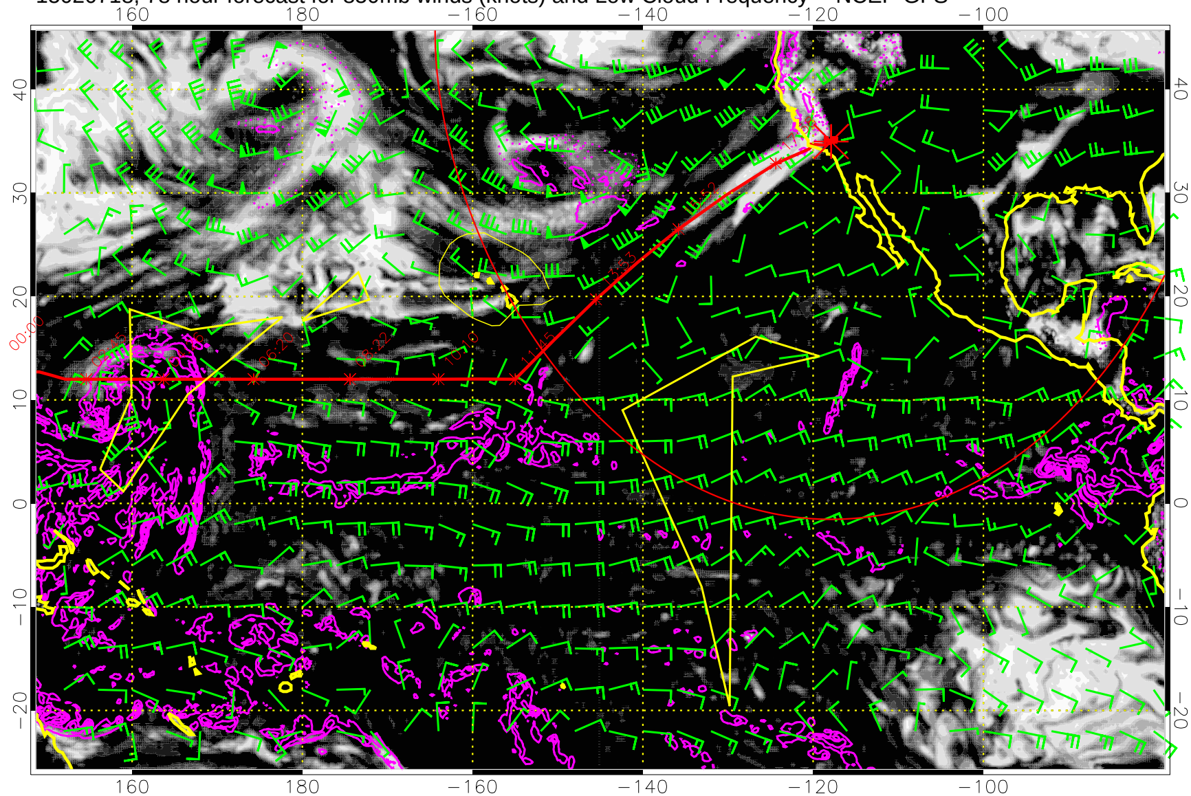
15020718, 78 hour forecast for 850mb winds (knots) and Low Cloud Frequency -- NCEP GFS
