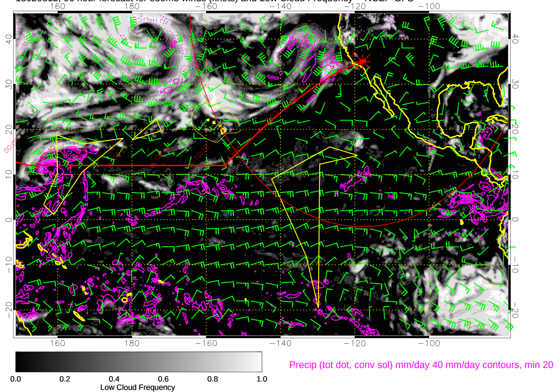
15020812, 96 hour forecast for 850mb winds (knots) and Low Cloud Frequency -- NCEP GFS
