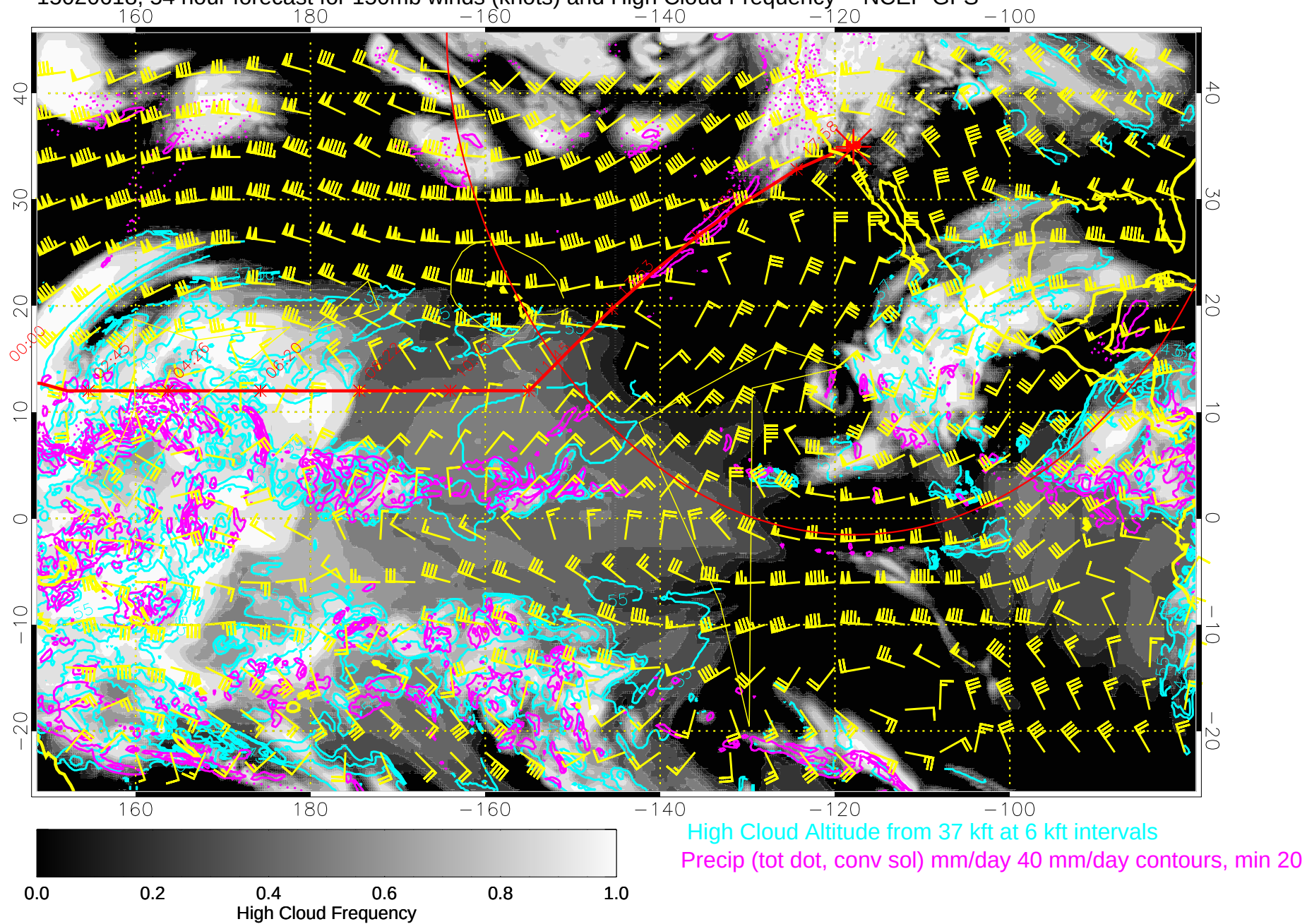
15020618, 54 hour forecast for 150mb winds (knots) and High Cloud Frequency -- NCEP GFS
