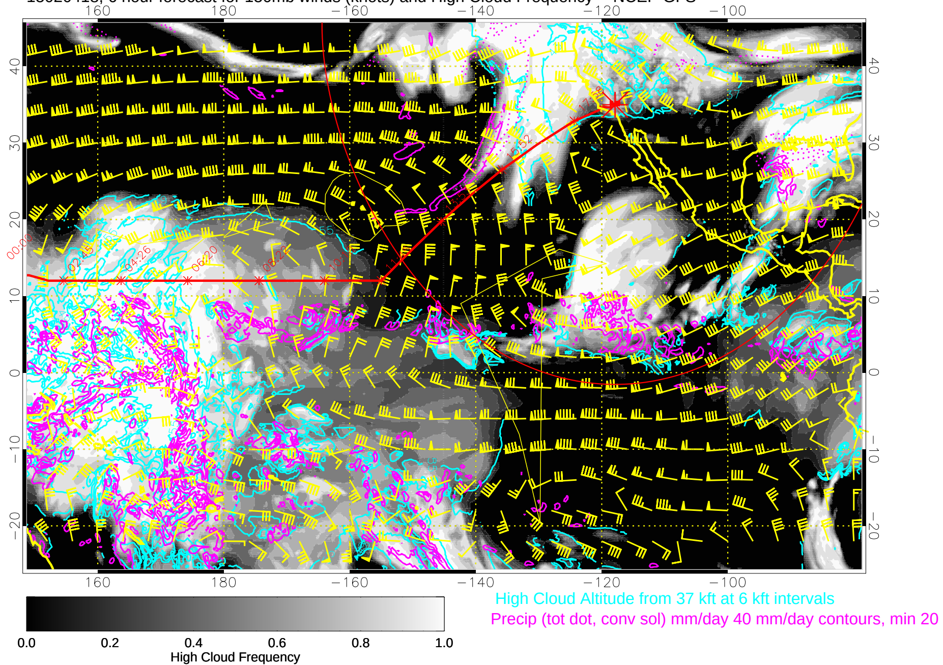
15020418, 6 hour forecast for 150mb winds (knots) and High Cloud Frequency -- NCEP GFS
