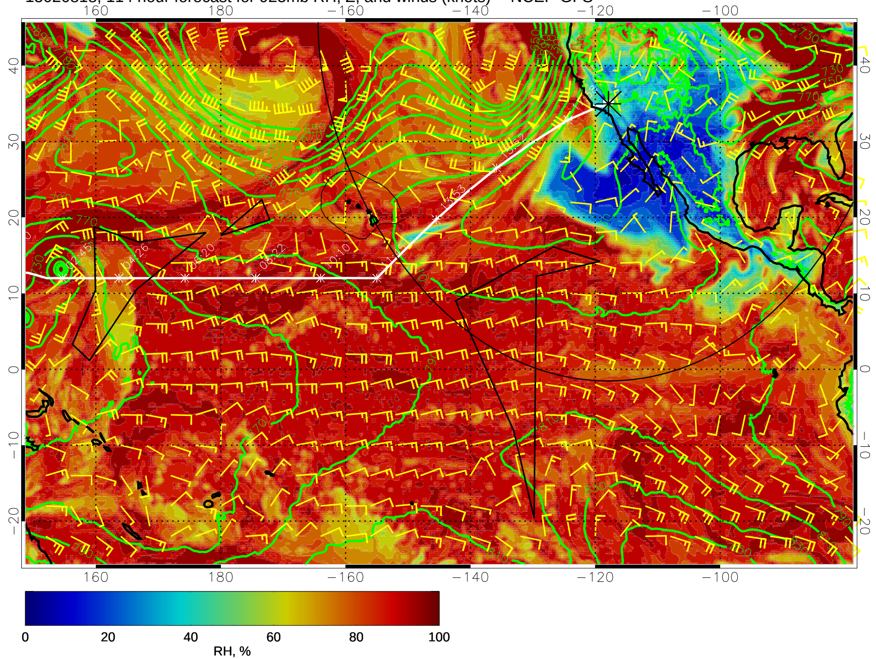
15020818, 114 hour forecast for 925mb RH, Z, and winds (knots) -- NCEP GFS
