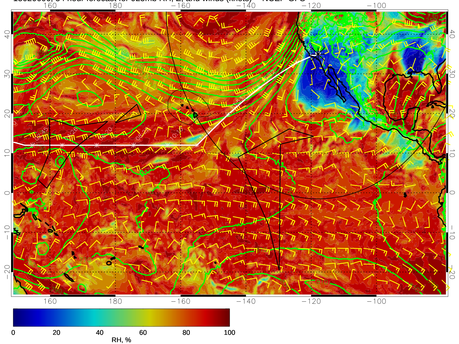
15020606, 54 hour forecast for 925mb RH, Z, and winds (knots) -- NCEP GFS
