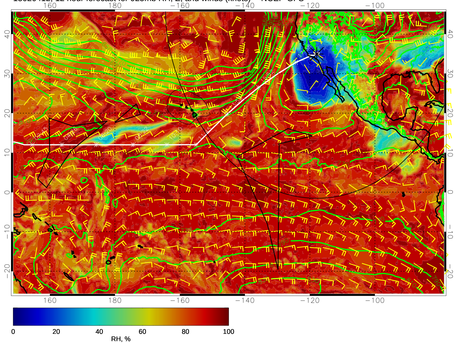
15020412, 12 hour forecast for 925mb RH, Z, and winds (knots) -- NCEP GFS
