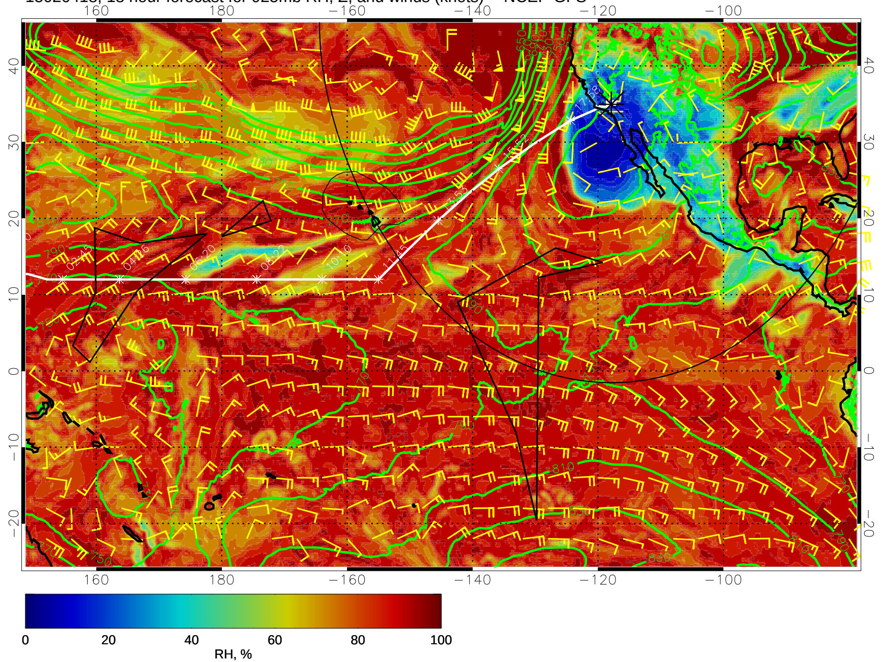
15020418, 18 hour forecast for 925mb RH, Z, and winds (knots) -- NCEP GFS
