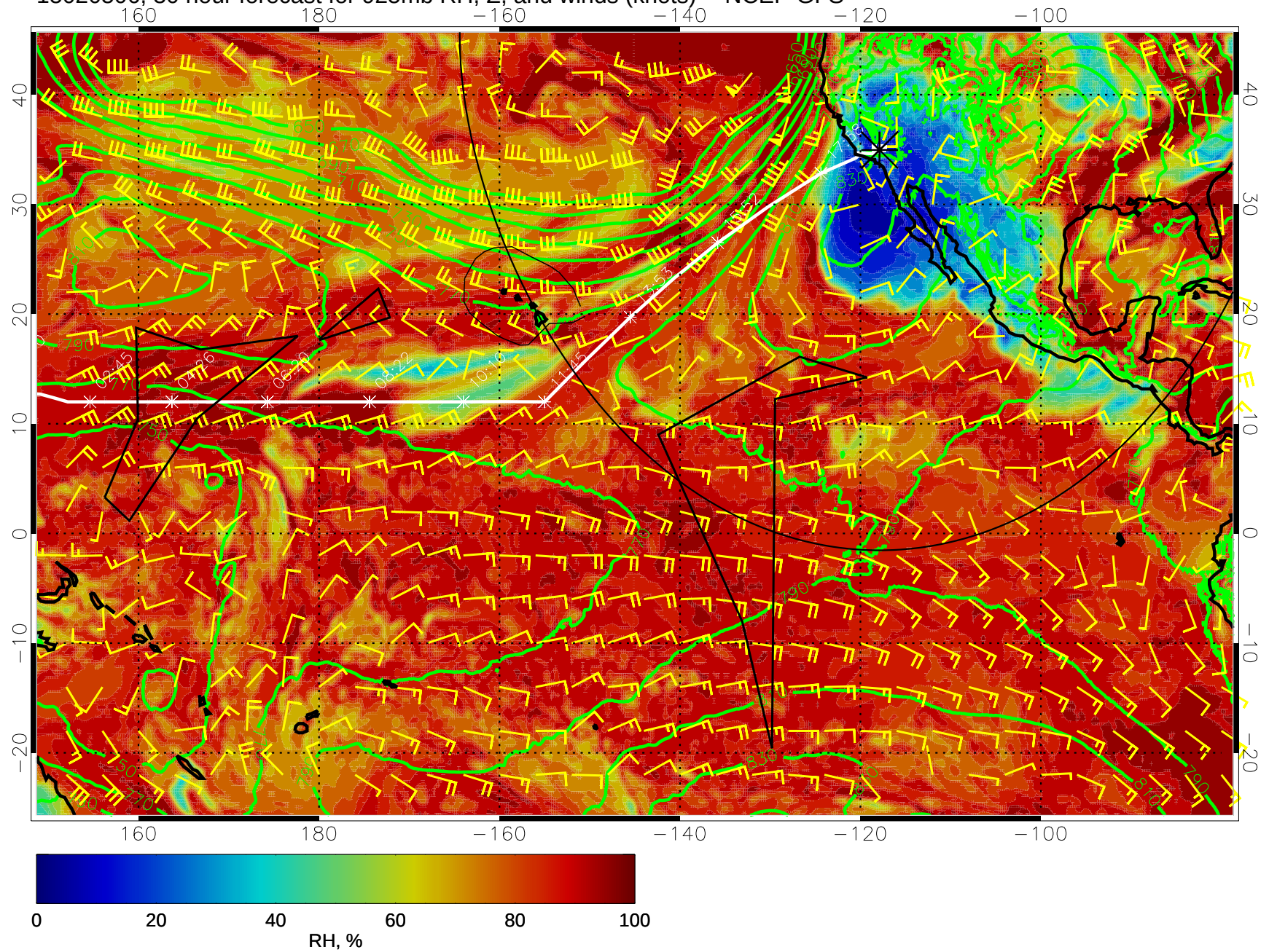
15020506, 30 hour forecast for 925mb RH, Z, and winds (knots) -- NCEP GFS
