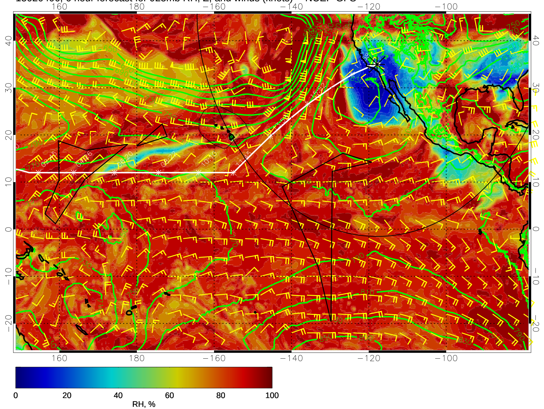
15020406, 6 hour forecast for 925mb RH, Z, and winds (knots) -- NCEP GFS
