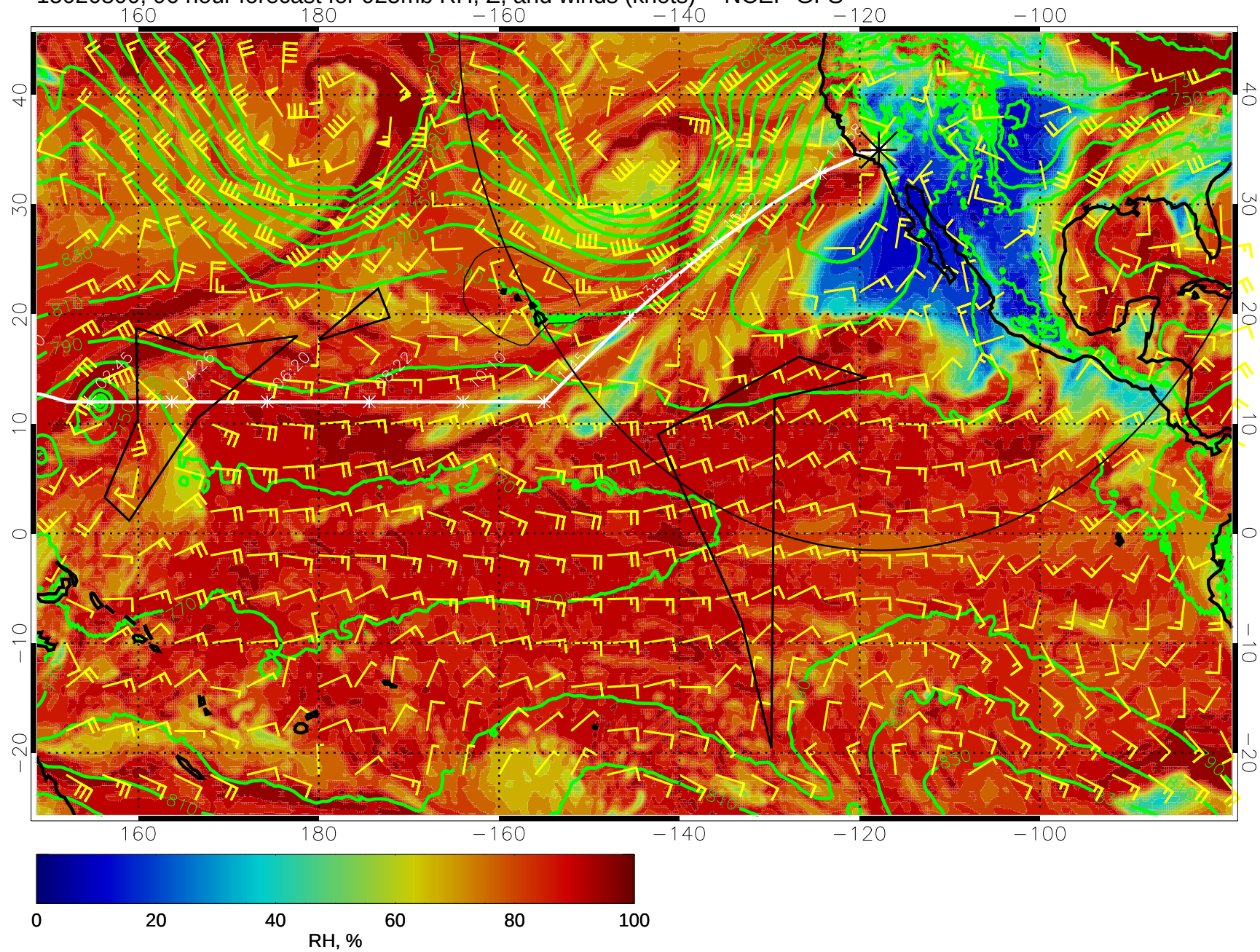
15020800, 96 hour forecast for 925mb RH, Z, and winds (knots) -- NCEP GFS
