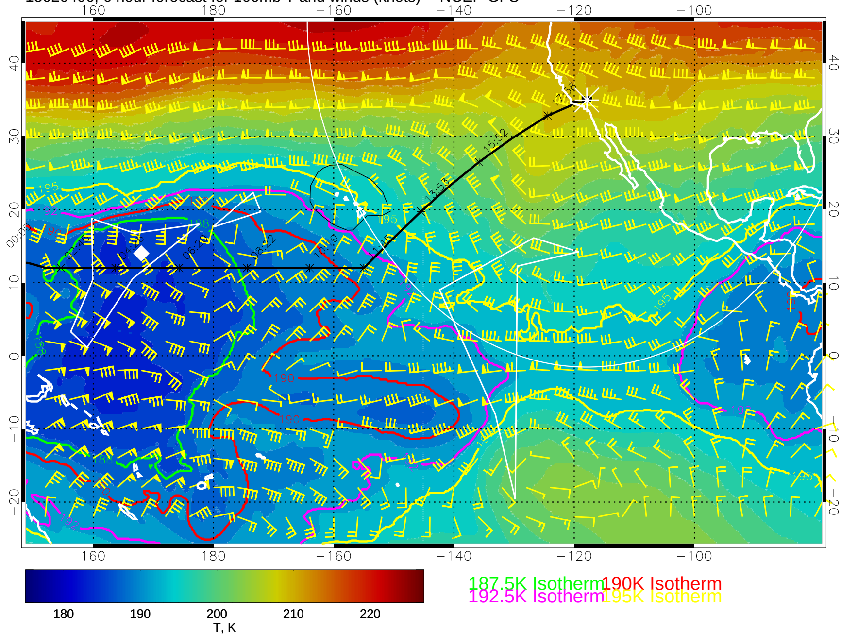
15020406, 6 hour forecast for 100mb T and winds (knots) -- NCEP GFS
