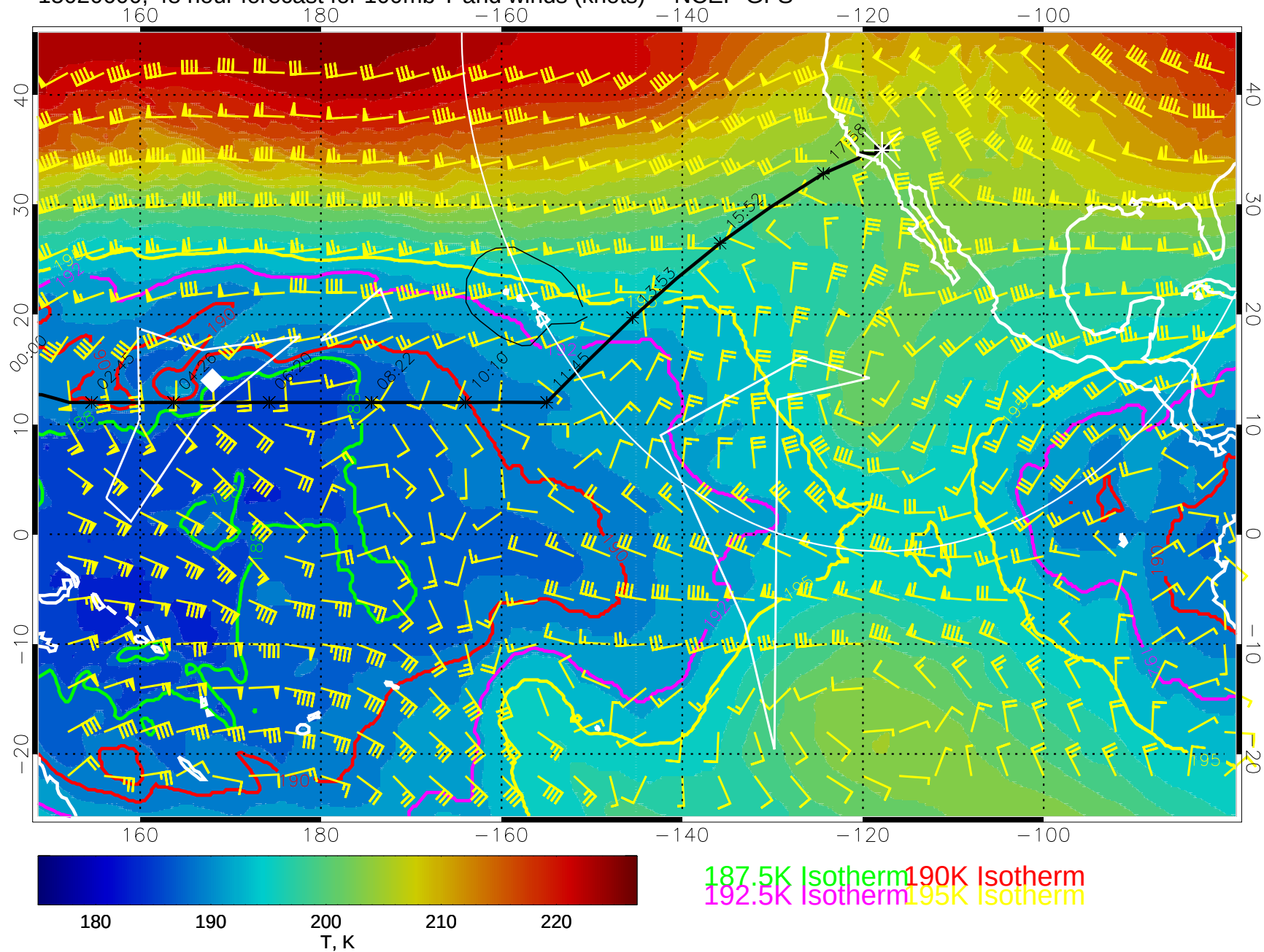
15020600, 48 hour forecast for 100mb T and winds (knots) -- NCEP GFS
