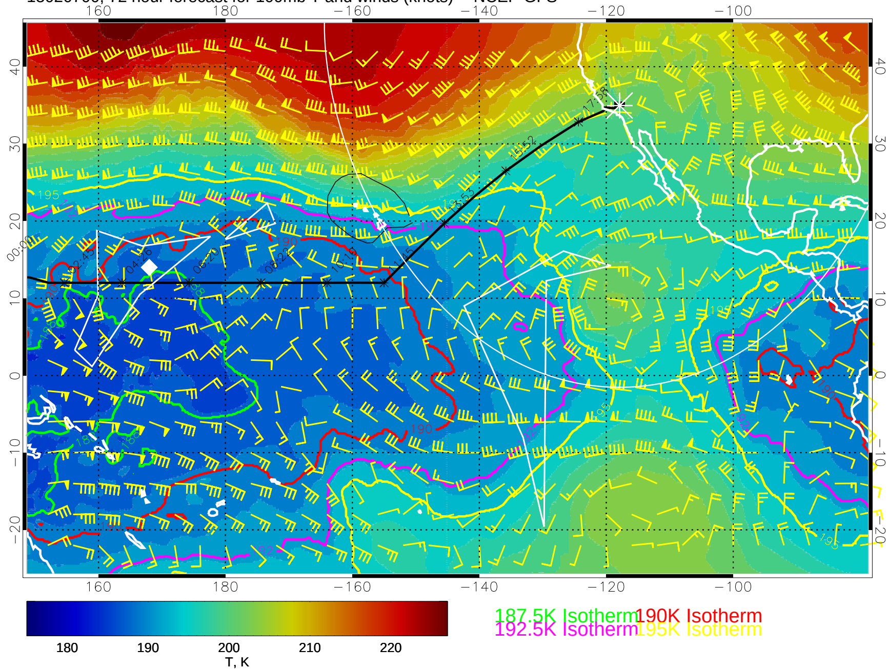
15020700, 72 hour forecast for 100mb T and winds (knots) -- NCEP GFS
