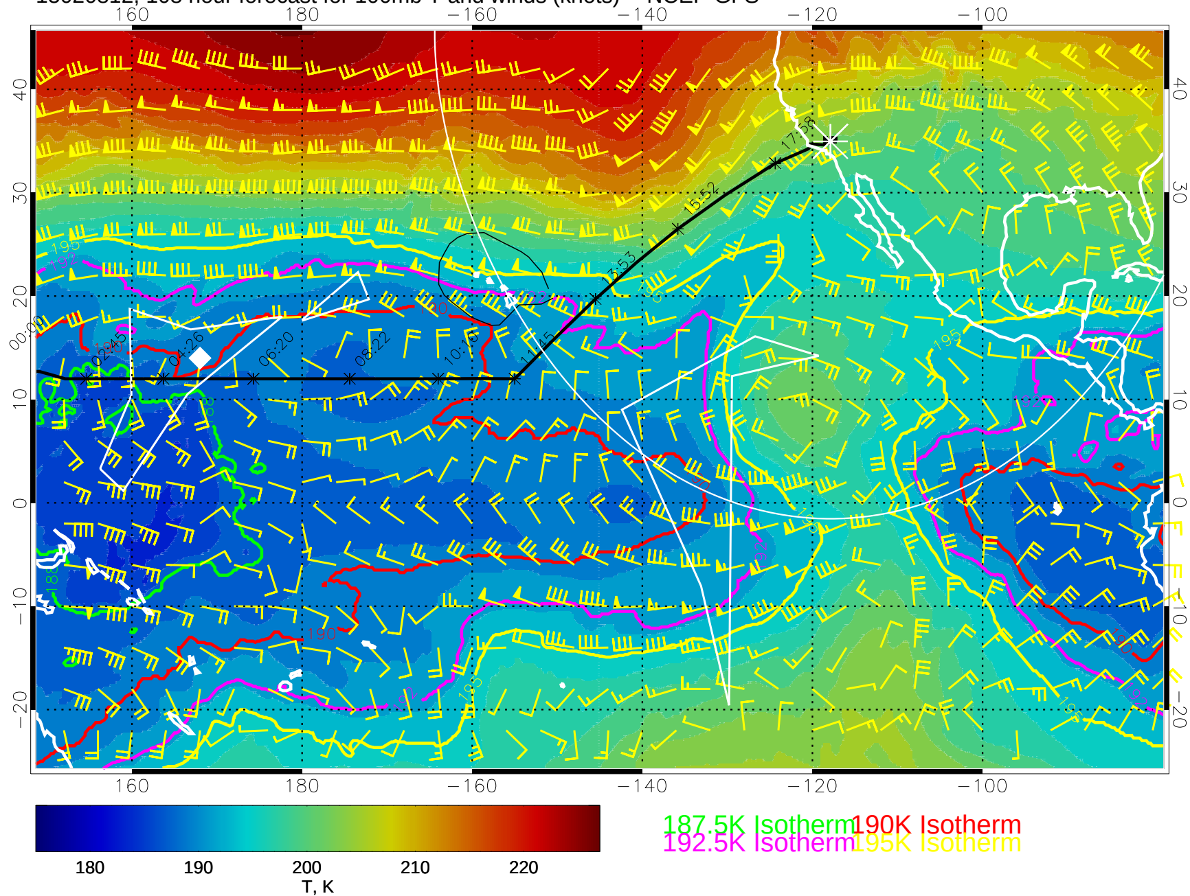
15020812, 108 hour forecast for 100mb T and winds (knots) -- NCEP GFS
