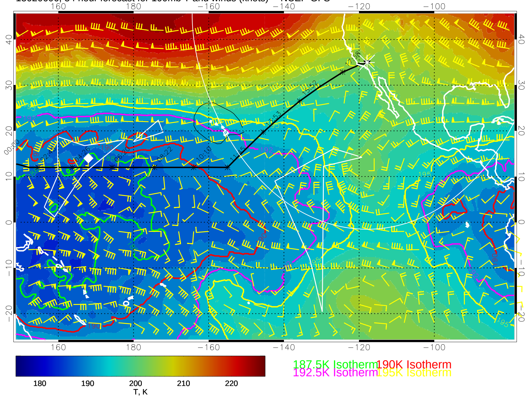
15020606, 54 hour forecast for 100mb T and winds (knots) -- NCEP GFS
