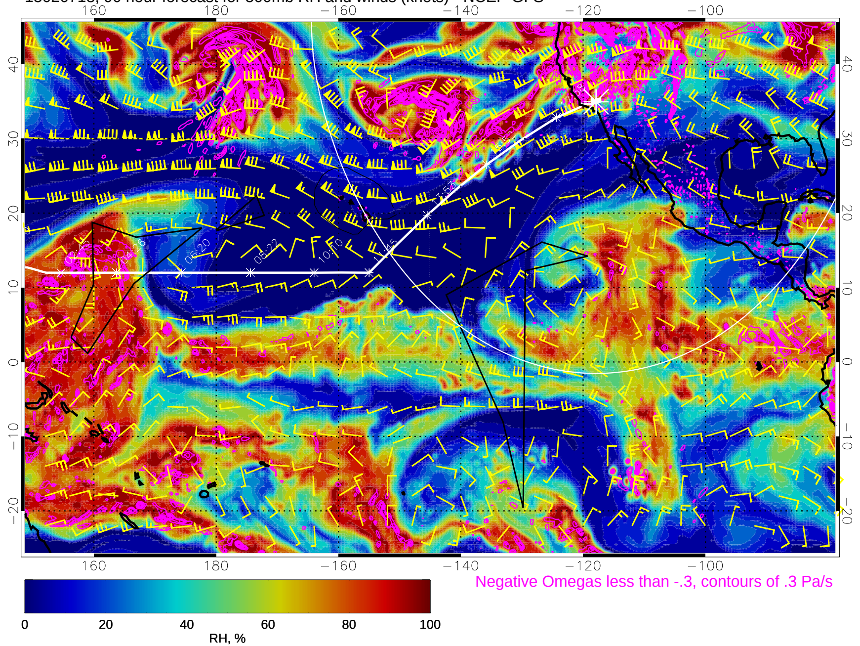
15020718, 90 hour forecast for 500mb RH and winds (knots) - NCEP GFS
