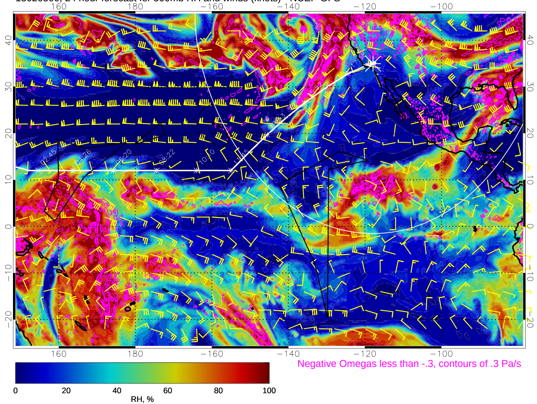
15020500, 24 hour forecast for 500mb RH and winds (knots) - NCEP GFS
