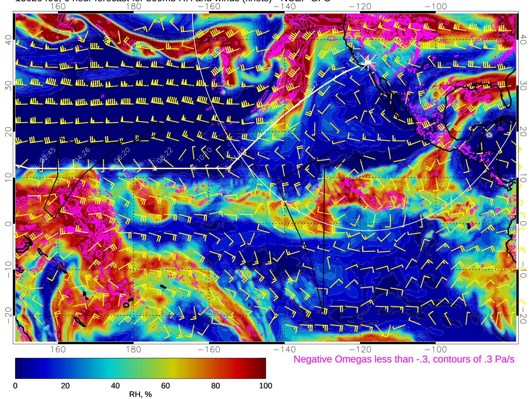
15020406, 6 hour forecast for 500mb RH and winds (knots) - NCEP GFS
