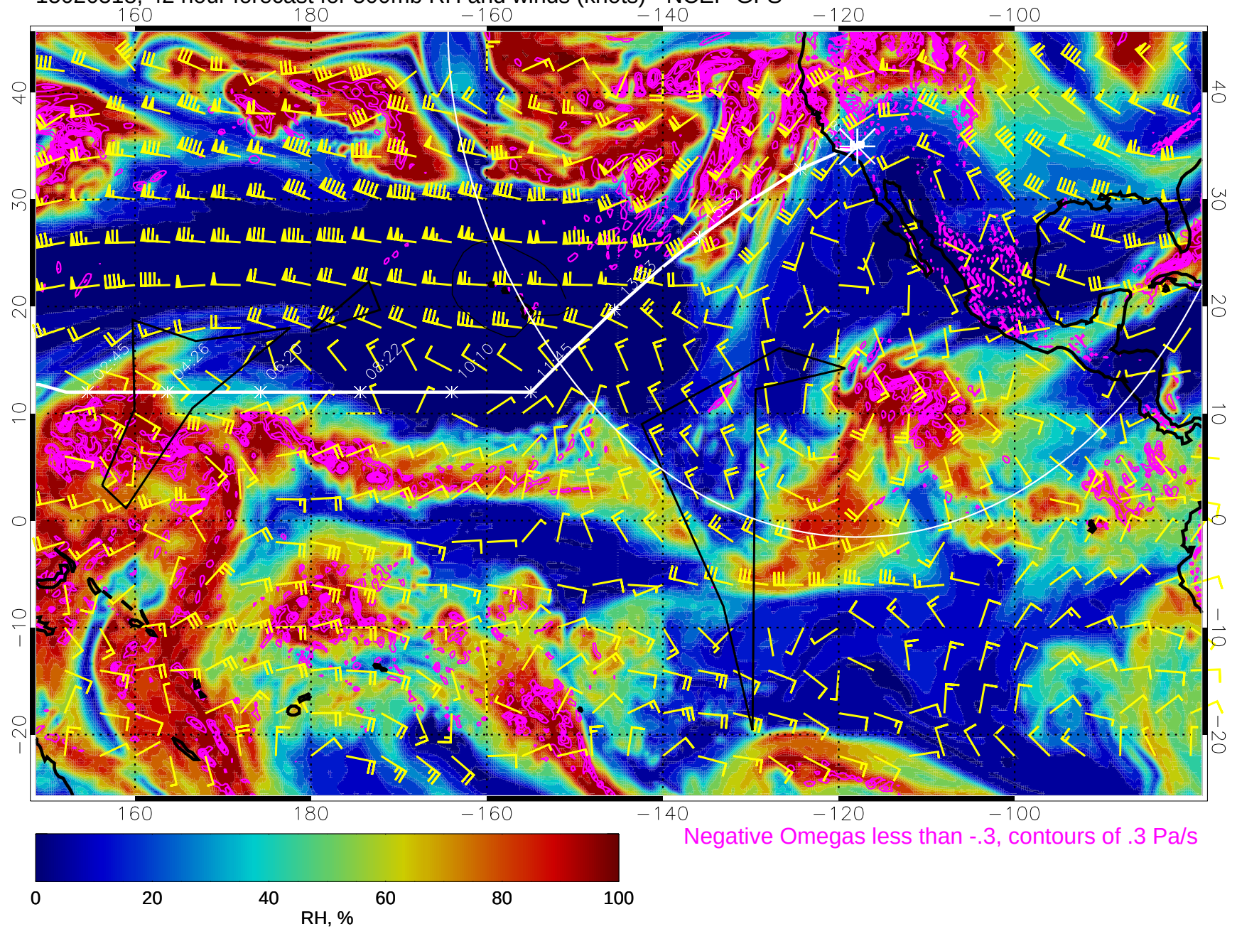
15020518, 42 hour forecast for 500mb RH and winds (knots) - NCEP GFS
