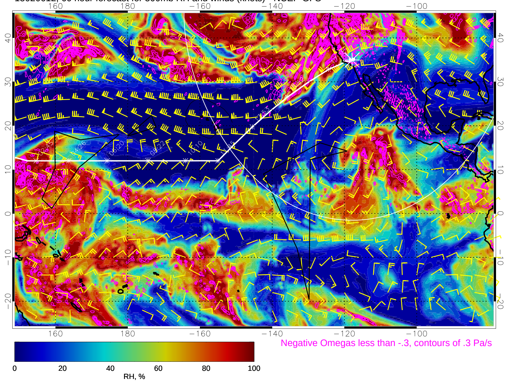
15020612, 60 hour forecast for 500mb RH and winds (knots) - NCEP GFS
