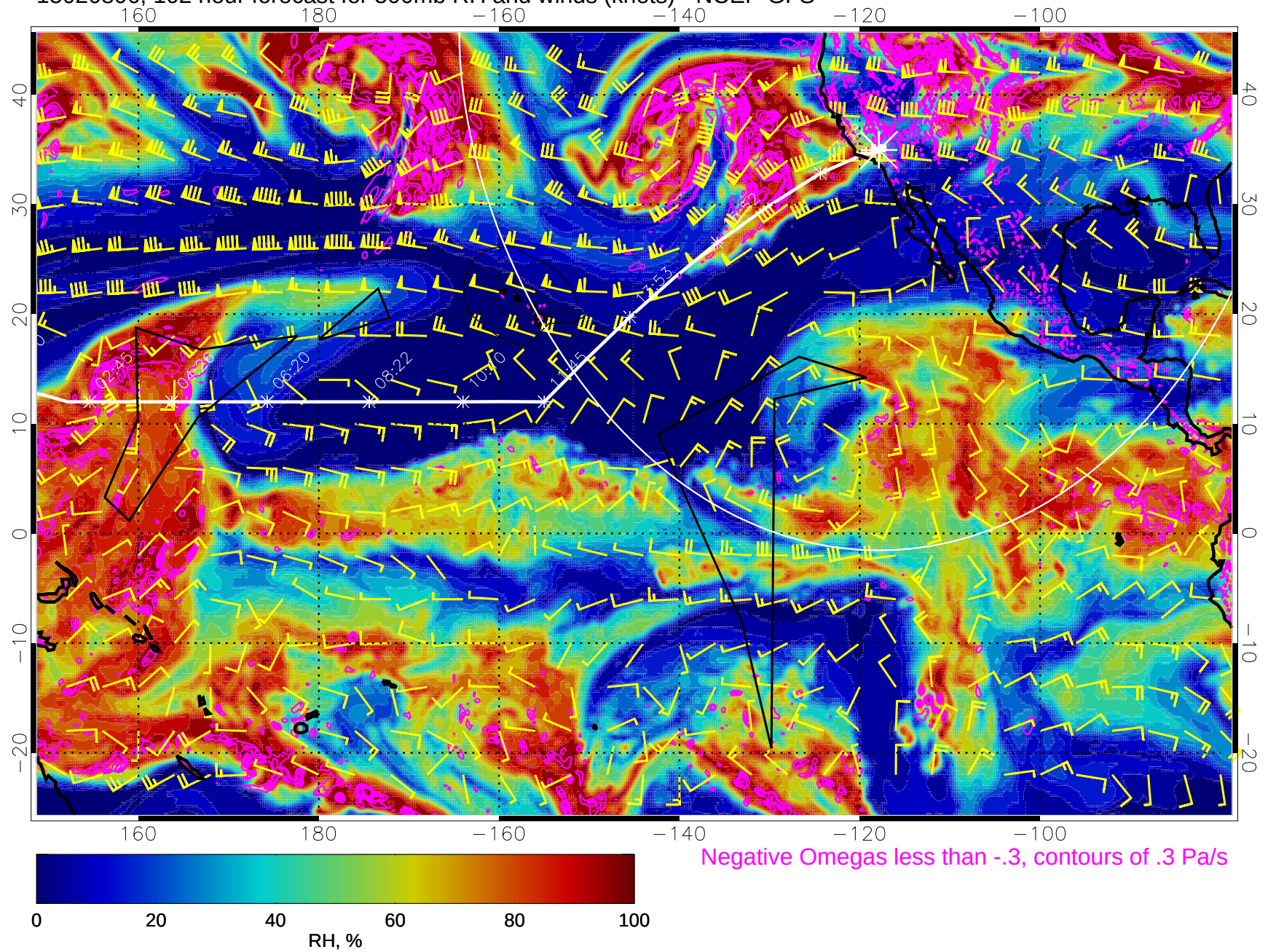
15020806, 102 hour forecast for 500mb RH and winds (knots) - NCEP GFS
