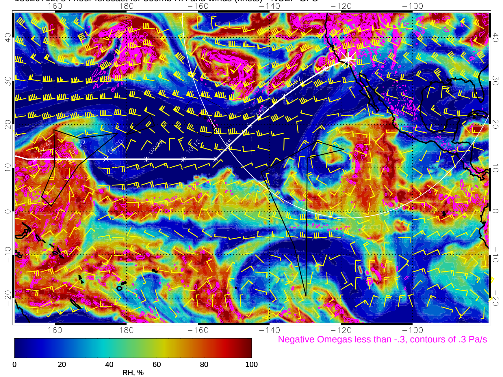
15020712, 84 hour forecast for 500mb RH and winds (knots) - NCEP GFS
