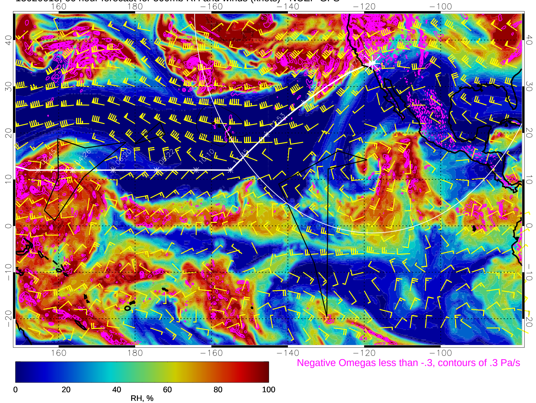
15020618, 66 hour forecast for 500mb RH and winds (knots) - NCEP GFS
