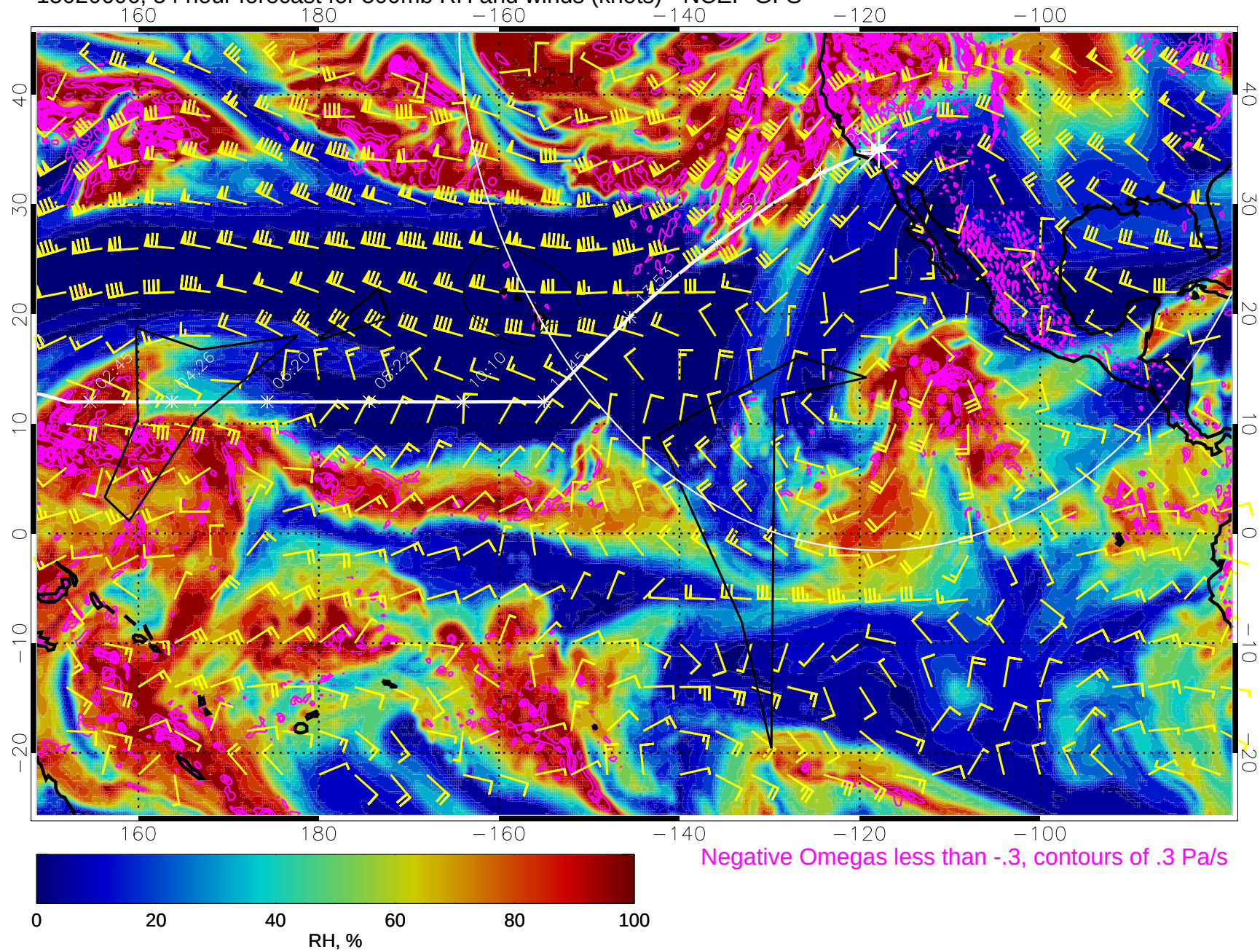
15020606, 54 hour forecast for 500mb RH and winds (knots) - NCEP GFS
