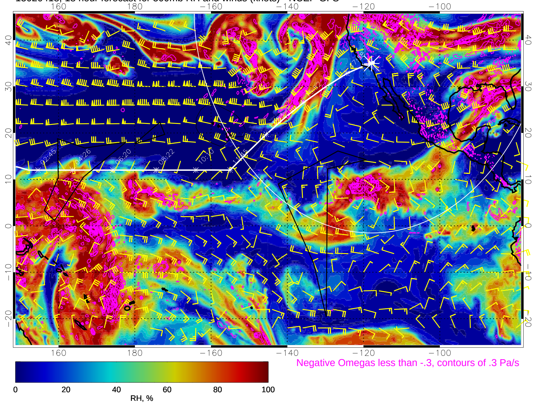
15020418, 18 hour forecast for 500mb RH and winds (knots) - NCEP GFS
