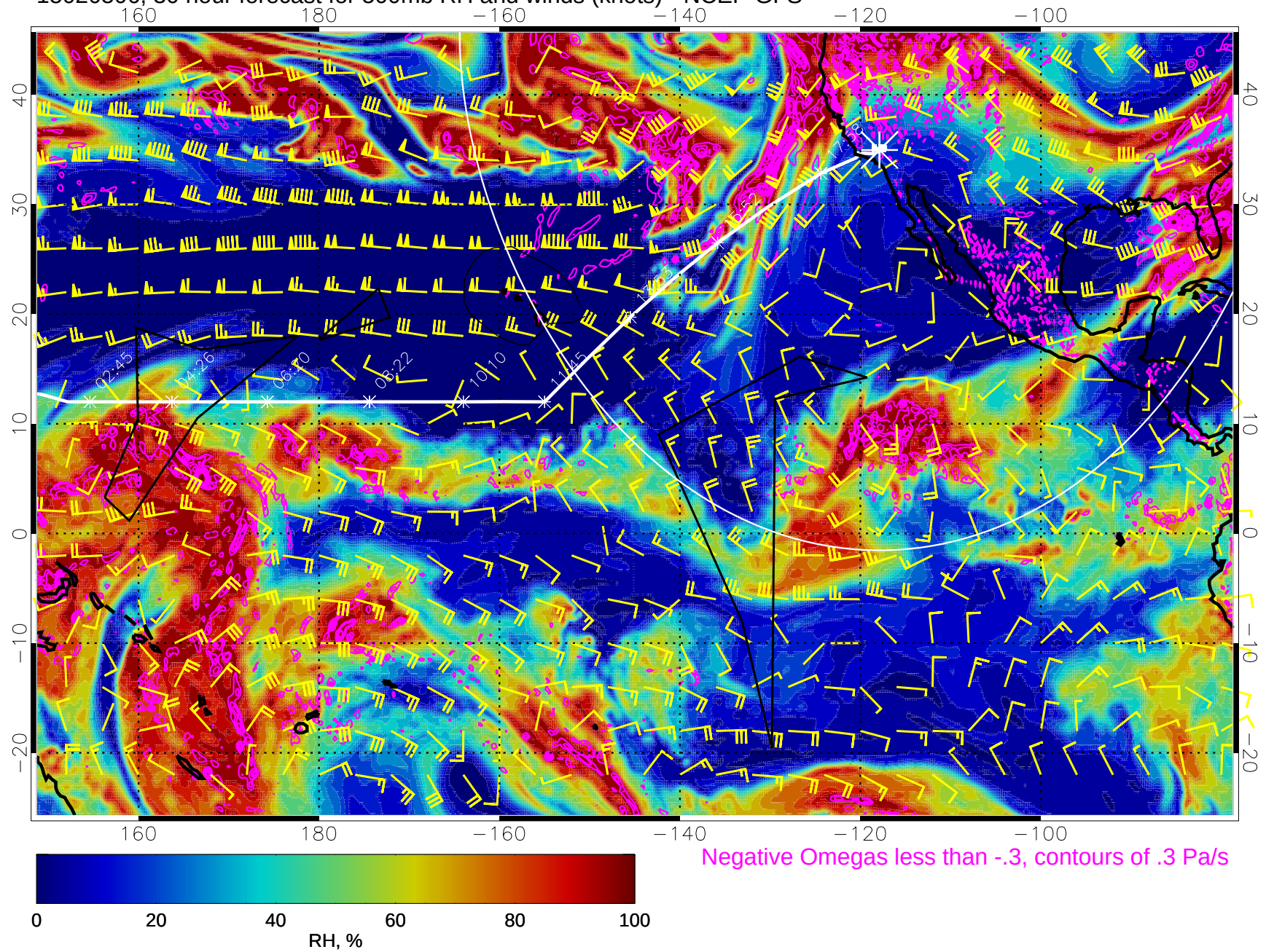
15020506, 30 hour forecast for 500mb RH and winds (knots) - NCEP GFS
