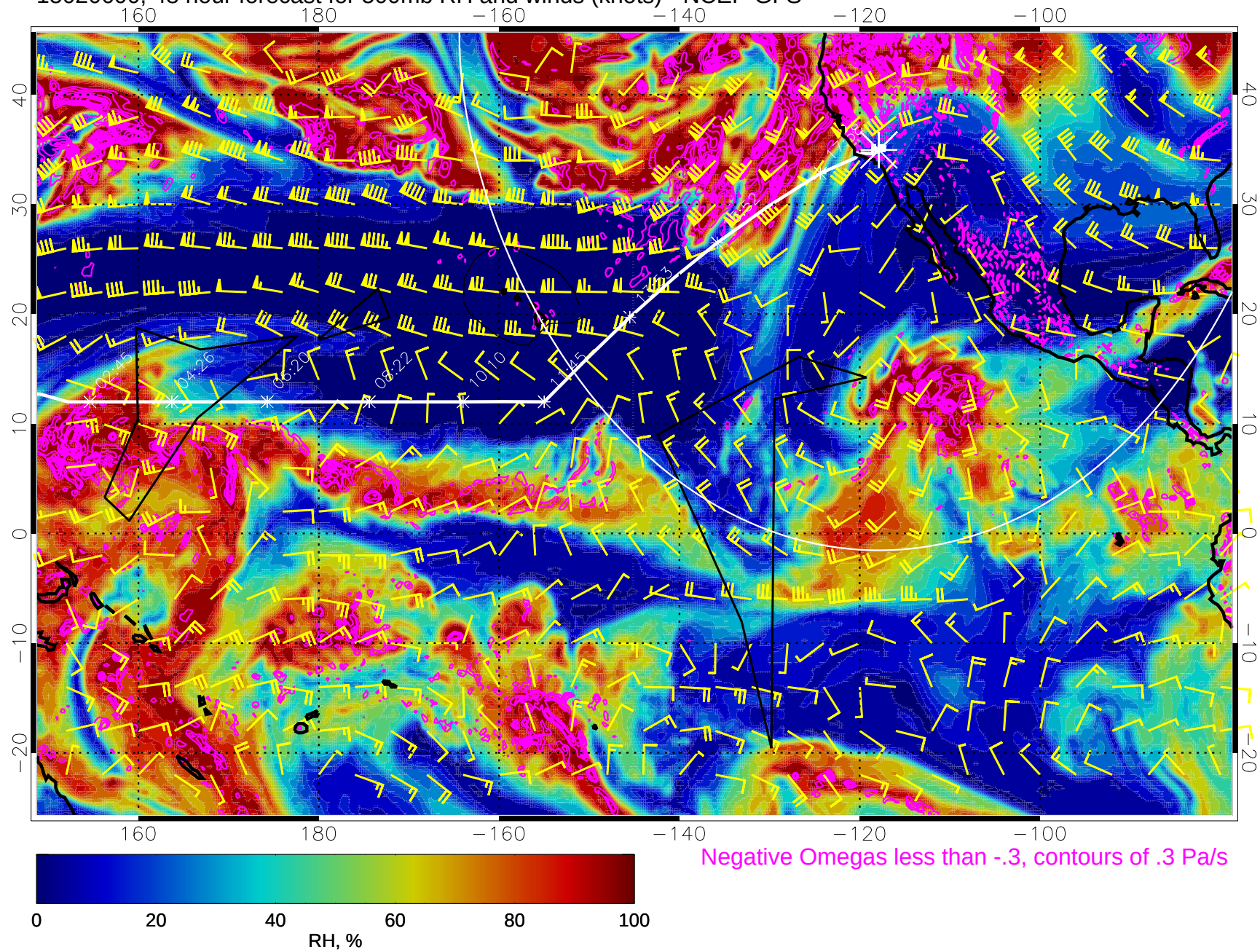
15020600, 48 hour forecast for 500mb RH and winds (knots) - NCEP GFS
