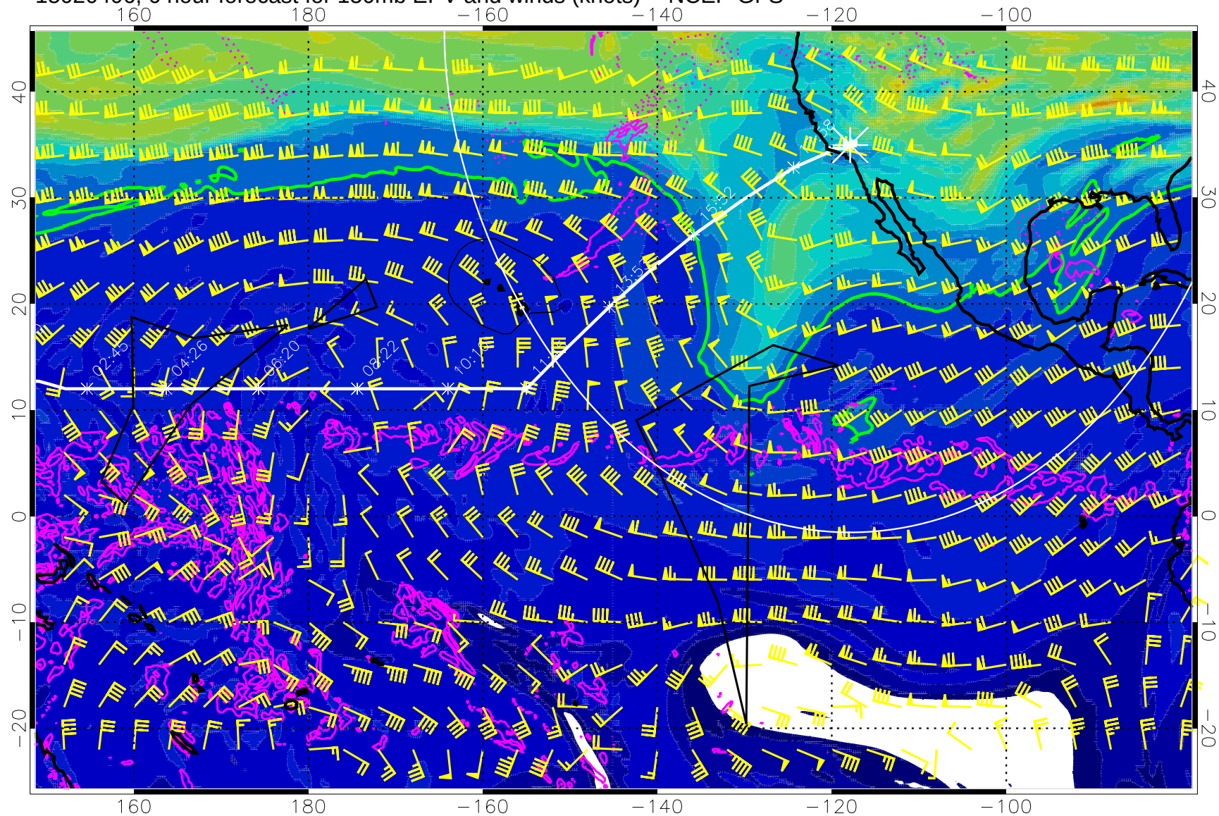
15020406, 6 hour forecast for 150mb EPV and winds (knots) -- NCEP GFS
