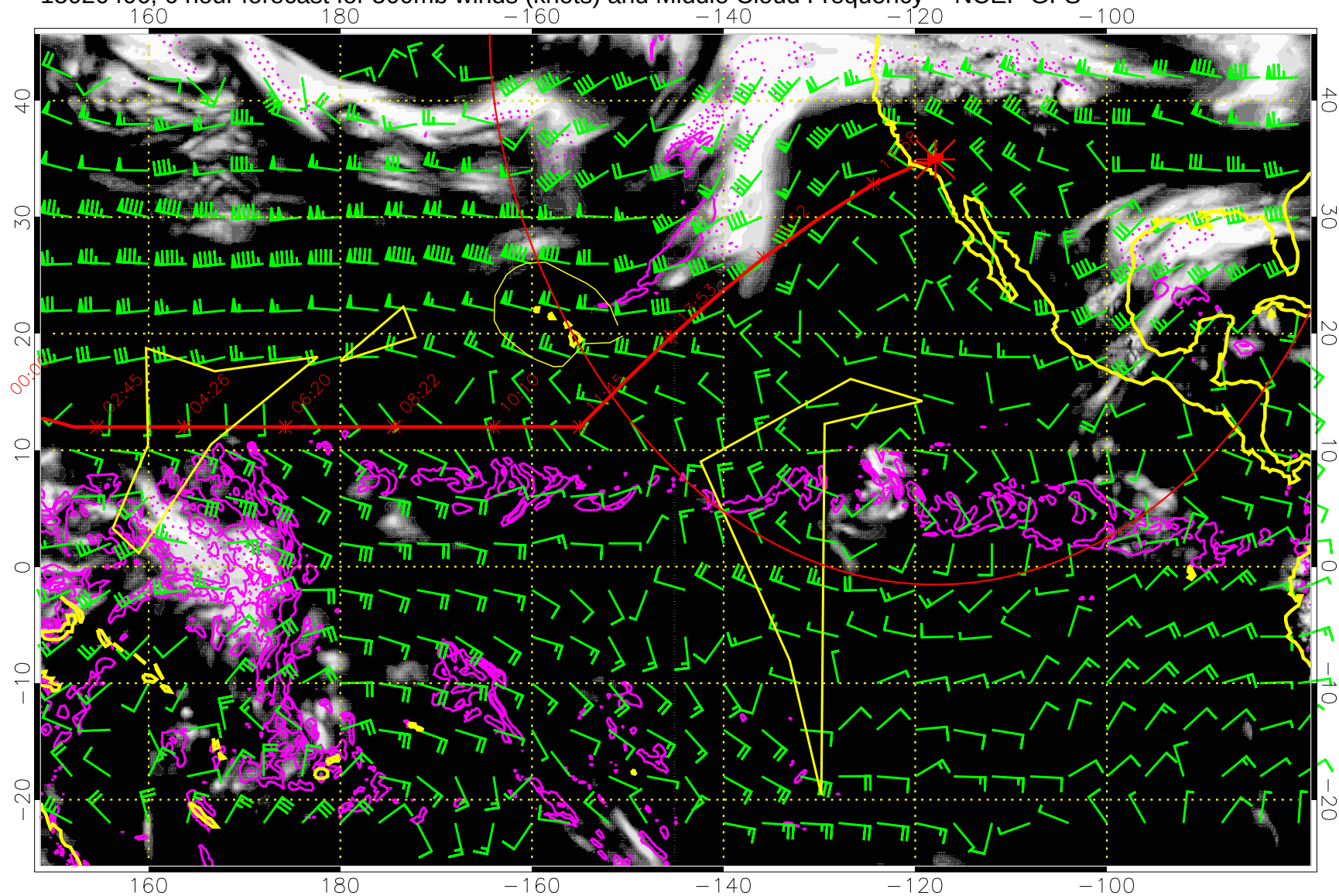
15020406, 6 hour forecast for 500mb winds (knots) and Middle Cloud Frequency -- NCEP GFS
