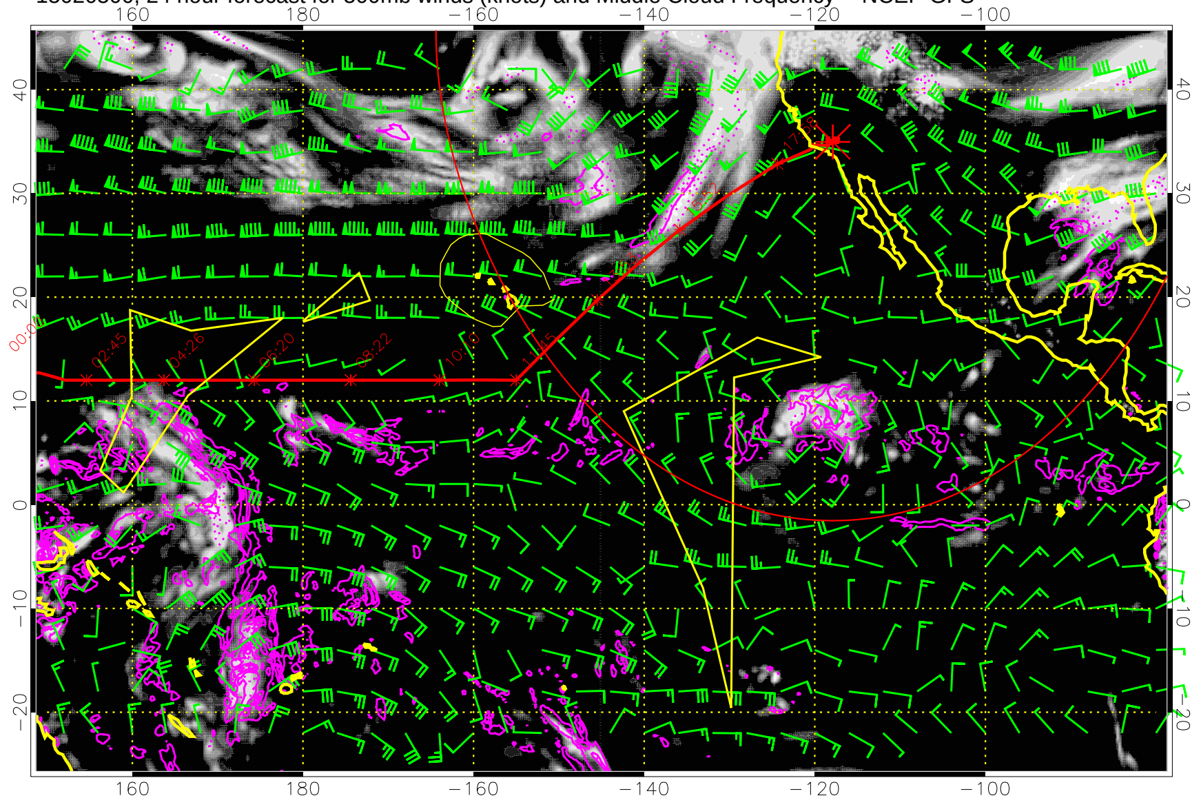
15020500, 24 hour forecast for 500mb winds (knots) and Middle Cloud Frequency -- NCEP GFS
