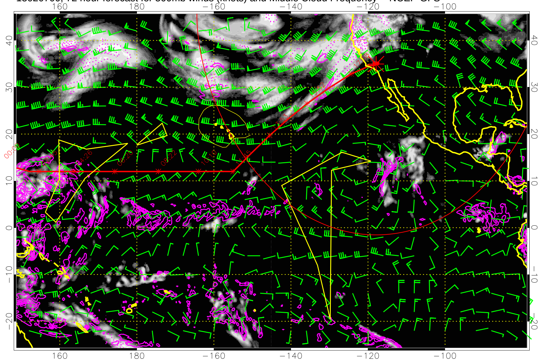
15020700, 72 hour forecast for 500mb winds (knots) and Middle Cloud Frequency -- NCEP GFS
