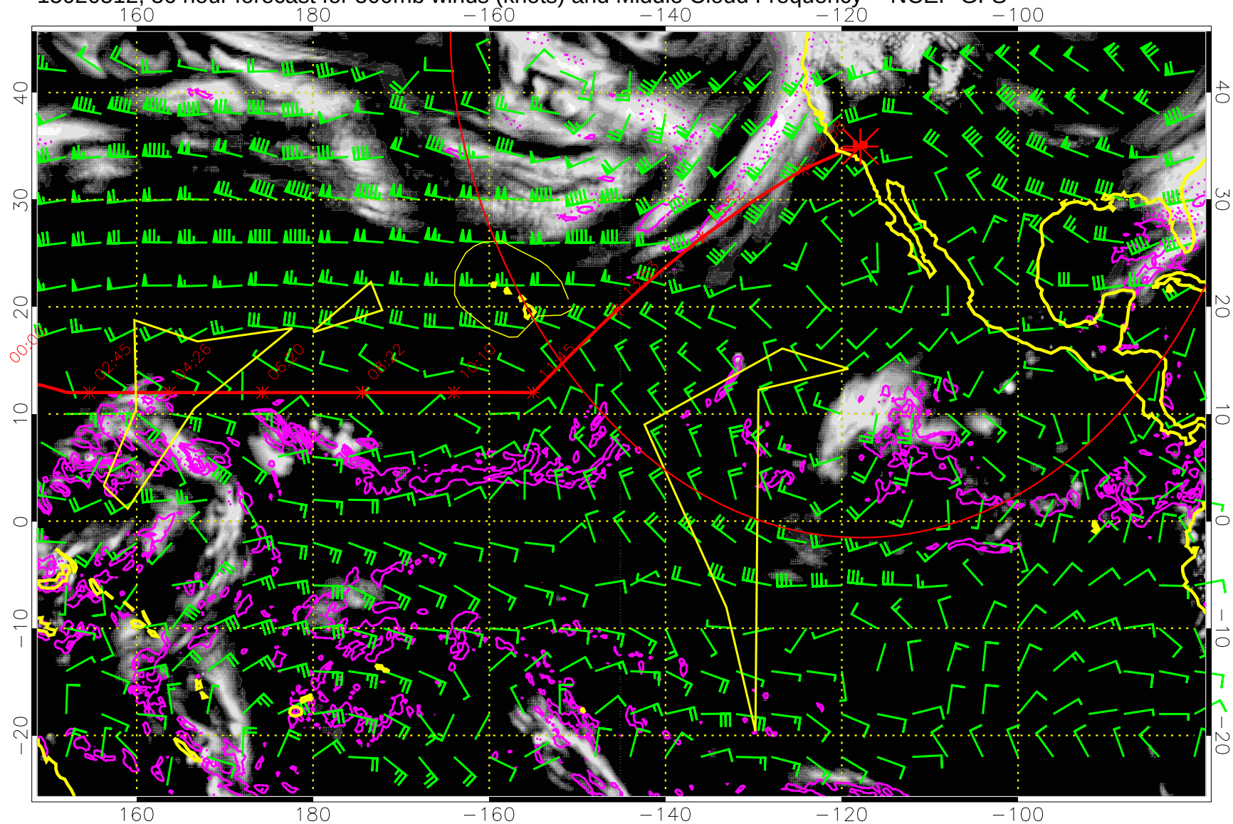
15020512, 36 hour forecast for 500mb winds (knots) and Middle Cloud Frequency -- NCEP GFS
