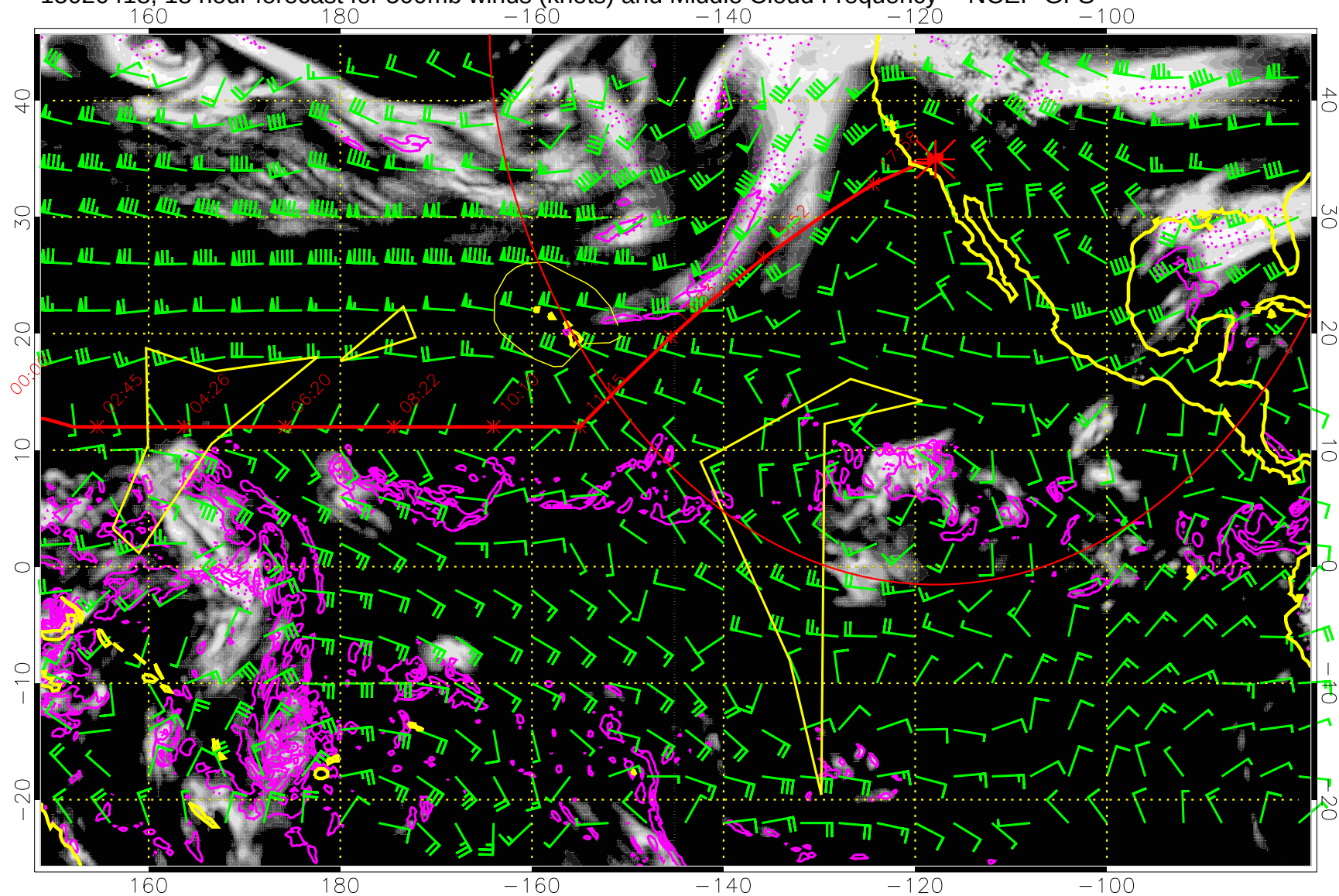
15020418, 18 hour forecast for 500mb winds (knots) and Middle Cloud Frequency -- NCEP GFS
