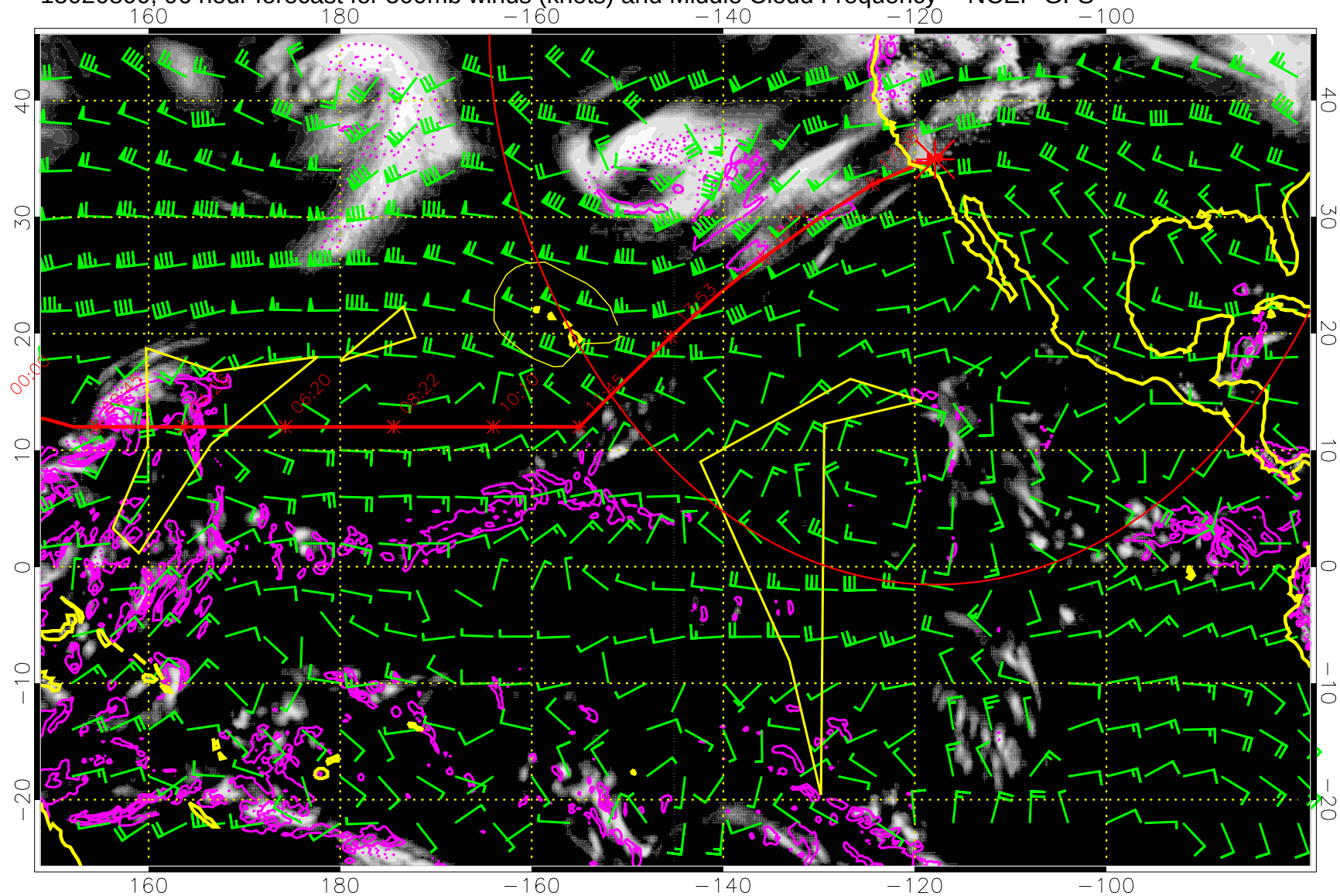
15020800, 96 hour forecast for 500mb winds (knots) and Middle Cloud Frequency -- NCEP GFS
