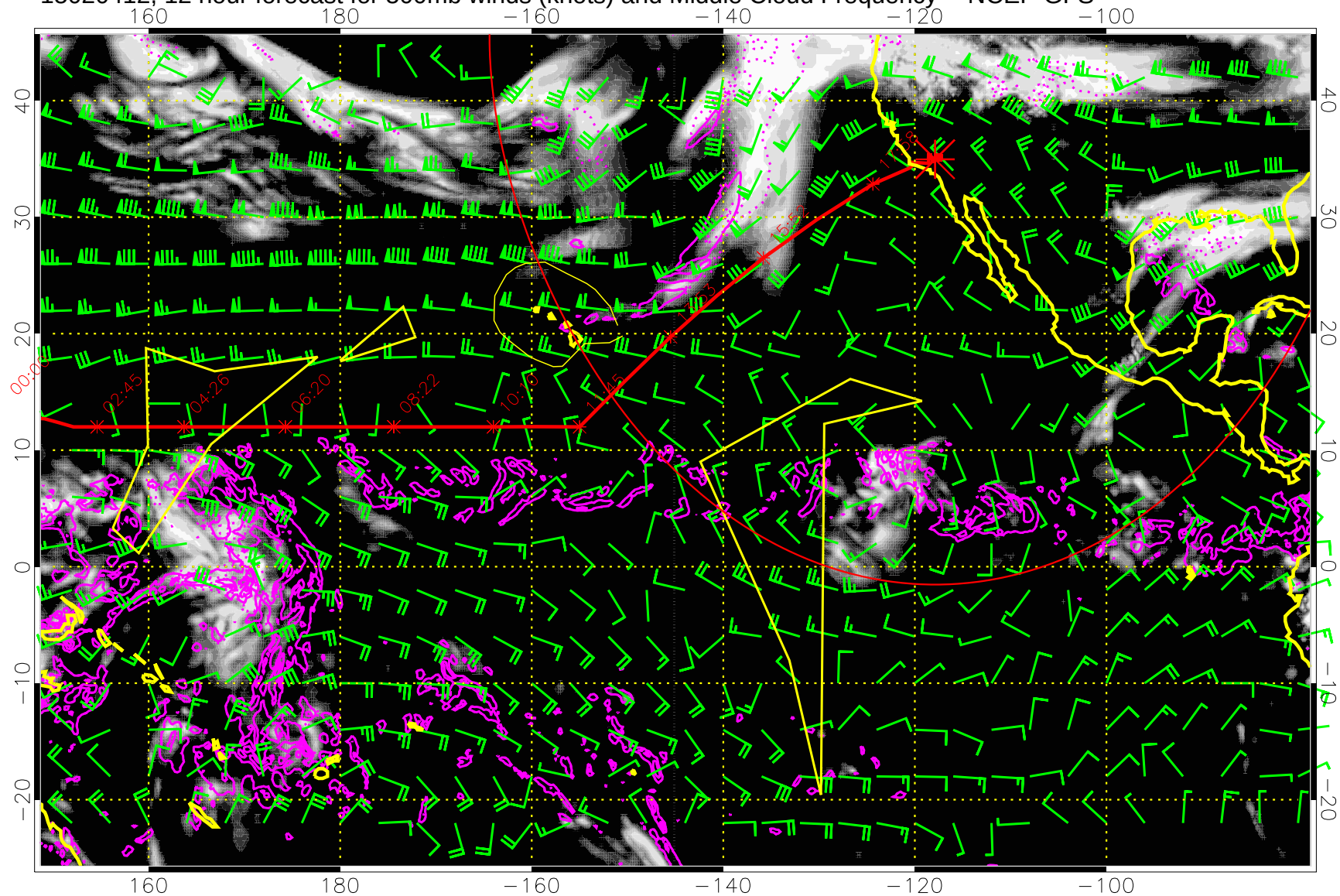
15020412, 12 hour forecast for 500mb winds (knots) and Middle Cloud Frequency -- NCEP GFS
