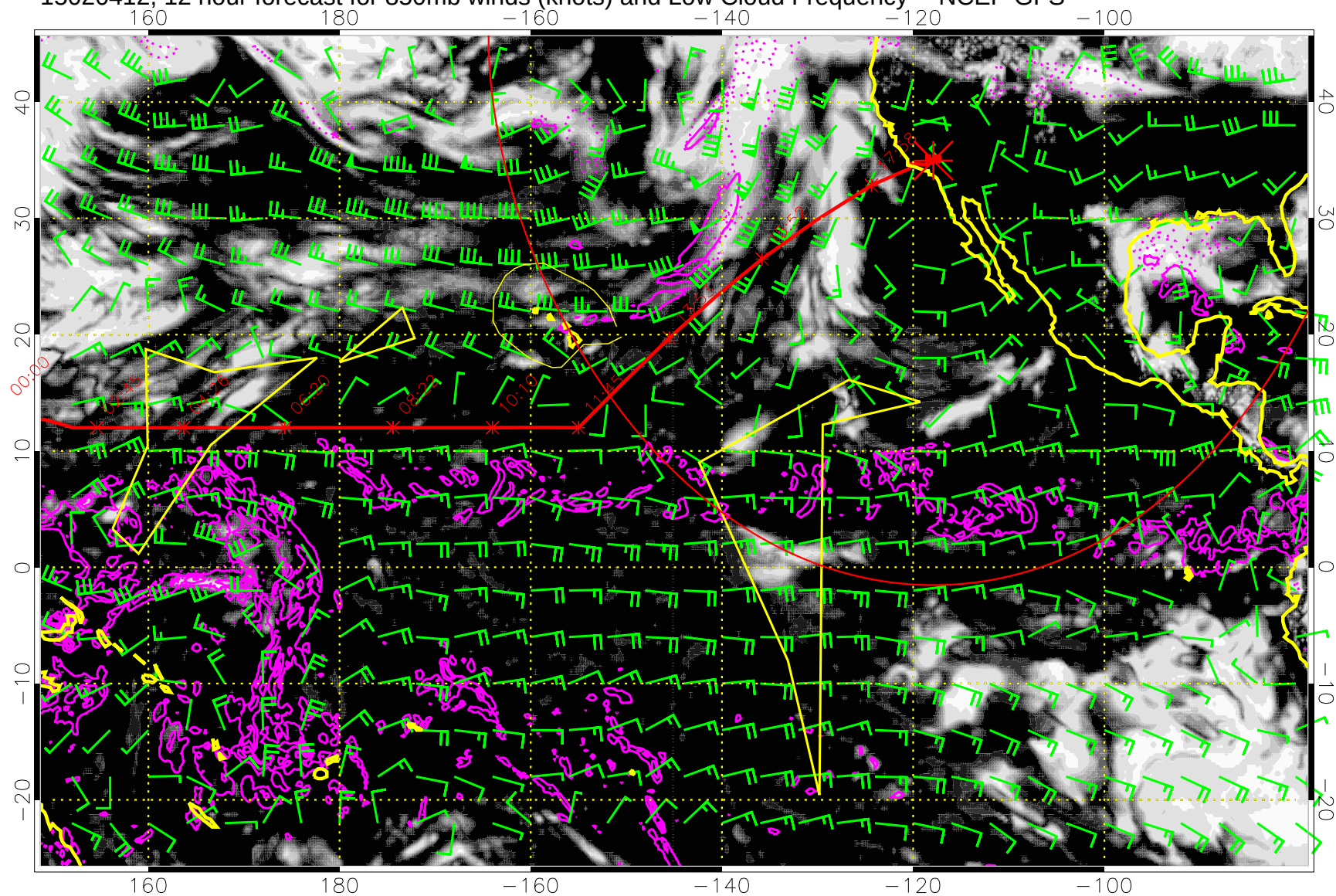
15020412, 12 hour forecast for 850mb winds (knots) and Low Cloud Frequency -- NCEP GFS
