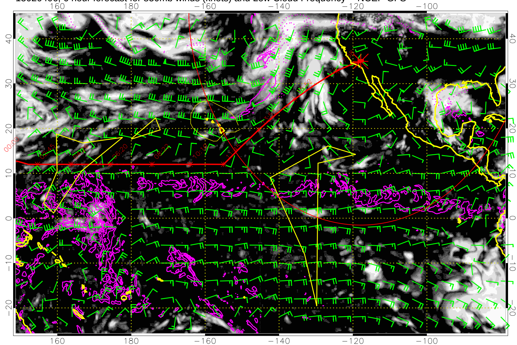
15020406, 6 hour forecast for 850mb winds (knots) and Low Cloud Frequency -- NCEP GFS
