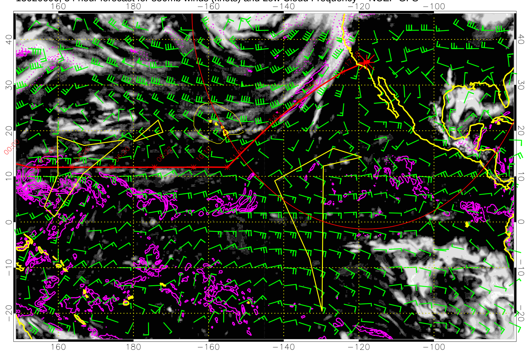
15020606, 54 hour forecast for 850mb winds (knots) and Low Cloud Frequency -- NCEP GFS
