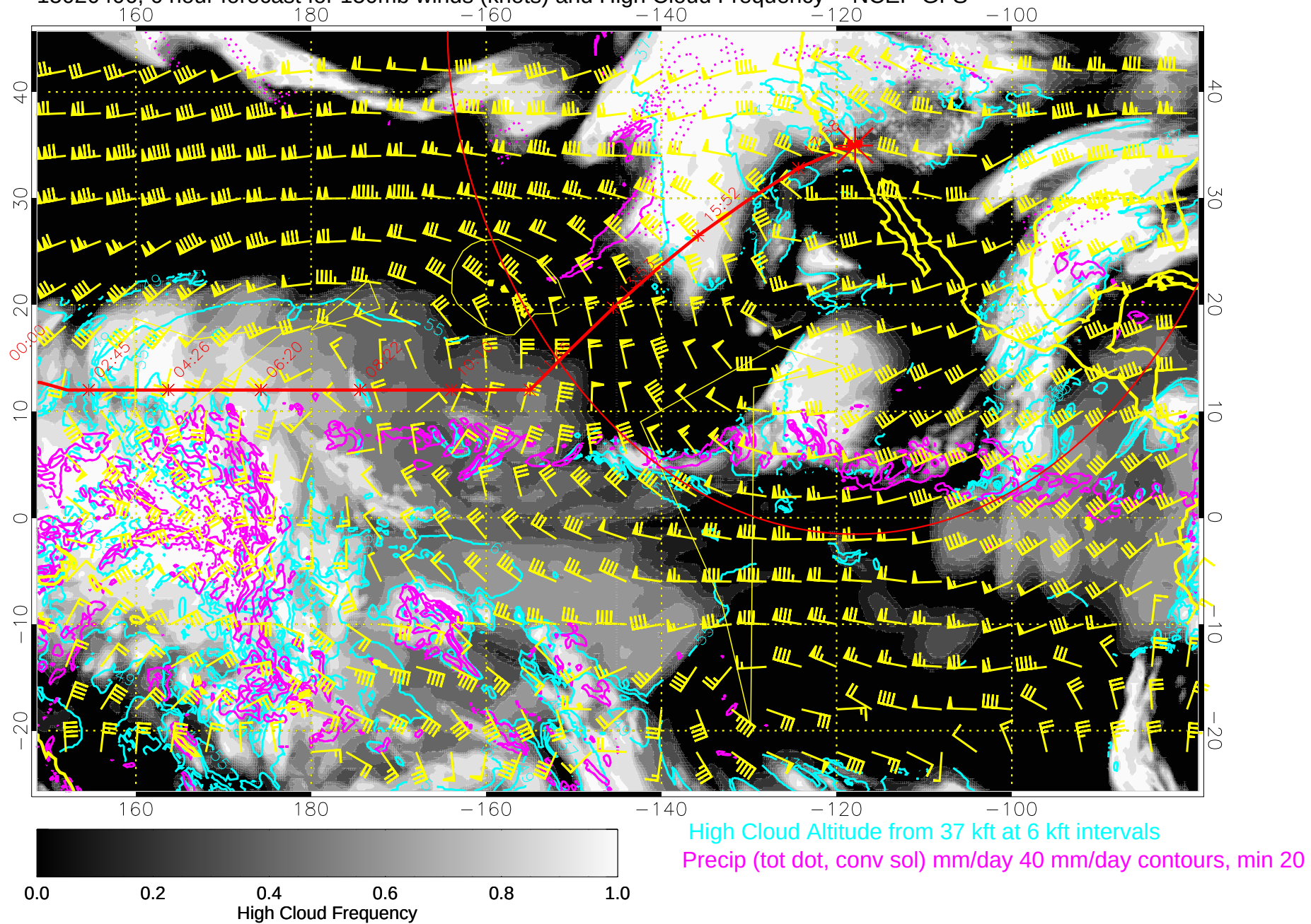
15020406, 6 hour forecast for 150mb winds (knots) and High Cloud Frequency -- NCEP GFS
