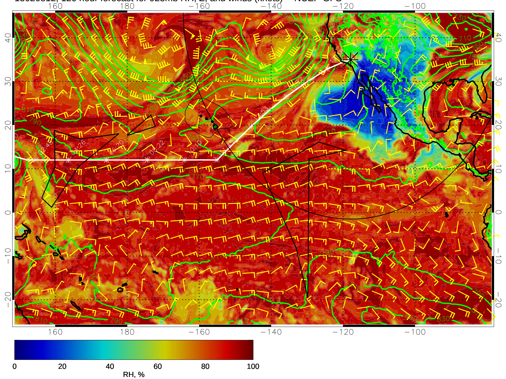
15020812, 120 hour forecast for 925mb RH, Z, and winds (knots) -- NCEP GFS
