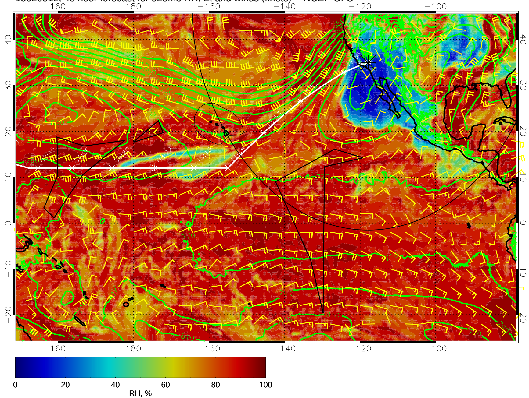
15020512, 48 hour forecast for 925mb RH, Z, and winds (knots) -- NCEP GFS
