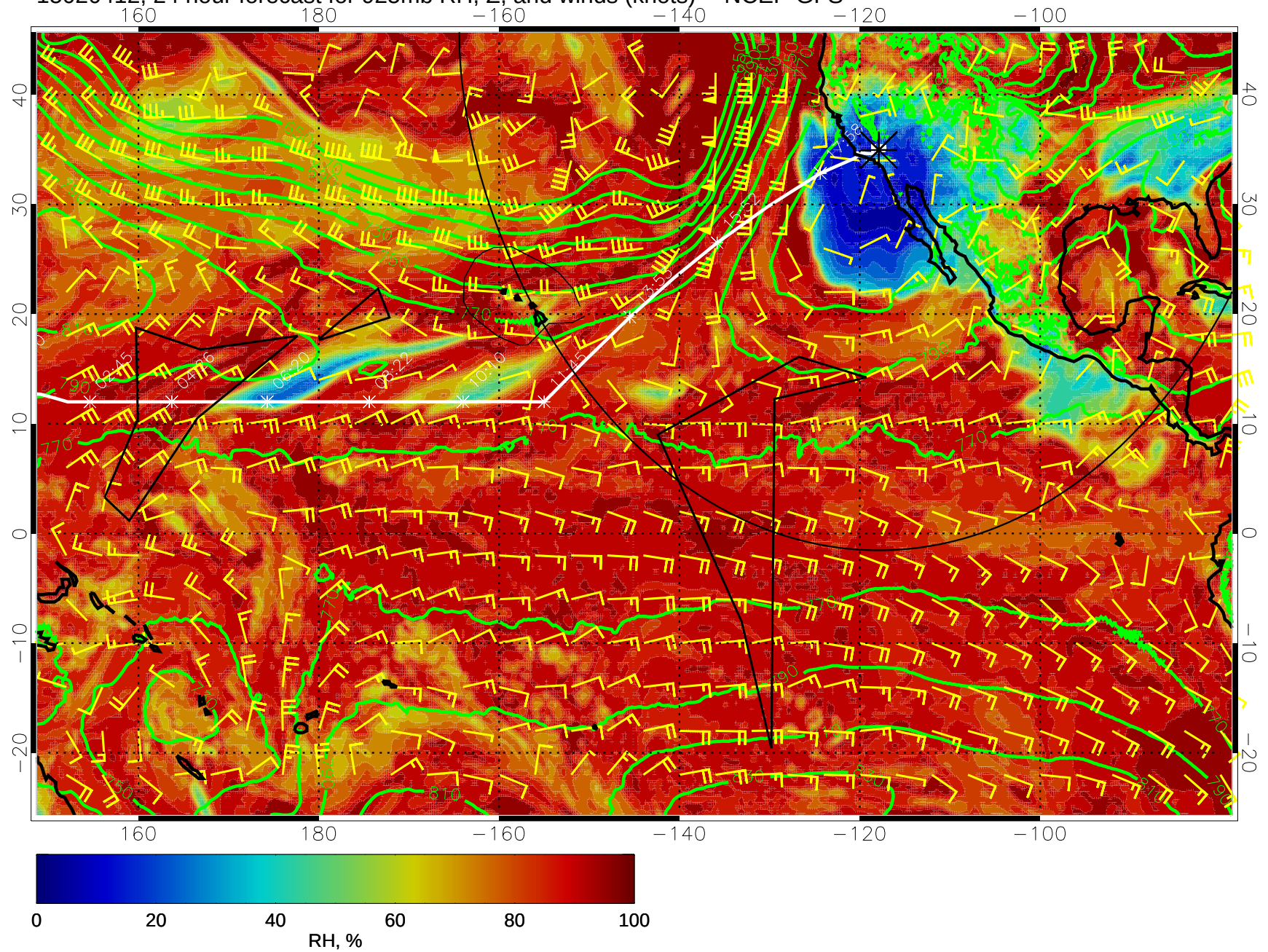
15020412, 24 hour forecast for 925mb RH, Z, and winds (knots) -- NCEP GFS
