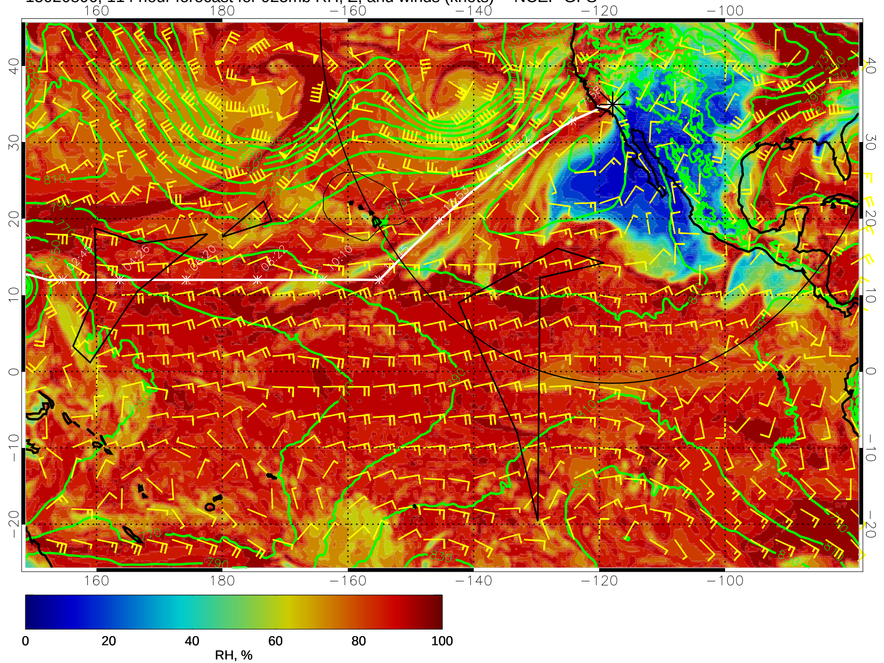
15020806, 114 hour forecast for 925mb RH, Z, and winds (knots) -- NCEP GFS
