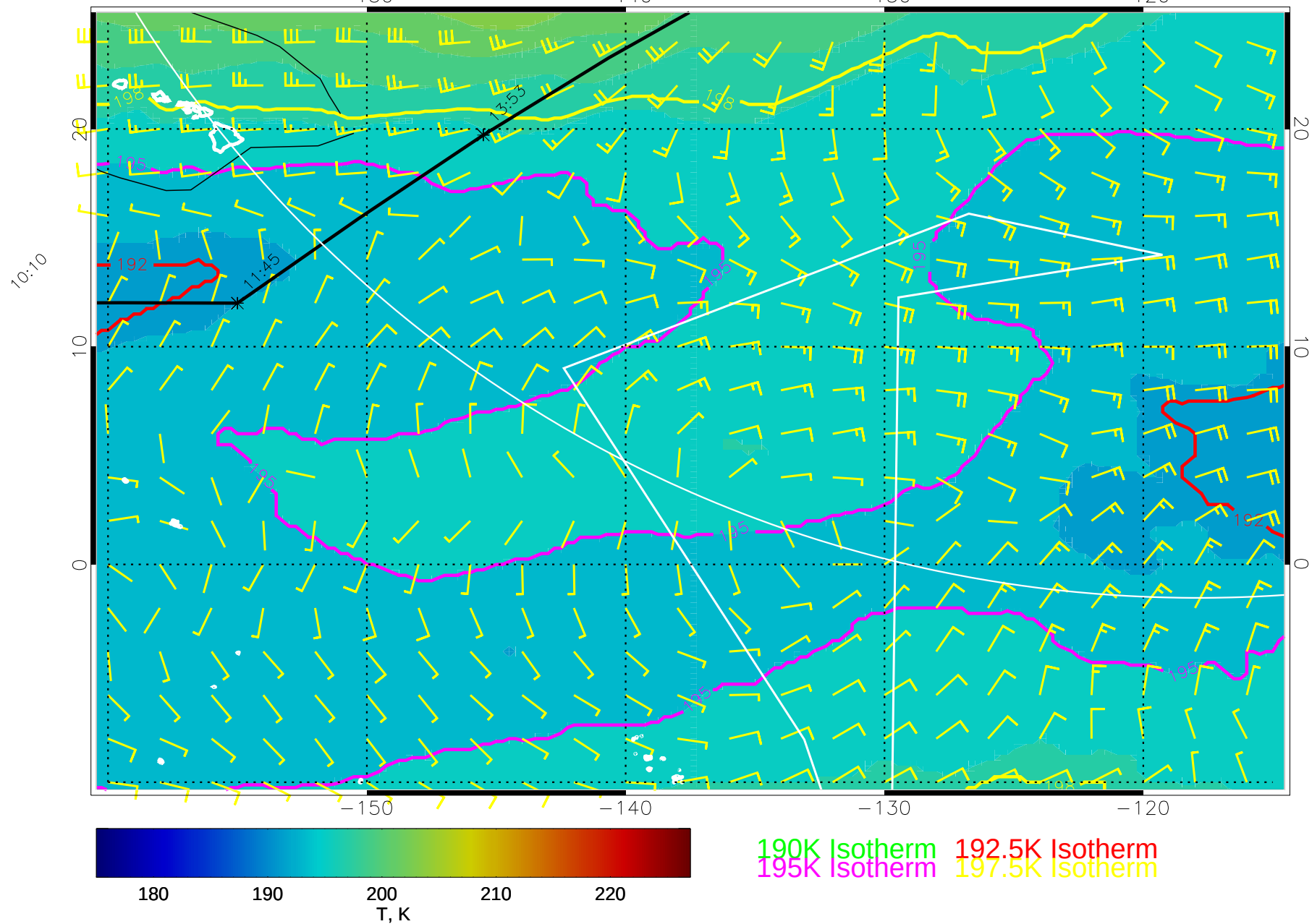
15020812, 120 hour forecast for 70mb T and winds (knots) -- NCEP GFS
