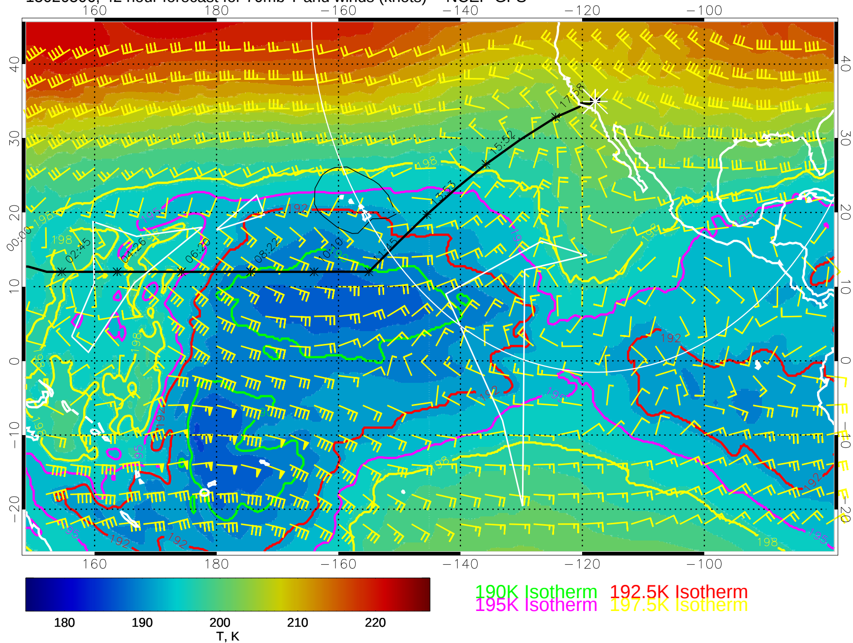
15020506, 42 hour forecast for 70mb T and winds (knots) -- NCEP GFS
