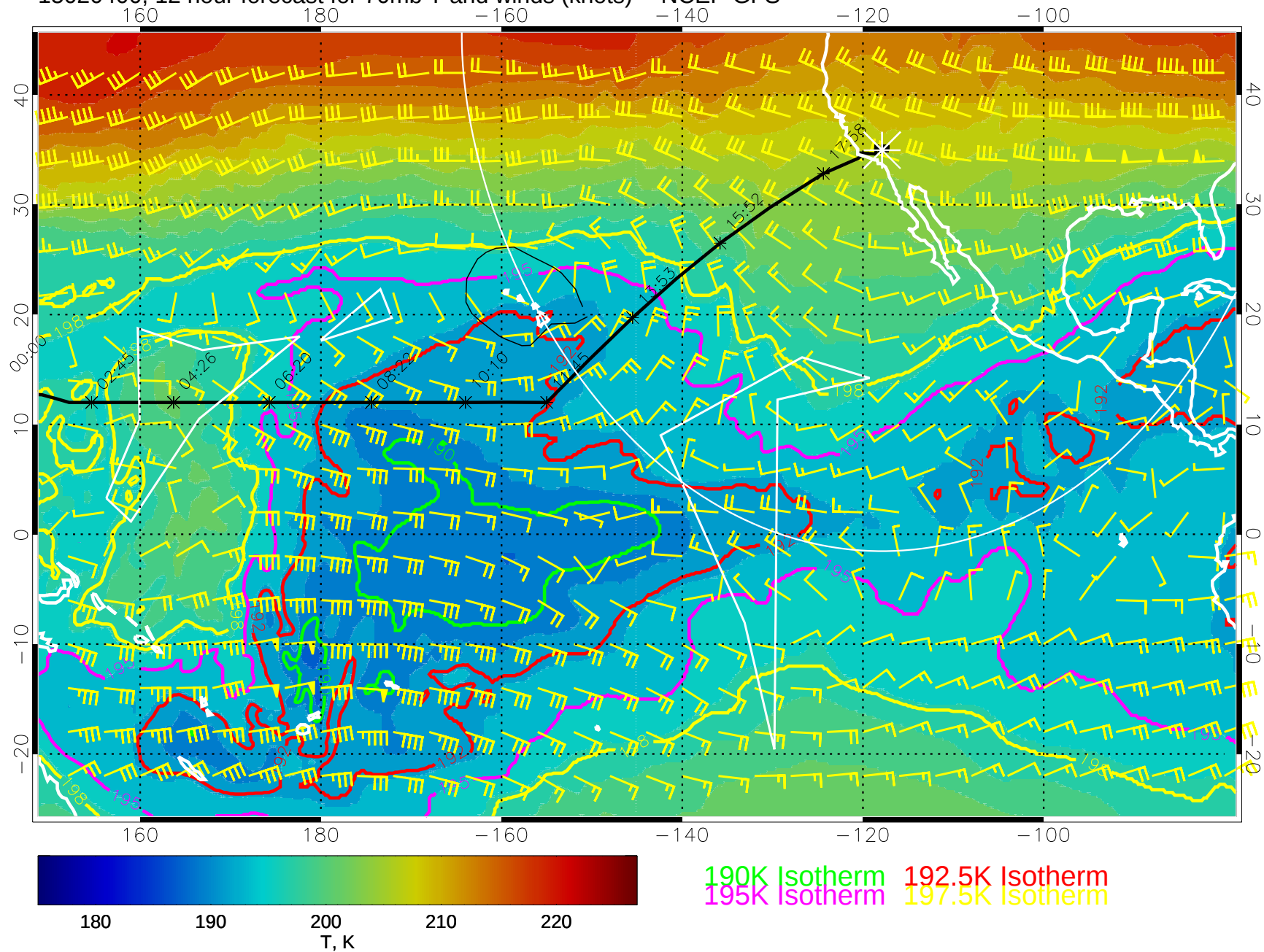
15020400, 12 hour forecast for 70mb T and winds (knots) -- NCEP GFS
