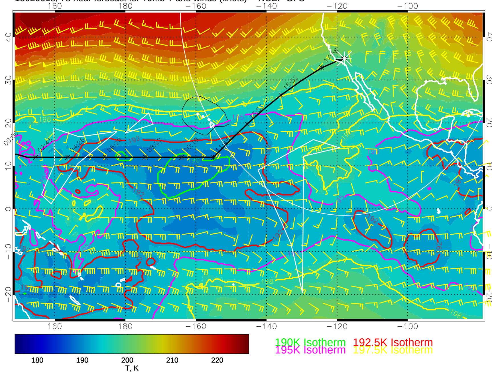
15020618, 78 hour forecast for 70mb T and winds (knots) -- NCEP GFS
