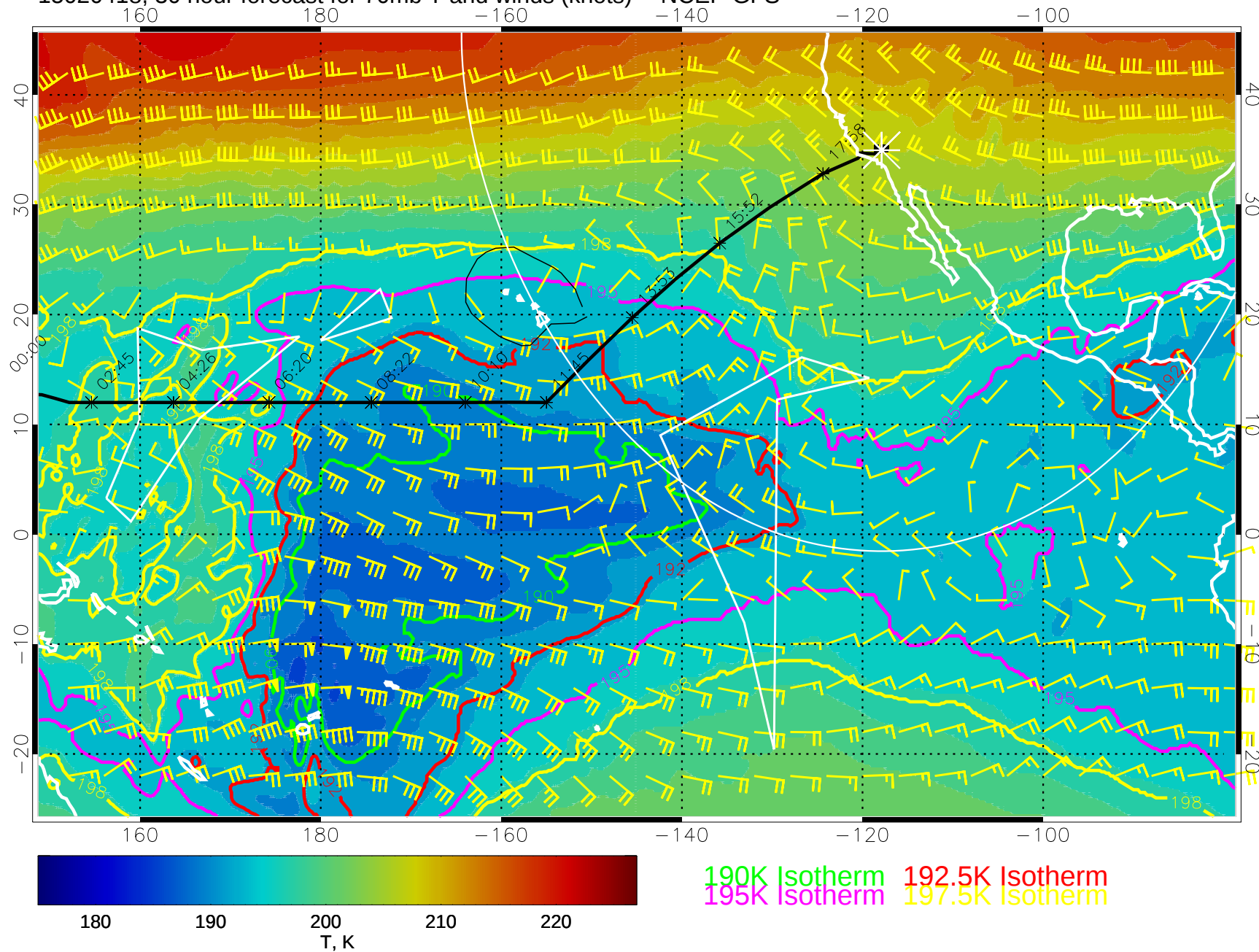
15020418, 30 hour forecast for 70mb T and winds (knots) -- NCEP GFS
