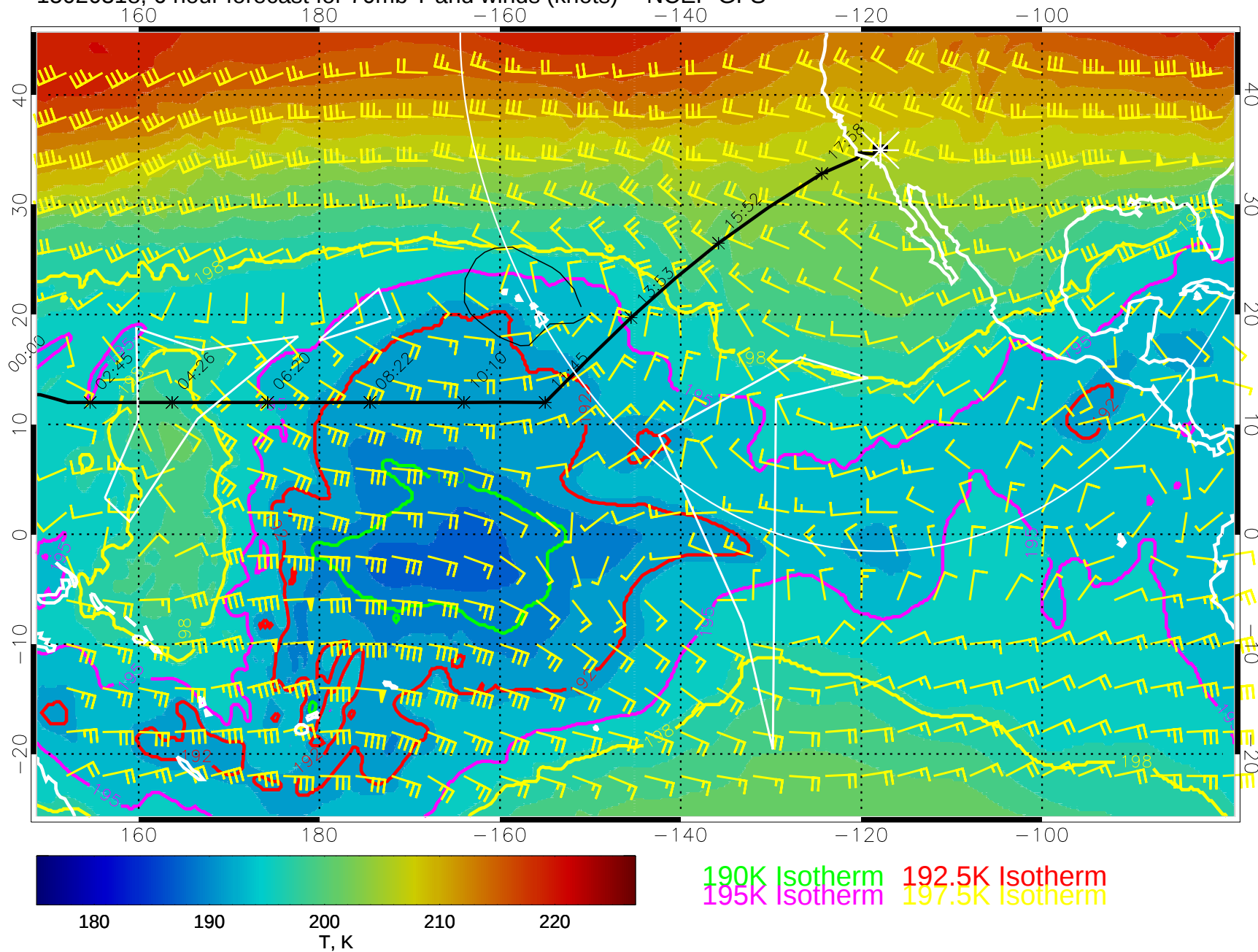
15020318, 6 hour forecast for 70mb T and winds (knots) -- NCEP GFS
