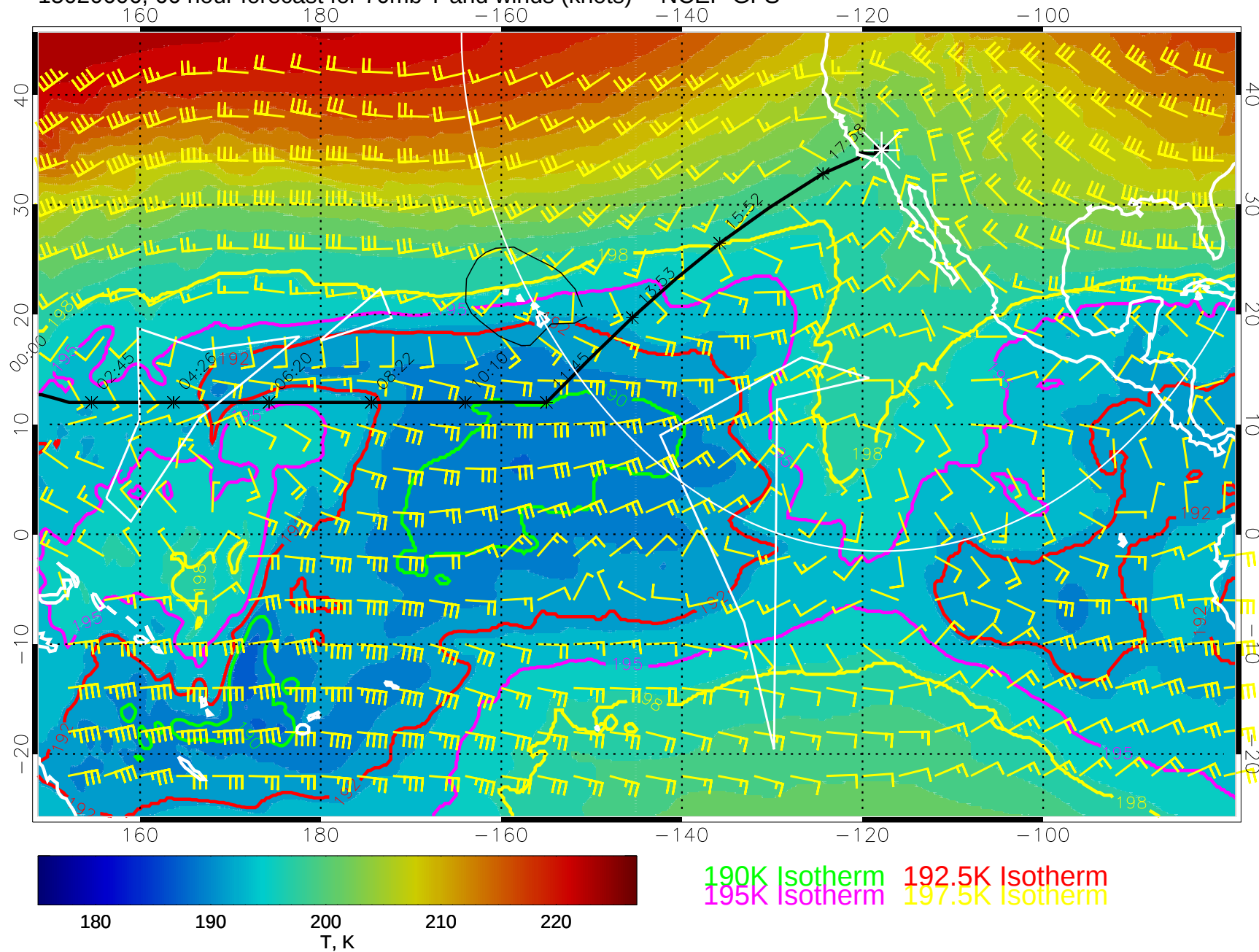
15020606, 66 hour forecast for 70mb T and winds (knots) -- NCEP GFS
