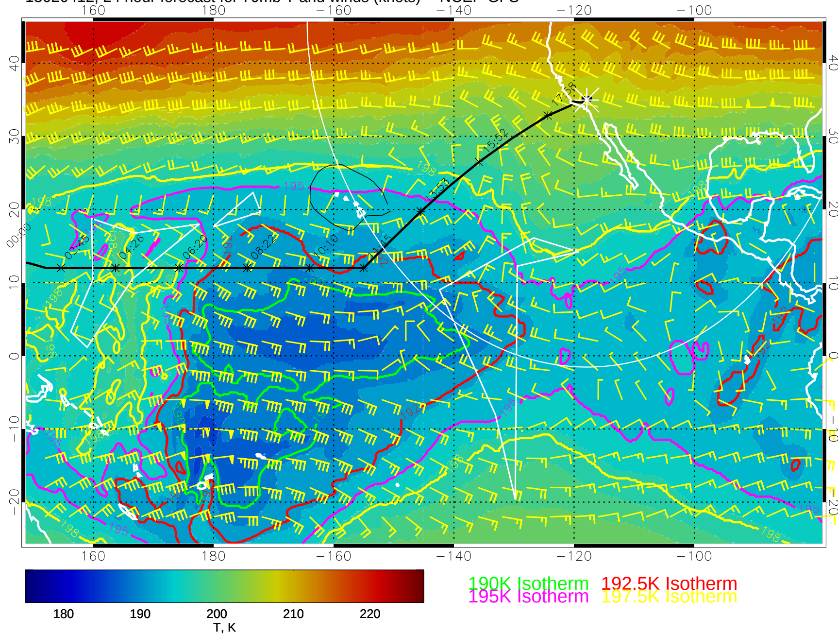
15020412, 24 hour forecast for 70mb T and winds (knots) -- NCEP GFS
