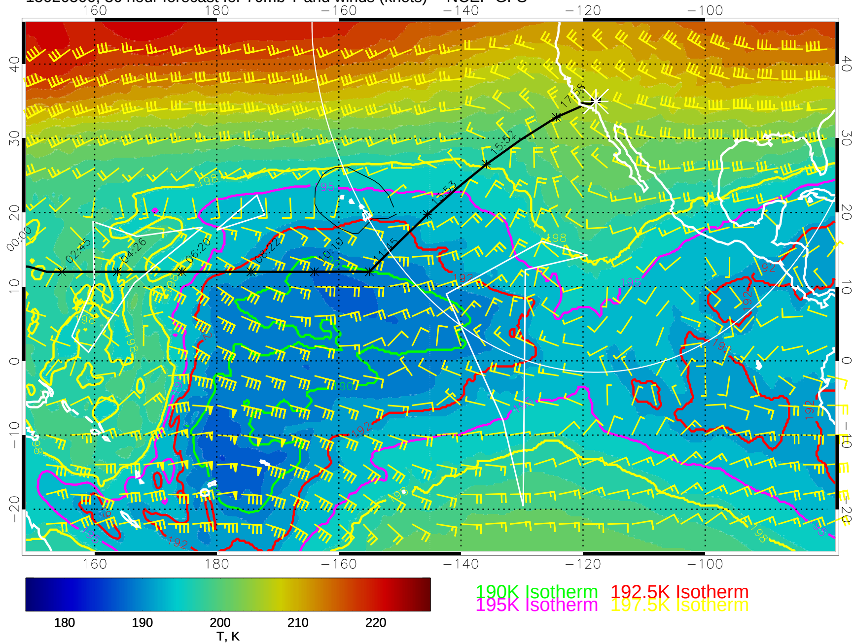
15020500, 36 hour forecast for 70mb T and winds (knots) -- NCEP GFS
