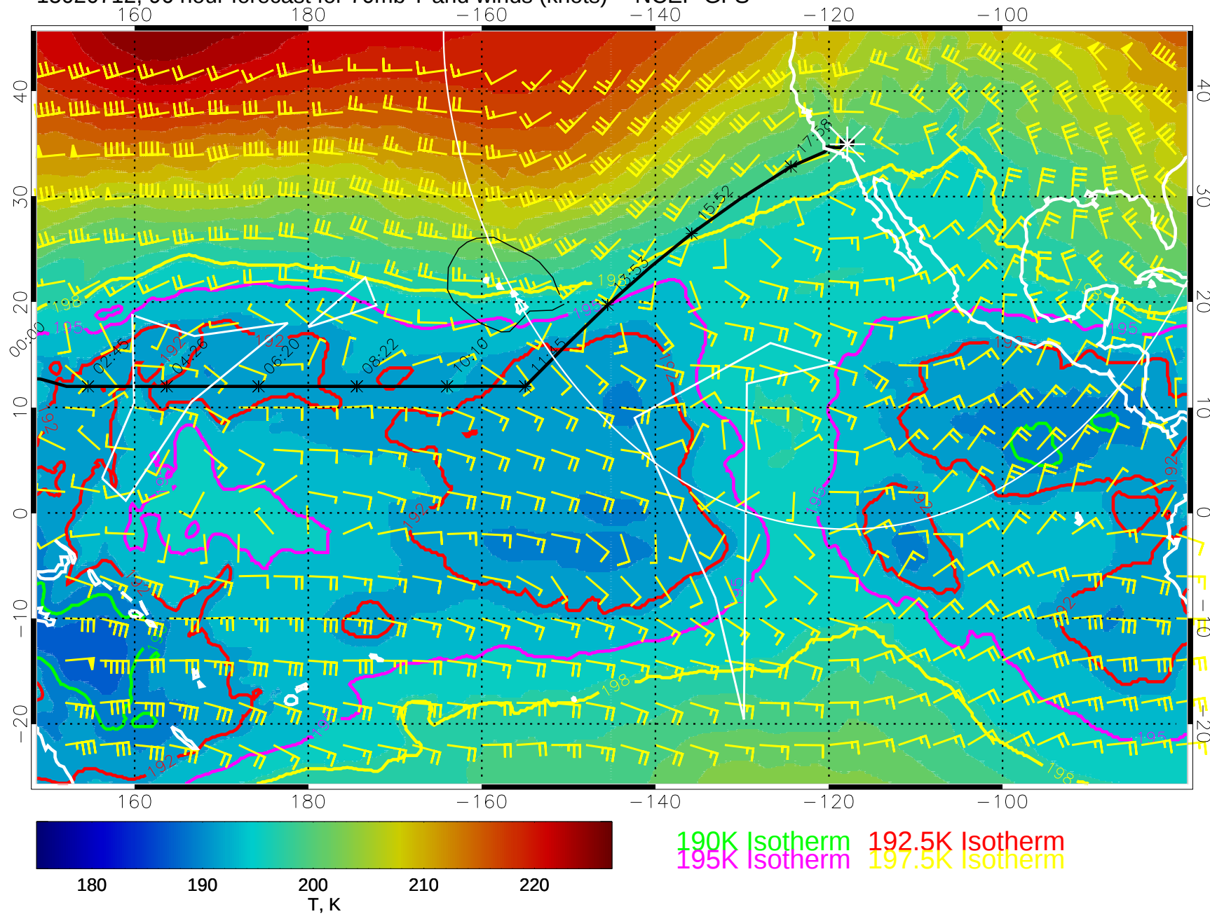
15020712, 96 hour forecast for 70mb T and winds (knots) -- NCEP GFS
