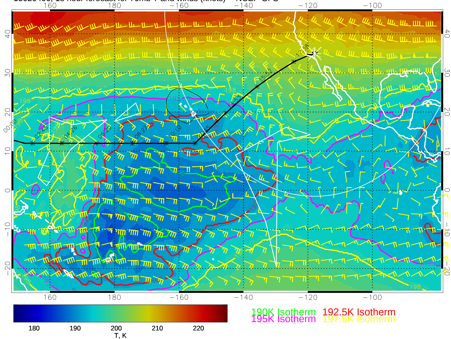
15020406, 18 hour forecast for 70mb T and winds (knots) -- NCEP GFS
