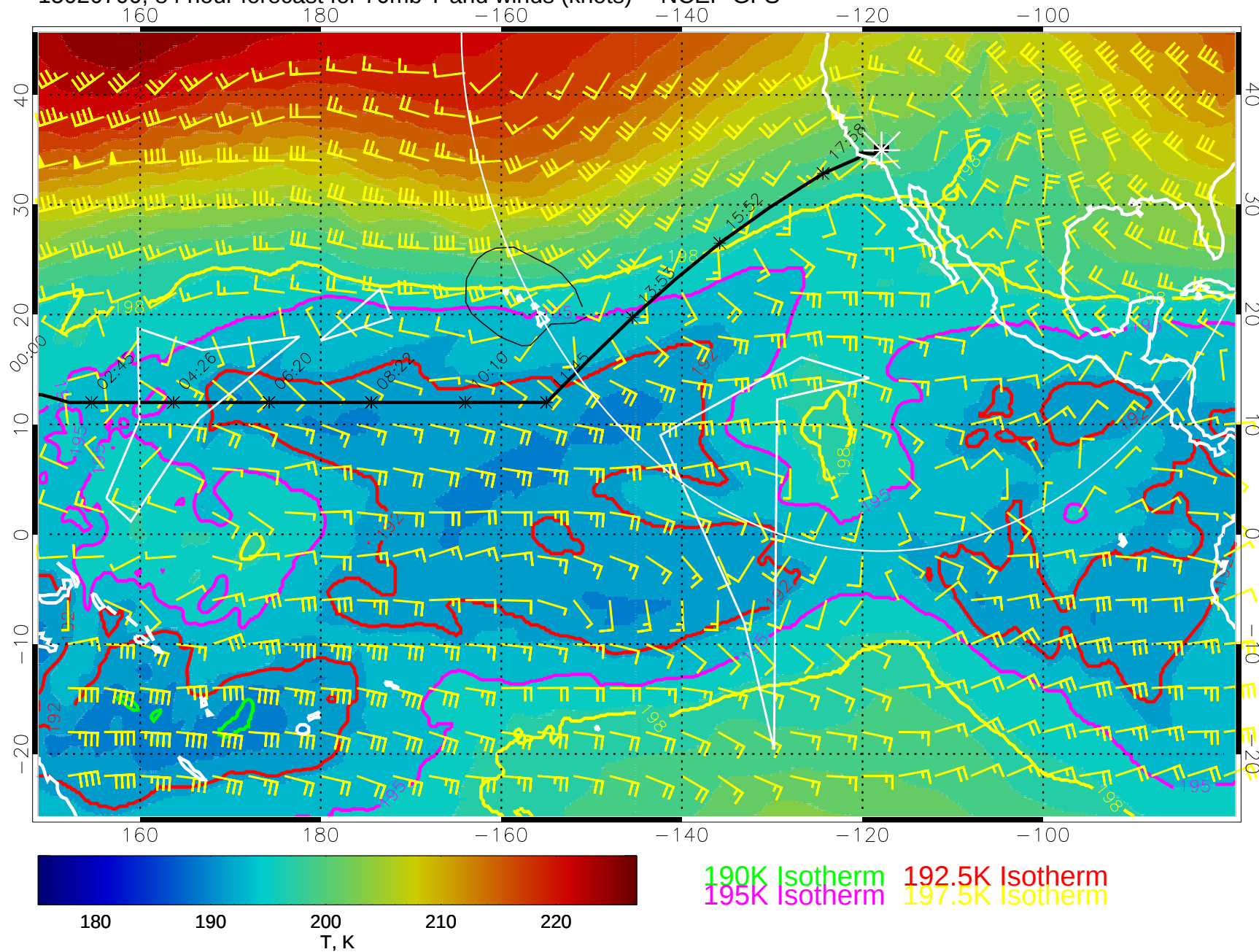
15020700, 84 hour forecast for 70mb T and winds (knots) -- NCEP GFS
