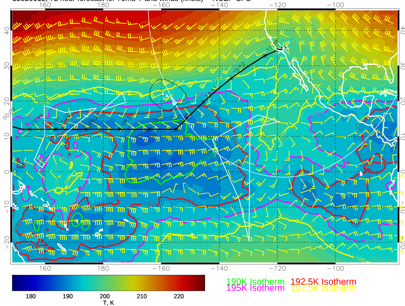
15020612, 72 hour forecast for 70mb T and winds (knots) -- NCEP GFS
