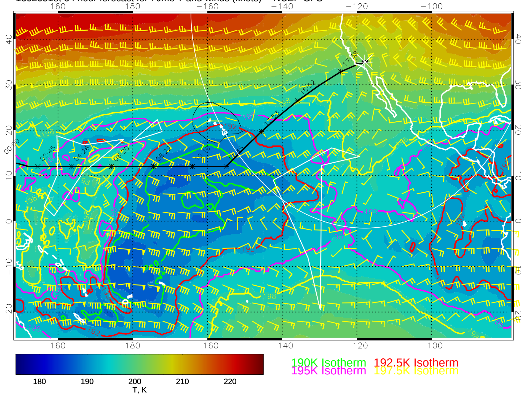
15020518, 54 hour forecast for 70mb T and winds (knots) -- NCEP GFS
