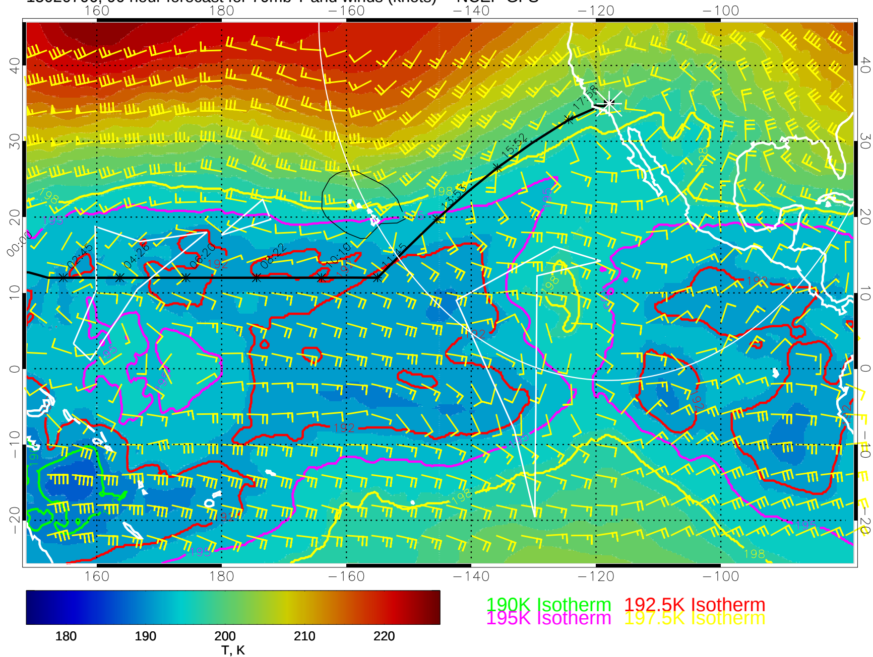
15020706, 90 hour forecast for 70mb T and winds (knots) -- NCEP GFS
