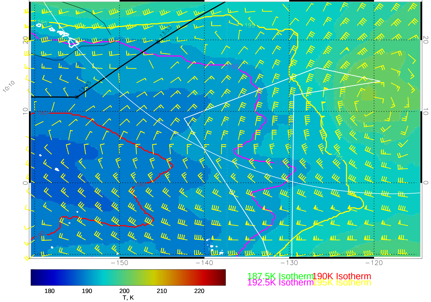
15020612, 72 hour forecast for 100mb T and winds (knots) -- NCEP GFS
