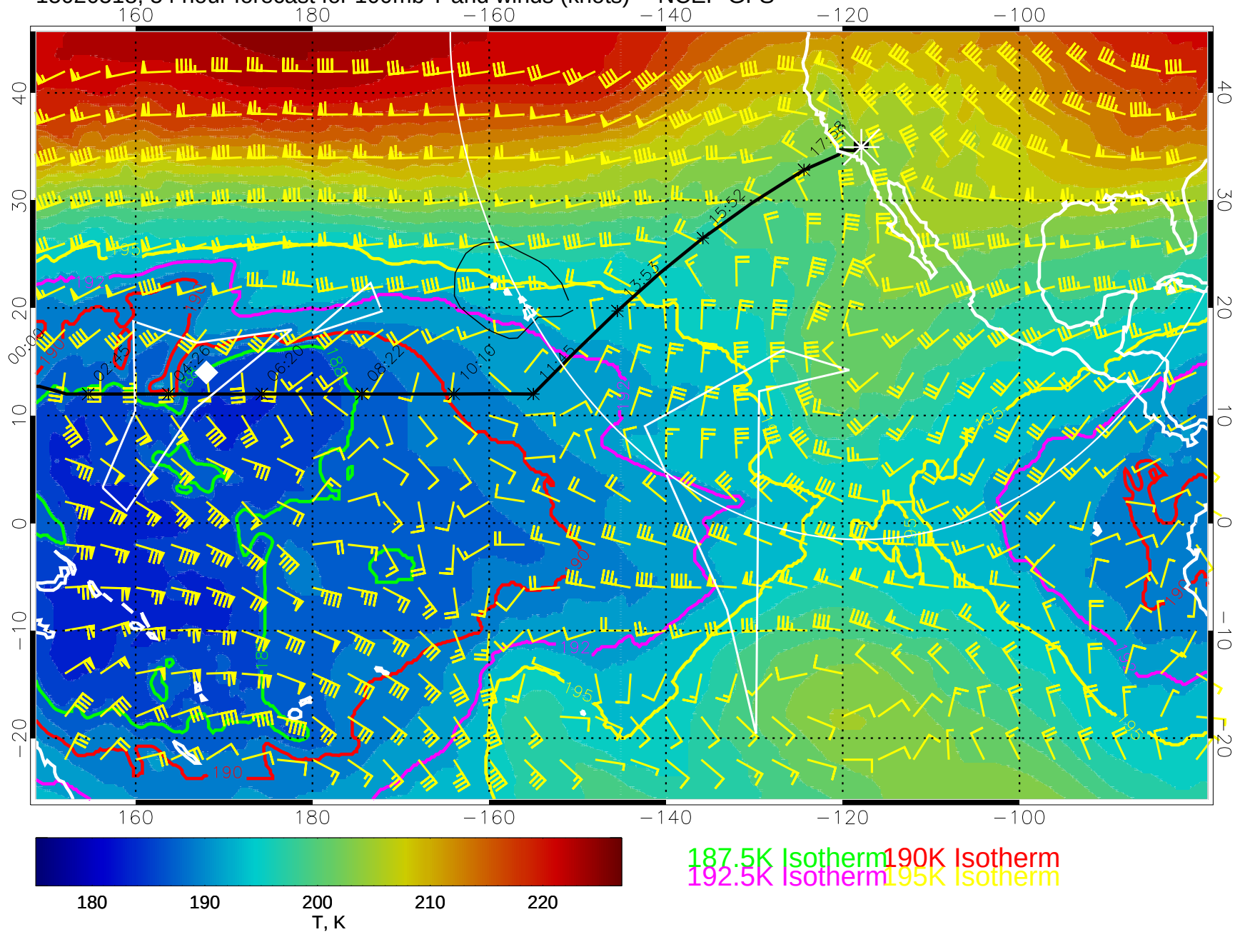
15020518, 54 hour forecast for 100mb T and winds (knots) -- NCEP GFS
