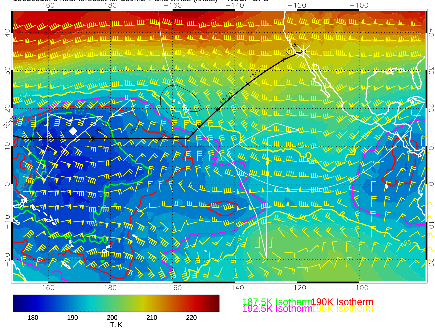
15020318, 6 hour forecast for 100mb T and winds (knots) -- NCEP GFS
