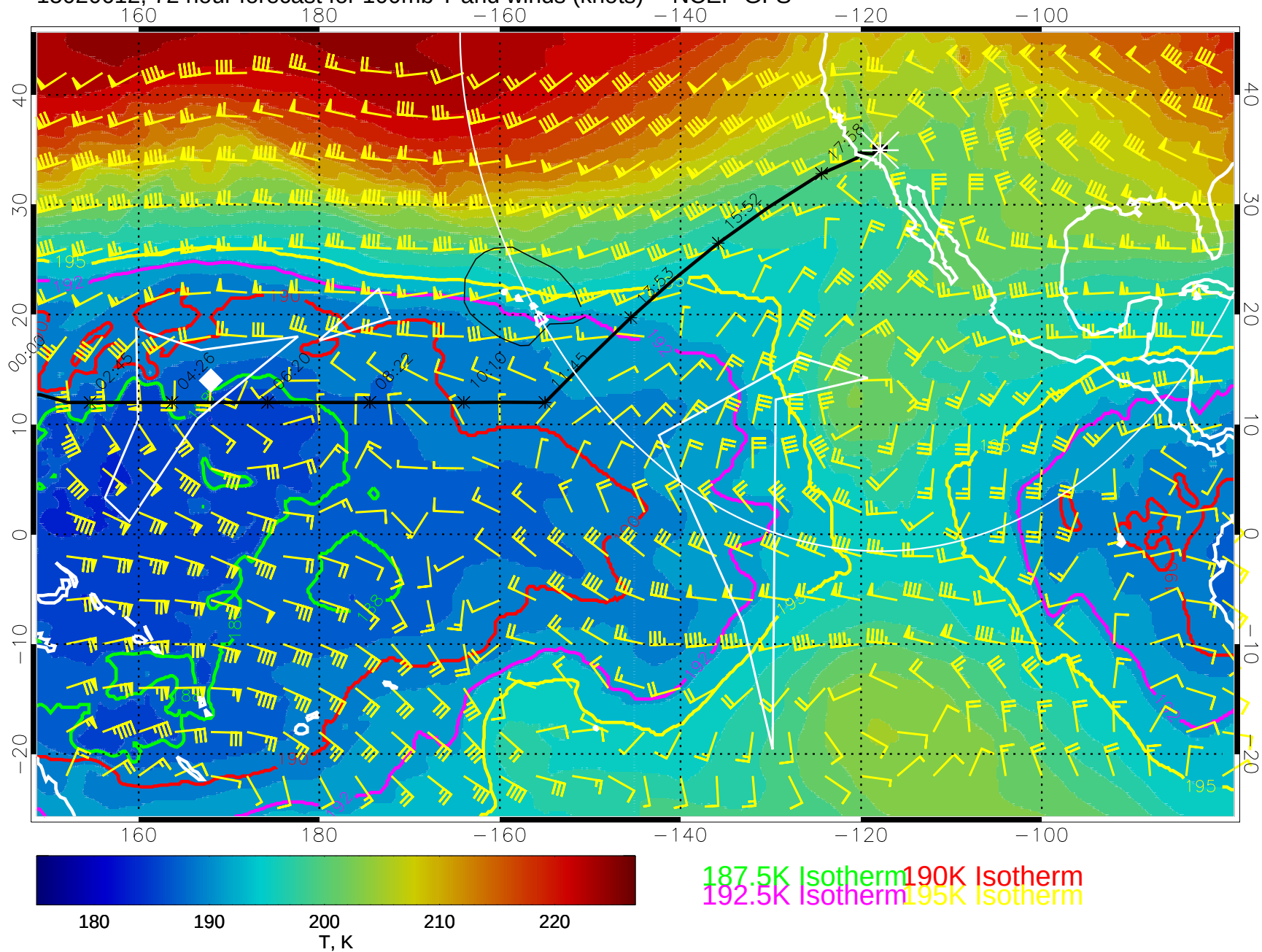
15020612, 72 hour forecast for 100mb T and winds (knots) -- NCEP GFS
