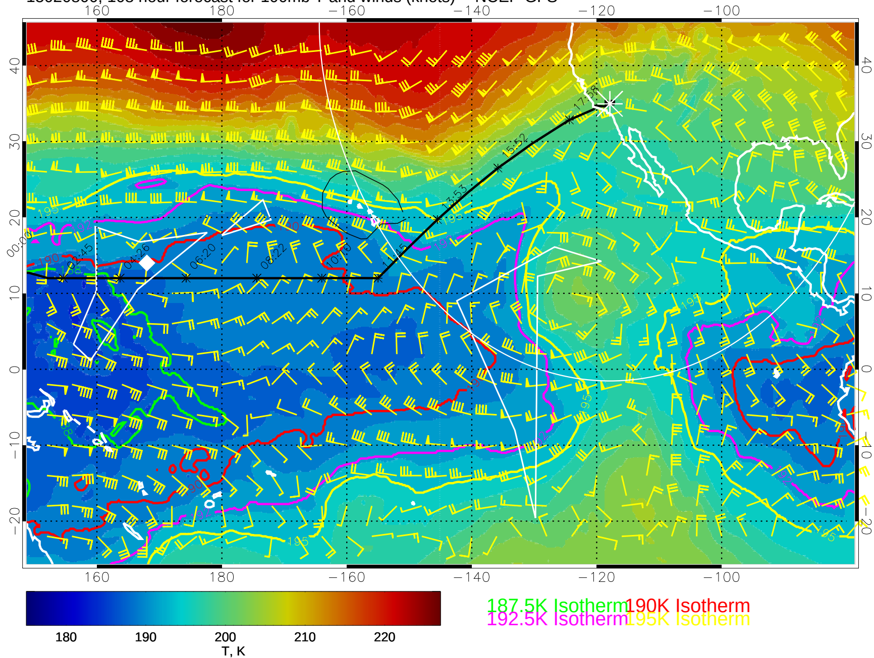
15020800, 108 hour forecast for 100mb T and winds (knots) -- NCEP GFS
