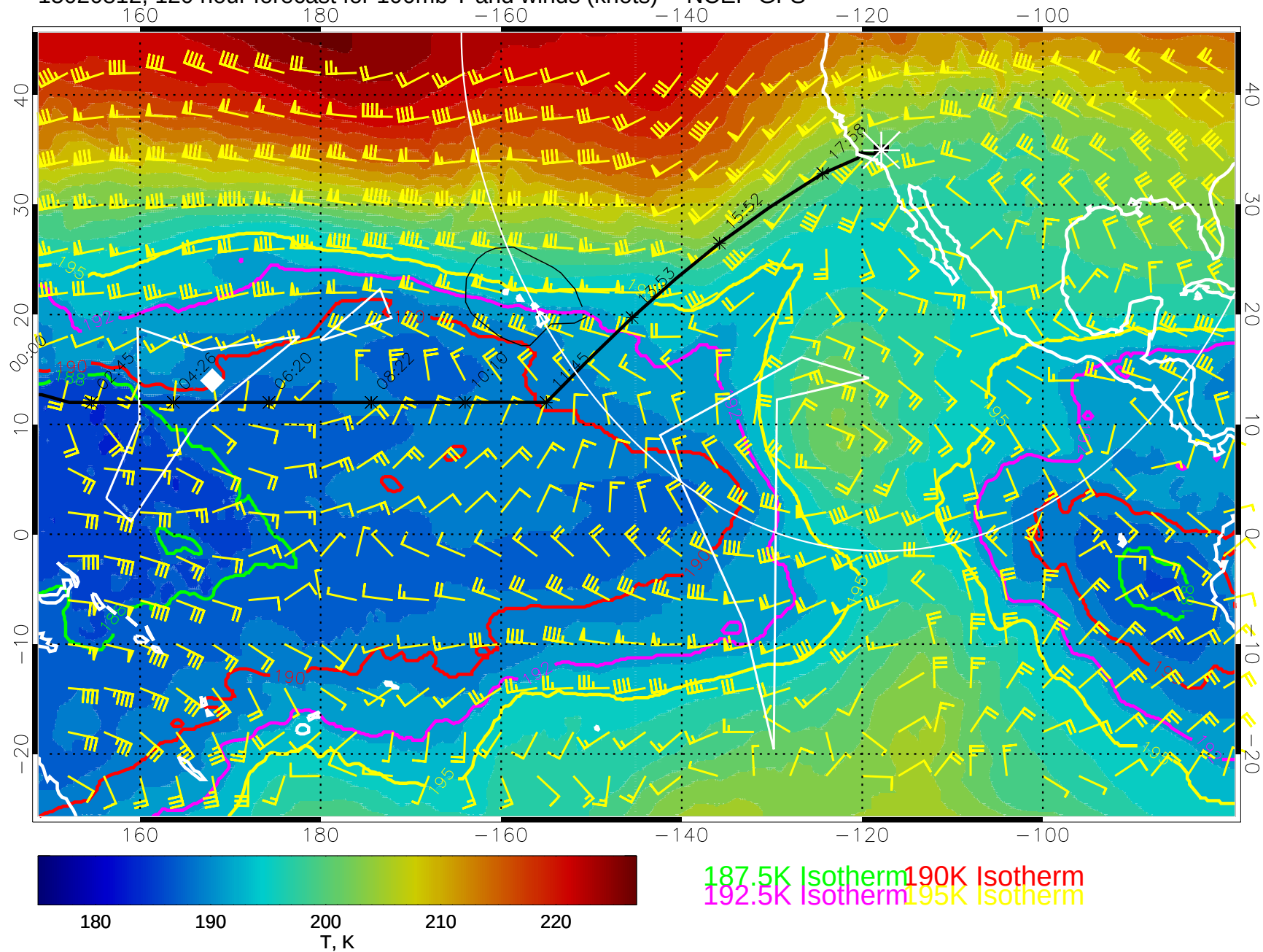
15020812, 120 hour forecast for 100mb T and winds (knots) -- NCEP GFS
