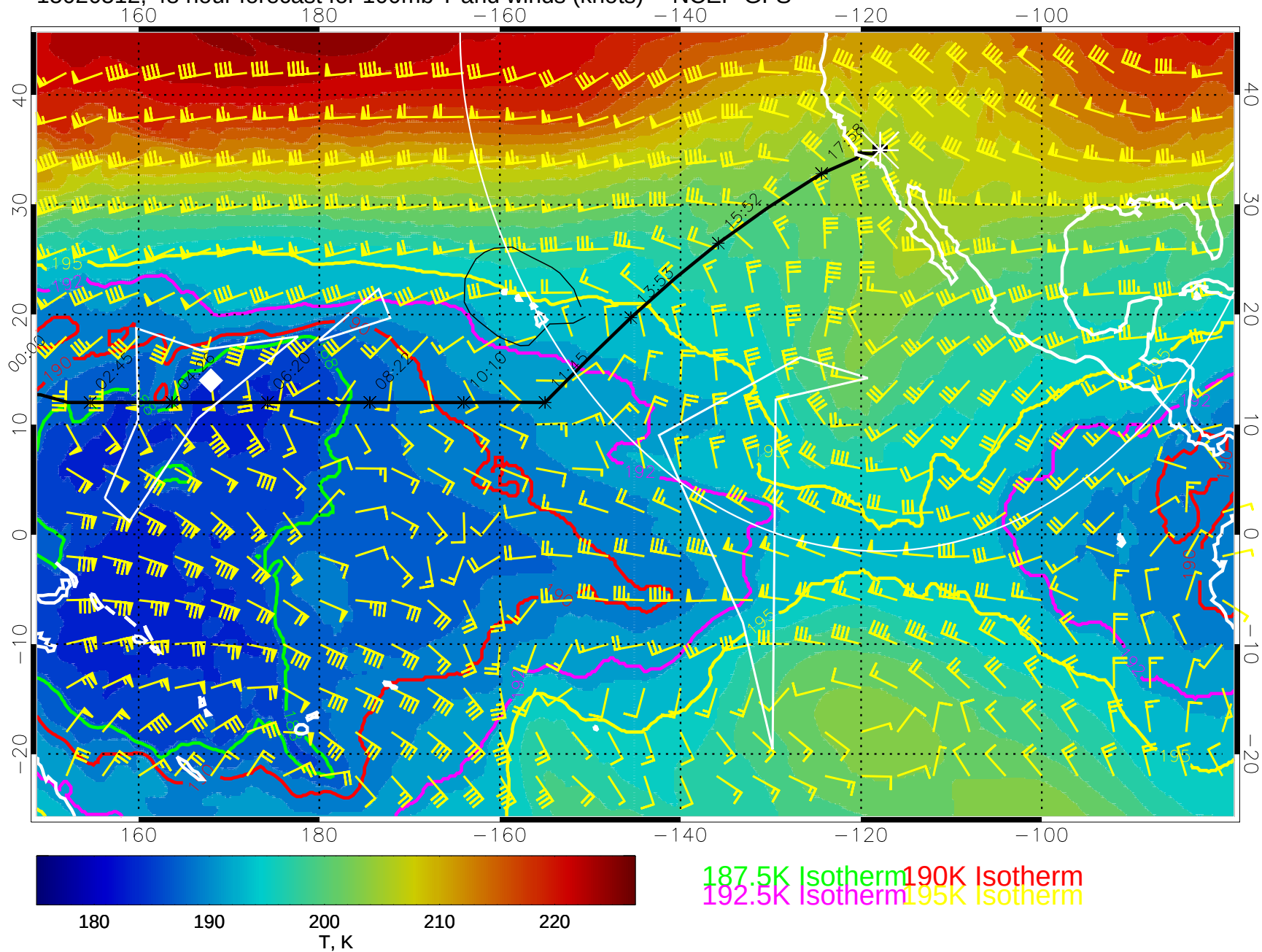
15020512, 48 hour forecast for 100mb T and winds (knots) -- NCEP GFS
